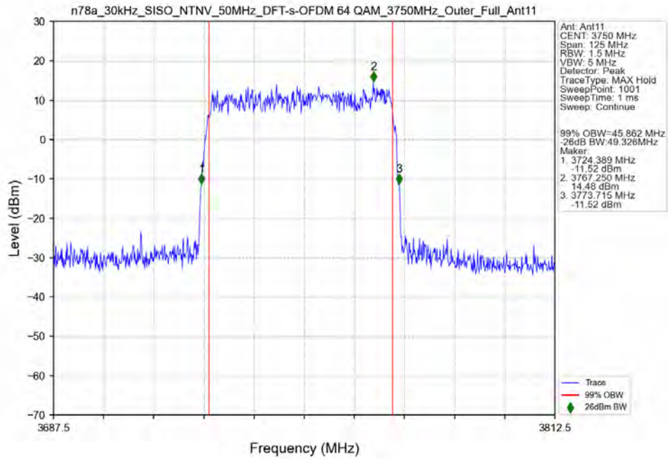
n78a_30kHz_SISO_NTNV_50MHz_DFT-s-OFDM_64_QAM_3750MHz_Outer_Full_Ant11
