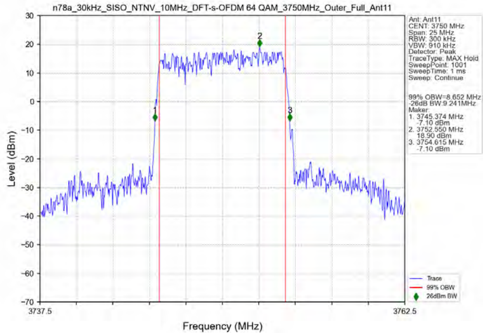
n78a_30kHz_SISO_NTNV_10MHz_DFT-s-OFDM_64_QAM_3750MHz_Outer_Full_Ant11
