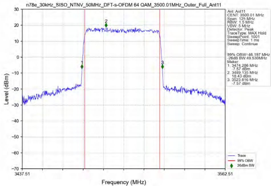
n78e_30kHz_SISO_NTNV_50MHz_DFT-s-OFDM_64_QAM_3500.01MHz_Outer_Full_Ant11
