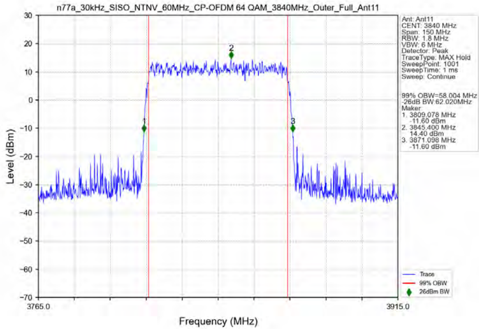
n77a_30kHz_SISO_NTNV_60MHz_CP-OFDM 64 QAM_3840MHz_Outer_Full_Ant11
