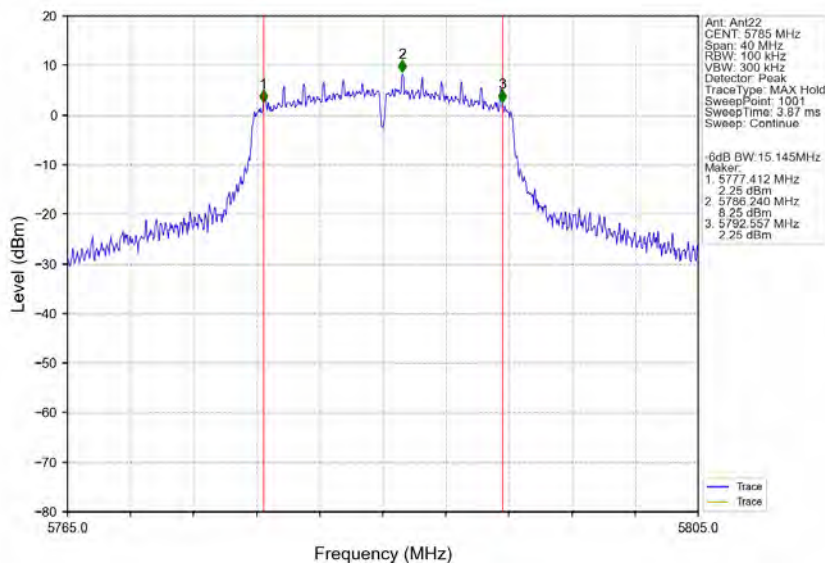
802.11a_MCH_5785MHz_Ant22_NTNV
