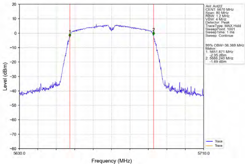
802.11ac(VHT40)_HCH_5670MHz_Ant22_NTNV
