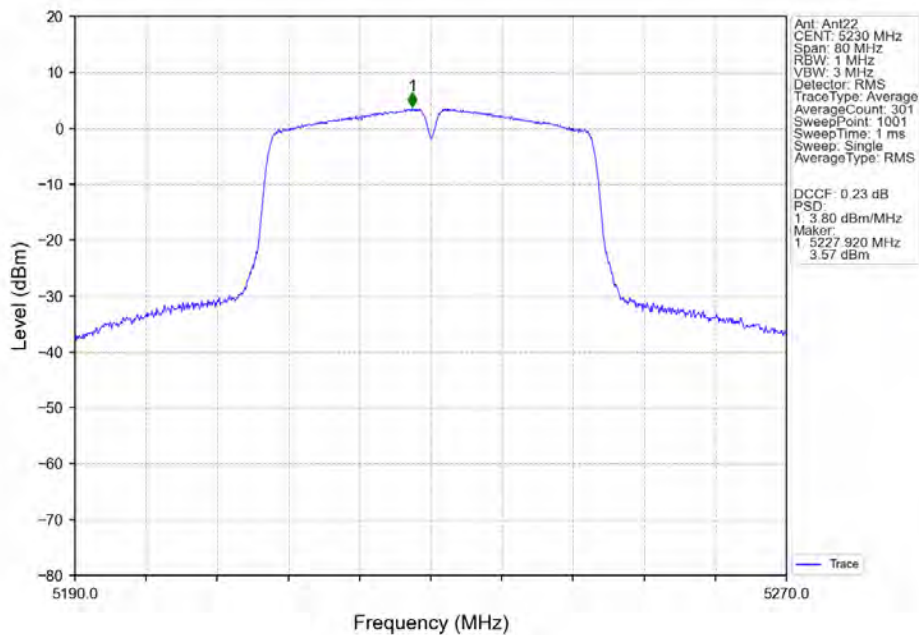
802.11ac(VHT40)_HCH_5230MHz_Ant22_NTNV
