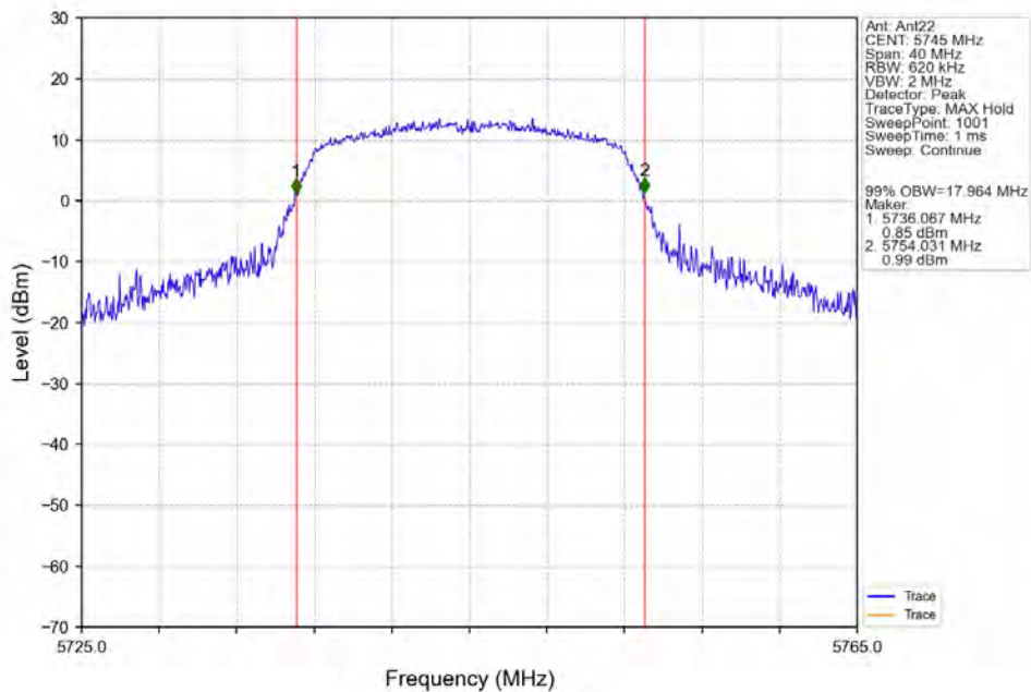
802.11a_LCH_5745MHz_Ant22_NTNV
