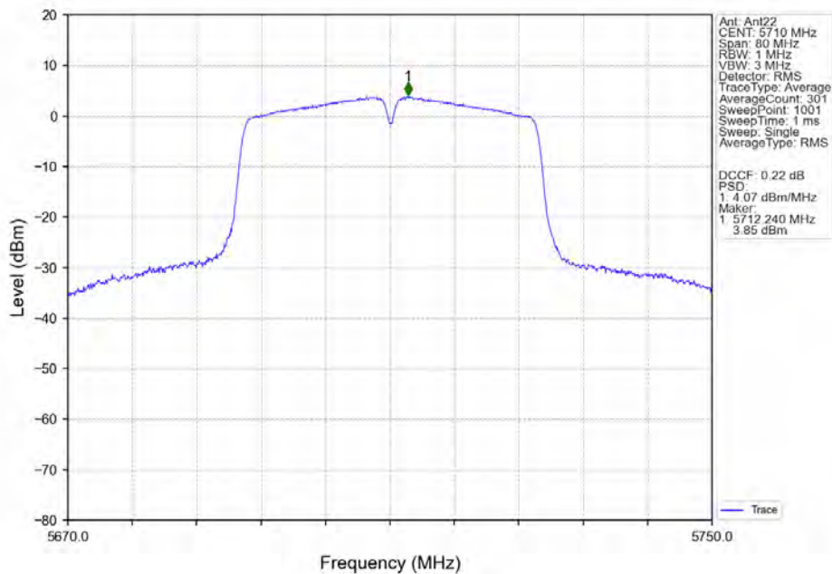
802.11ac(VHT40)_HCH_5710MHz_Ant22_NTNV
