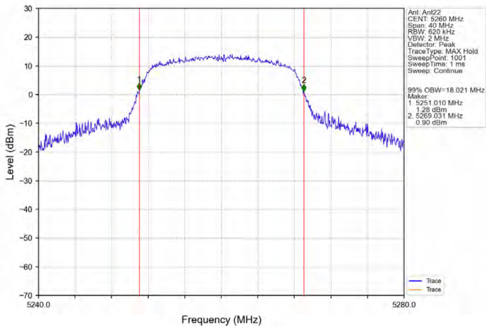
802.11a_LCH_5260MHz_Ant22_NTNV
