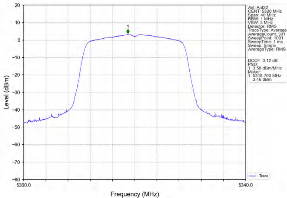
802.11ac(VHT20)_HCH_5320MHz_Ant22_NTNV
