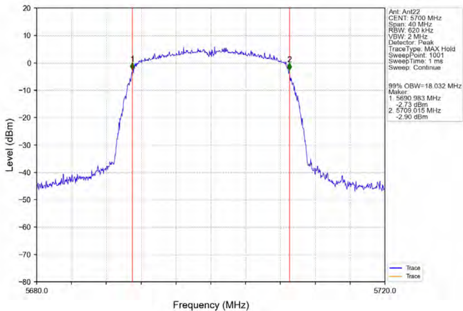
802.11n(HT20)_HCH_5700MHz_Ant22_NTNV
