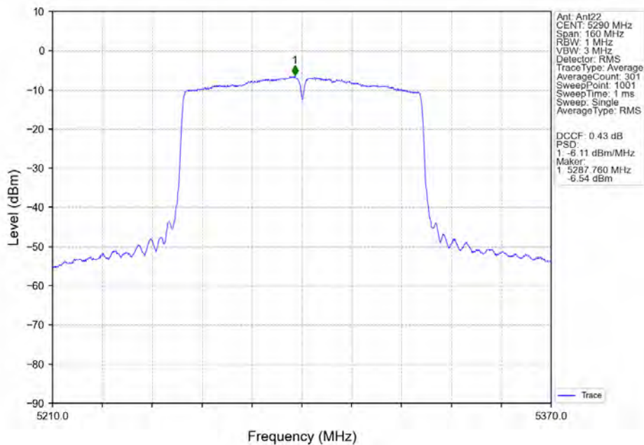
802.11ac(VHT80)_MCH_5290MHz_Ant22_NTNV
