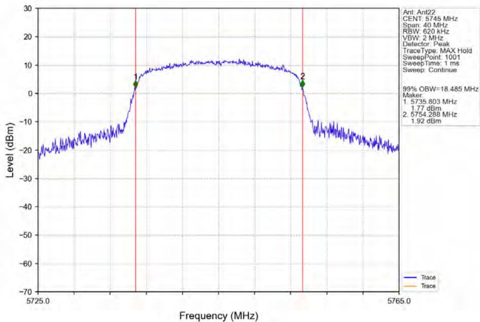
802.11ac(VHT20)_LCH_5745MHz_Ant22_NTNV
