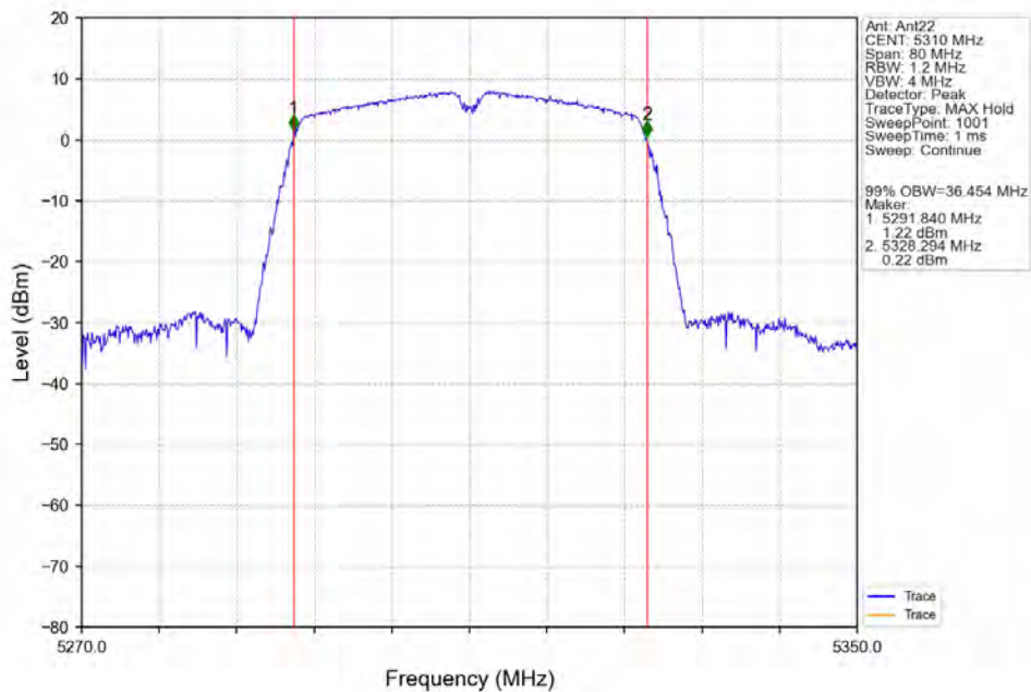
802.11n(HT40)_HCH_5310MHz_Ant22_NTNV
