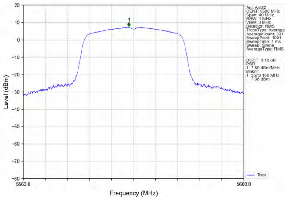
802.11n(HT20)_MCH_5580MHz_Ant22_NTNV
