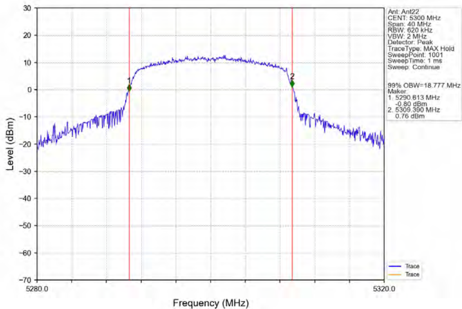
802.11n(HT20)_MCH_5300MHz_Ant22_NTNV
