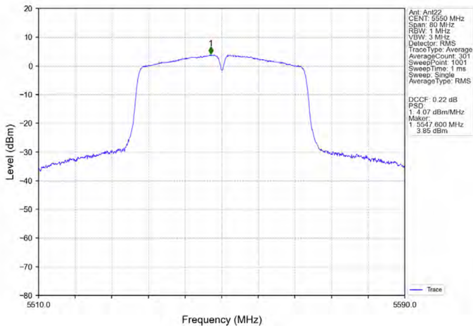
802.11ac(VHT40)_MCH_5550MHz_Ant22_NTNV
