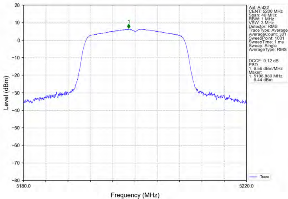
802.11ac(VHT20)_MCH_5200MHz_Ant22_NTNV
