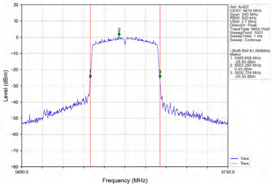
802.11ac(VHT80)_HCH_5610MHz_Ant22_NTNV
