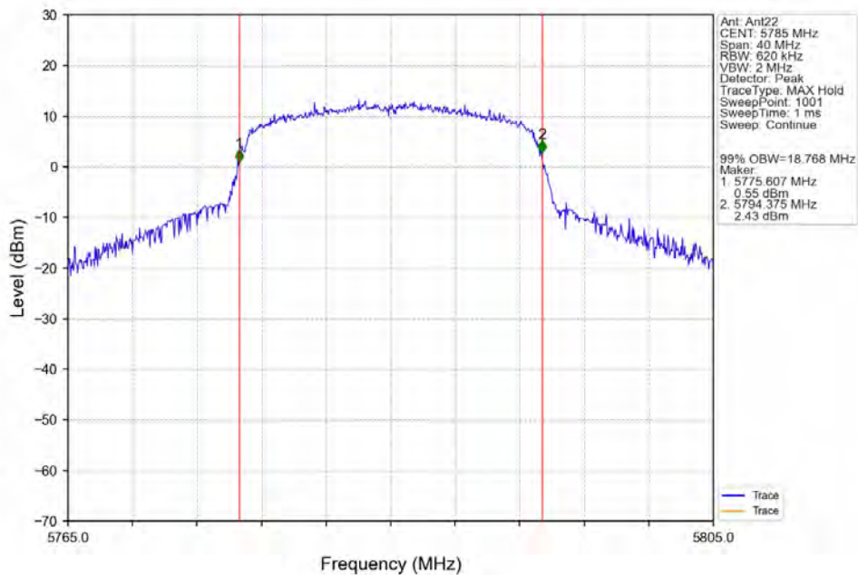
802.11n(HT20)_MCH_5785MHz_Ant22_NTNV
