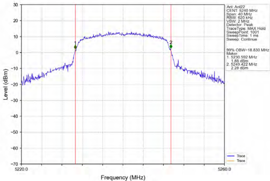
802.11n(HT20)_HCH_5240MHz_Ant22_NTNV
