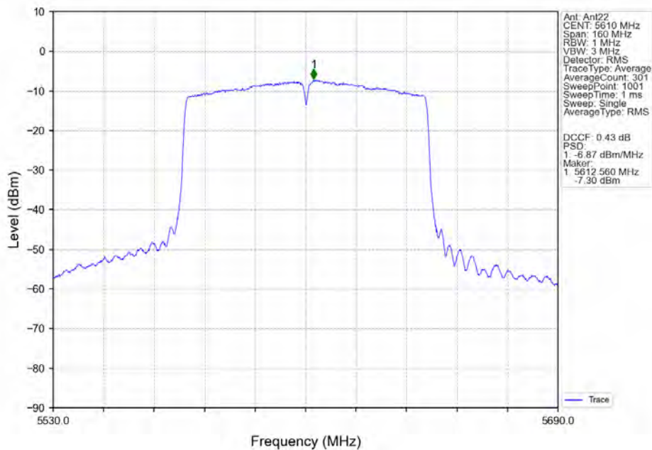
802.11ac(VHT80)_HCH_5610MHz_Ant22_NTNV
