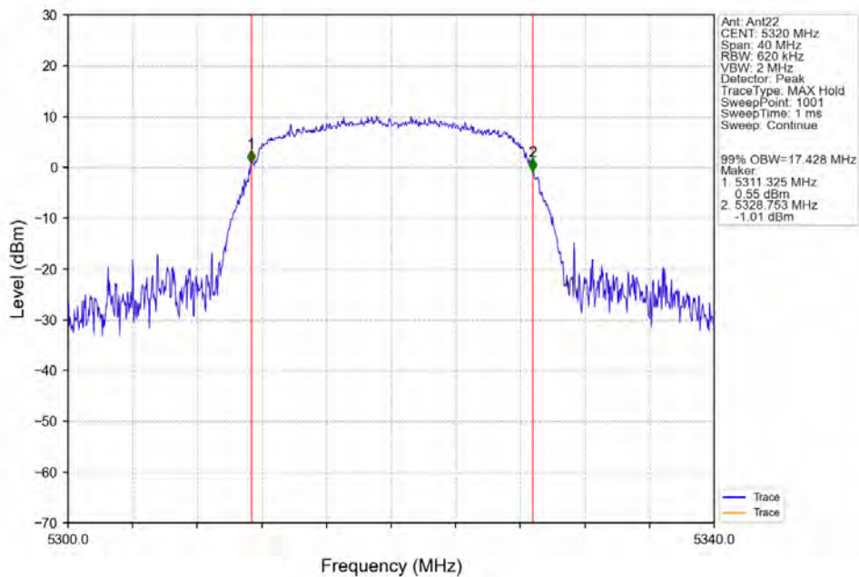
802.11a_HCH_5320MHz_Ant22_NTNV
