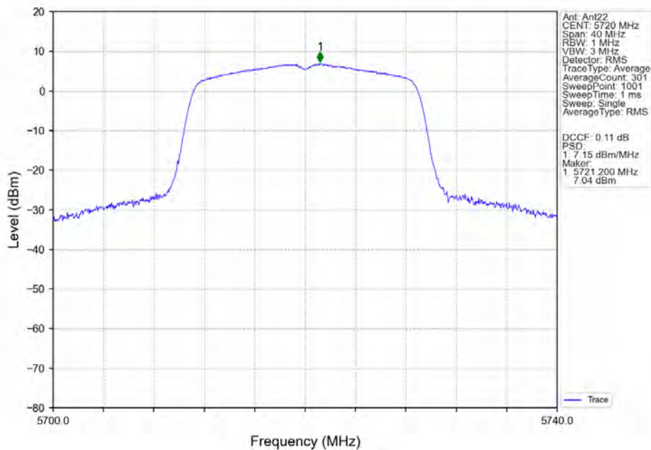
802.11ac(VHT20)_HCH_5720MHz_Ant22_NTNV
