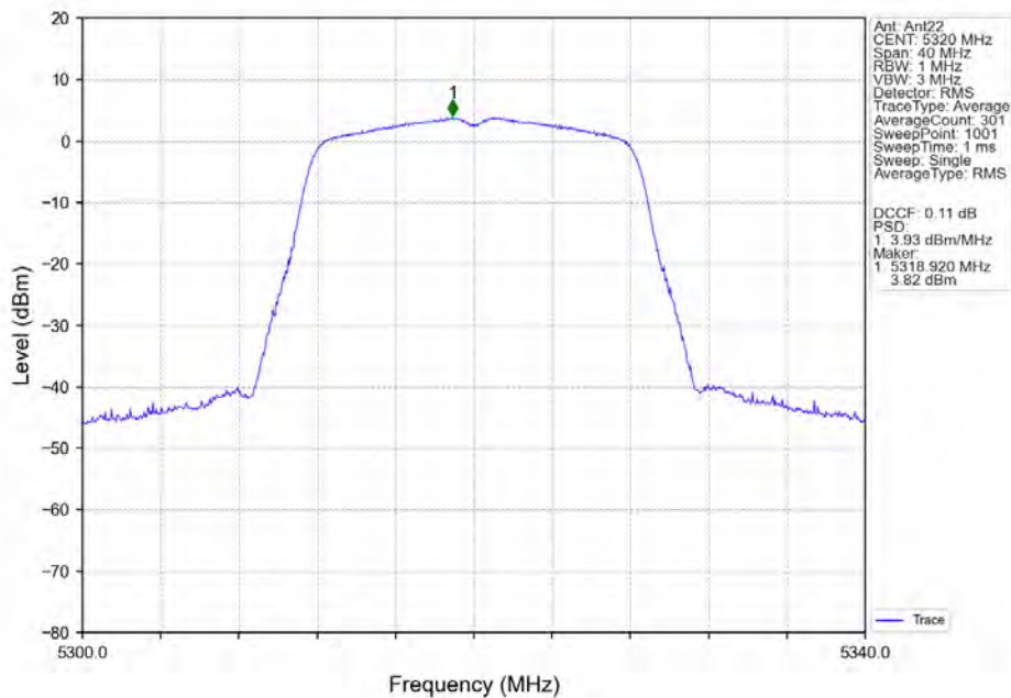
802.11a_HCH_5320MHz_Ant22_NTNV
