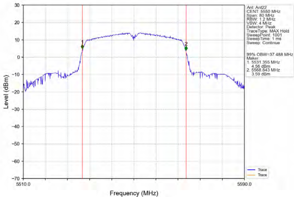
802.11n(HT40)_MCH_5550MHz_Ant22_NTNV
