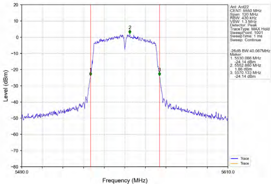
802.11n(HT40)_MCH_5550MHz_Ant22_NTNV
