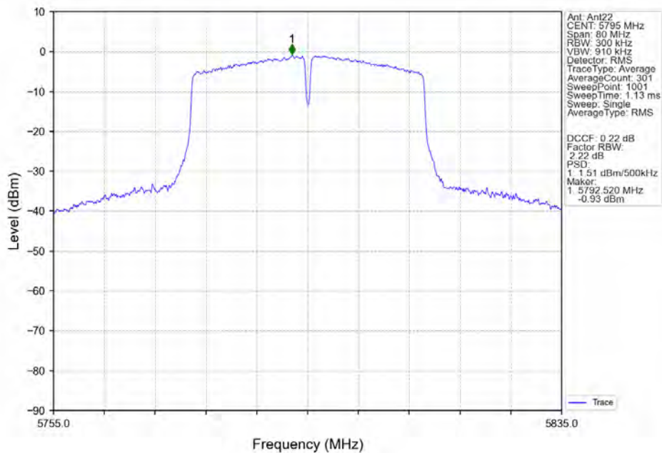
802.11n(HT40)_HCH_5795MHz_Ant22_NTNV
