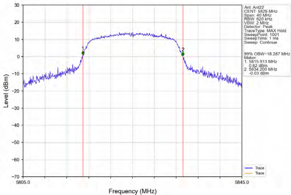
802.11a_HCH_5825MHz_Ant22_NTNV
