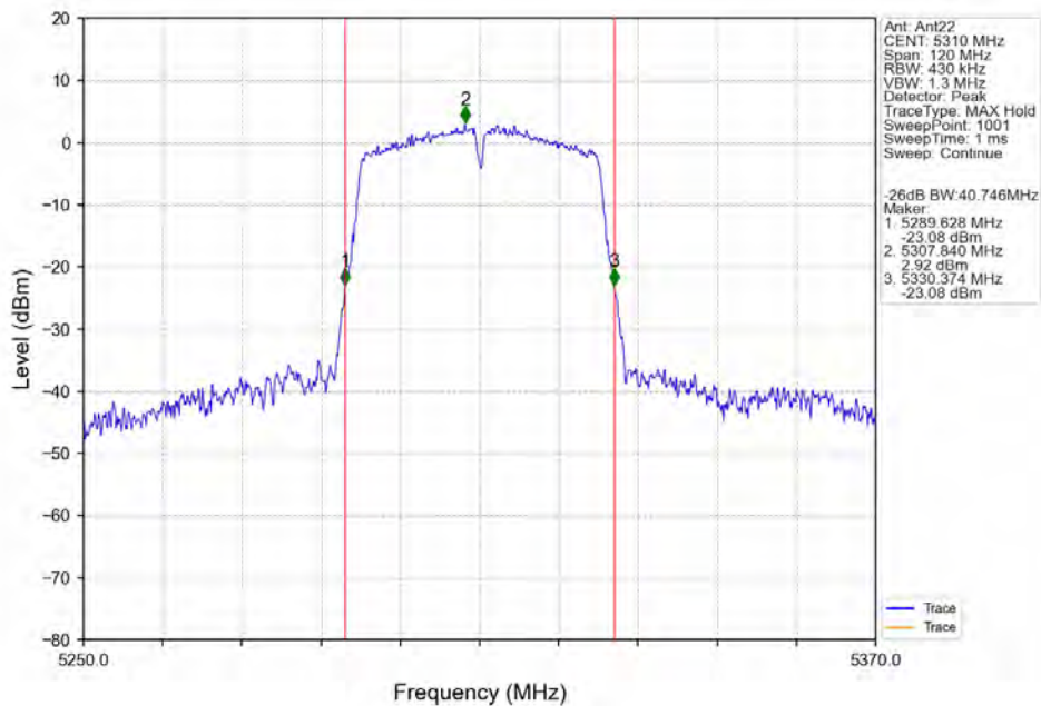
802.11n(HT40)_HCH_5310MHz_Ant22_NTNV
