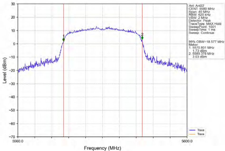
802.11ac(VHT20)_MCH_5580MHz_Ant22_NTNV
