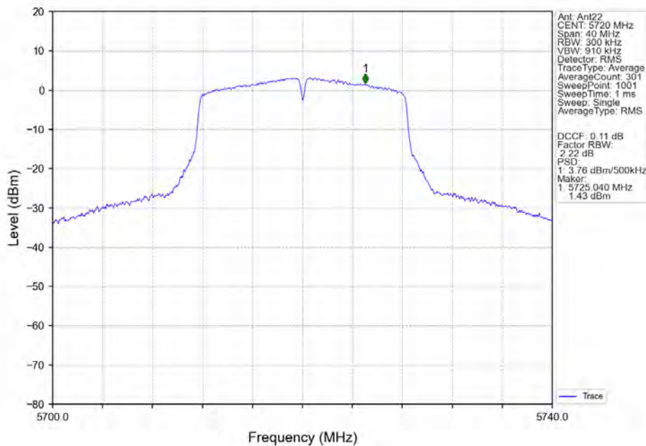
802.11a_HCH_5720MHz_Ant22_NTNV
