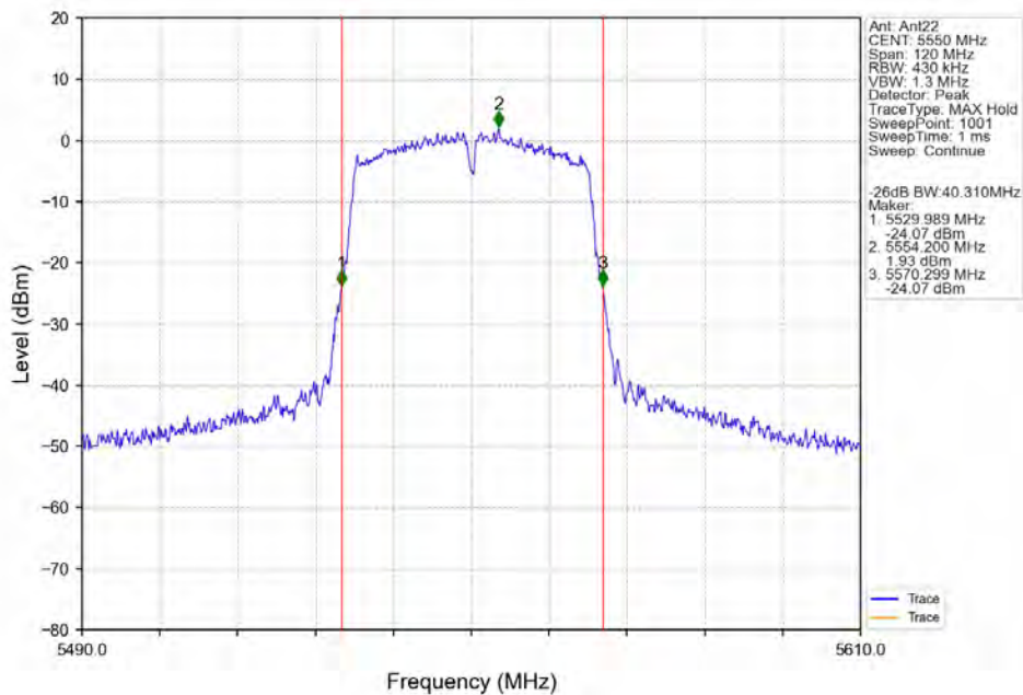
802.11ac(VHT40)_MCH_5550MHz_Ant22_NTNV
