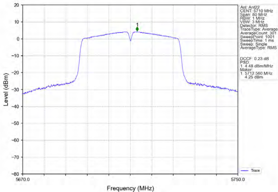
802.11n(HT40)_HCH_5710MHz_Ant22_NTNV
