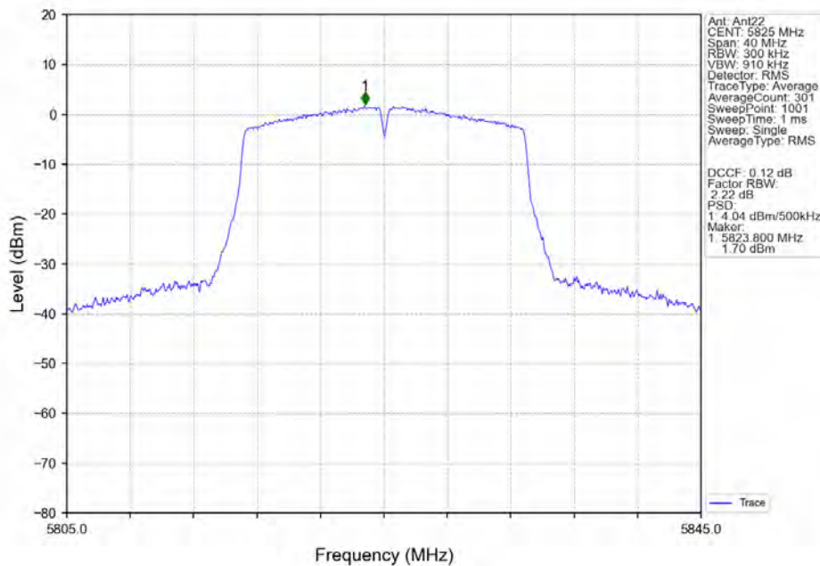
802.11ac(VHT20)_HCH_5825MHz_Ant22_NTNV
