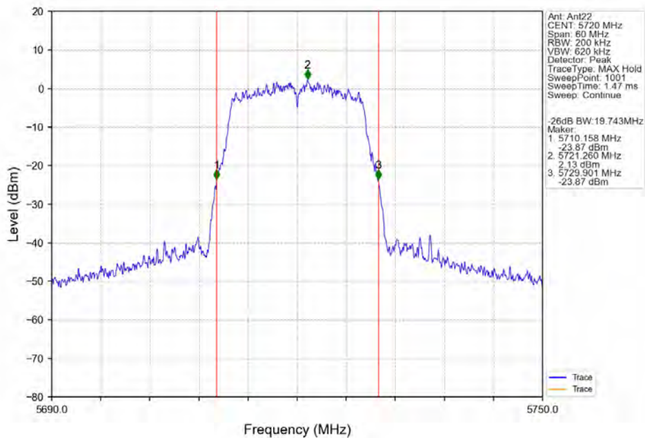
802.11a_HCH_5720MHz_Ant22_NTNV
