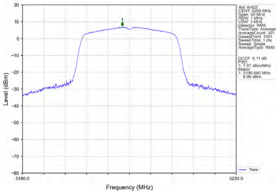
802.11n(HT20)_MCH_5200MHz_Ant22_NTNV
