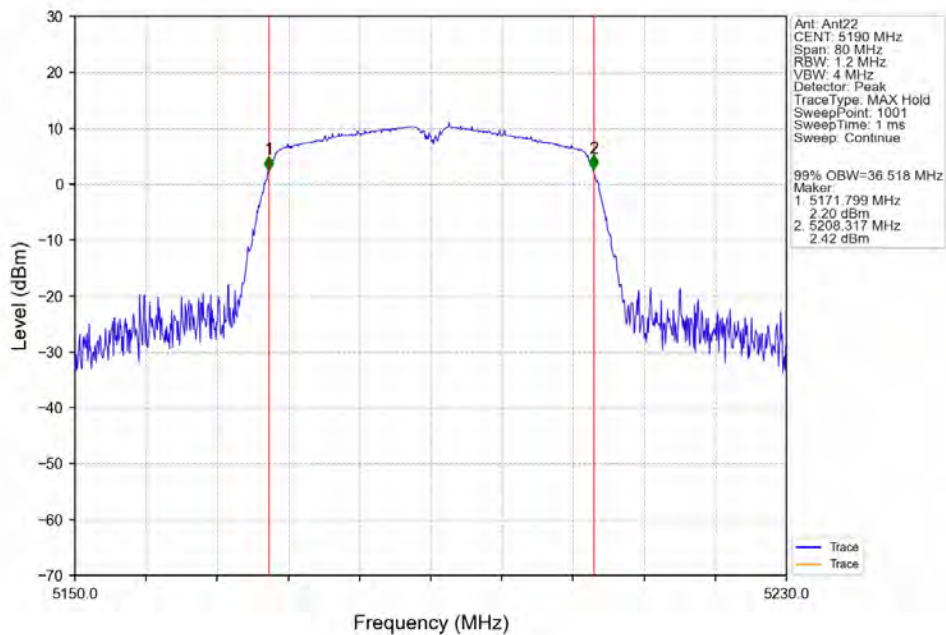
802.11ac(VHT40)_LCH_5190MHz_Ant22_NTNV
