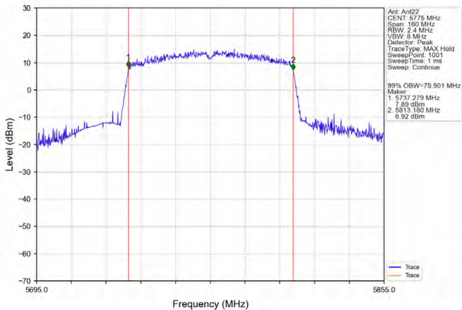
802.11ac(VHT80)_MCH_5775MHz_Ant22_NTNV
