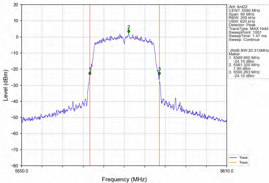
802.11n(HT20)_MCH_5580MHz_Ant22_NTNV
