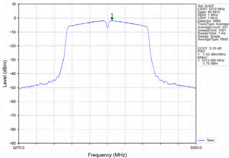
802.11ac(VHT40)_HCH_5310MHz_Ant22_NTNV
