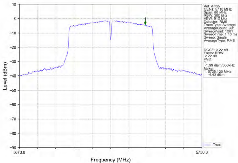
802.11ac(VHT40)_HCH_5710MHz_Ant22_NTNV
