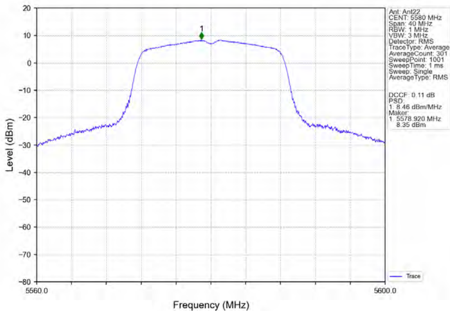
802.11a_MCH_5580MHz_Ant22_NTNV
