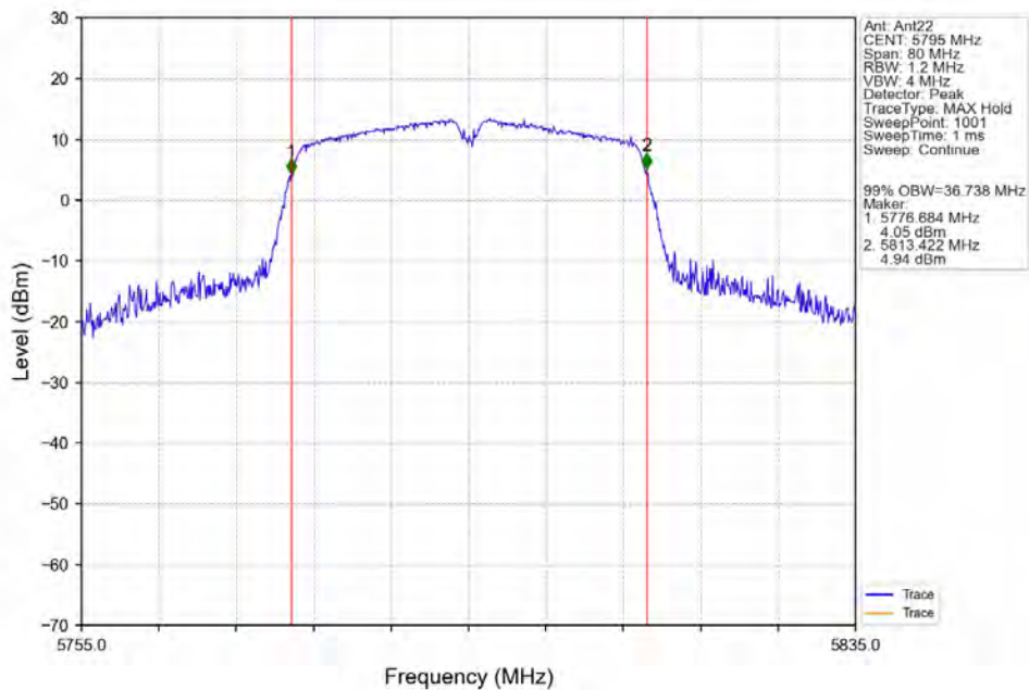
802.11ac(VHT40)_HCH_5795MHz_Ant22_NTNV
