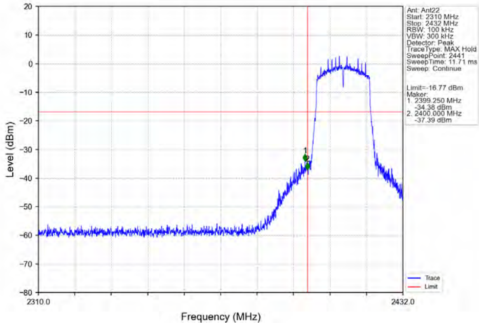
802.11ac(VHT20)_LCH_2412MHz_Ant22_NTNV
