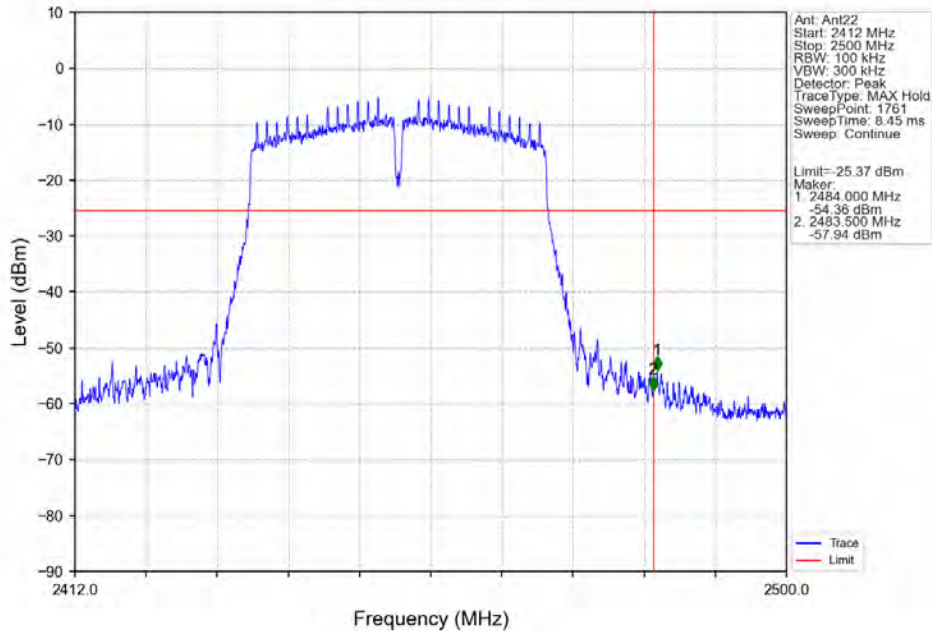
802.11n(HT40)_HCH_2452MHz_Ant22_NTNV
