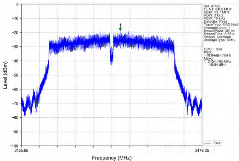
802.11ac(VHT40)_HCH_2452MHz_Ant22_NTNV
