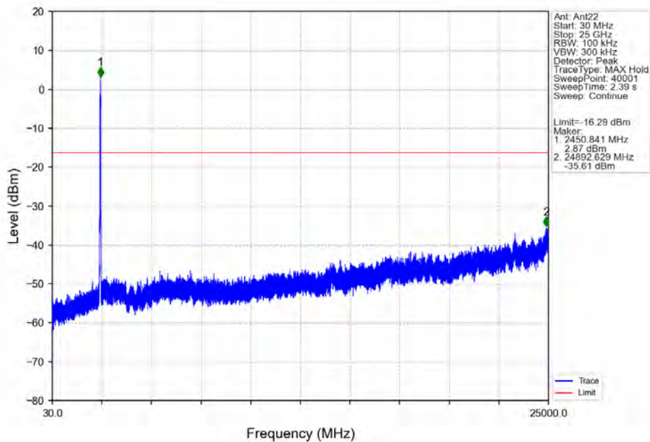
802.11ac(VHT40)_HCH_2447MHz_Ant22_NTNV
