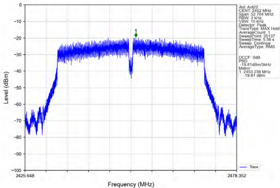
802.11n(HT40)_HCH_2452MHz_Ant22_NTNV
