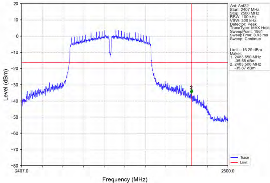
802.11ac(VHT40)_HCH_2447MHz_Ant22_NTNV
