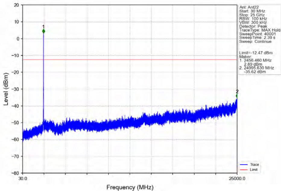
802.11g_HCH_2457MHz_Ant22_NTNV
