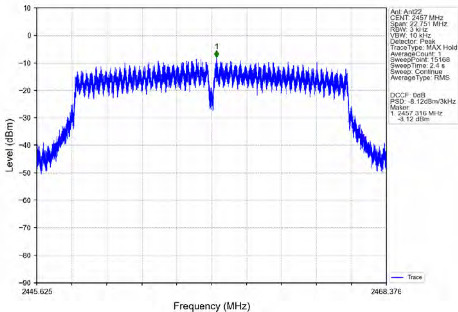
802.11ac(VHT20)_HCH_2457MHz_Ant22_NTNV
