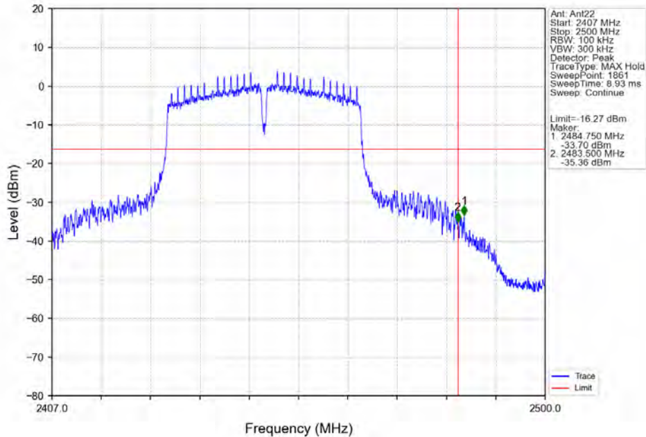
802.11n(HT40)_HCH_2447MHz_Ant22_NTNV
