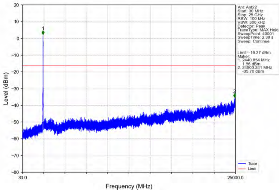
802.11n(HT40)_HCH_2447MHz_Ant22_NTNV
