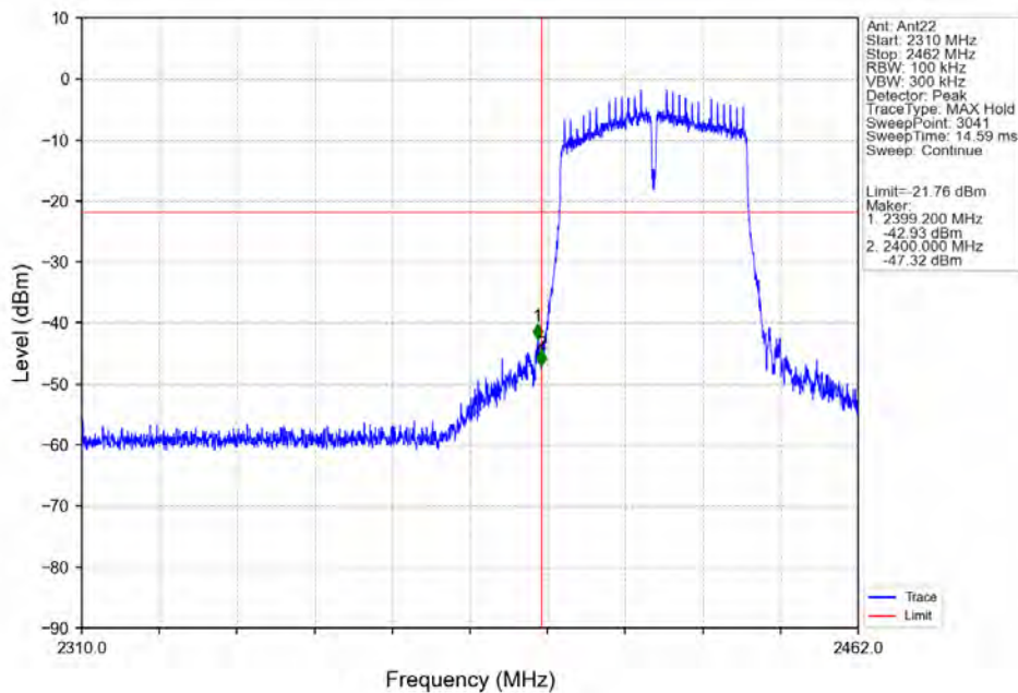
802.11ac(VHT40)_LCH_2422MHz_Ant22_NTNV
