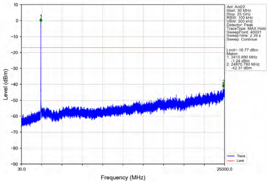
802.11ac(VHT20)_LCH_2412MHz_Ant22_NTNV
