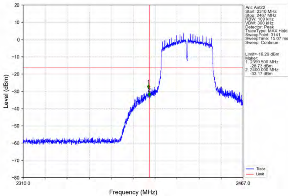
802.11ac(VHT40)_LCH_2427MHz_Ant22_NTNV
