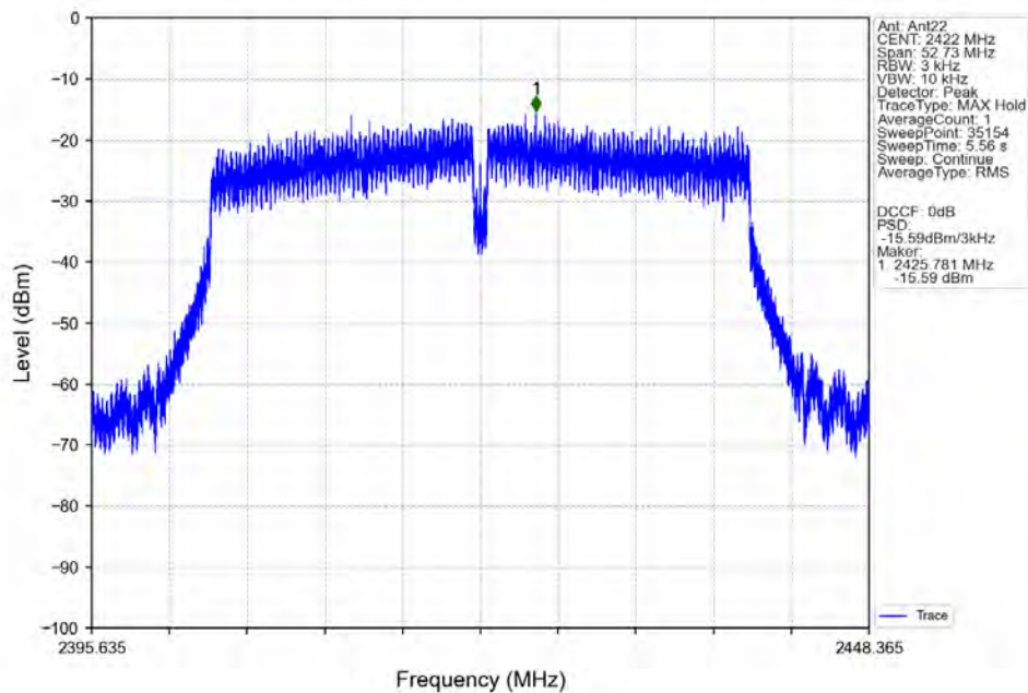
802.11ac(VHT40)_LCH_2422MHz_Ant22_NTNV
