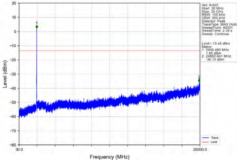
802.11n(HT20)_HCH_2462MHz_Ant22_NTNV
