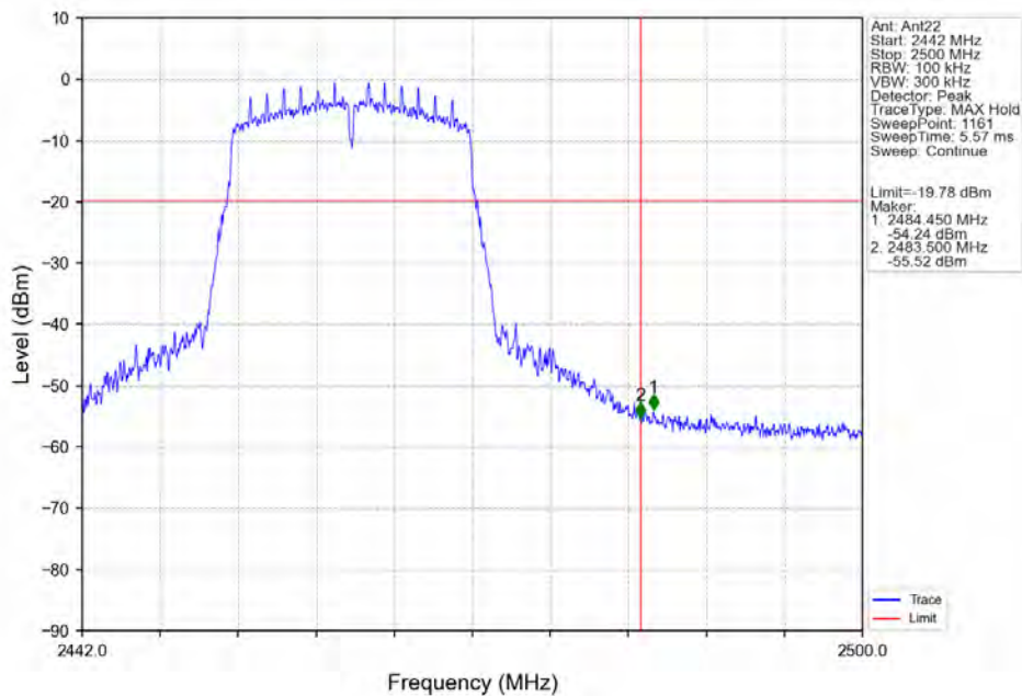
802.11n(HT20)_HCH_2462MHz_Ant22_NTNV
