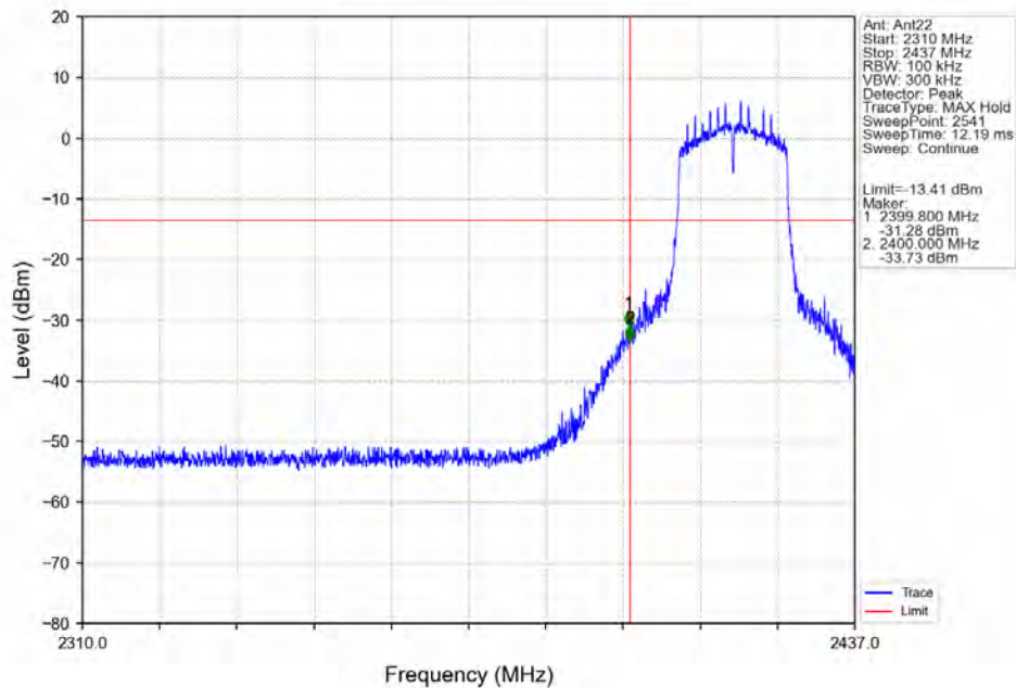
802.11ac(VHT20)_LCH_2417MHz_Ant22_NTNV
