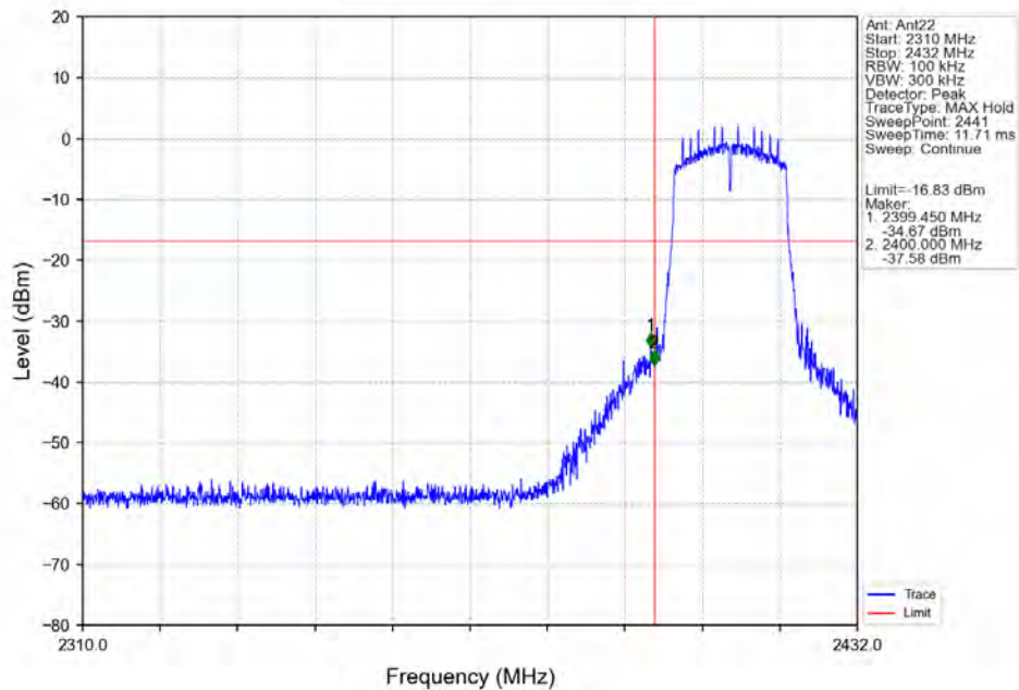
802.11n(HT20)_LCH_2412MHz_Ant22_NTNV
