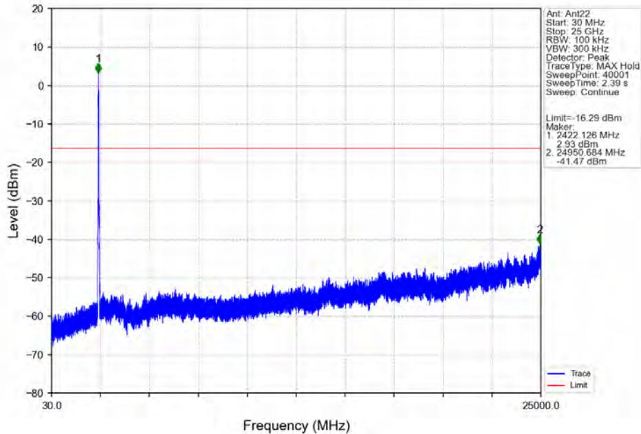
802.11ac(VHT40)_MCH_2437MHz_Ant22_NTNV
