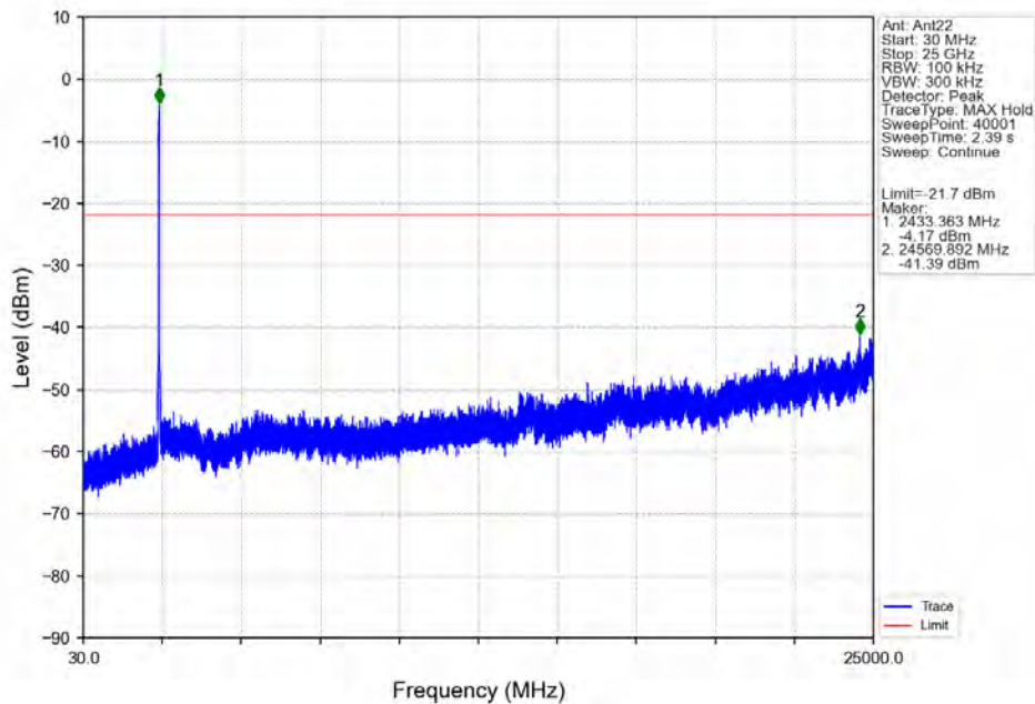
802.11n(HT40)_LCH_2427MHz_Ant22_NTNV
