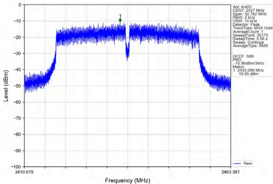
802.11ac(VHT40)_MCH_2437MHz_Ant22_NTNV
