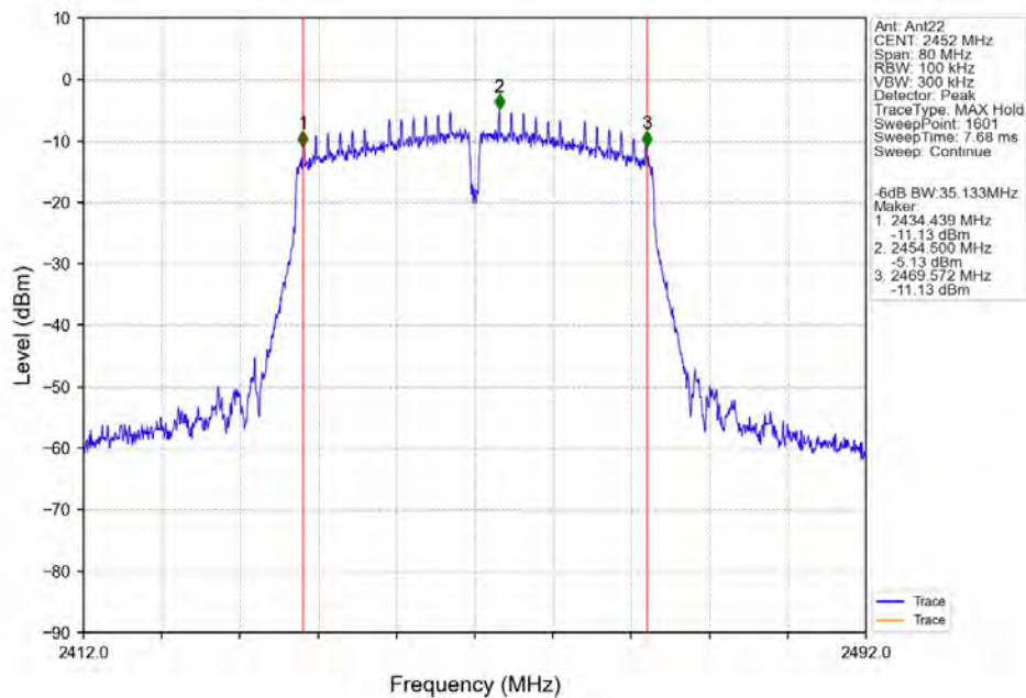
802.11ac(VHT40)_HCH_2452MHz_Ant22_NTNV
