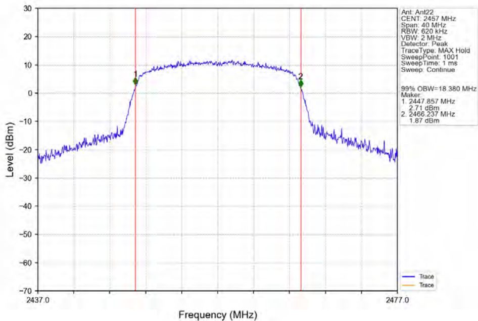
802.11ac(VHT20)_HCH_2457MHz_Ant22_NTNV
