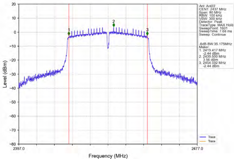
802.11ac(VHT40)_MCH_2437MHz_Ant22_NTNV
