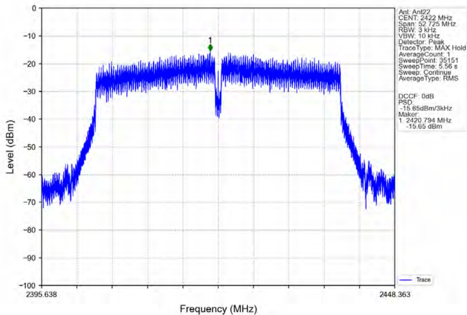
802.11n(HT40)_LCH_2422MHz_Ant22_NTNV
