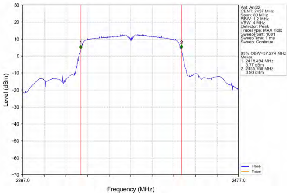
802.11n(HT40)_MCH_2437MHz_Ant22_NTNV
