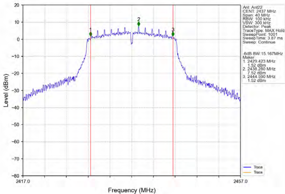
802.11g_MCH_2437MHz_Ant22_NTNV
