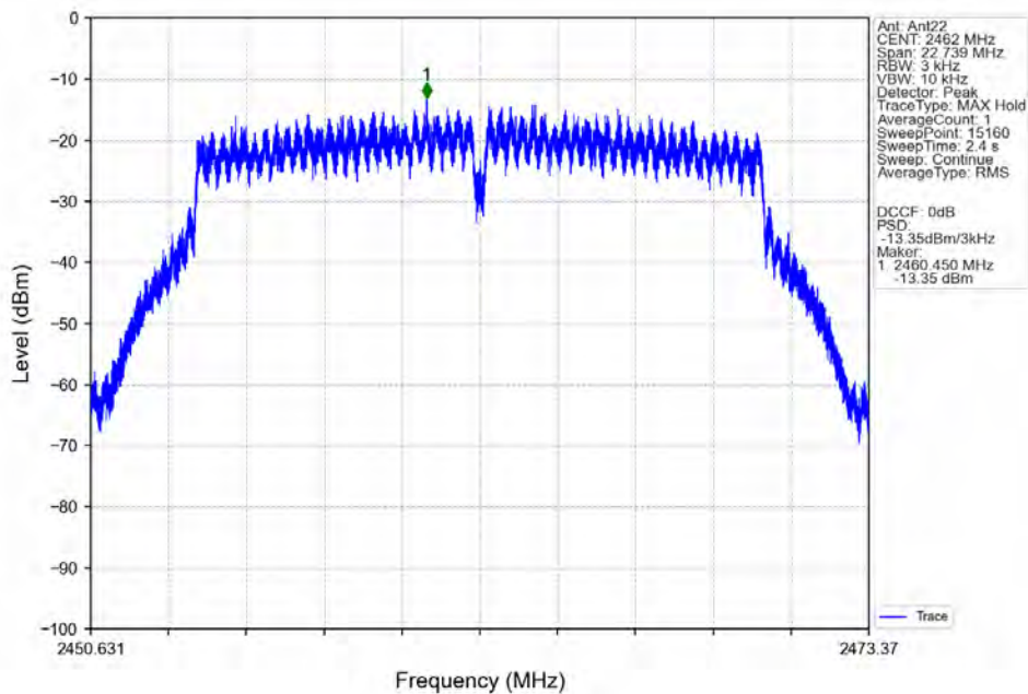
802.11g_HCH_2462MHz_Ant22_NTNV
