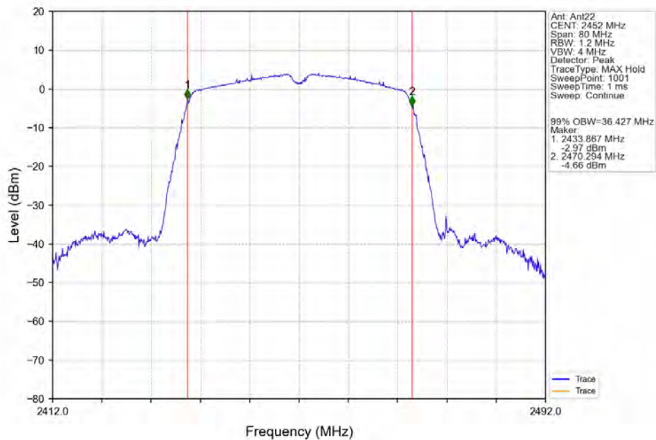
802.11n(HT40)_HCH_2452MHz_Ant22_NTNV
