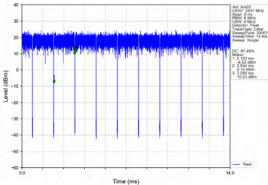
802.11g_MCH_2437MHz_Ant22_NTNV
