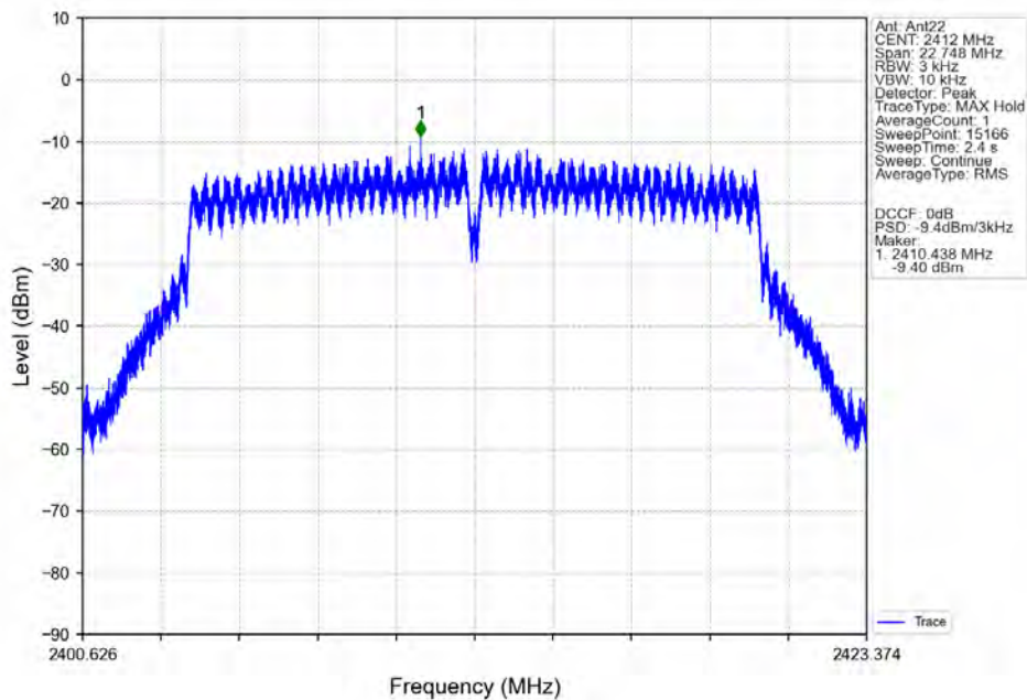
802.11g_LCH_2412MHz_Ant22_NTNV
