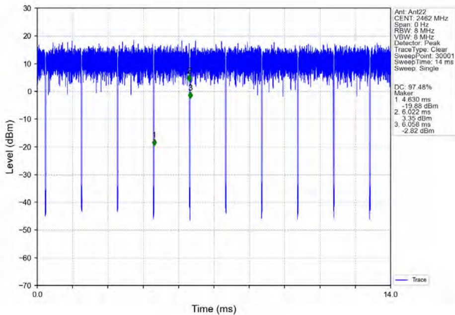
802.11g_HCH_2462MHz_Ant22_NTNV
