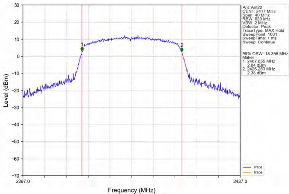
802.11ac(VHT20)_LCH_2417MHz_Ant22_NTNV
