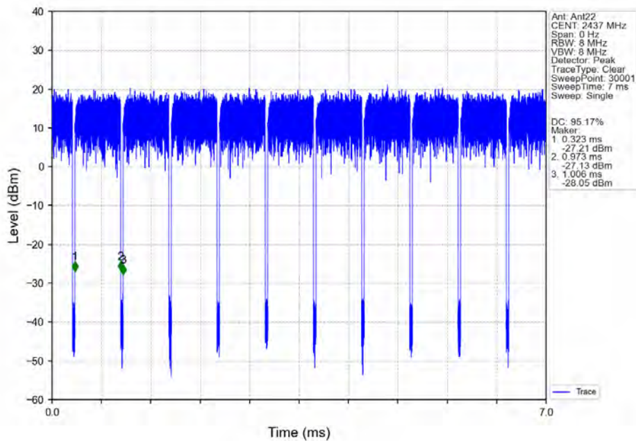
802.11n(HT40)_MCH_2437MHz_Ant22_NTNV
