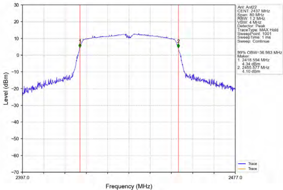
802.11ac(VHT40)_MCH_2437MHz_Ant22_NTNV
