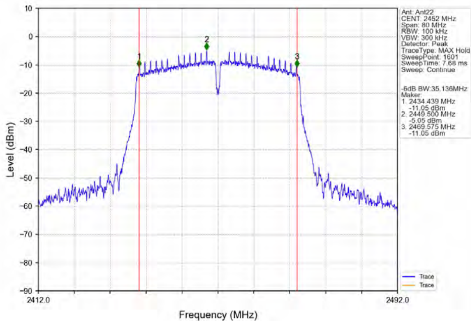
802.11n(HT40)_HCH_2452MHz_Ant22_NTNV
