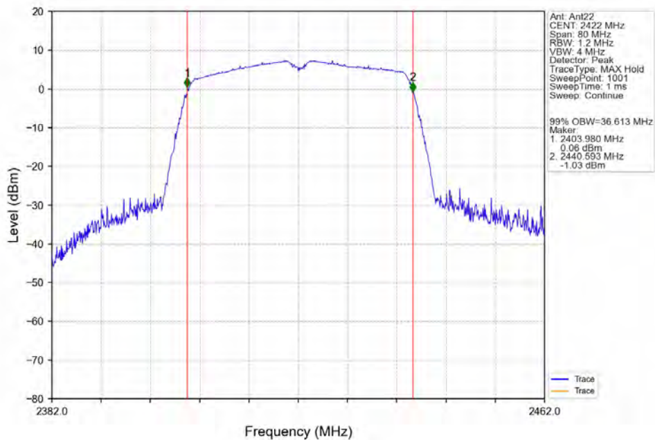
802.11ac(VHT40)_LCH_2422MHz_Ant22_NTNV
