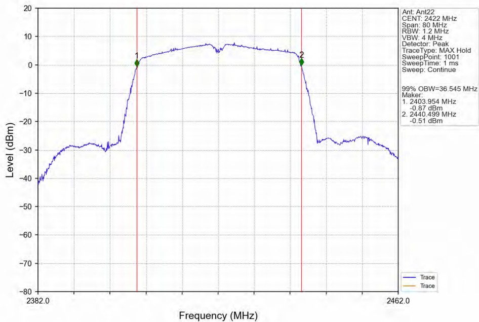
802.11n(HT40)_LCH_2422MHz_Ant22_NTNV
