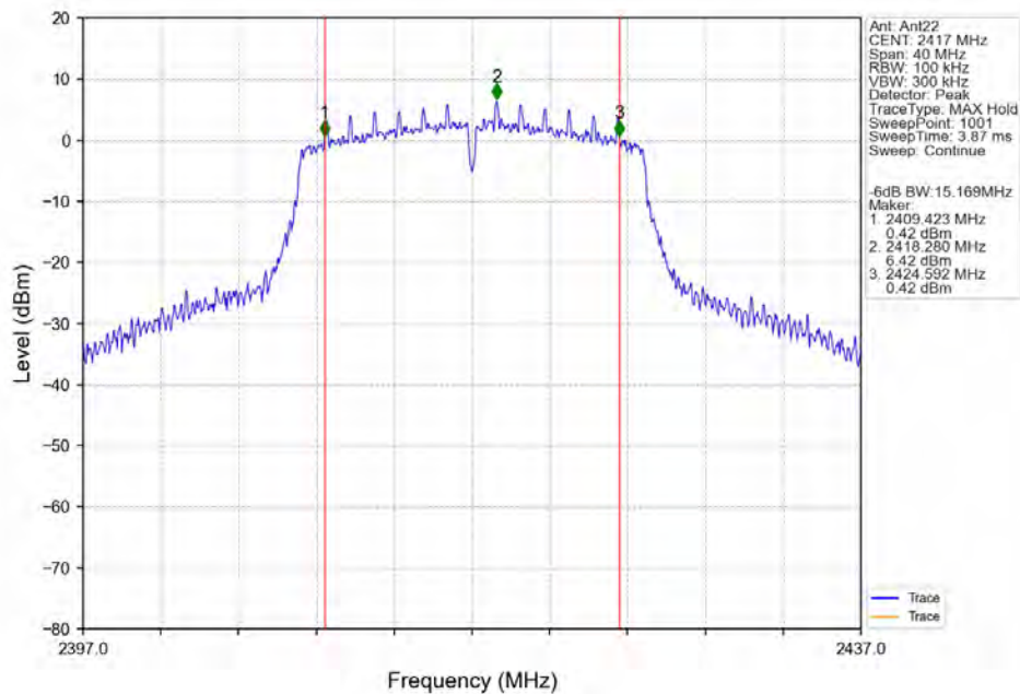
802.11ac(VHT20)_LCH_2417MHz_Ant22_NTNV
