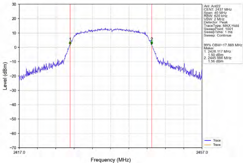
802.11g_MCH_2437MHz_Ant22_NTNV
