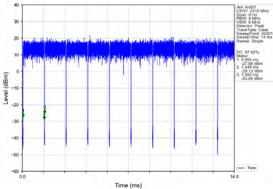
802.11g_LCH_2412MHz_Ant22_NTNV
