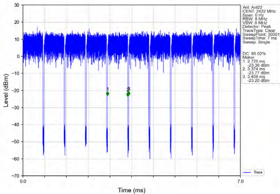
802.11n(HT40)_LCH_2422MHz_Ant22_NTNV
