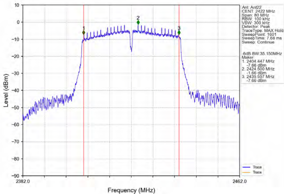
802.11n(HT40)_LCH_2422MHz_Ant22_NTNV
