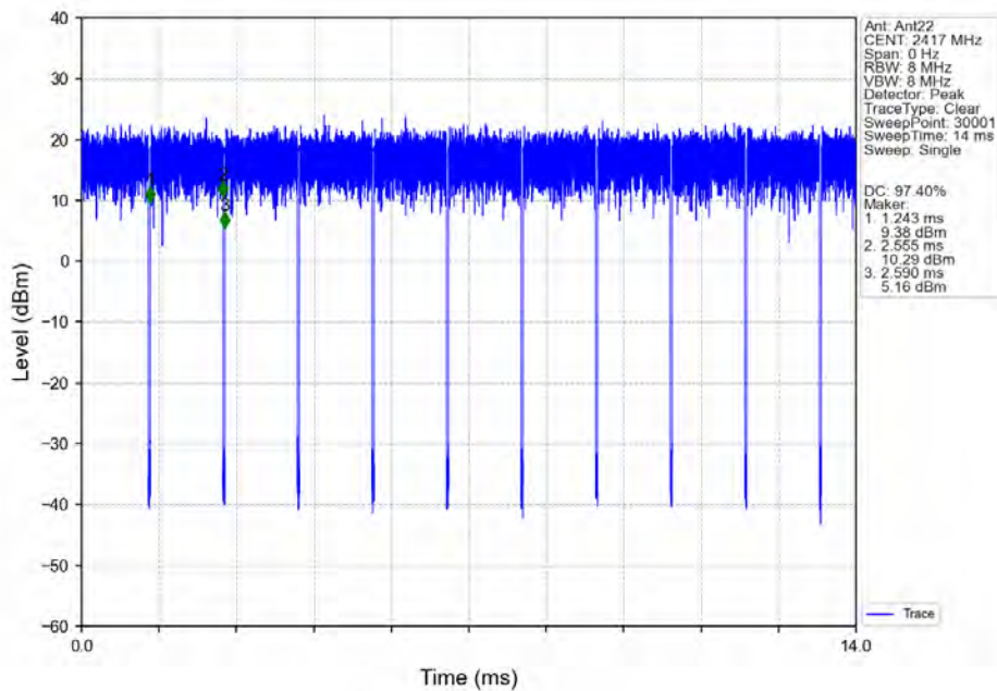
802.11ac(VHT20)_LCH_2417MHz_Ant22_NTNV
