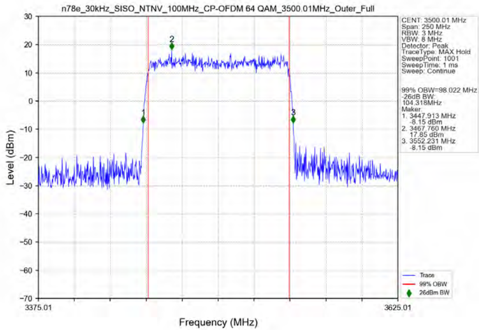
n78e 30kHz SISO NTN 100MHz CP-OFDM 64 QAM 3500.01MHz Outer Full Ant11
