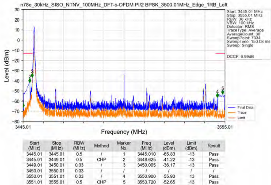
n78e_30kHz_SISO_NTNV_100MHz_DFT-s-OFDM PI/2 BPSK_3500.01MHz_Edge_1RB_Left_Ant11
