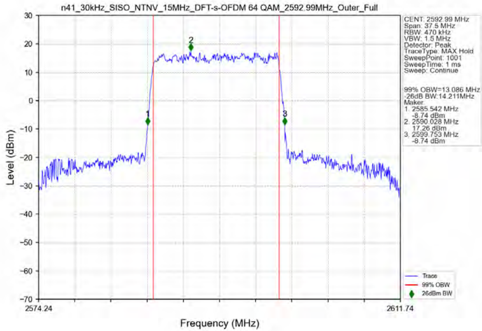
n41_30kHz_SISO_NTNV_15MHz_DFT-s-OFDM_64_QAM_2592.99MHz_Outer_Full_Ant31
