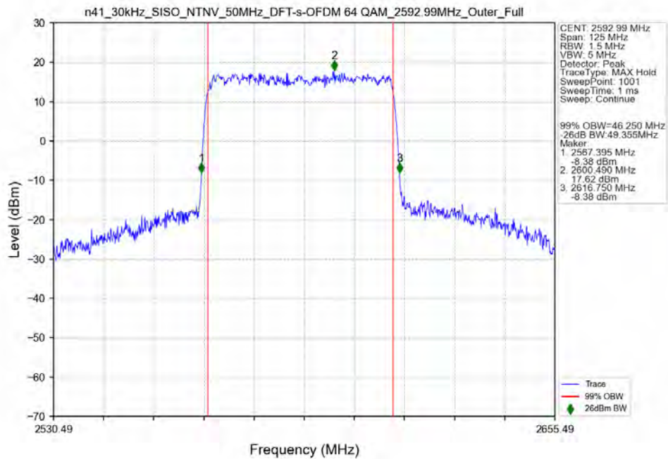
n41_30kHz_SISO_NTNV_50MHz_DFT-s-OFDM_64_QAM_2592.99MHz_Outer_Full_Ant31
