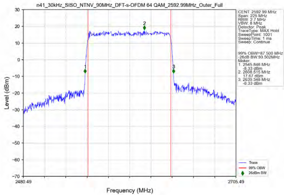
n41_30kHz_SISO_NTNV_90MHz_DFT-s-OFDM_64_QAM_2592.99MHz_Outer_Full_Ant31
