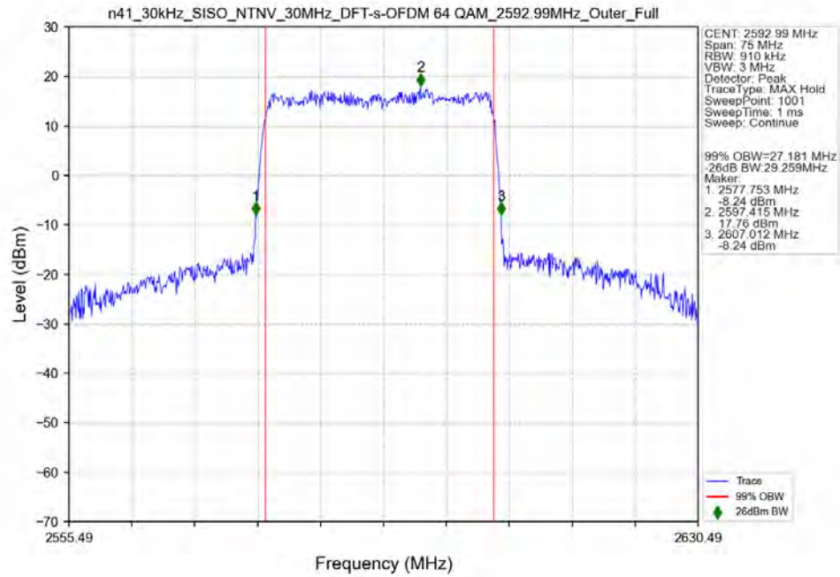
n41_30kHz_SISO_NTNV_30MHz_DFT-s-OFDM_64_QAM_2592.99MHz_Outer_Full_Ant31
