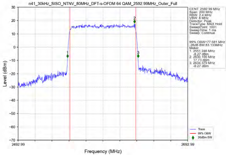
n41_30kHz_SISO_NTNV_80MHz_DFT-s-OFDM_64_QAM_2592.99MHz_Outer_Full_Ant31
