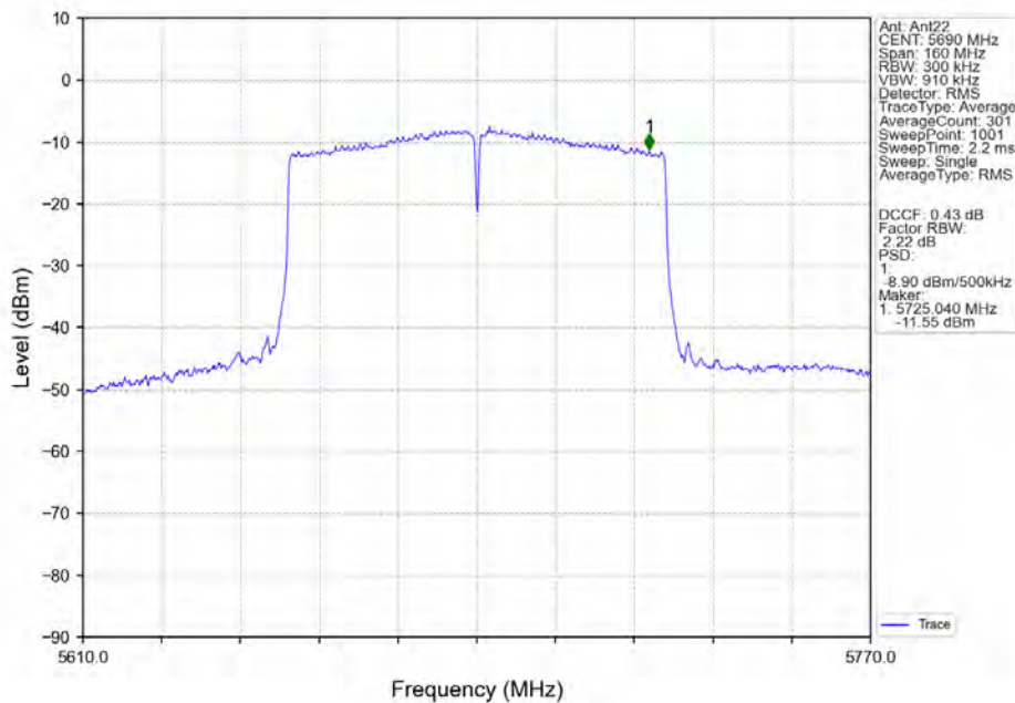
802.11ac(VHT80)_HCH_5690MHz_Ant22_NTNV
