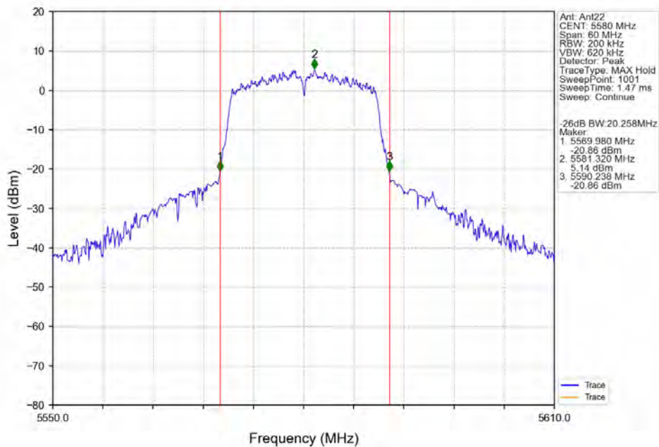
802.11n(HT20)_MCH_5580MHz_Ant22_NTNV
