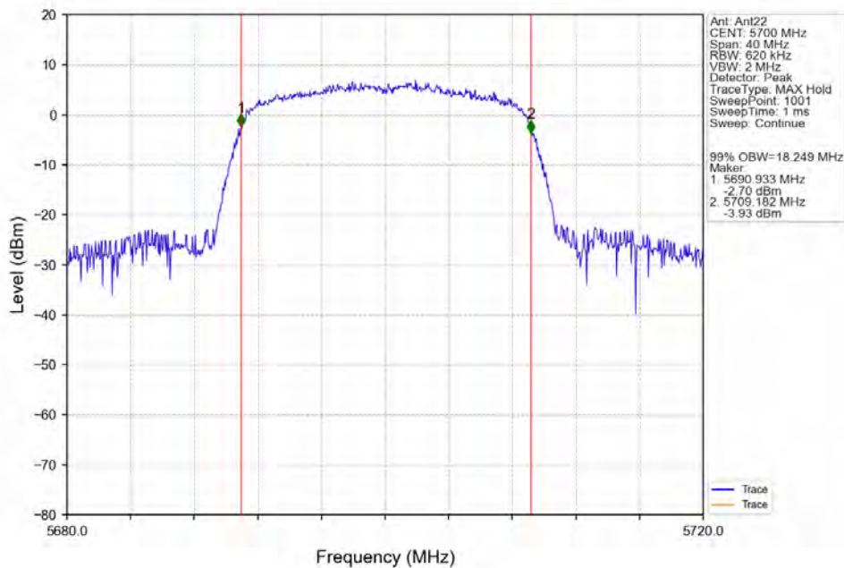
802.11n(HT20)_HCH_5700MHz_Ant22_NTNV
