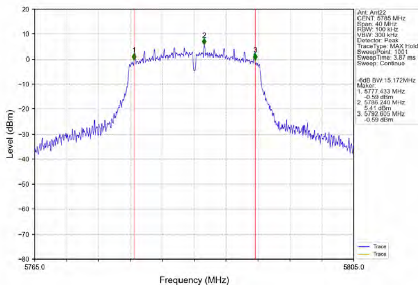
802.11a_MCH_5785MHz_Ant22_NTNV
