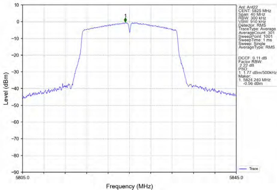
802.11ac(VHT20)_HCH_5825MHz_Ant22_NTNV
