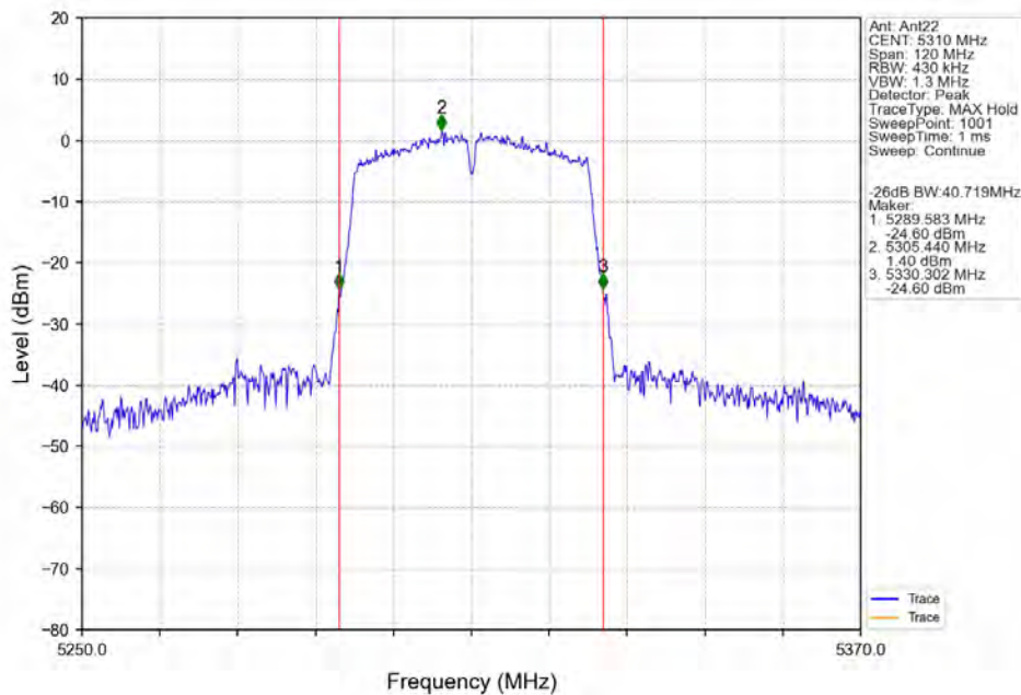
802.11n(HT40)_HCH_5310MHz_Ant22_NTNV
