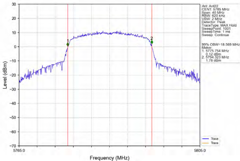
802.11n(HT20)_MCH_5785MHz_Ant22_NTNV
