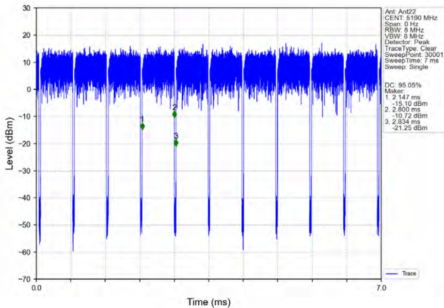
802.11ac(VHT40)_LCH_5190MHz_Ant22_NTNV
