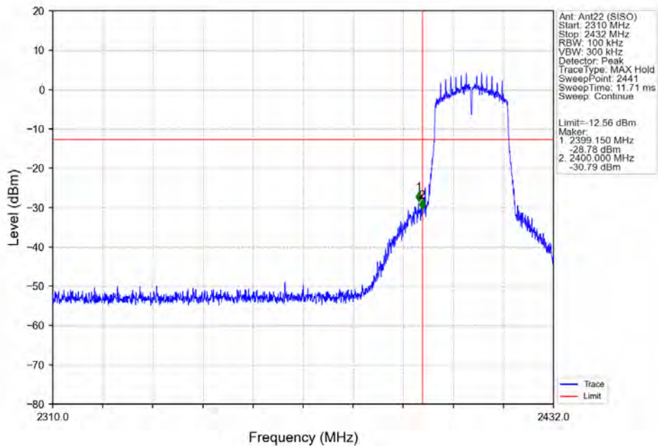
802.11n(HT20)_LCH_2412MHz_Ant22 (SISO)_NTNV
