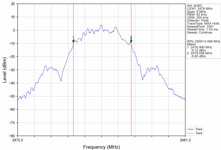
2M_HCH_2478MHz_Ant22_NTNV
