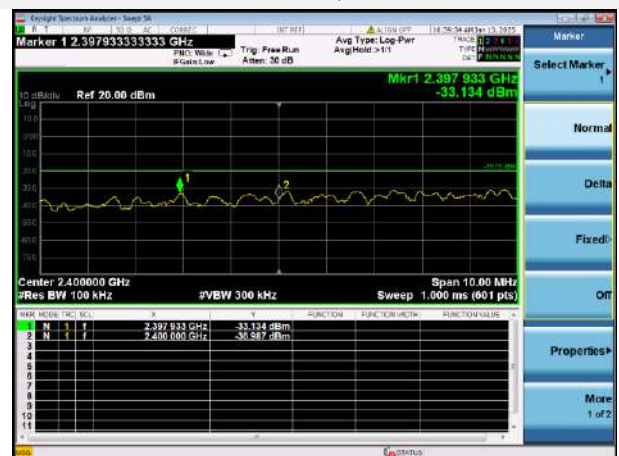
802.11n-40 MHz CHANNEL 5, BAND EDGE
