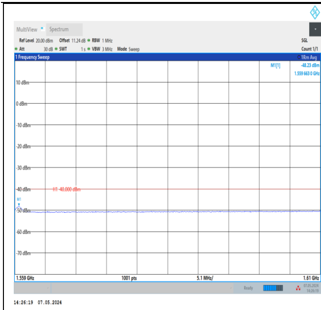
Band13_5MHz_QPSK_23230_1RB#0_1559~1610_1559~1610 610
