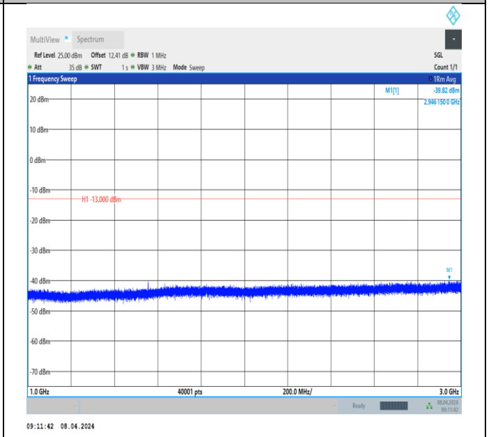
Band13_10MHz_QPSK_23230_1RB#0_1000~3000_1000~3000
