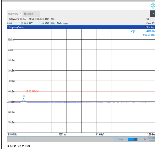
Band13_5MHz_QPSK_23255_1RB#0_1559~1610_1559~1 610
