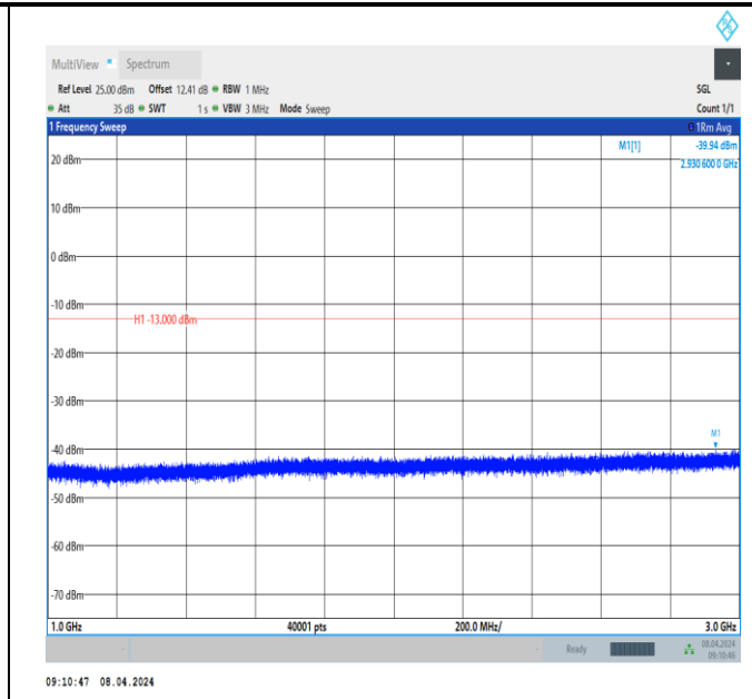
Band13_5MHz_QPSK_23255_1RB#0_1000~3000_1000~3000 0
