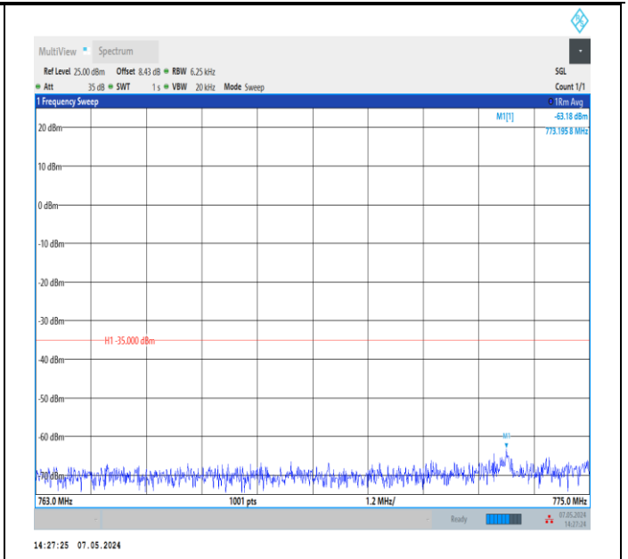
Band13_10MHz_QPSK_23230_1RB#0_763~775_763~775
