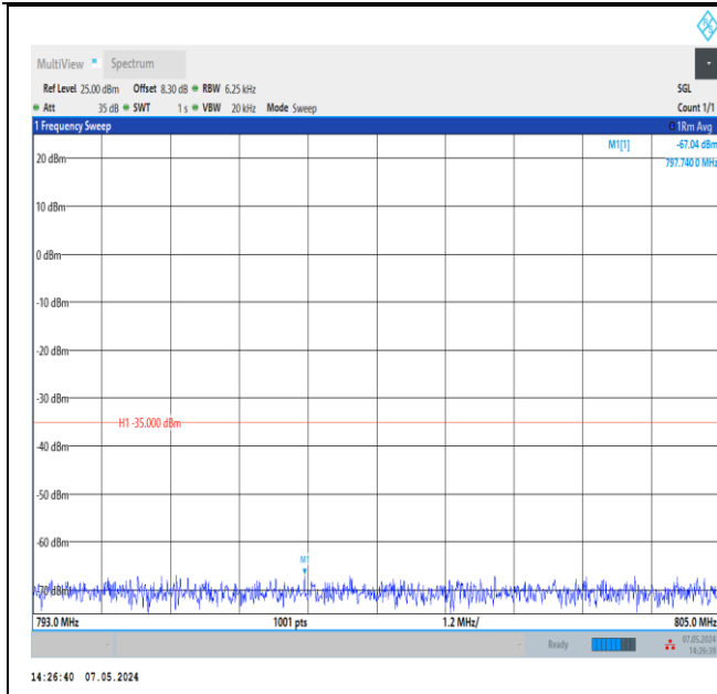
Band13_5MHz_QPSK_23255_1RB#0_793~805_793~805
