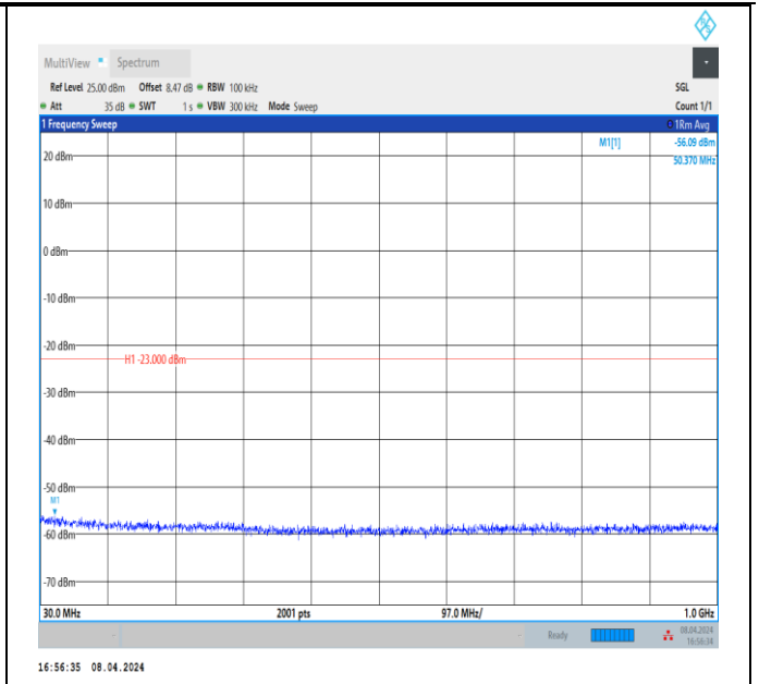
Band66_10MHz_QPSK_132622_1RB#0_30~1000_30~1000
