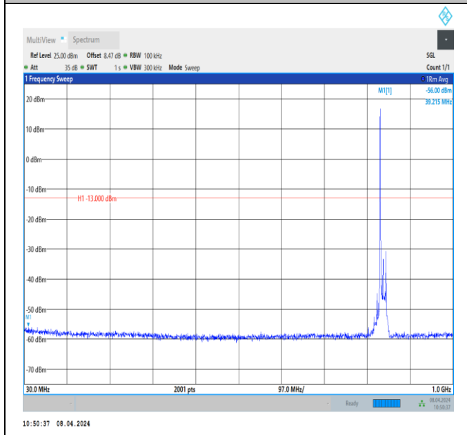
Band26_15MHz_QPSK_26965_1RB#0_30~1000_30~1000
