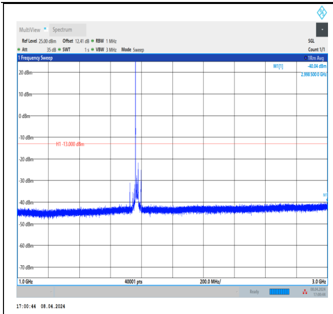
Band66_20MHz_QPSK_132572_1RB#0_1000~3000_1000~3000
