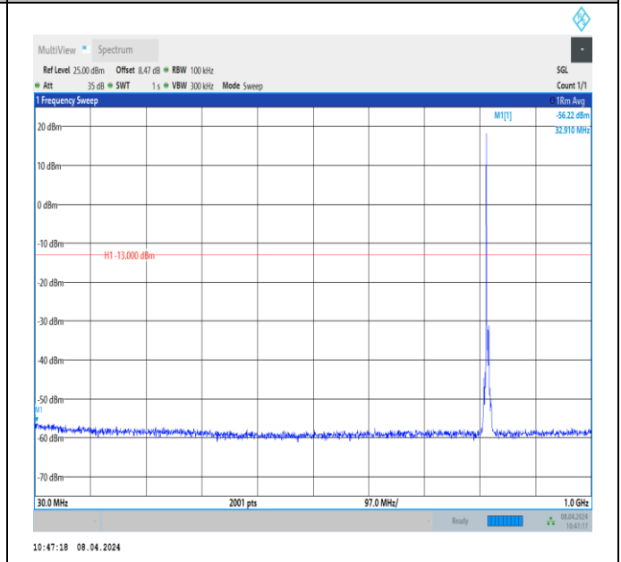
Band26_5MHz_QPSK_26740_1RB#0_30~1000_30~1000
