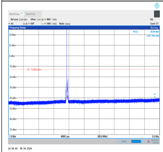
Band66_10MHz_QPSK_132622_1RB#0_1000~3000_1000~3000
