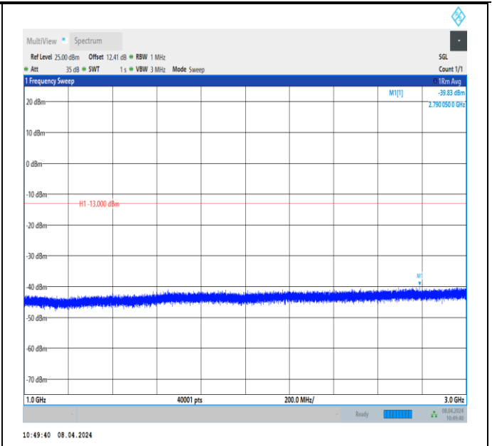
Band26_15MHz_QPSK_26865_1RB#0_1000~3000_1000~3000
