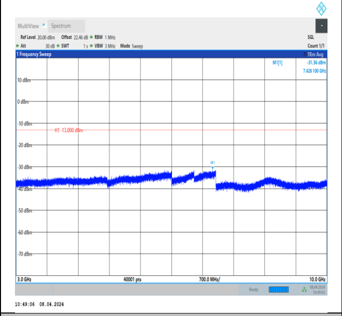
Band26_10MHz_QPSK_26740_1RB#0_3000~10000_3000~10000
