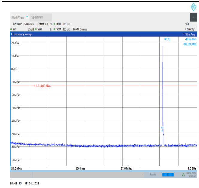
Band26_1.4MHz_QPSK_26783_1RB#0_30~1000_30~1000
