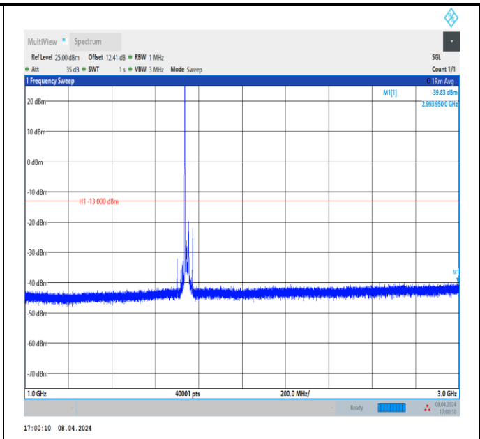
Band66_20MHz_QPSK_132322_1RB#0_1000~3000_1000~3000
