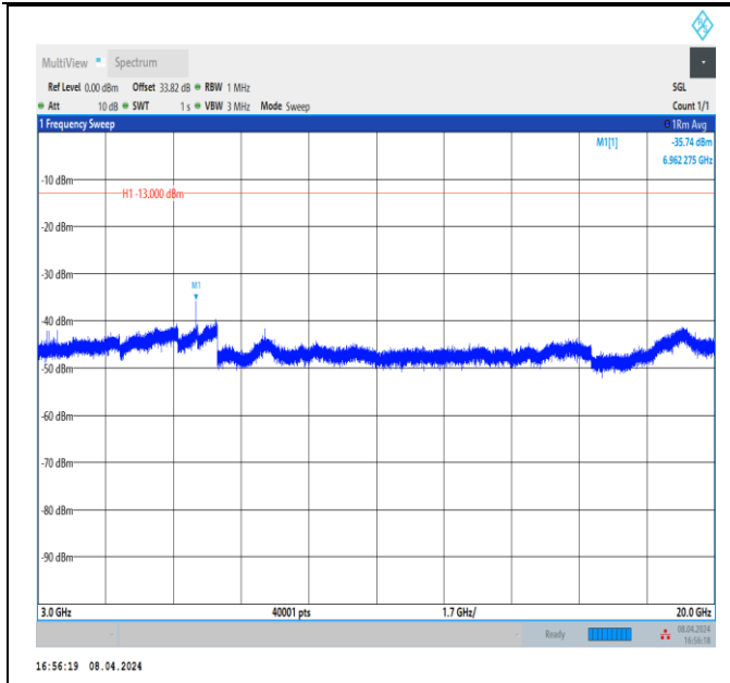
Band66_10MHz_QPSK_132322_1RB#0_3000~20000_3000~20000
