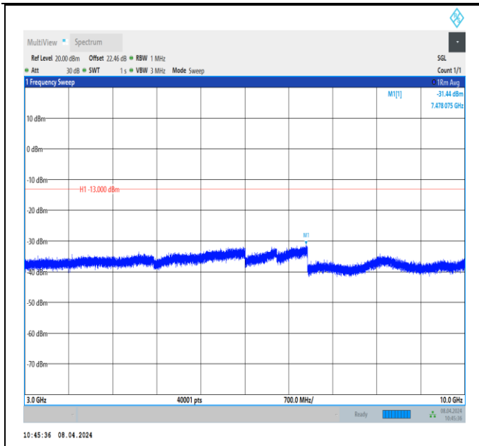
Band26_3MHz_QPSK_26740_1RB#0_3000~10000_3000~10000
