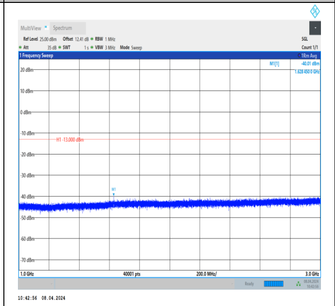
Band26_1.4MHz_QPSK_26697_1RB#0_1000~3000_1000~3000
