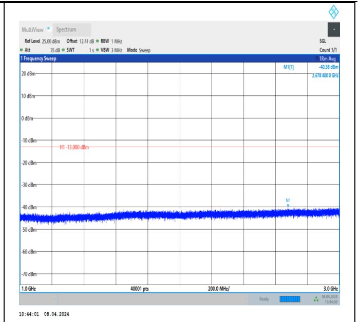
Band26_1.4MHz_QPSK_26783_1RB#0_1000~3000_1000~3000
