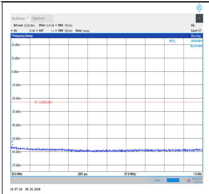
Band66_15MHz_QPSK_132047_1RB#0_30~1000_30~1000
