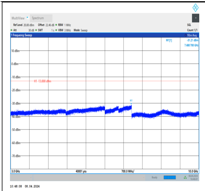
Band26_5MHz_QPSK_26765_1RB#0_3000~10000_3000~10000
