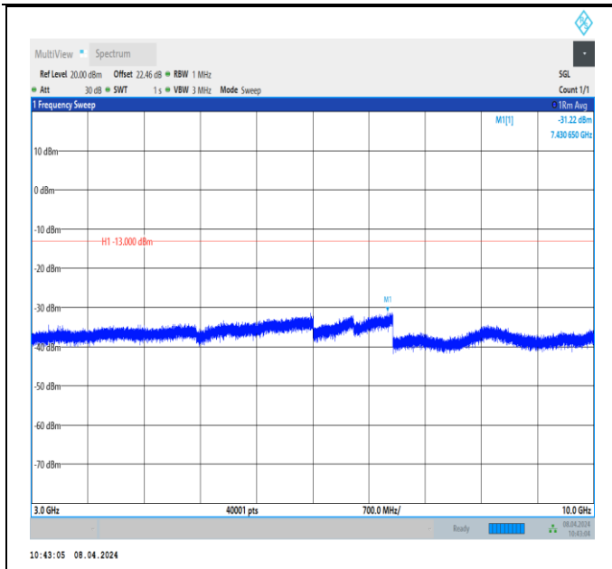
Band26_1.4MHz_QPSK_26697_1RB#0_3000~10000_3000 ~10000
