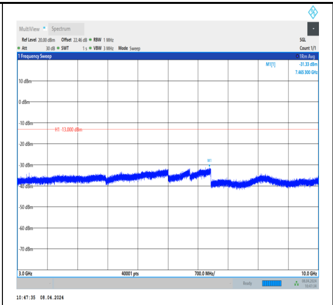
Band26_5MHz_QPSK_26740_1RB#0_3000~10000_3000~10000 0000
