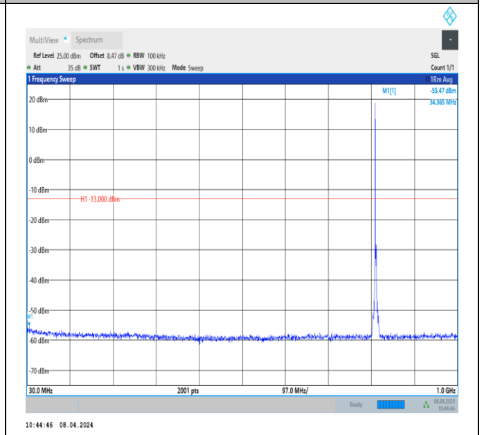
Band26_3MHz_QPSK_26705_1RB#0_30~1000_30~1000
