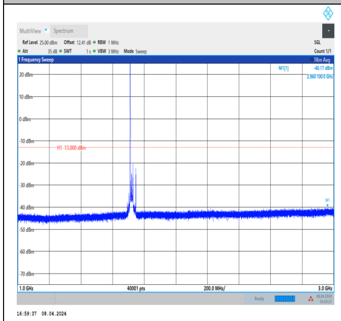
Band66_20MHz_QPSK_132072_1RB#0_1000~3000_1000~3000
