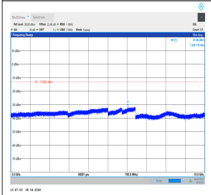
Band26_5MHz_QPSK_26715_1RB#0_3000~10000_3000~10000 0000
