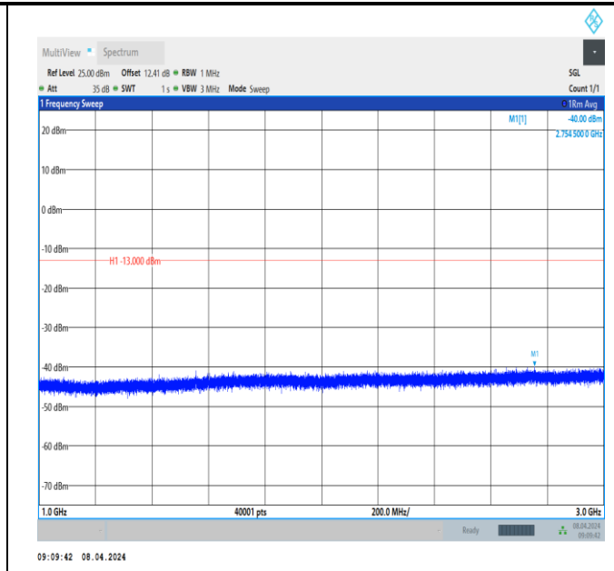
Band13_5MHz_QPSK_23205_1RB#0_1000~3000_1000~3000 0
