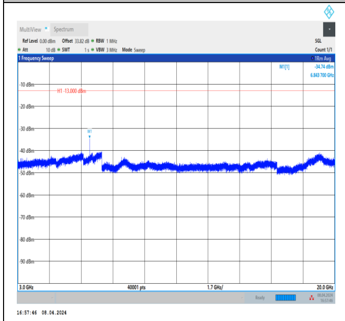
Band66_15MHz_QPSK_132047_1RB#0_3000~20000_3000~20000
