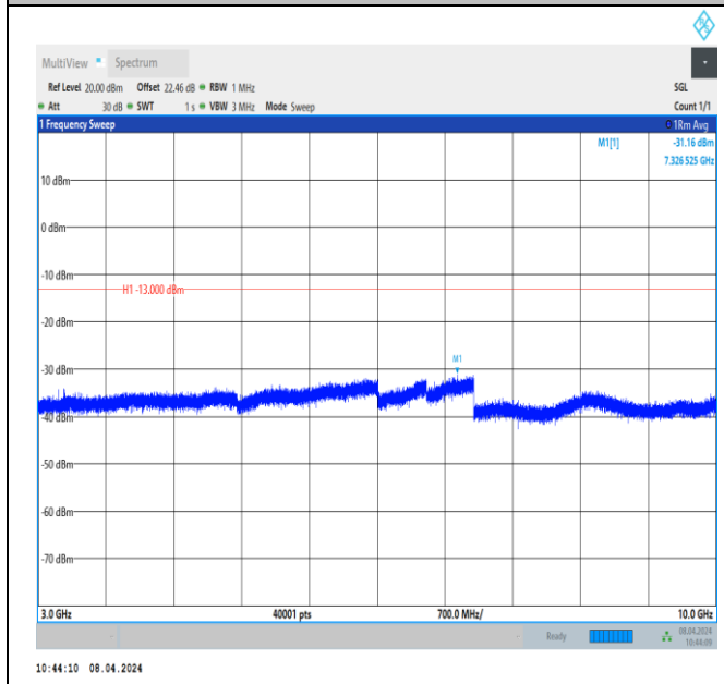
Band26_1.4MHz_QPSK_26783_1RB#0_3000~10000_3000~10000
