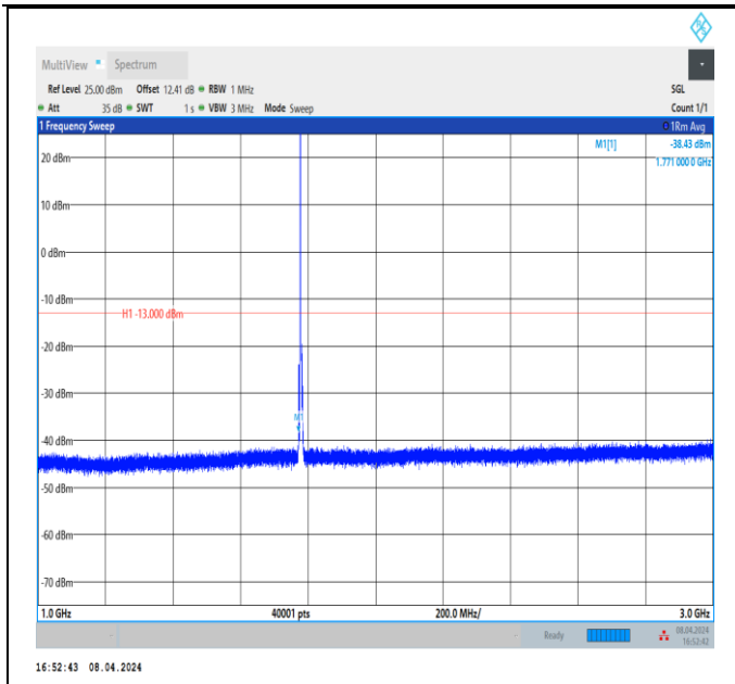
Band66_3MHz_QPSK_132657_1RB#0_1000~3000_1000~3000
