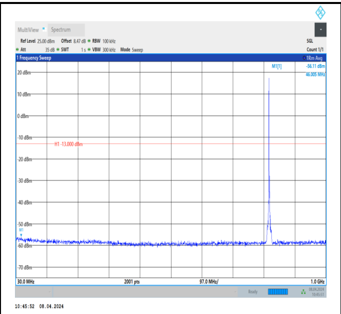
Band26_3MHz_QPSK_26775_1RB#0_30~1000_30~1000
