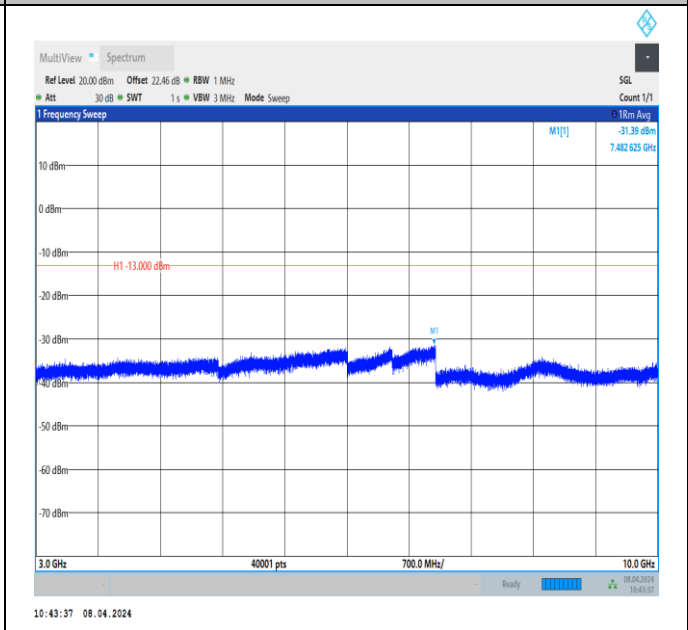
Band26_1.4MHz_QPSK_26740_1RB#0_3000~10000_3000 ~10000
