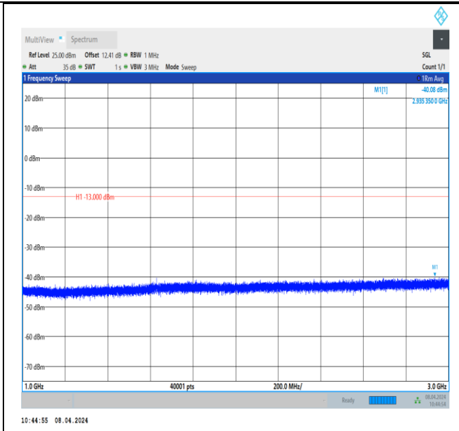
Band26_3MHz_QPSK_26705_1RB#0_1000~3000_1000~3000 00
