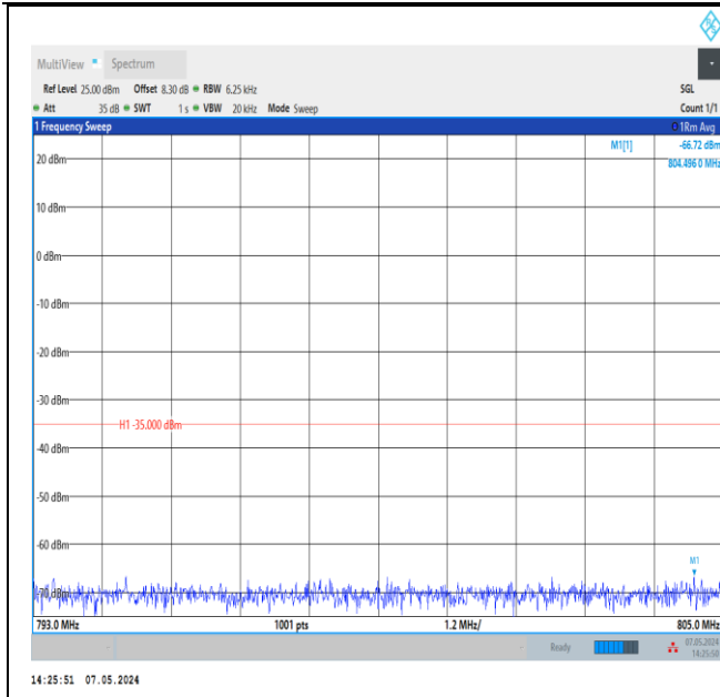
Band13_5MHz_QPSK_23205_1RB#0_793~805_793~805
