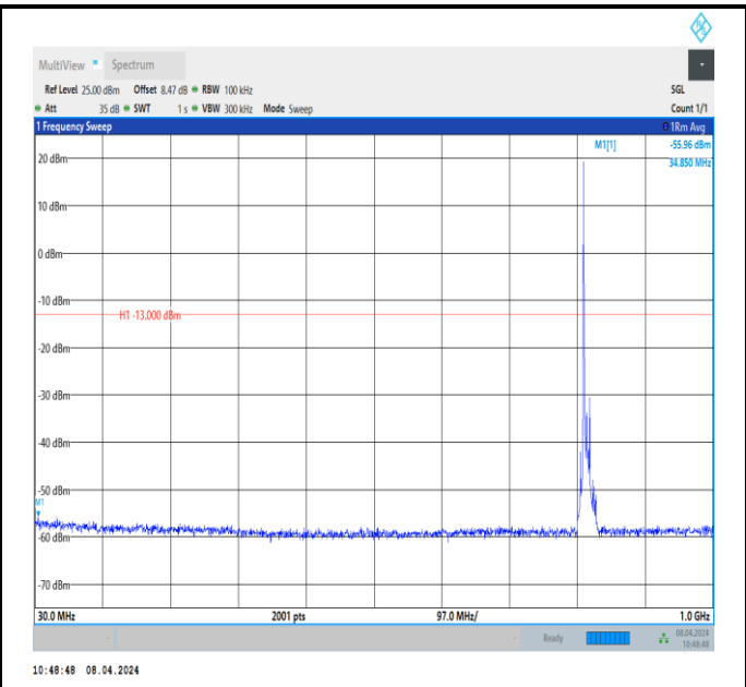
Band26_10MHz_QPSK_26740_1RB#0_30~1000_30~1000
