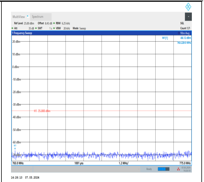
Band13_5MHz_QPSK_23230_1RB#0_763~775_763~775
