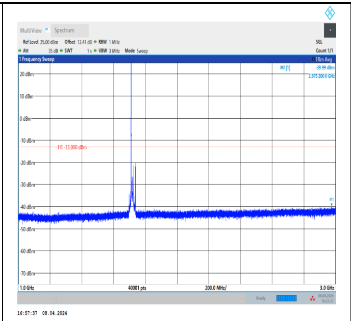
Band66_15MHz_QPSK_132047_1RB#0_1000~3000_1000~3000
