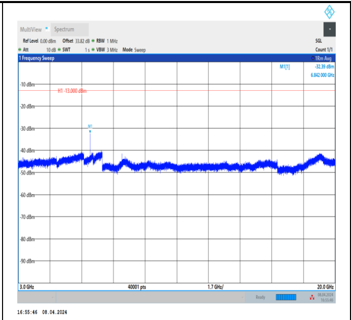
Band66_10MHz_QPSK_132022_1RB#0_3000~20000_3000~20000
