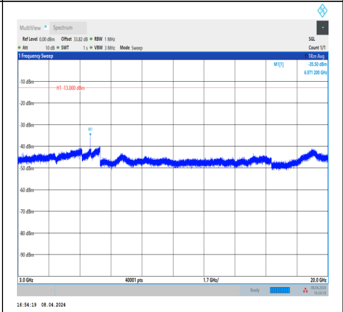
Band66_5MHz_QPSK_132322_1RB#0_3000~20000_3000~20000
