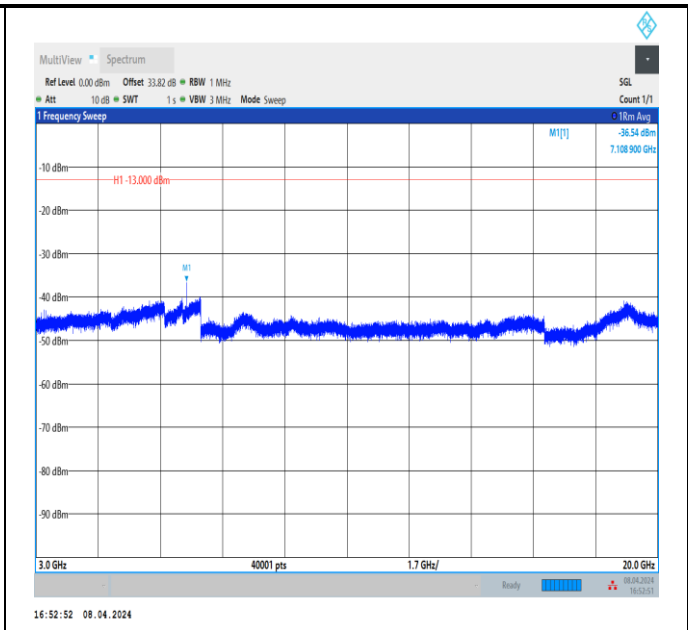
Band66_3MHz_QPSK_132657_1RB#0_3000~20000_3000~20000
