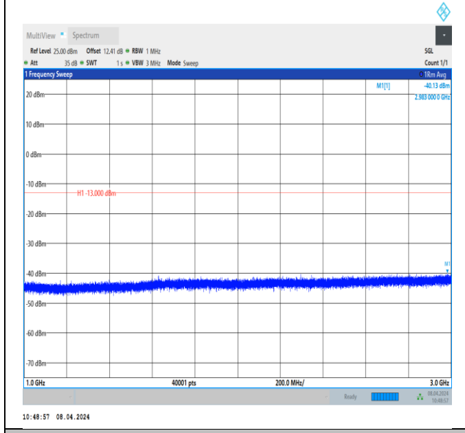
Band26_10MHz_QPSK_26740_1RB#0_1000~3000_1000~3000
