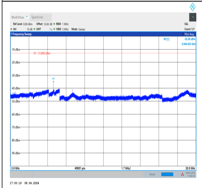
Band66_20MHz_QPSK_132322_1RB#0_3000~20000_3000~20000
