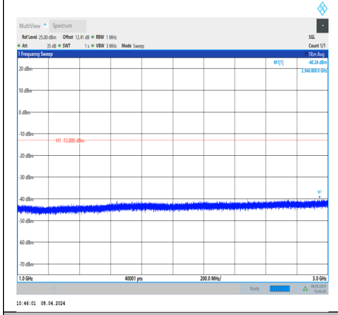
Band26_3MHz_QPSK_26775_1RB#0_1000~3000_1000~3000
