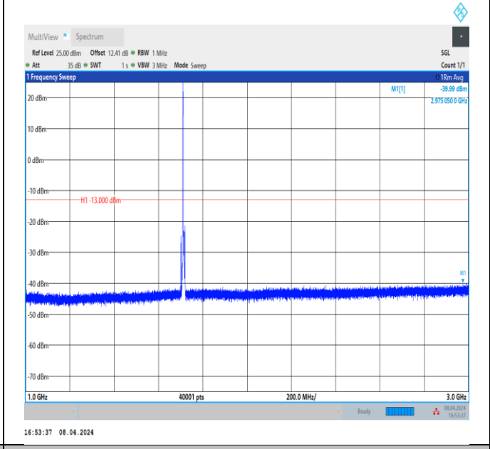
Band66_5MHz_QPSK_131997_1RB#0_1000~3000_1000~3000
