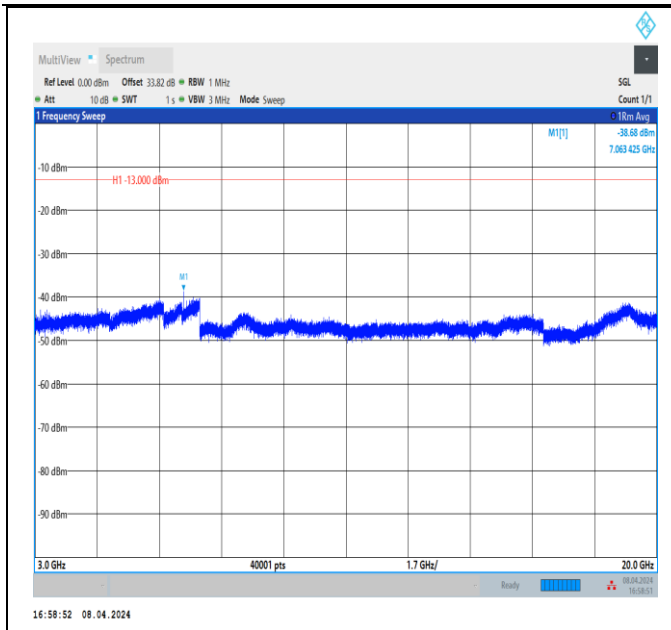
Band66_15MHz_QPSK_132597_1RB#0_3000~20000_3000~20000
