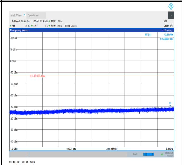
Band26_3MHz_QPSK_26740_1RB#0_1000~3000_1000~3000 00
