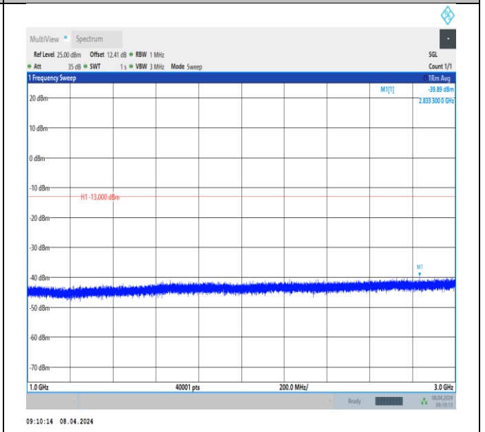
Band13_5MHz_QPSK_23230_1RB#0_1000~3000_1000~3000
