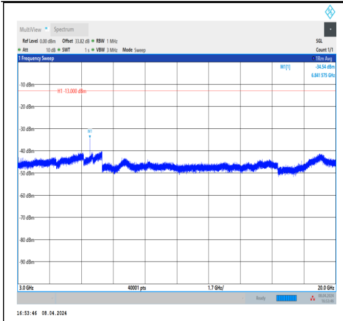
Band66_5MHz_QPSK_131997_1RB#0_3000~20000_3000~20000
