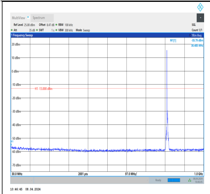
Band26_5MHz_QPSK_26715_1RB#0_30~1000_30~1000
