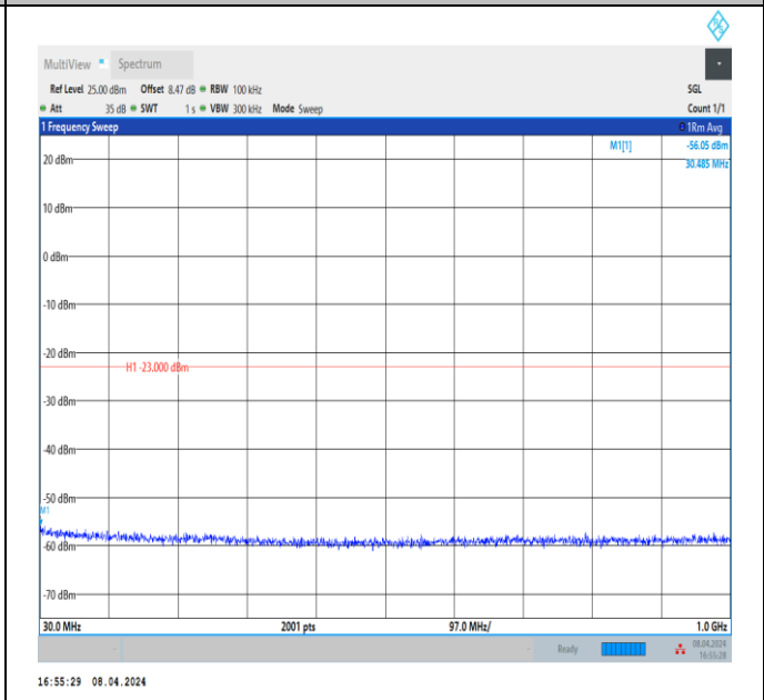
Band66_10MHz_QPSK_132022_1RB#0_30~1000_30~1000
