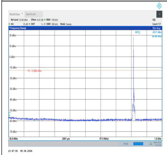
Band26_5MHz_QPSK_26765_1RB#0_30~1000_30~1000 00
