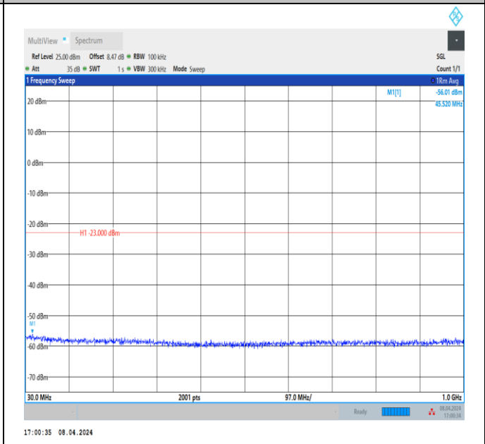
Band66_20MHz_QPSK_132572_1RB#0_30~1000_30~1000
