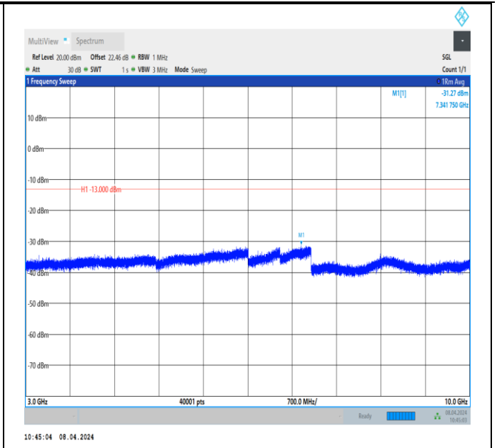
Band26_3MHz_QPSK_26705_1RB#0_3000~10000_3000~10000 0000
