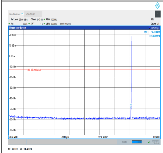
Band26_1.4MHz_QPSK_26697_1RB#0_30~1000_30~1000
