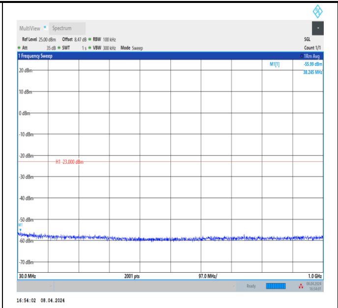
Band66_5MHz_QPSK_132322_1RB#0_30~1000_30~1000
