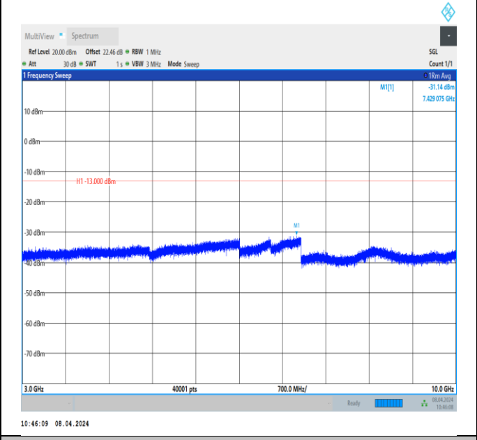
Band26_3MHz_QPSK_26775_1RB#0_3000~10000_3000~10000
