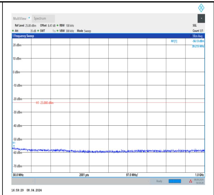
Band66_20MHz_QPSK_132072_1RB#0_30~1000_30~1000
