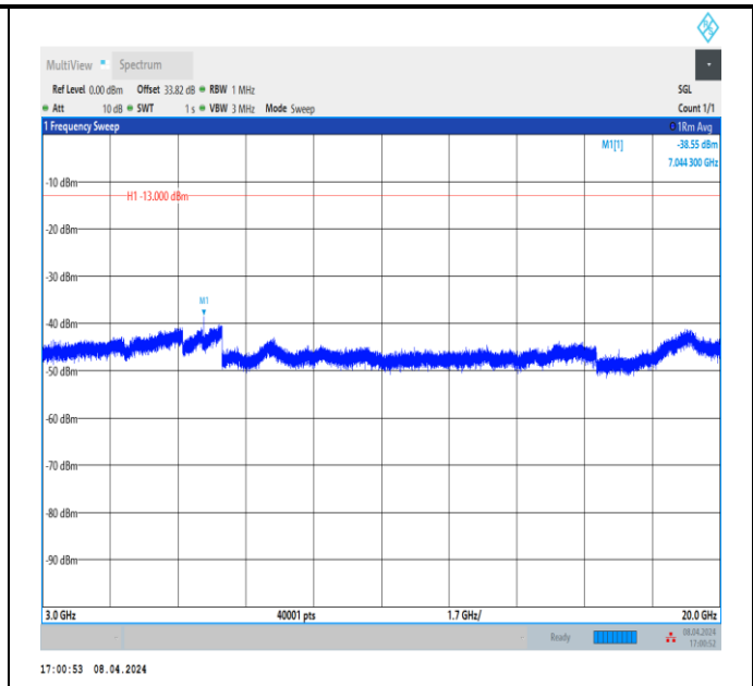
Band66_20MHz_QPSK_132572_1RB#0_3000~20000_3000~20000
