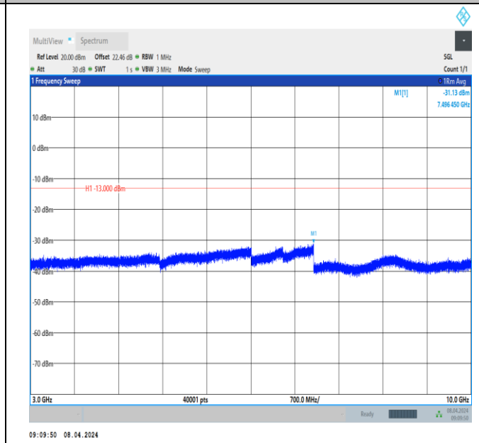
Band13_5MHz_QPSK_23205_1RB#0_3000~10000_3000~10 000
