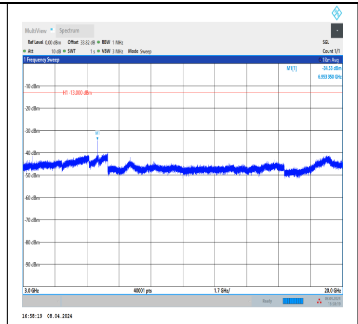
Band66_15MHz_QPSK_132322_1RB#0_3000~20000_3000~20000
