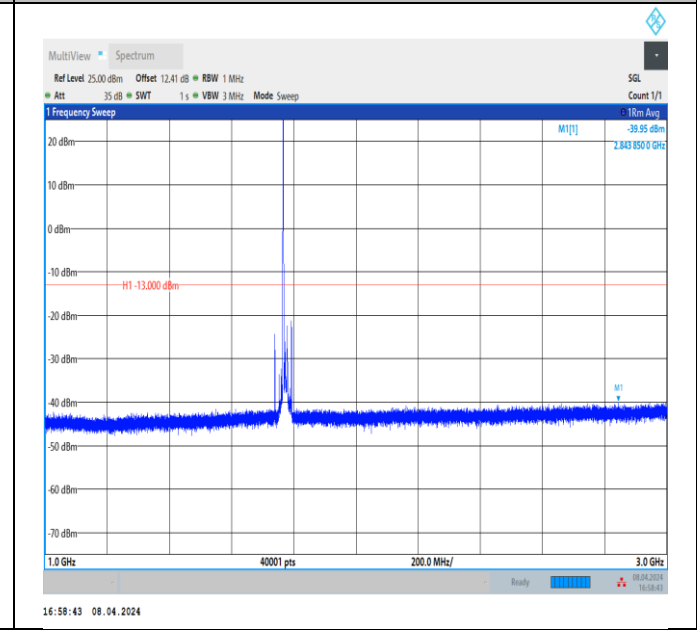
Band66_15MHz_QPSK_132597_1RB#0_1000~3000_1000~3000
