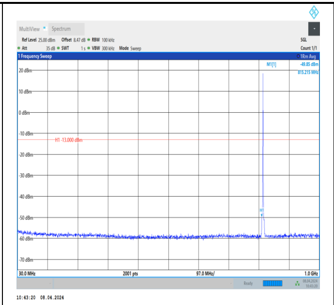
Band26_1.4MHz_QPSK_26740_1RB#0_30~1000_30~1000
