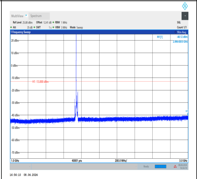
Band66_10MHz_QPSK_132322_1RB#0_1000~3000_1000~3000
