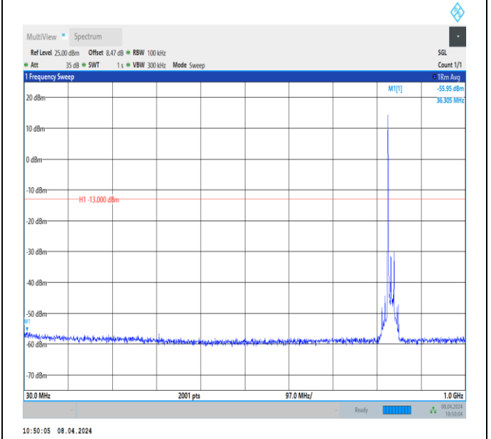
Band26_15MHz_QPSK_26915_1RB#0_30~1000_30~1000
