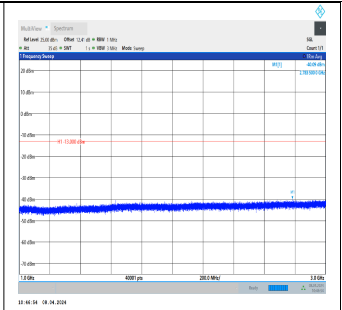
Band26_5MHz_QPSK_26715_1RB#0_1000~3000_1000~3000 00
