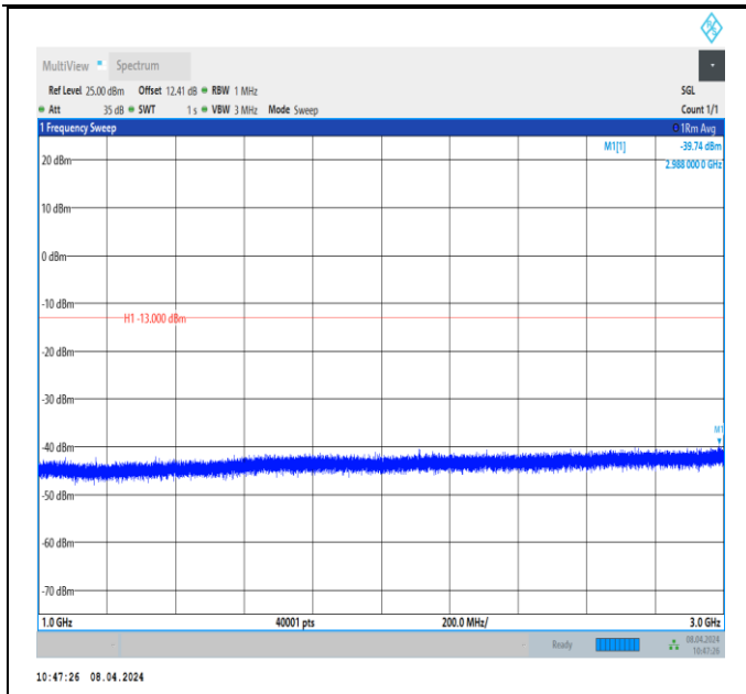
Band26_5MHz_QPSK_26740_1RB#0_1000~3000_1000~3000 00
