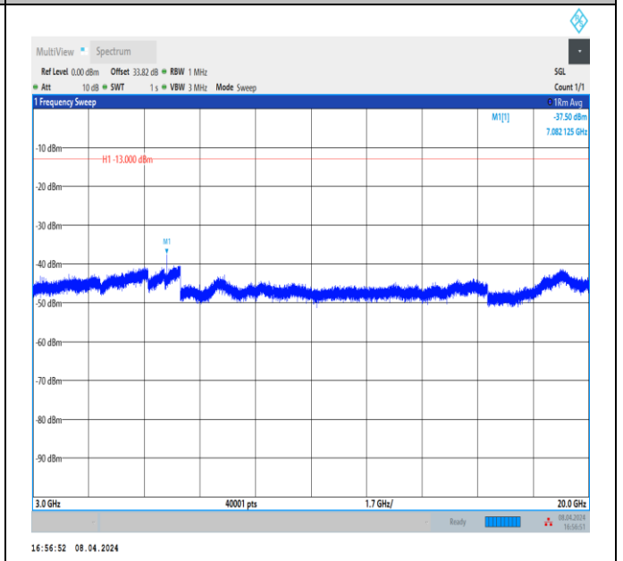
Band66_10MHz_QPSK_132622_1RB#0_3000~20000_3000~20000
