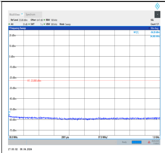
Band66_20MHz_QPSK_132322_1RB#0_30~1000_30~1000
