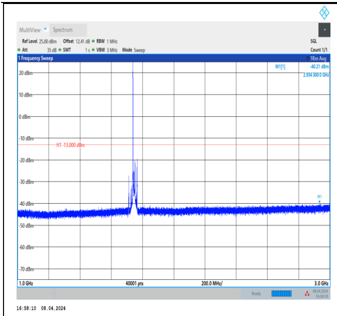
Band66_15MHz_QPSK_132322_1RB#0_1000~3000_1000~3000
