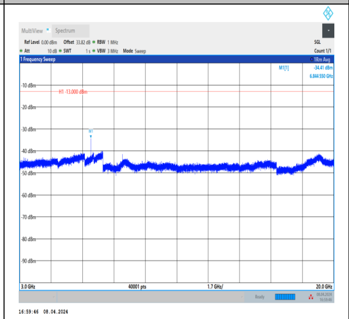
Band66_20MHz_QPSK_132072_1RB#0_3000~20000_3000~20000
