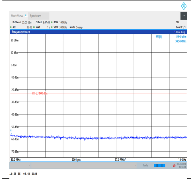
Band66_15MHz_QPSK_132597_1RB#0_30~1000_30~1000
