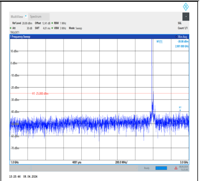
Band41_20MHz_QPSK_40620_1RB#0_1000~3000_1000~3000
