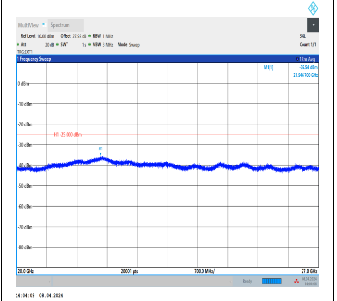
Band38_20MHz_QPSK_38150_1RB#0_20000~27000_20000~27000
