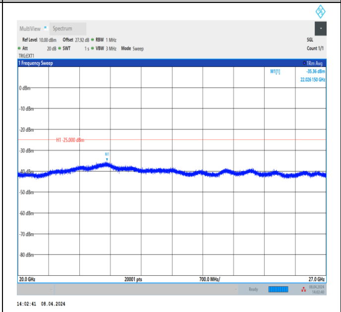
Band38_20MHz_QPSK_37850_1RB#0_20000~27000_20000~27000
