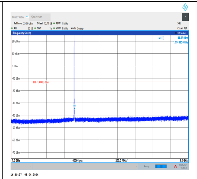
Band66_1.4MHz_QPSK_131979_1RB#0_1000~3000_1000 ~3000
