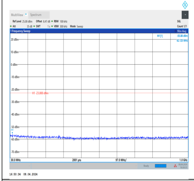
Band66_1.4MHz_QPSK_132665_1RB#0_30~1000_30~100 0
