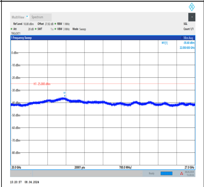
Band41_10MHz_QPSK_39700_1RB#0_20000~27000_20000~27000
