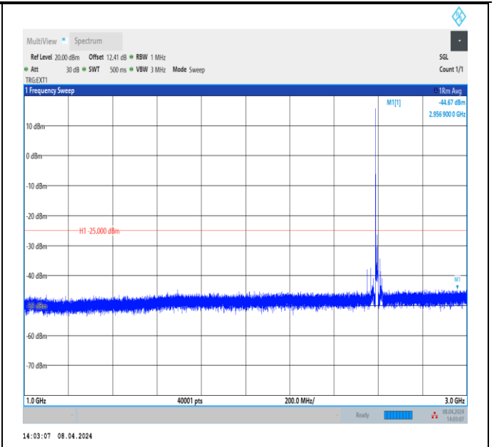
Band38_20MHz_QPSK_38000_1RB#0_1000~3000_1000~3000
