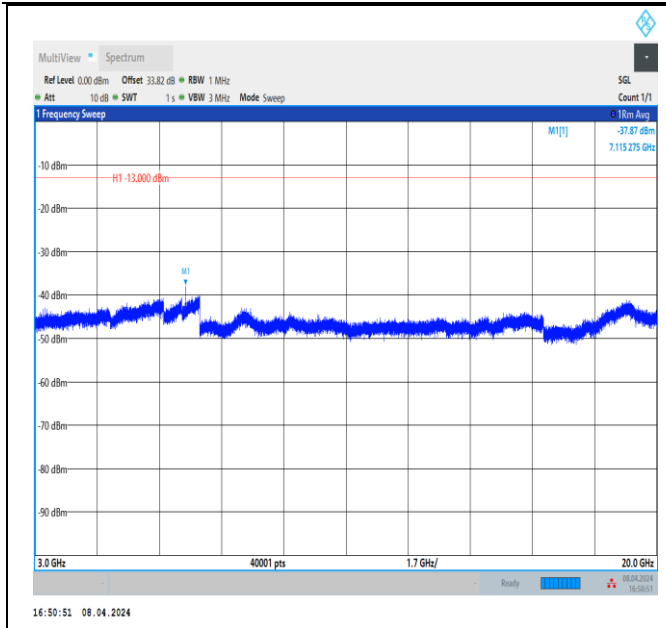
Band66_1.4MHz_QPSK_132665_1RB#0_3000~20000_3000~20000
