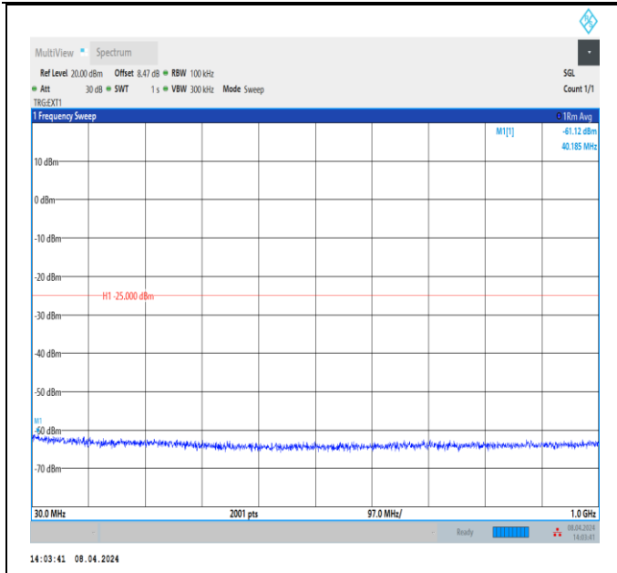
Band38_20MHz_QPSK_38150_1RB#0_30~1000_30~1000
