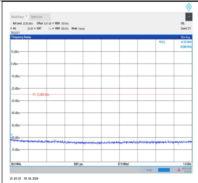
Band41_20MHz_QPSK_41490_1RB#0_30~1000_30~1000
