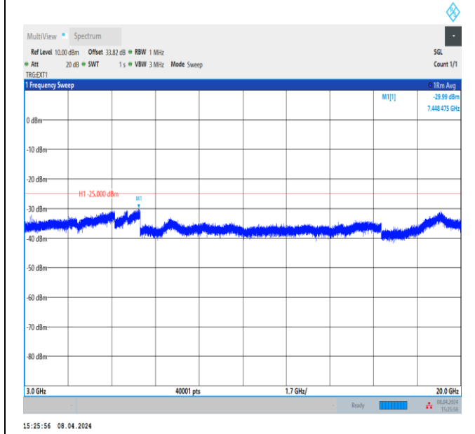
Band41_20MHz_QPSK_40620_1RB#0_3000~20000_3000~20000
