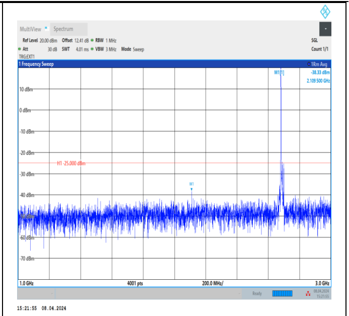
Band41_10MHz_QPSK_41540_1RB#0_1000~3000_1000~3000
