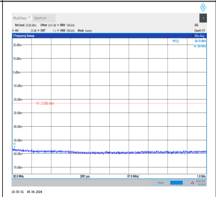
Band66_1.4MHz_QPSK_132322_1RB#0_30~1000_30~100 0
