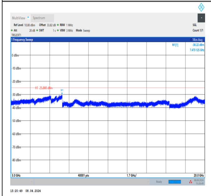
Band41_10MHz_QPSK_39700_1RB#0_3000~20000_3000~20000
