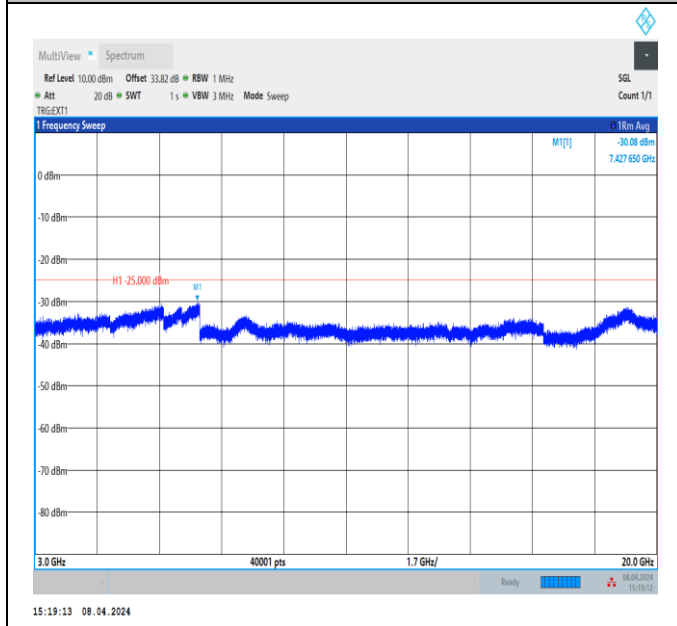
Band41_5MHz_QPSK_40620_1RB#0_3000~20000_3000~20000
