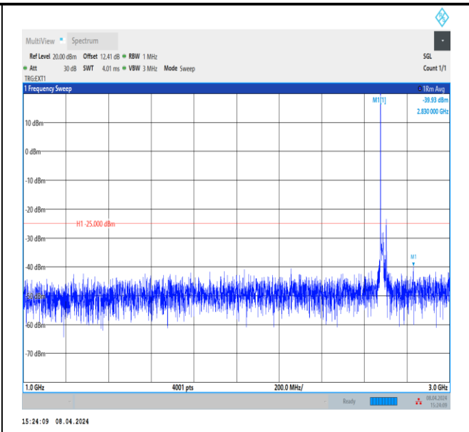
Band41_15MHz_QPSK_41515_1RB#0_1000~3000_1000~3000
