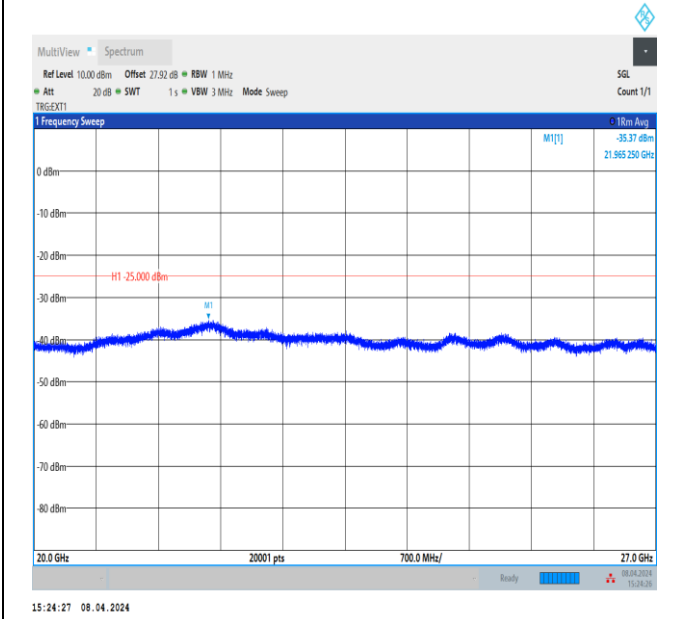
Band41_15MHz_QPSK_41515_1RB#0_20000~27000_20000~27000
