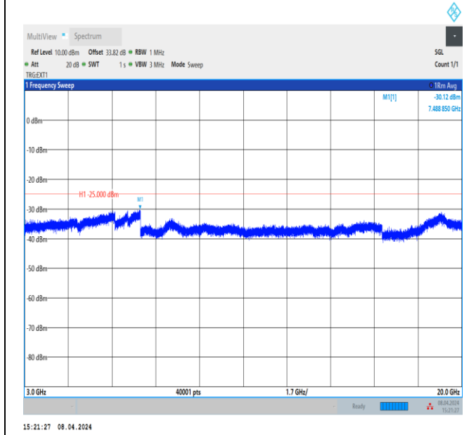
Band41_10MHz_QPSK_40620_1RB#0_3000~20000_3000~20000
