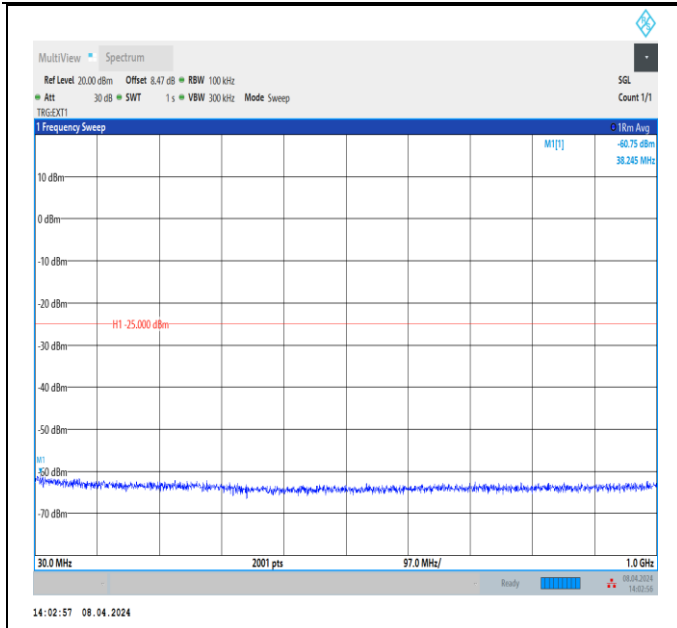
Band38_20MHz_QPSK_38000_1RB#0_30~1000_30~1000
