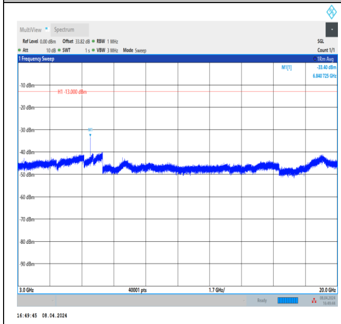
Band66_1.4MHz_QPSK_131979_1RB#0_3000~20000_300 0~20000
