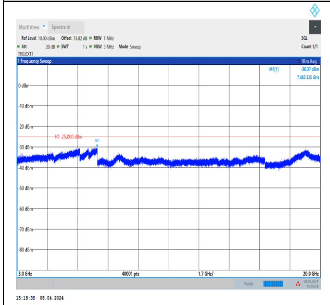
Band41_5MHz_QPSK_39675_1RB#0_3000~20000_3000~20000 0000
