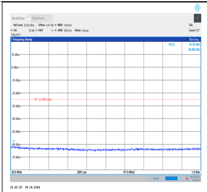
Band41_10MHz_QPSK_39700_1RB#0_30~1000_30~1000
