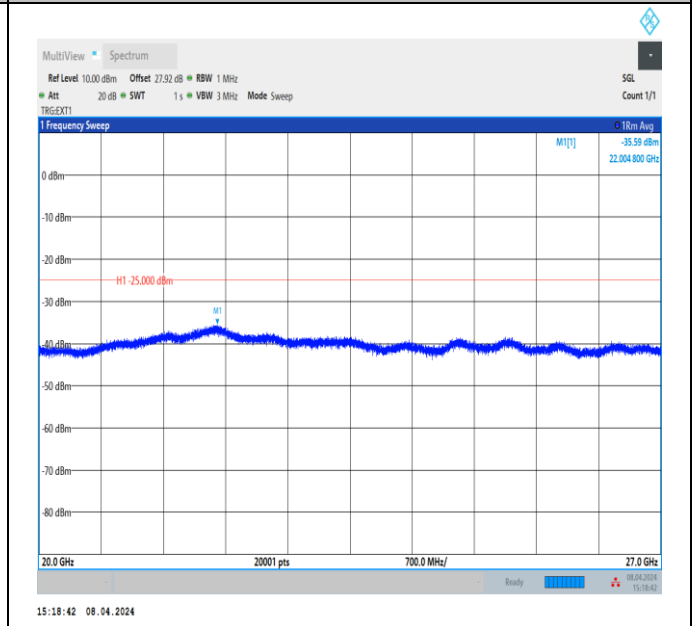
Band41_5MHz_QPSK_39675_1RB#0_20000~27000_20000~27000
