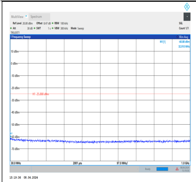
Band41_5MHz_QPSK_41565_1RB#0_30~1000_30~1000
