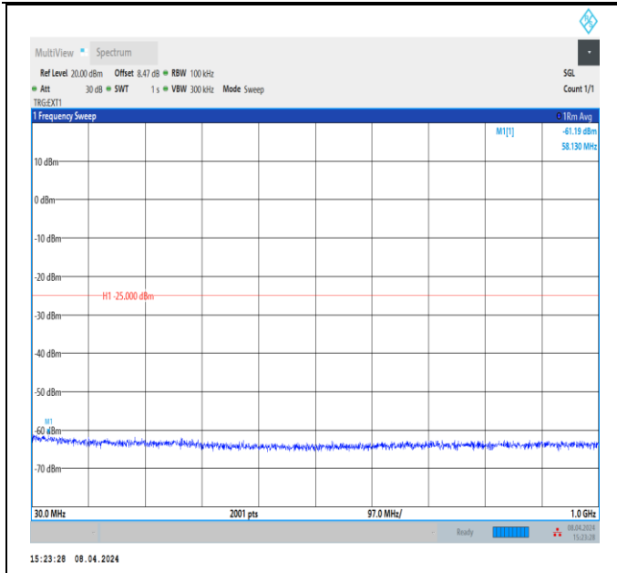
Band41_15MHz_QPSK_40620_1RB#0_30~1000_30~1000
