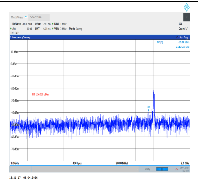
Band41_10MHz_QPSK_40620_1RB#0_1000~3000_1000~3000
