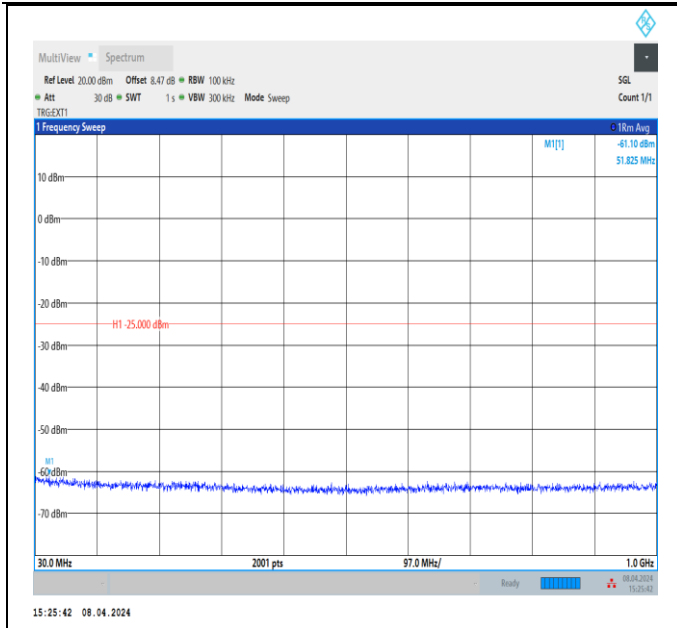
Band41_20MHz_QPSK_40620_1RB#0_30~1000_30~1000
