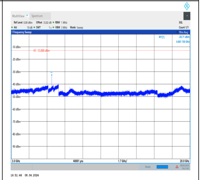
Band66_3MHz_QPSK_131987_1RB#0_3000~20000_3000~20000
