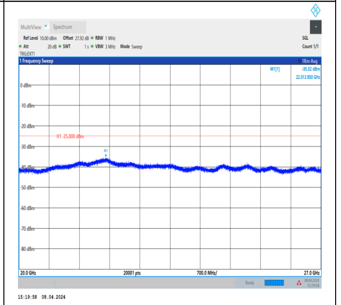
Band41_5MHz_QPSK_41565_1RB#0_20000~27000_20000~27000
