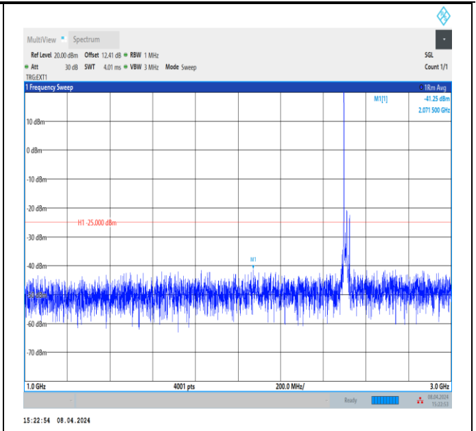
Band41_15MHz_QPSK_39725_1RB#0_1000~3000_1000~3000
