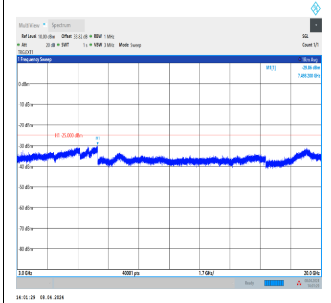
Band38_15MHz_QPSK_38175_1RB#0_3000~20000_3000~20000
