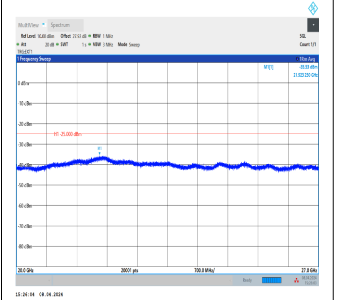
Band41_20MHz_QPSK_40620_1RB#0_20000~27000_20000~27000
