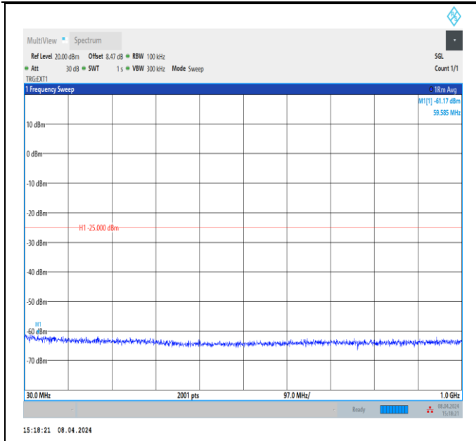
Band41_5MHz_QPSK_39675_1RB#0_30~1000_30~1000
