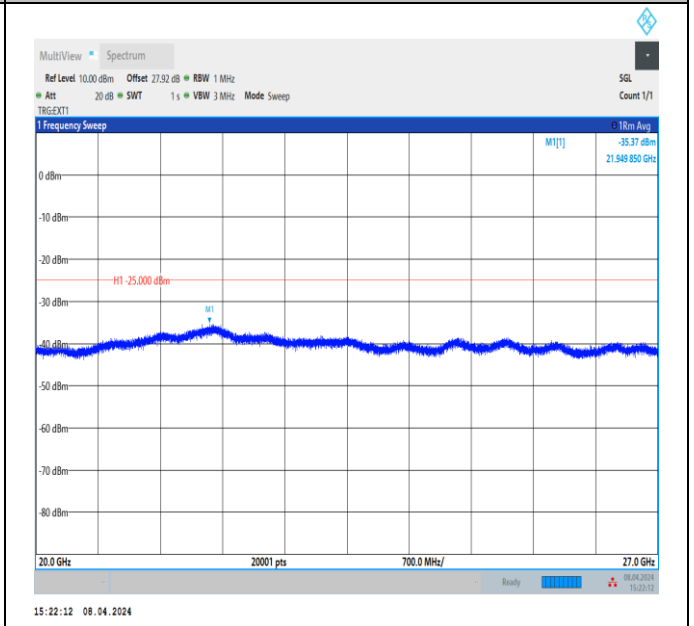
Band41_10MHz_QPSK_41540_1RB#0_20000~27000_20000~27000
