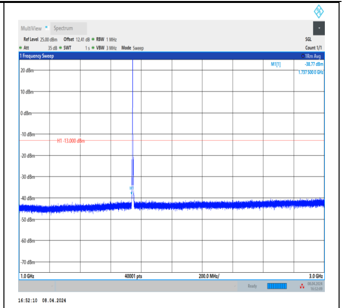
Band66_3MHz_QPSK_132322_1RB#0_1000~3000_1000~3000
