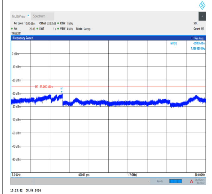
Band41_15MHz_QPSK_40620_1RB#0_3000~20000_3000~20000
