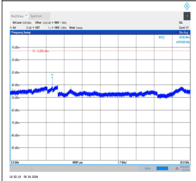
Band66_3MHz_QPSK_132322_1RB#0_3000~20000_3000~20000
