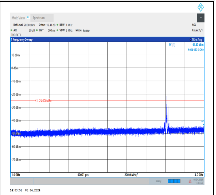
Band38_20MHz_QPSK_38150_1RB#0_1000~3000_1000~3000
