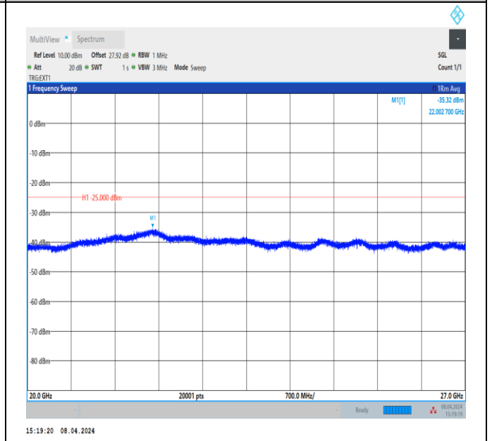
Band41_5MHz_QPSK_40620_1RB#0_20000~27000_20000~27000
