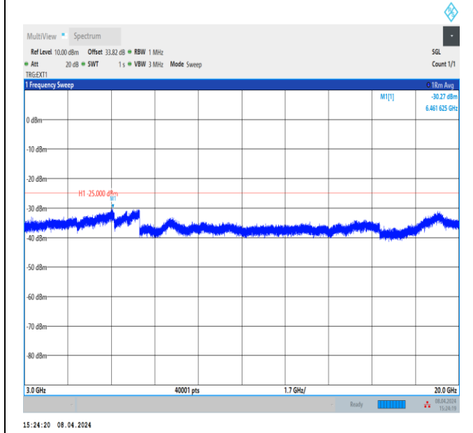
Band41_15MHz_QPSK_41515_1RB#0_3000~20000_3000~20000
