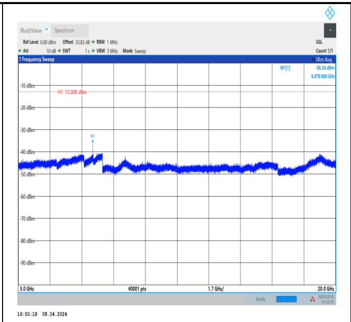
Band66_1.4MHz_QPSK_132322_1RB#0_3000~20000_3000 ~20000
