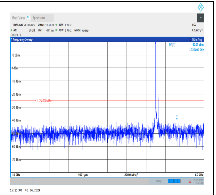
Band41_20MHz_QPSK_39750_1RB#0_1000~3000_1000~3000
