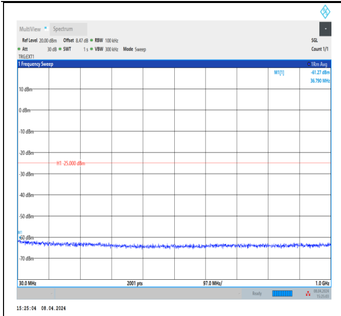
Band41_20MHz_QPSK_39750_1RB#0_30~1000_30~1000
