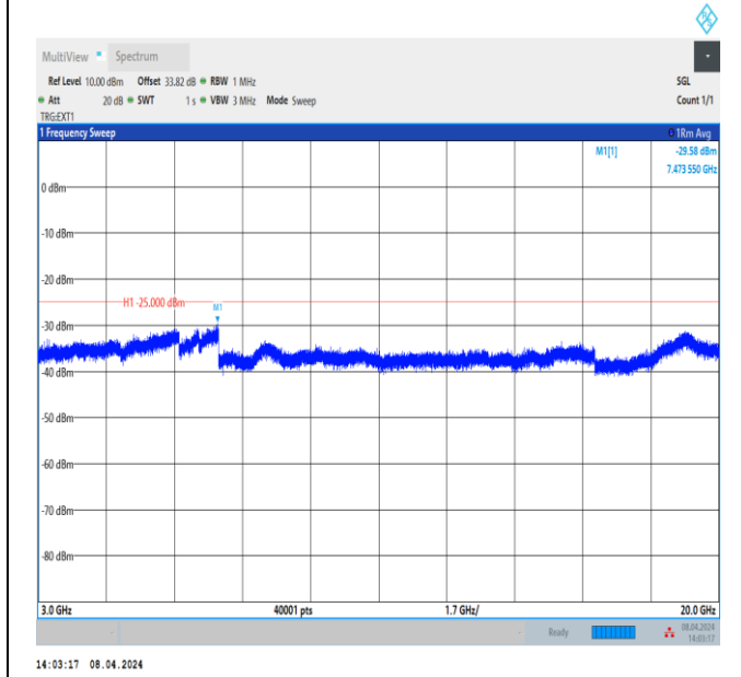
Band38_20MHz_QPSK_38000_1RB#0_3000~20000_3000~20000
