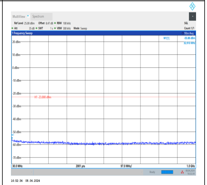
Band66_3MHz_QPSK_132657_1RB#0_30~1000_30~1000
