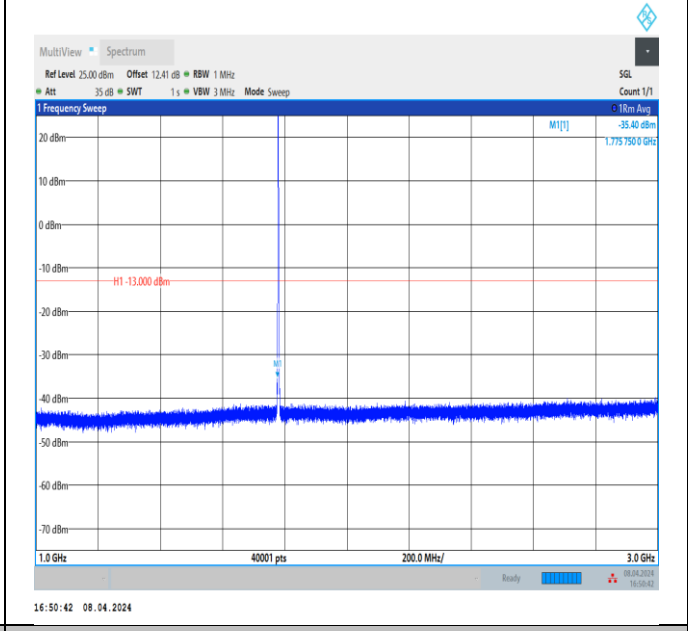
Band66_1.4MHz_QPSK_132665_1RB#0_1000~3000_1000 ~3000
