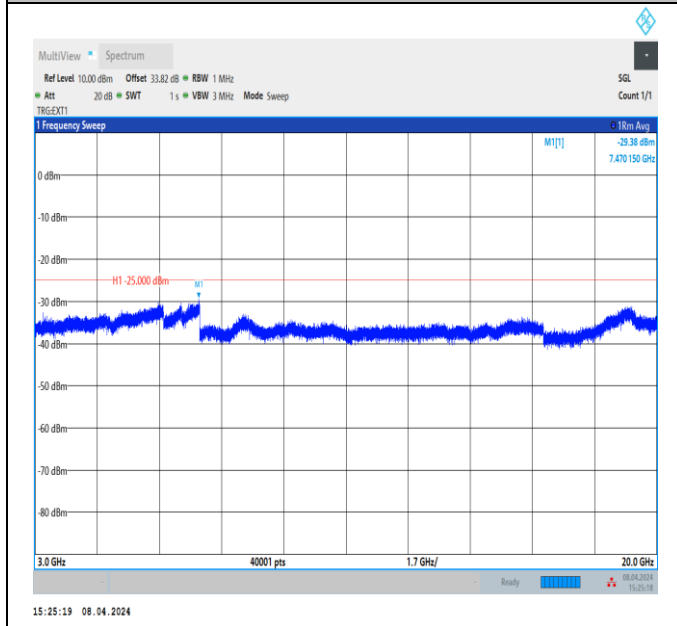
Band41_20MHz_QPSK_39750_1RB#0_3000~20000_3000~20000
