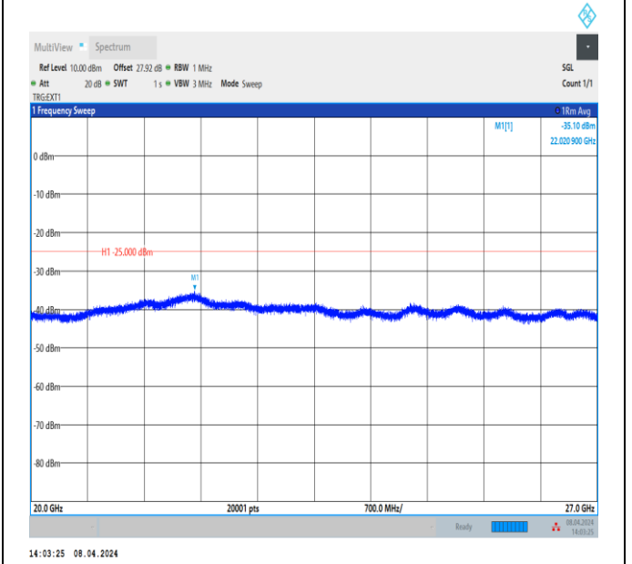
Band38_20MHz_QPSK_38000_1RB#0_20000~27000_20000~27000
