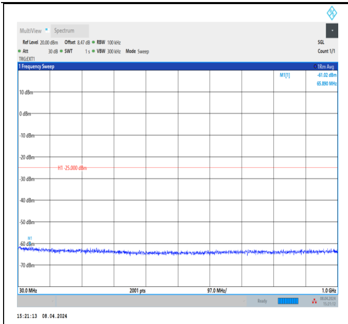
Band41_10MHz_QPSK_40620_1RB#0_30~1000_30~1000
