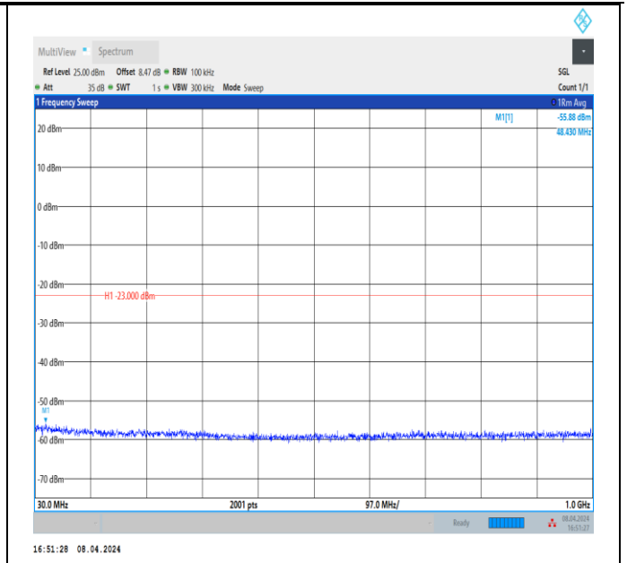
Band66_3MHz_QPSK_131987_1RB#0_30~1000_30~1000
