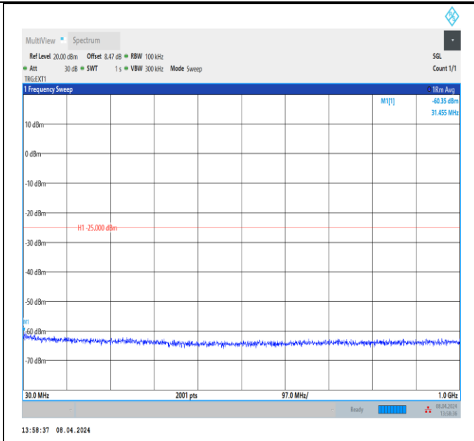
Band38_10MHz_QPSK_38200_1RB#0_30~1000_30~1000
