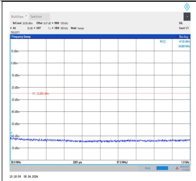
Band41_5MHz_QPSK_40620_1RB#0_30~1000_30~1000
