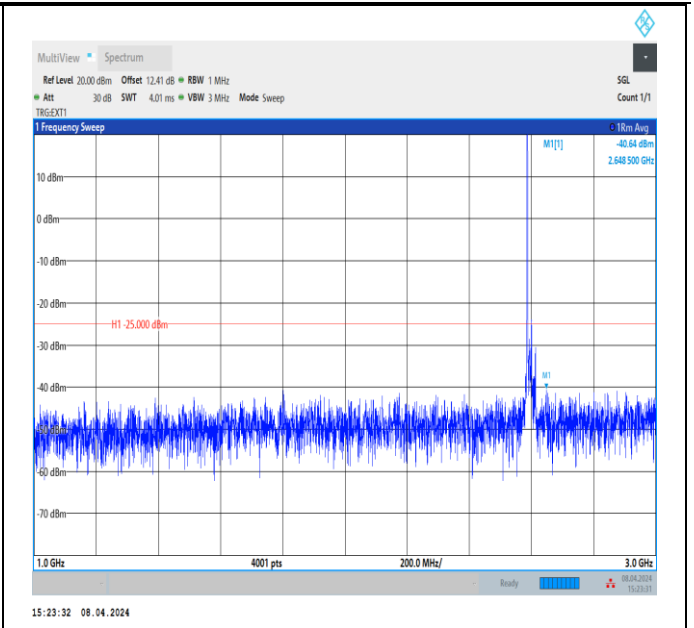
Band41_15MHz_QPSK_40620_1RB#0_1000~3000_1000~3000
