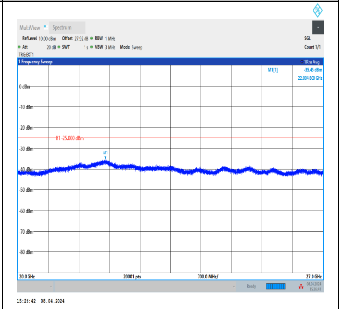
Band41_20MHz_QPSK_41490_1RB#0_20000~27000_20000~27000
