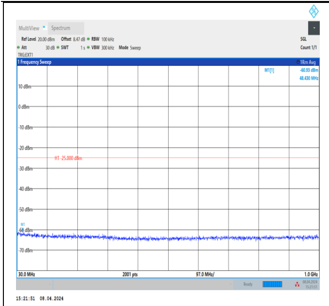
Band41_10MHz_QPSK_41540_1RB#0_30~1000_30~1000
