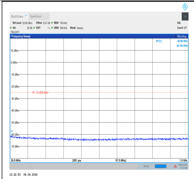
Band41_15MHz_QPSK_39725_1RB#0_30~1000_30~1000
