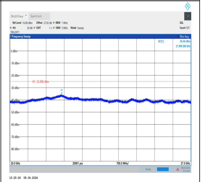
Band41_20MHz_QPSK_39750_1RB#0_20000~27000_20000~27000
