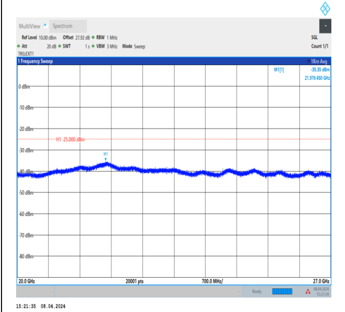
Band41_10MHz_QPSK_40620_1RB#0_20000~27000_20000~27000
