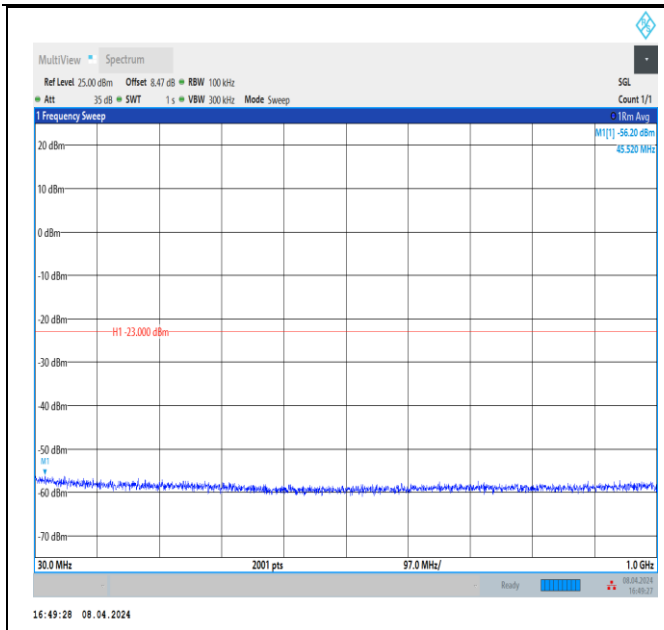
Band66_1.4MHz_QPSK_131979_1RB#0_30~1000_30~100 0
