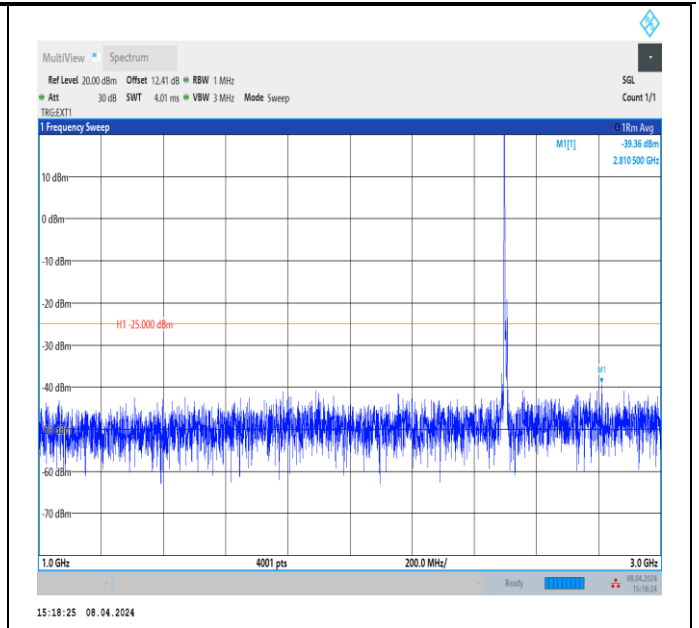
Band41_5MHz_QPSK_39675_1RB#0_1000~3000_1000~3000 00
