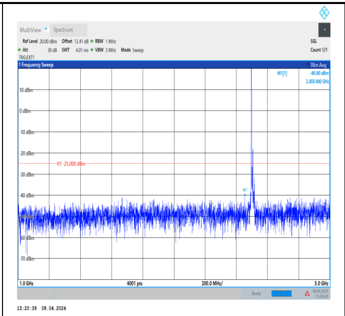
Band41_10MHz_QPSK_39700_1RB#0_1000~3000_1000~3000
