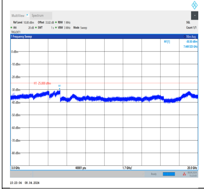
Band41_15MHz_QPSK_39725_1RB#0_3000~20000_3000~20000
