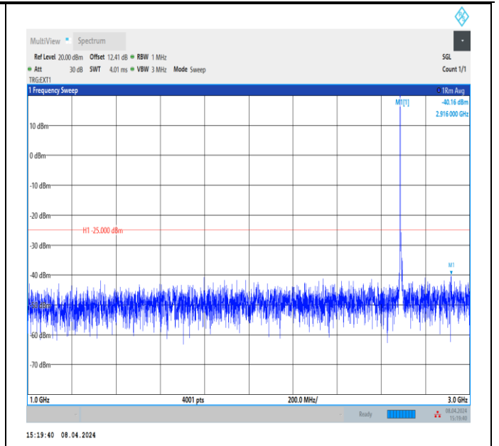
Band41_5MHz_QPSK_41565_1RB#0_1000~3000_1000~3000 00
