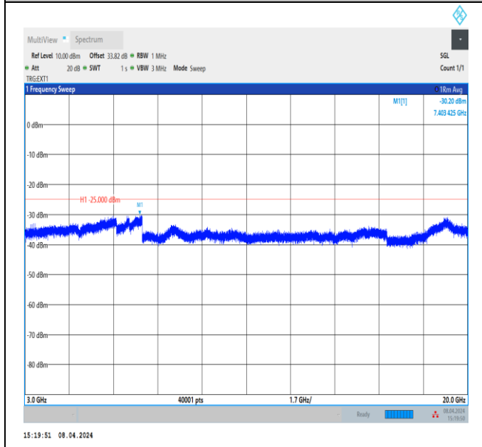
Band41_5MHz_QPSK_41565_1RB#0_3000~20000_3000~20000 0000
