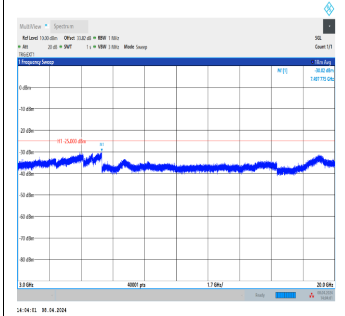
Band38_20MHz_QPSK_38150_1RB#0_3000~20000_3000~20000
