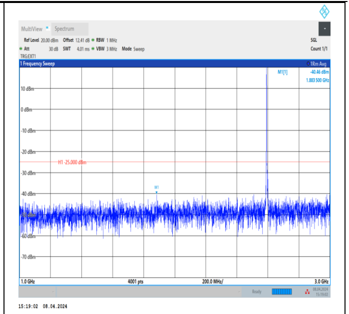
Band41_5MHz_QPSK_40620_1RB#0_1000~3000_1000~3000
