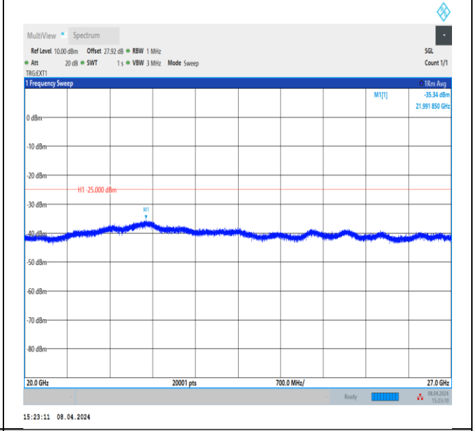
Band41_15MHz_QPSK_39725_1RB#0_20000~27000_20000~27000
