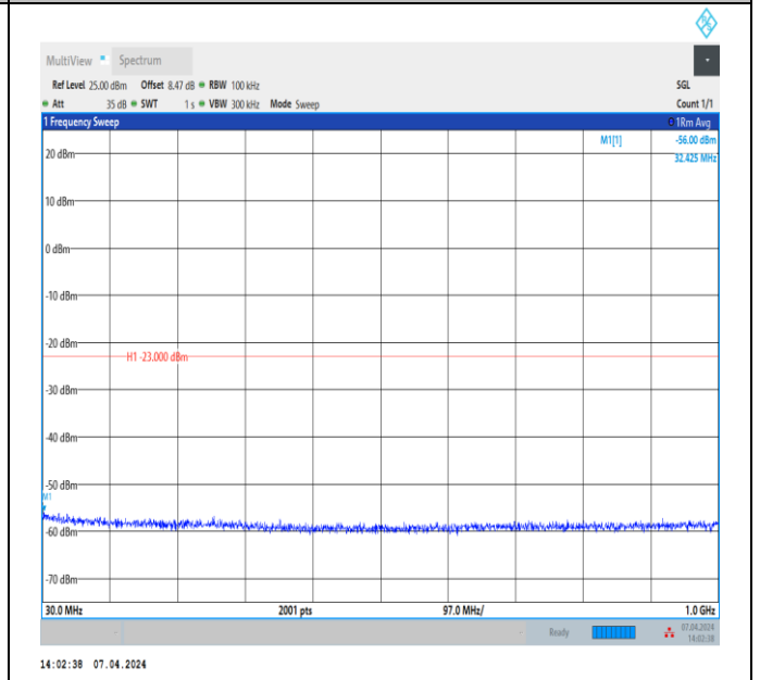
Band4_3MHz_QPSK_19965_1RB#0_30~1000_30~1000
