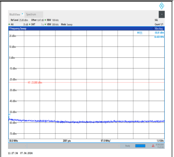
Band2_20MHz_QPSK_18700_1RB#0_30~1000_30~1000
