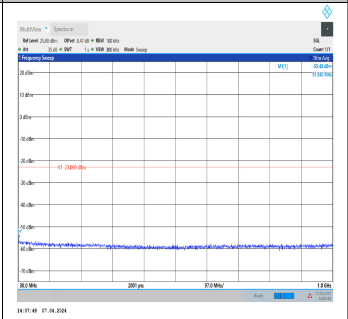
Band4_10MHz_QPSK_20350_1RB#0_30~1000_30~1000
