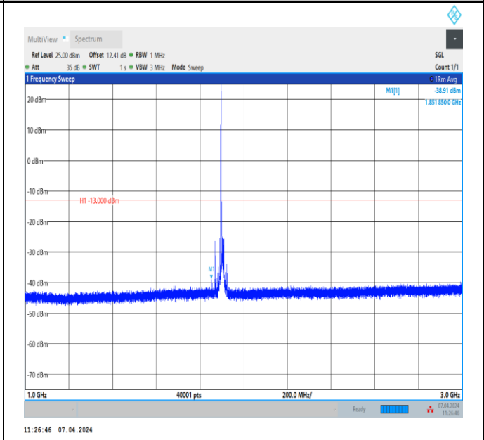
Band2_15MHz_QPSK_19125_1RB#0_1000~3000_1000~3000
