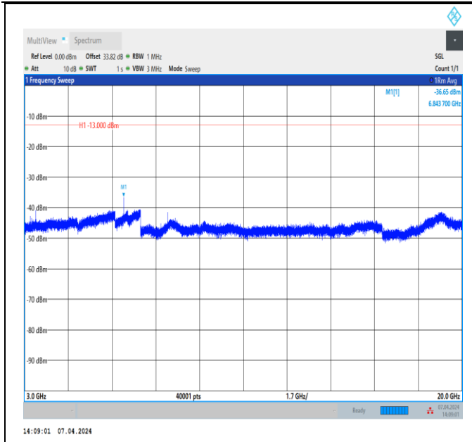
Band4_15MHz_QPSK_20025_1RB#0_3000~20000_3000~20000
