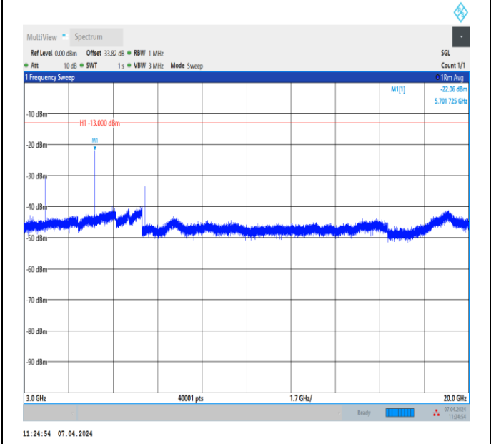
Band2_10MHz_QPSK_19150_1RB#0_3000~20000_3000~20000
