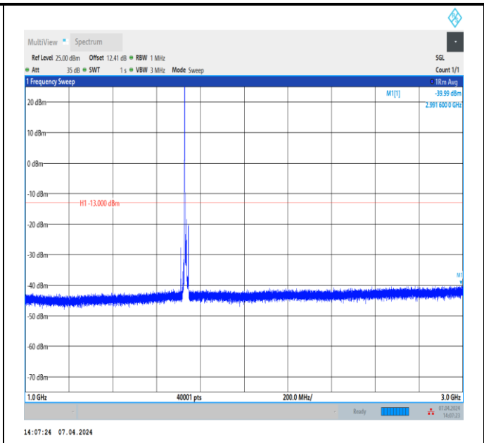
Band4_10MHz_QPSK_20175_1RB#0_1000~3000_1000~3000 00
