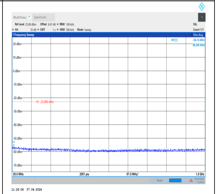
Band2_15MHz_QPSK_18900_1RB#0_30~1000_30~1000
