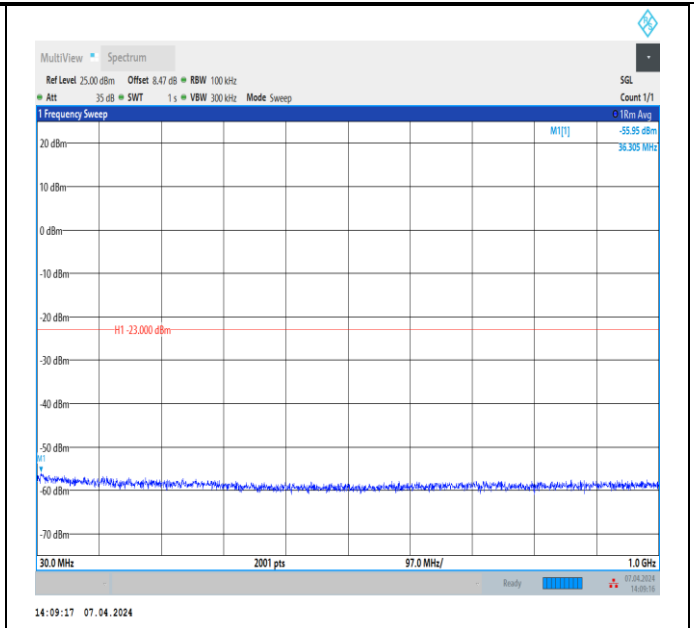
Band4_15MHz_QPSK_20175_1RB#0_30~1000_30~1000
