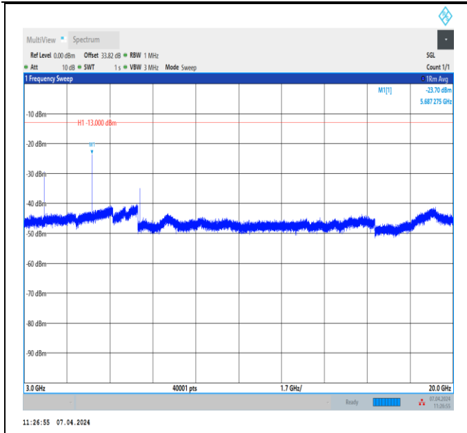
Band2_15MHz_QPSK_19125_1RB#0_3000~20000_3000~20000
