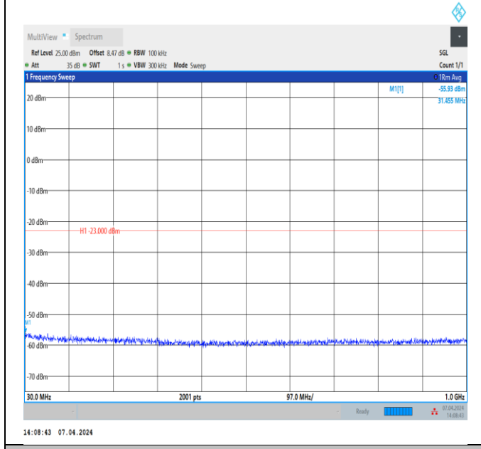
Band4_15MHz_QPSK_20025_1RB#0_30~1000_30~1000 00
