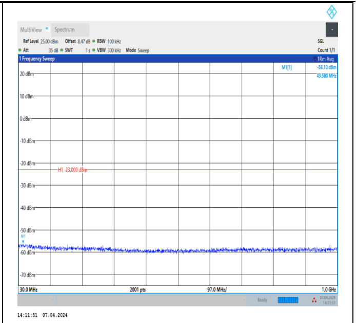
Band4_20MHz_QPSK_20300_1RB#0_30~1000_30~1000
