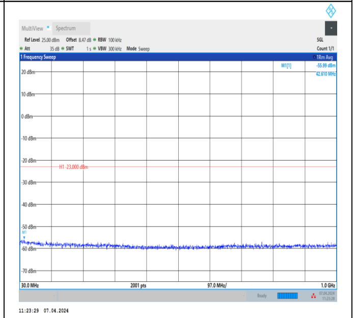
Band2_10MHz_QPSK_18650_1RB#0_30~1000_30~1000
