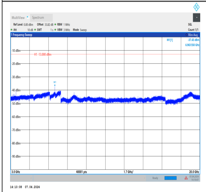
Band4_15MHz_QPSK_20325_1RB#0_3000~20000_3000~20000 0000
