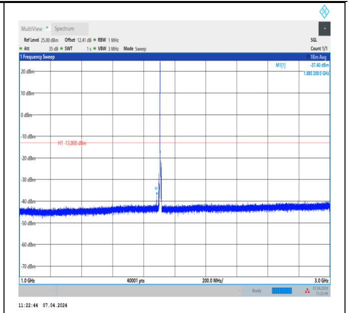
Band2_5MHz_QPSK_19175_1RB#0_1000~3000_1000~3000 0
