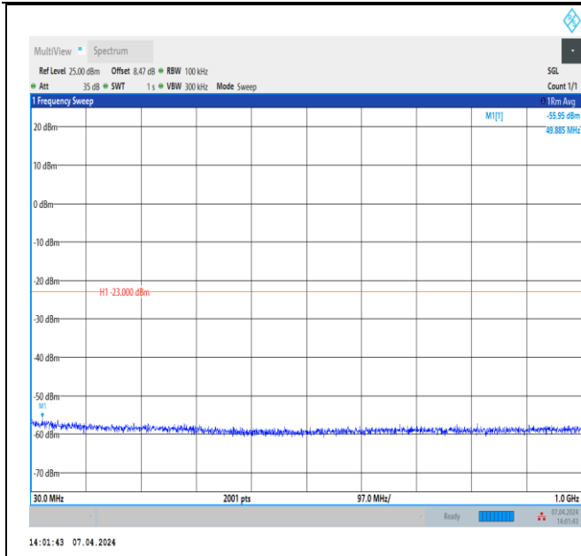
Band4_1.4MHz_QPSK_20393_1RB#0_30~1000_30~1000
