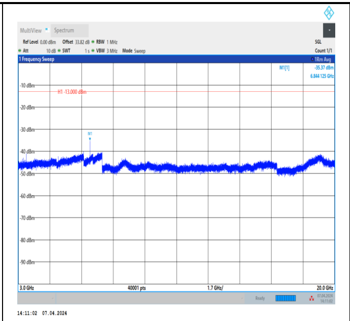
Band4_20MHz_QPSK_20050_1RB#0_3000~20000_3000~2 0000
