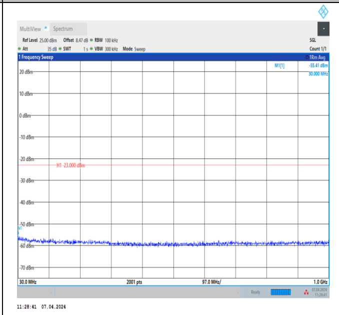
Band2_20MHz_QPSK_19100_1RB#0_30~1000_30~1000
