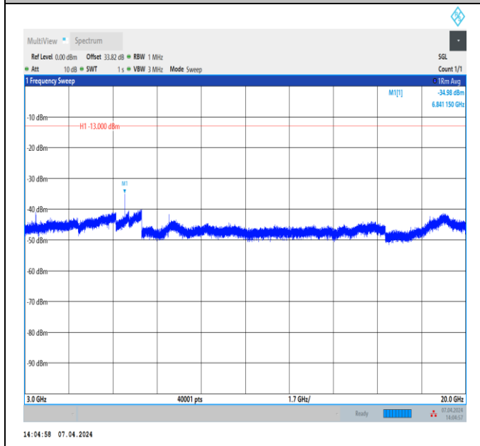
Band4_5MHz_QPSK_19975_1RB#0_3000~20000_3000~20000 000
