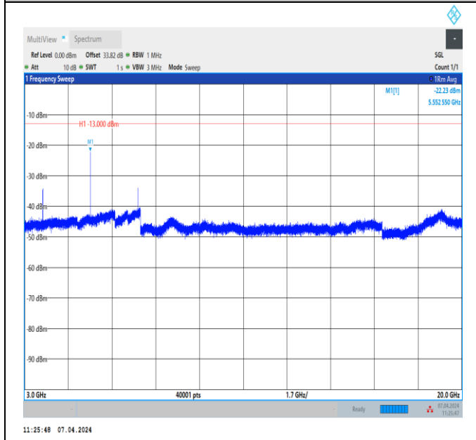
Band2_15MHz_QPSK_18675_1RB#0_3000~20000_3000~20000
