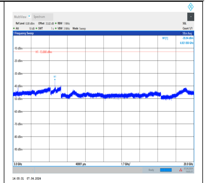
Band4_5MHz_QPSK_20175_1RB#0_3000~20000_3000~20 000
