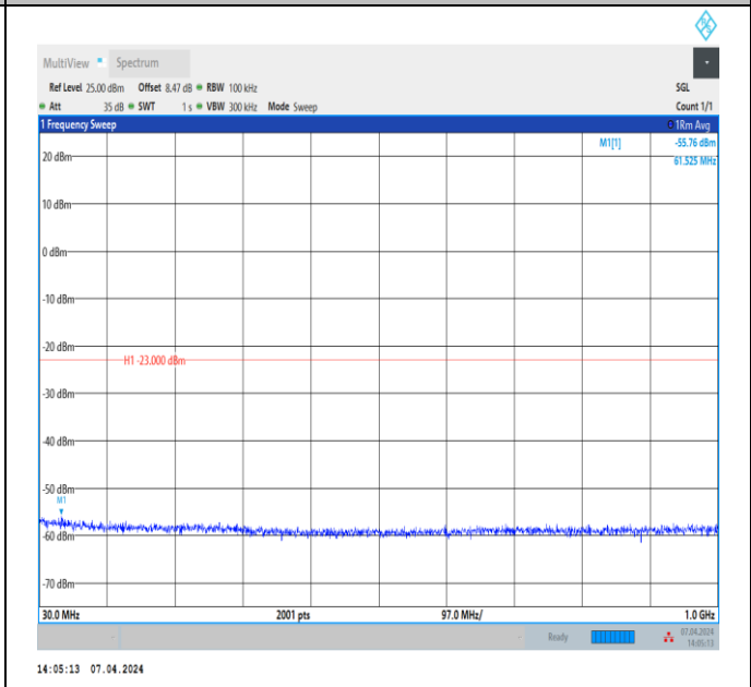
Band4_5MHz_QPSK_20175_1RB#0_30~1000_30~1000
