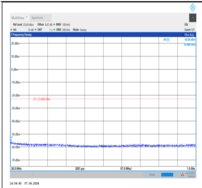
Band4_5MHz_QPSK_19975_1RB#0_30~1000_30~1000
