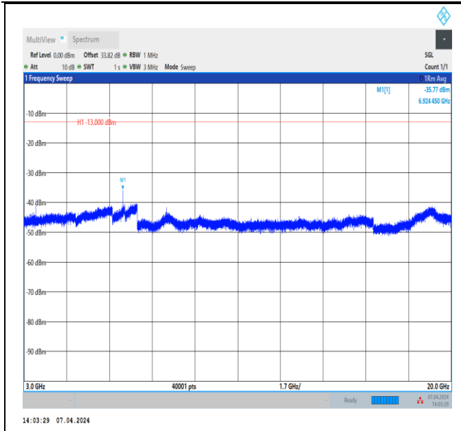
Band4_3MHz_QPSK_20175_1RB#0_3000~20000_3000~20000
