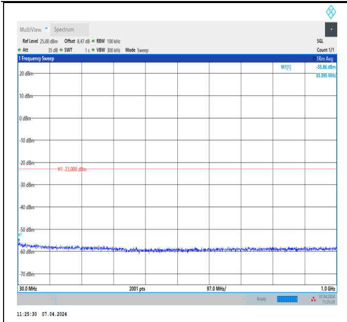
Band2_15MHz_QPSK_18675_1RB#0_30~1000_30~1000
