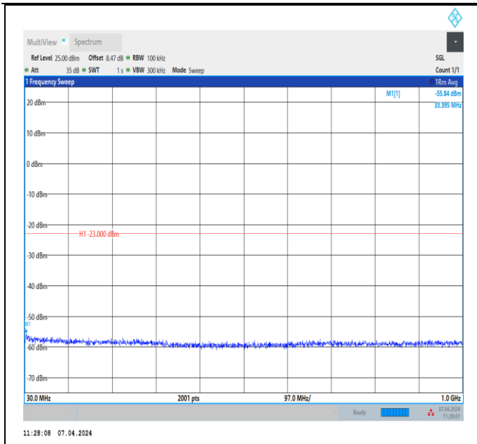
Band2_20MHz_QPSK_18900_1RB#0_30~1000_30~1000
