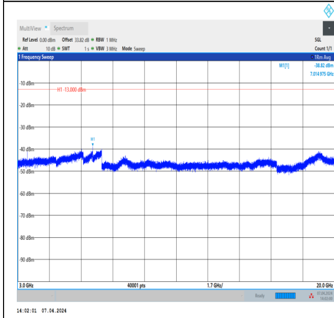
Band4_1.4MHz_QPSK_20393_1RB#0_3000~20000_3000~20000
