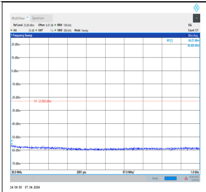
Band4_15MHz_QPSK_20325_1RB#0_30~1000_30~1000
