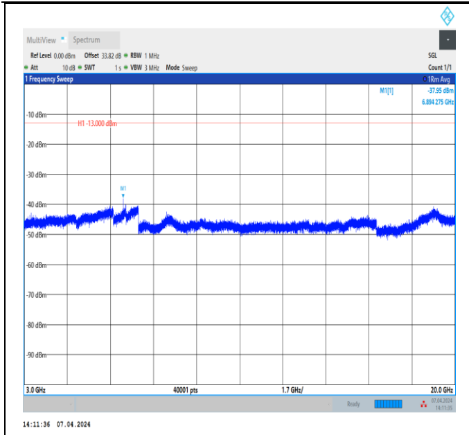
Band4_20MHz_QPSK_20175_1RB#0_3000~20000_3000~20000
