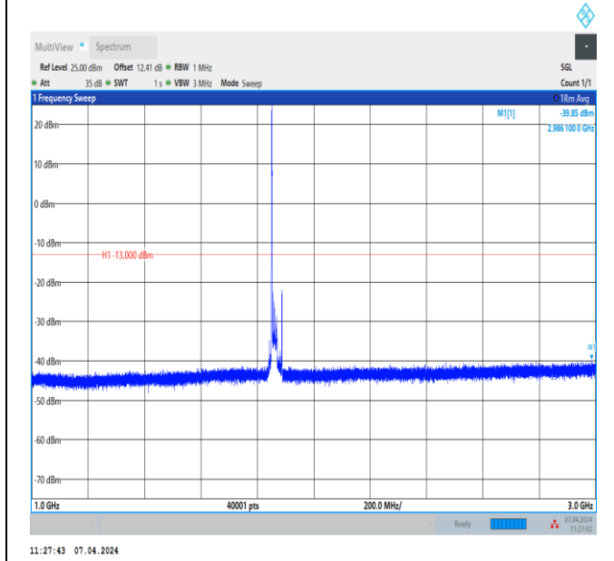
Band2_20MHz_QPSK_18700_1RB#0_1000~3000_1000~3000
