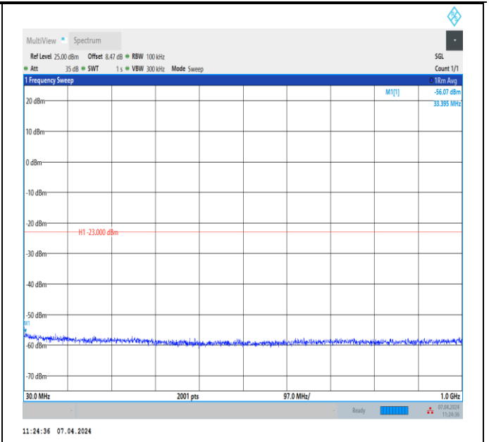
Band2_10MHz_QPSK_19150_1RB#0_30~1000_30~1000
