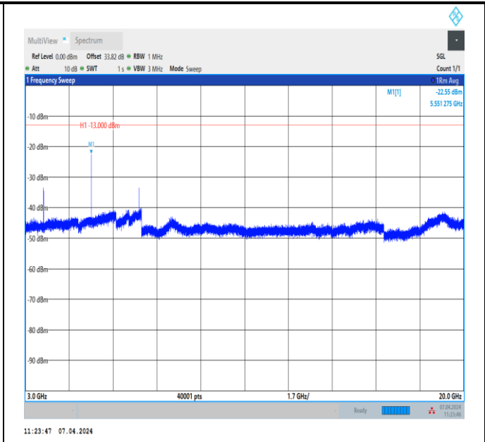
Band2_10MHz_QPSK_18650_1RB#0_3000~20000_3000~20000 0000
