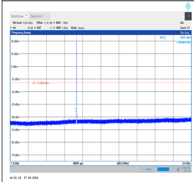
Band4_1.4MHz_QPSK_20175_1RB#0_1000~3000_1000~3000
