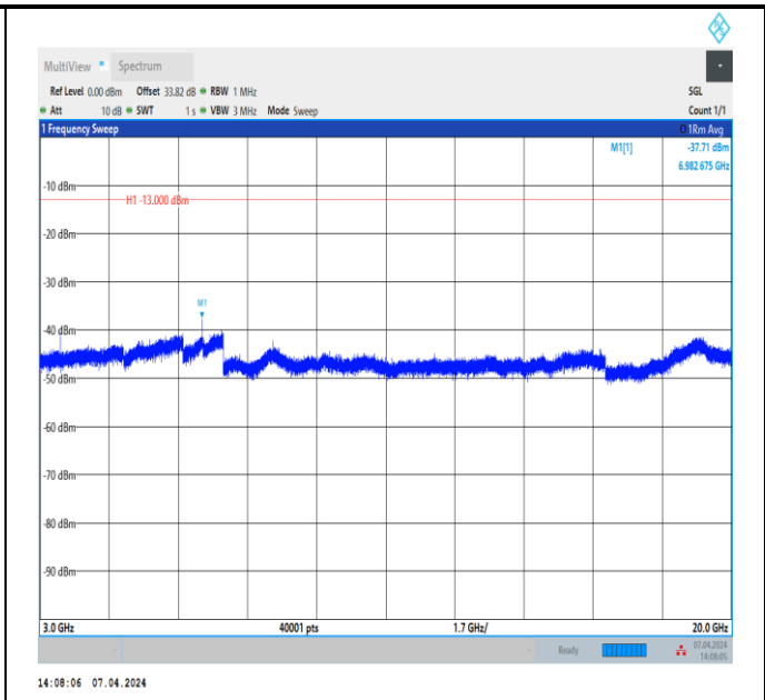
Band4_10MHz_QPSK_20350_1RB#0_3000~20000_3000~2 0000
