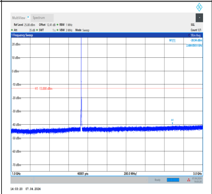
Band4_3MHz_QPSK_20175_1RB#0_1000~3000_1000~300 0
