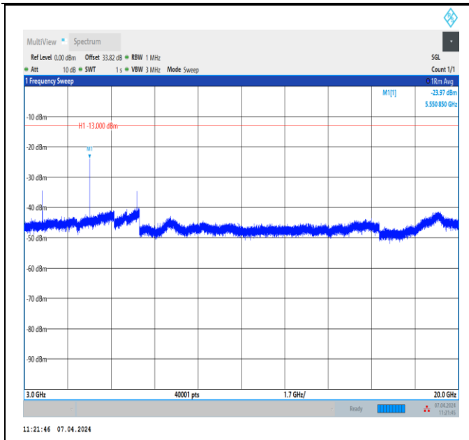
Band2_5MHz_QPSK_18625_1RB#0_3000~20000_3000~2000
