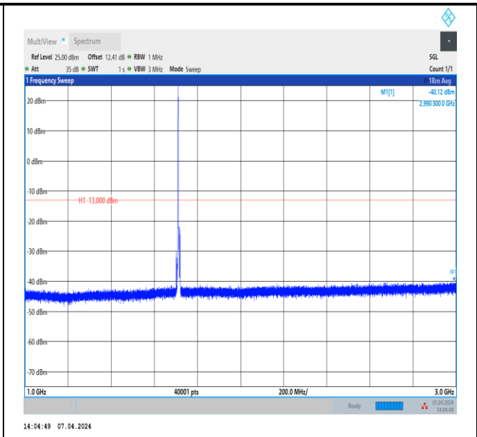
Band4_5MHz_QPSK_19975_1RB#0_1000~3000_1000~3000 0
