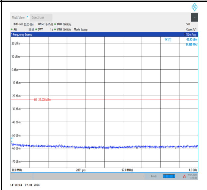
Band4_20MHz_QPSK_20050_1RB#0_30~1000_30~1000
