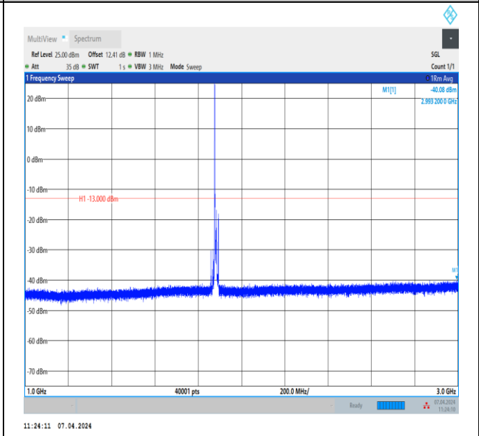
Band2_10MHz_QPSK_18900_1RB#0_1000~3000_1000~3000 00
