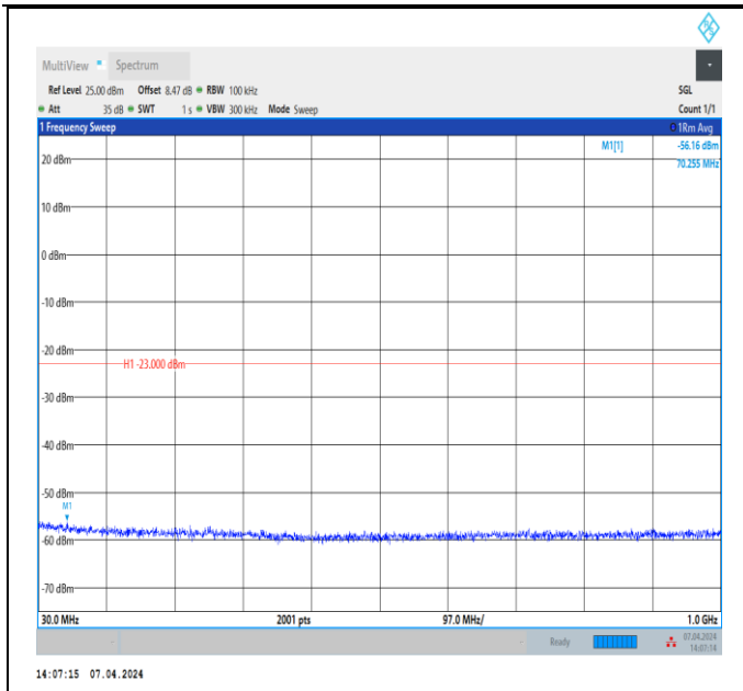
Band4_10MHz_QPSK_20175_1RB#0_30~1000_30~1000
