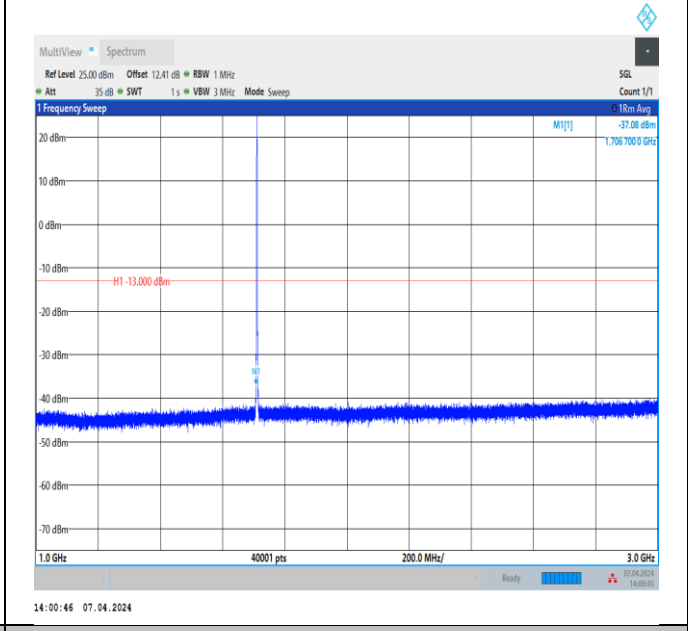
Band4_1.4MHz_QPSK_19957_1RB#0_1000~3000_1000~3000
