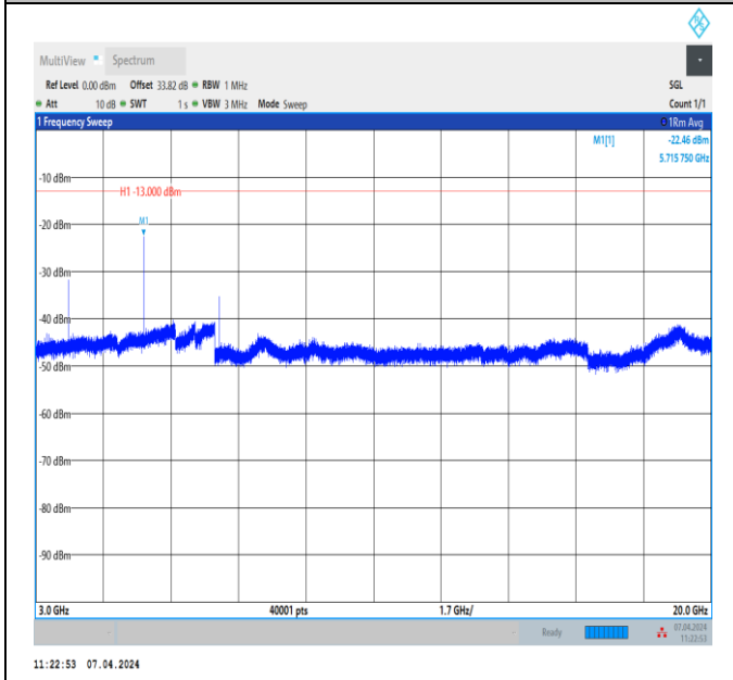
Band2_5MHz_QPSK_19175_1RB#0_3000~20000_3000~20000 000
