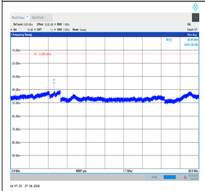
Band4_10MHz_QPSK_20175_1RB#0_3000~20000_3000~20000 0000
