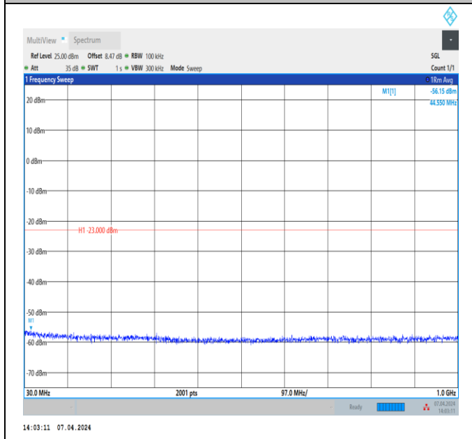
Band4_3MHz_QPSK_20175_1RB#0_30~1000_30~1000 0
