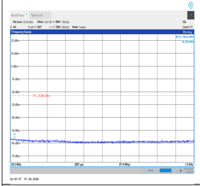
Band4_1.4MHz_QPSK_19957_1RB#0_30~1000_30~1000
