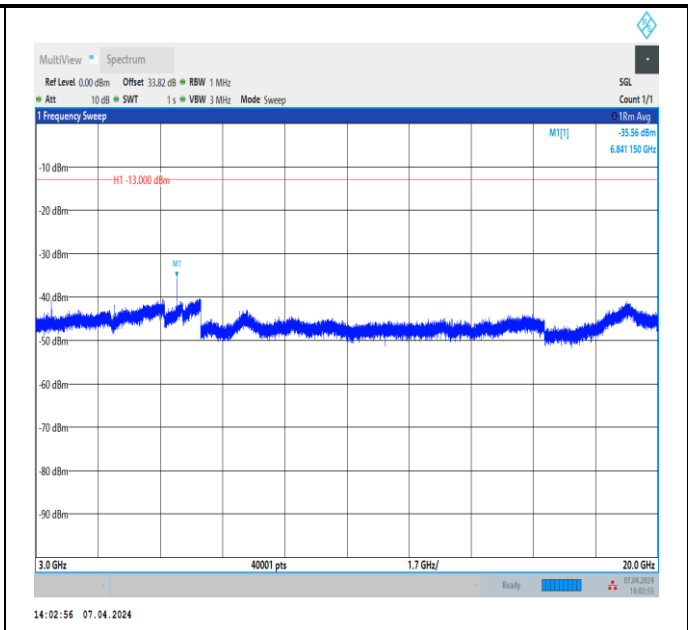
Band4_3MHz_QPSK_19965_1RB#0_3000~20000_3000~20 000
