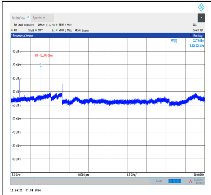
Band2_10MHz_QPSK_18900_1RB#0_3000~20000_3000~20000
