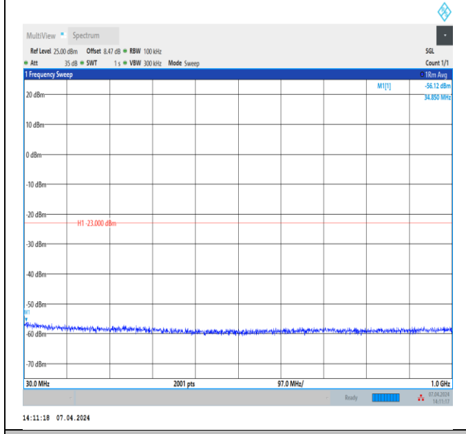
Band4_20MHz_QPSK_20175_1RB#0_30~1000_30~1000 00
