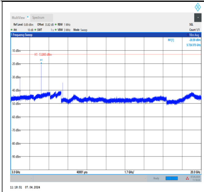
Band2_1.4MHz_QPSK_19193_1RB#0_3000~20000_3000~20000
