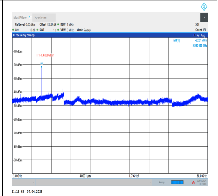
Band2_3MHz_QPSK_18615_1RB#0_3000~20000_3000~20000
