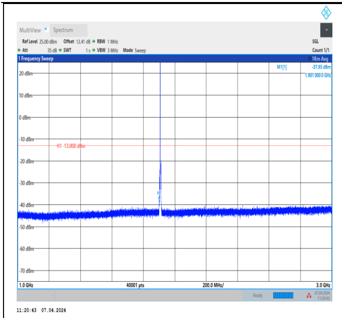
Band2_3MHz_QPSK_19185_1RB#0_1000~3000_1000~300 0
