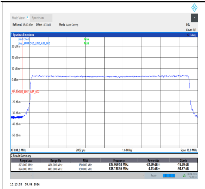
Band26_15MHz_QPSK_26865_75RB#0
