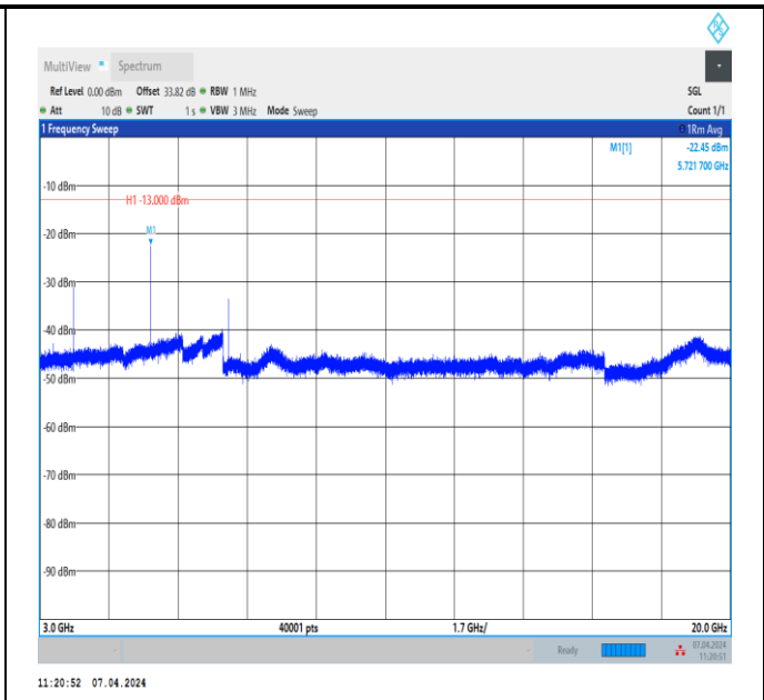
Band2_3MHz_QPSK_19185_1RB#0_3000~20000_3000~20 000
