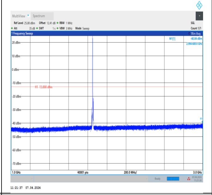
Band2_5MHz_QPSK_18625_1RB#0_1000~3000_1000~300 0
