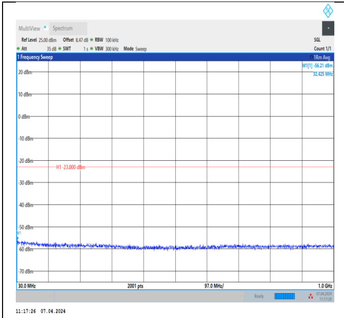
Band2_1.4MHz_QPSK_18607_1RB#0_30~1000_30~1000
