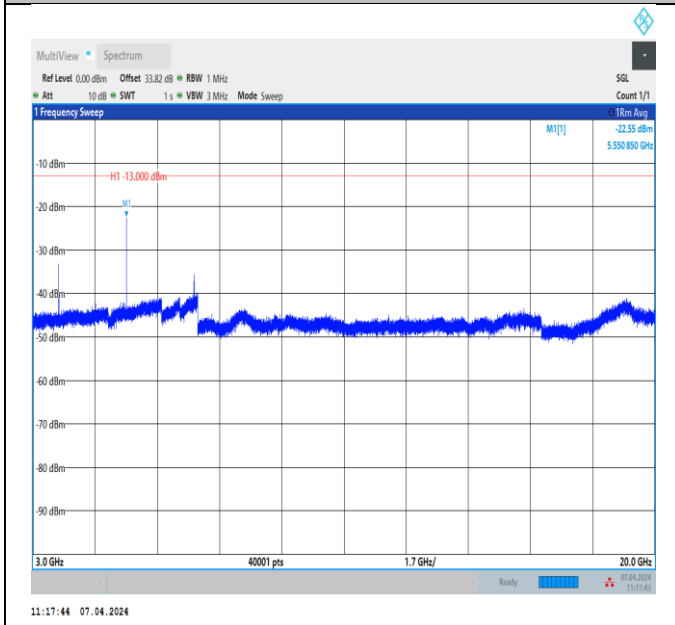
Band2_1.4MHz_QPSK_18607_1RB#0_3000~20000_3000~20000
