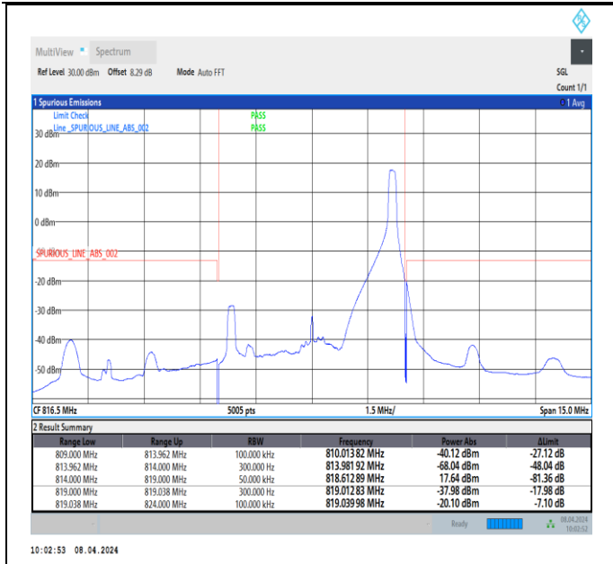
Band26_5MHz_64QAM_26715_1RB#24
