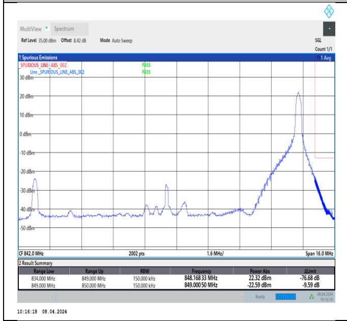
Band26_15MHz_64QAM_26965_1RB#74
