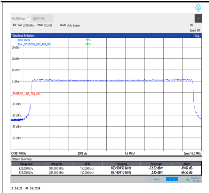
Band26_15MHz_64QAM_26865_75RB#0
