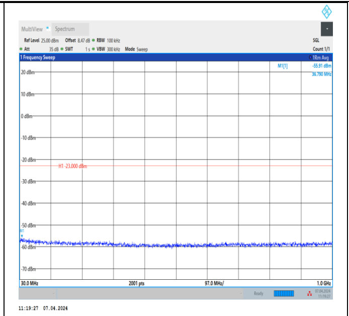
Band2_3MHz_QPSK_18615_1RB#0_30~1000_30~1000
