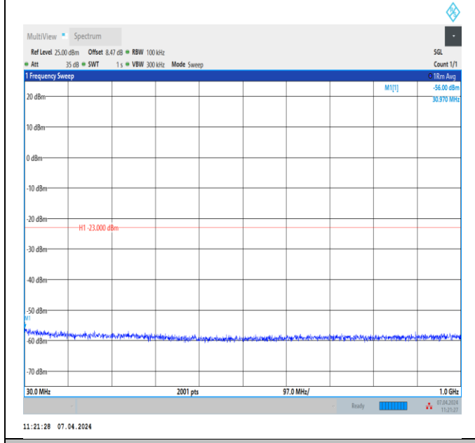
Band2_5MHz_QPSK_18625_1RB#0_30~1000_30~1000 0
