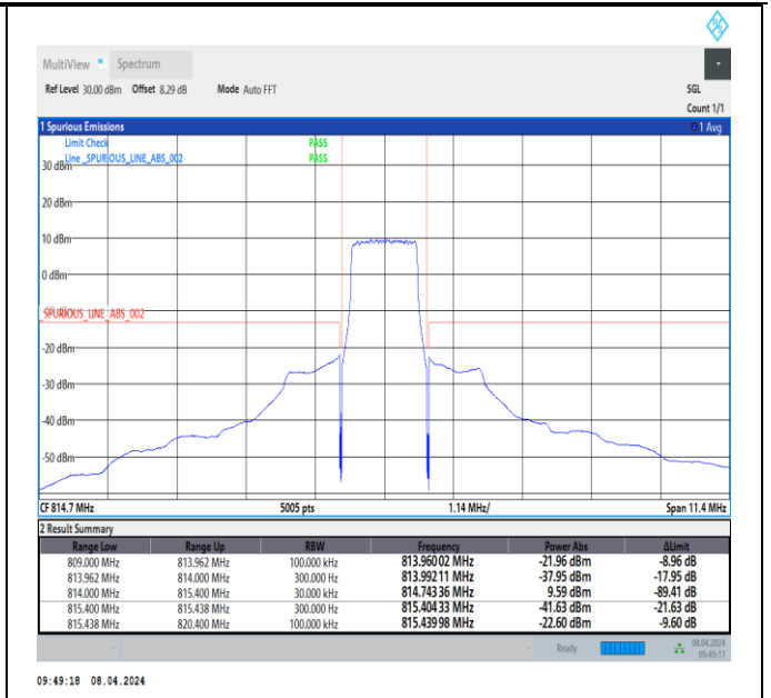
Band26_1.4MHz_QPSK_26697_6RB#0
