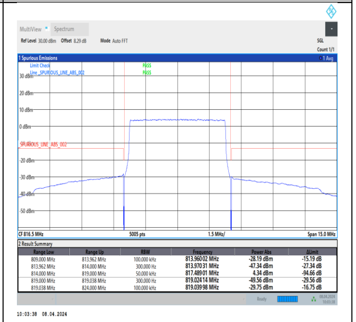
Band26_5MHz_16QAM_26715_25RB#0
