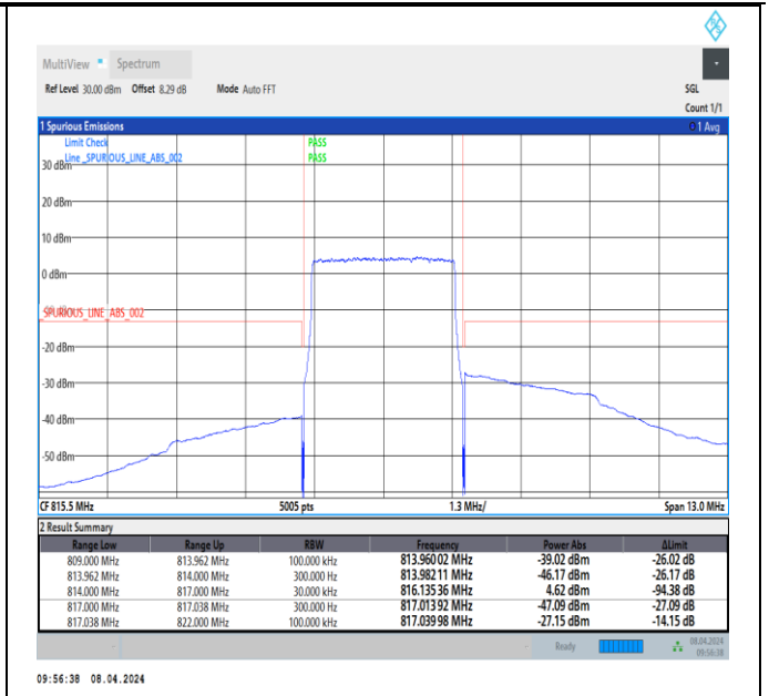
Band26_3MHz_16QAM_26705_15RB#0
