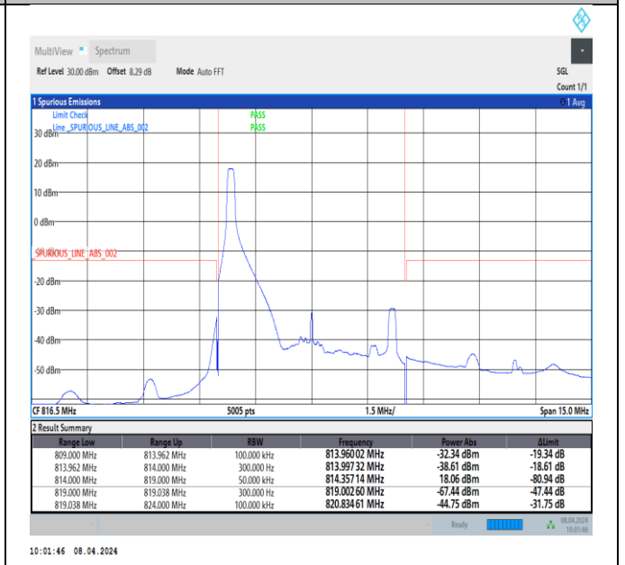
Band26_5MHz_64QAM_26715_1RB#0
