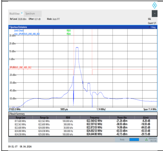
Band26_1.4MHz_64QAM_26783_1RB#0
