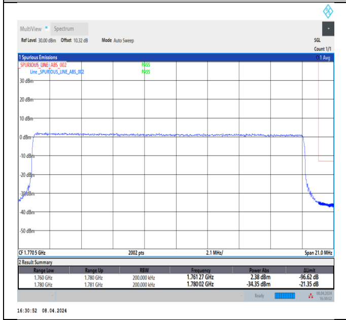
Band66_20MHz_64QAM_132572_100RB#0
