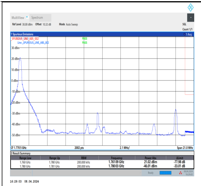
Band66_20MHz_64QAM_132572_1RB#0
