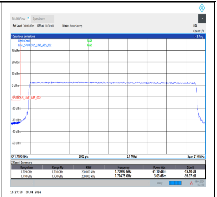
Band66_20MHz_16QAM_132072_100RB#0
