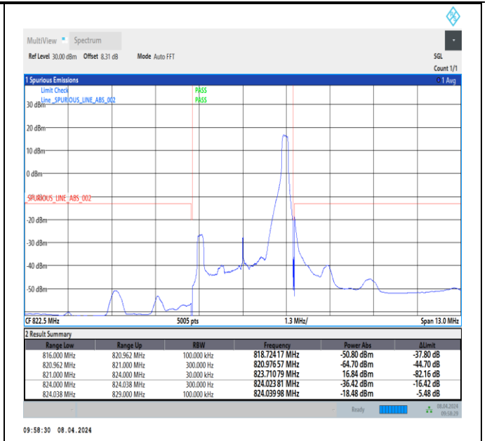
Band26_3MHz_QPSK_26775_1RB#14
