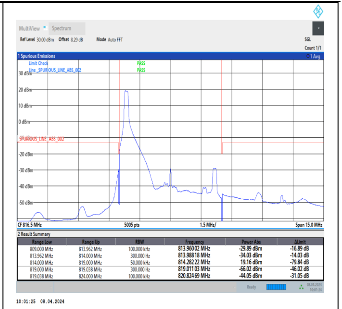
Band26_5MHz_16QAM_26715_1RB#0
