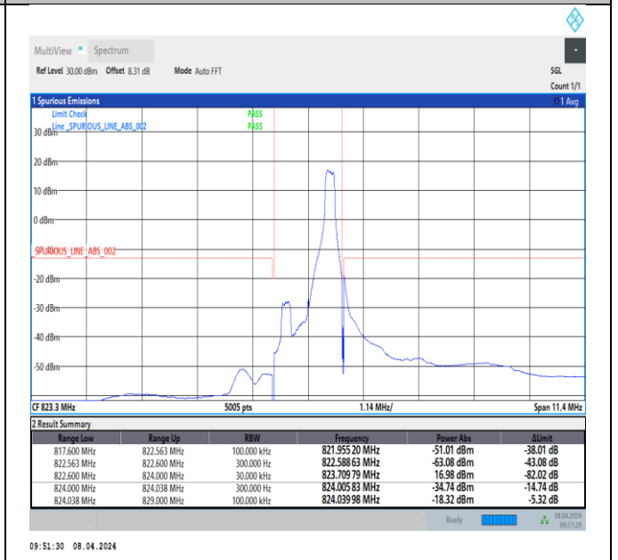
Band26_1.4MHz_QPSK_26783_1RB#5
