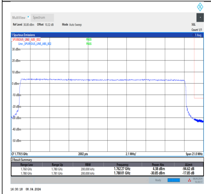
Band66_20MHz_QPSK_132572_100RB#0
