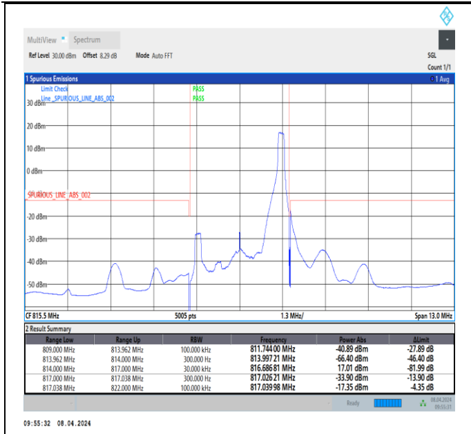
Band26_3MHz_16QAM_26705_1RB#14
