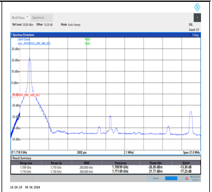
Band66_20MHz_64QAM_132072_1RB#0
