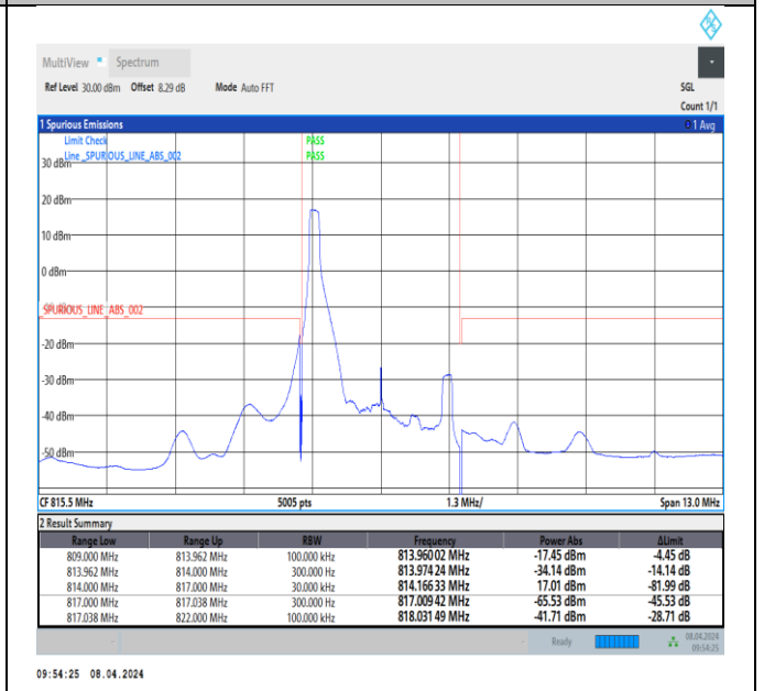
Band26_3MHz_16QAM_26705_1RB#0
