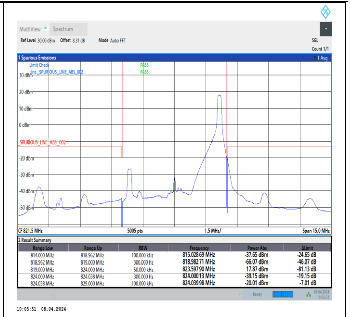
Band26_5MHz_16QAM_26765_1RB#24
