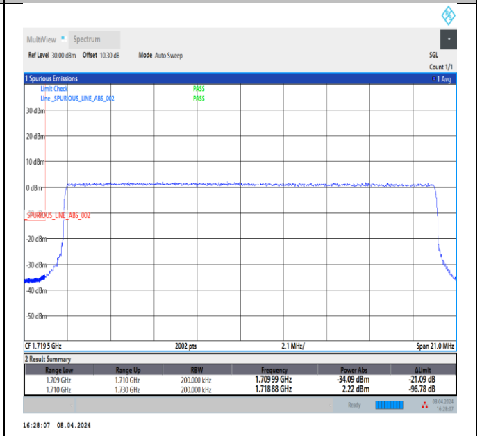
Band66_20MHz_64QAM_132072_100RB#0
