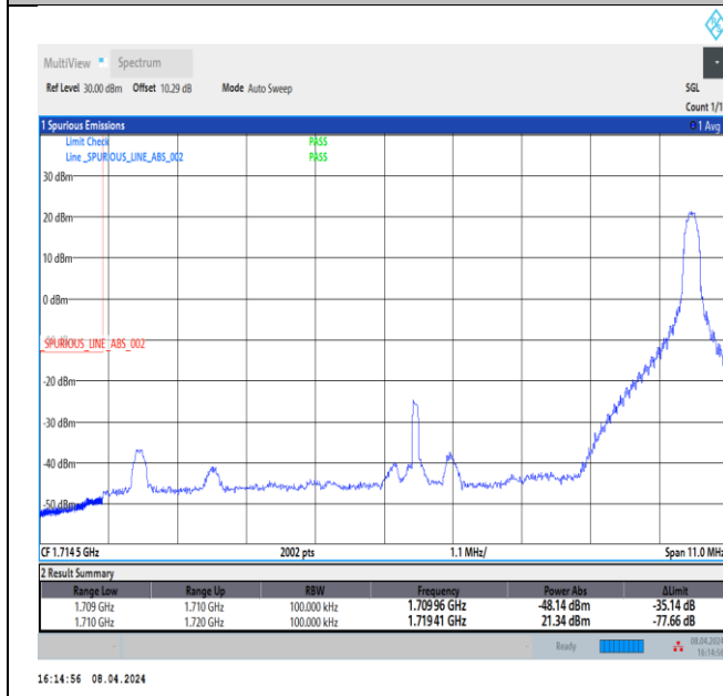
Band66_10MHz_QPSK_132022_1RB#49
