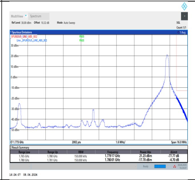
Band66_15MHz_64QAM_132597_1RB#74
