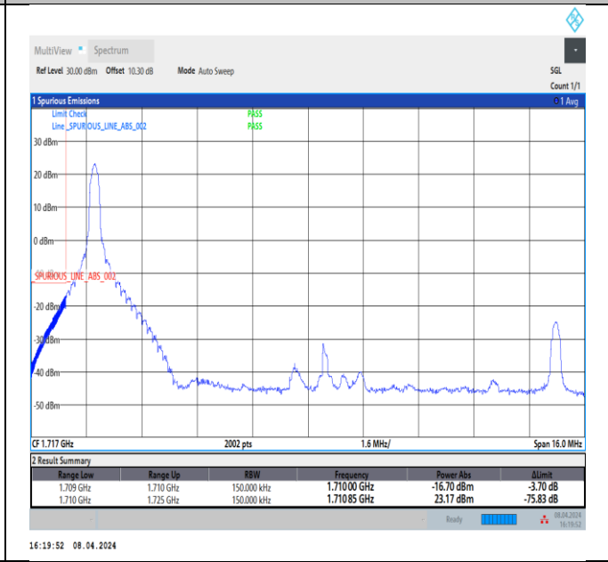
Band66_15MHz_QPSK_132047_1RB#0
