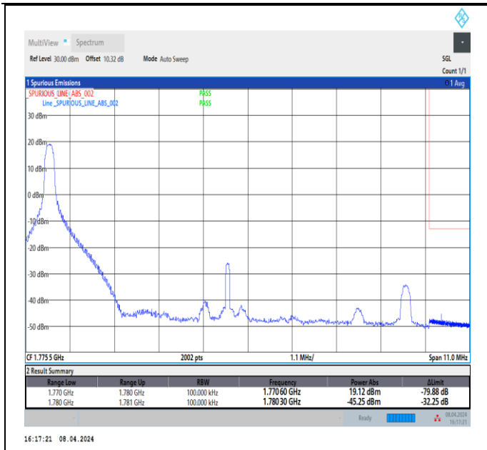
Band66_10MHz_64QAM_132622_1RB#0
