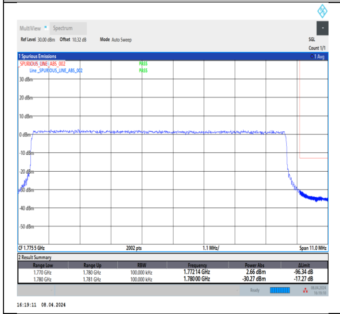
Band66_10MHz_64QAM_132622_50RB#0
