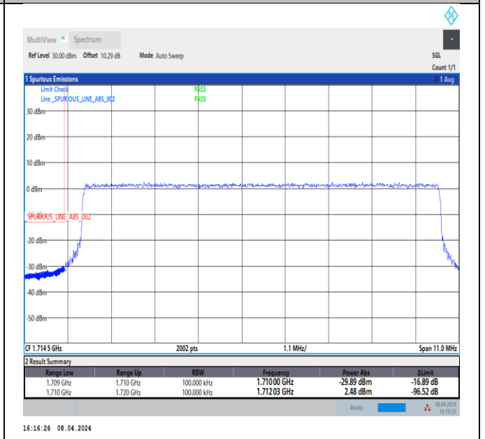
Band66_10MHz_64QAM_132022_50RB#0
