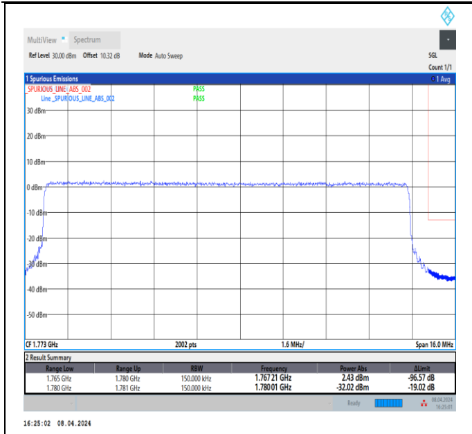
Band66_15MHz_64QAM_132597_75RB#0
