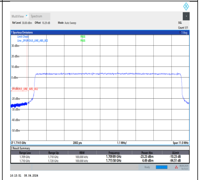
Band66_10MHz_QPSK_132022_50RB#0
