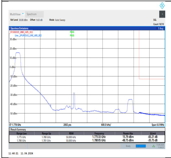
Band66_5MHz_64QAM_132647_1RB#0
