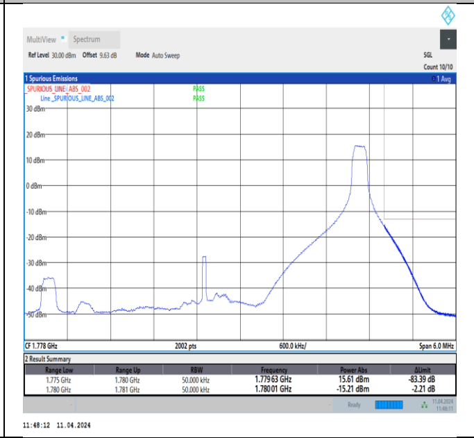
Band66_5MHz_64QAM_132647_1RB#24
