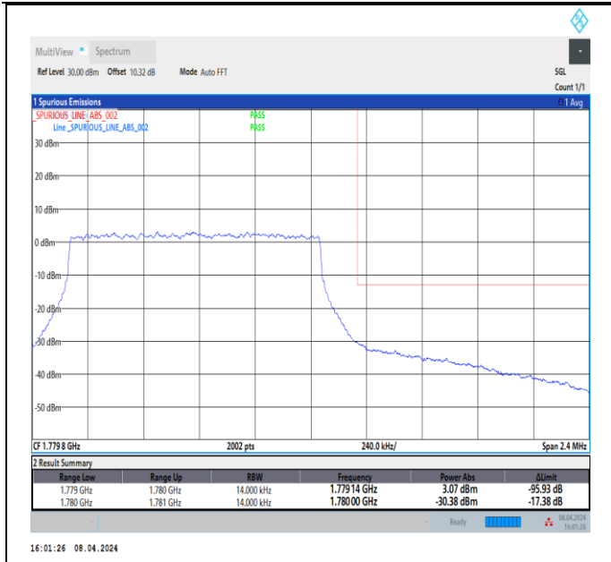
Band66_1.4MHz_64QAM_132665_6RB#0
