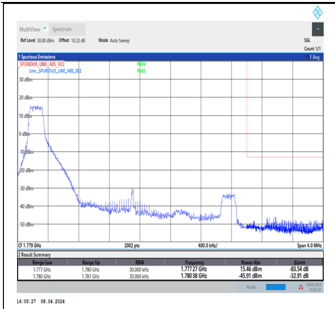
Band66_3MHz_64QAM_132657_1RB#0
