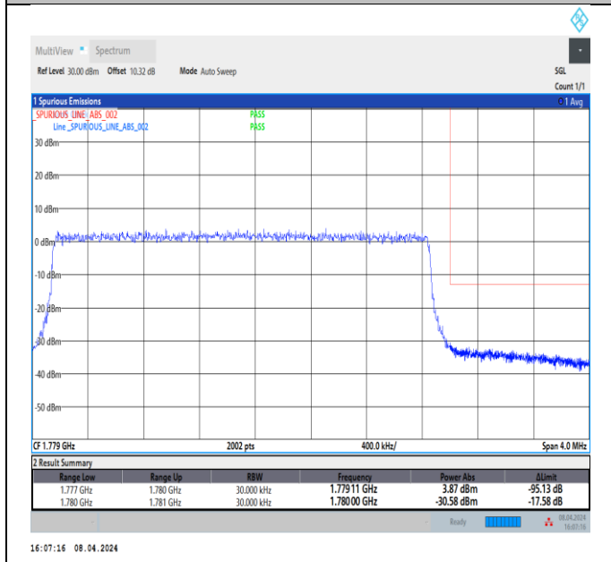
Band66_3MHz_64QAM_132657_15RB#0
