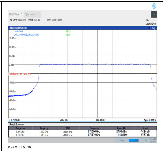
Band66_5MHz_64QAM_131997_25RB#0
