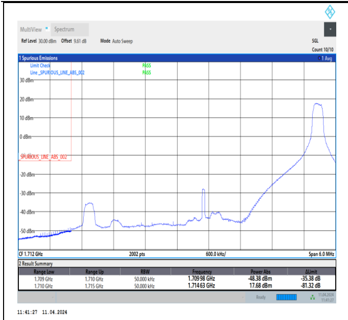
Band66_5MHz_QPSK_131997_1RB#24
