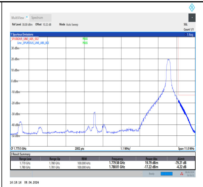
Band66_10MHz_64QAM_132622_1RB#49
