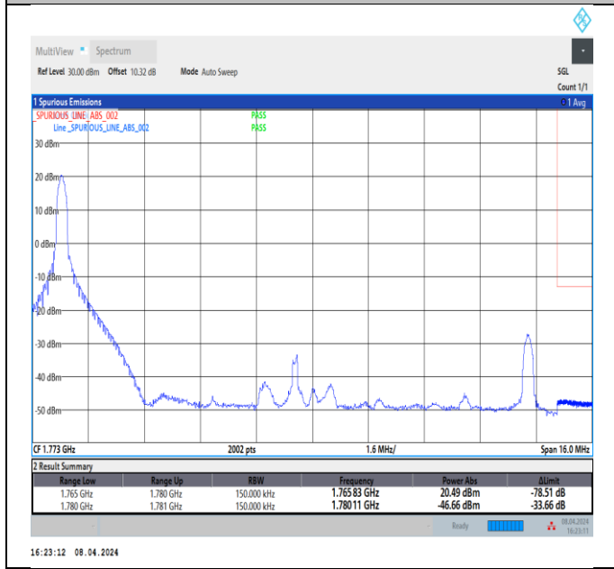
Band66_15MHz_64QAM_132597_1RB#0
