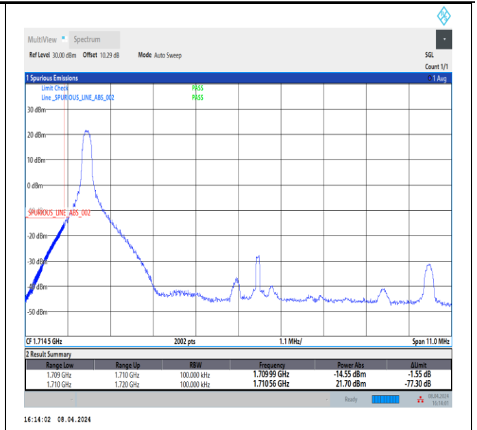
Band66_10MHz_QPSK_132022_1RB#0
