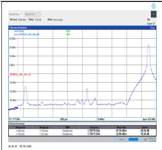
Band66_15MHz_QPSK_132047_1RB#74
