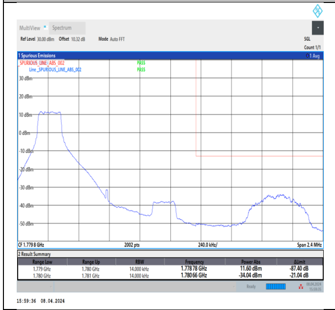
Band66_1.4MHz_64QAM_132665_1RB#0
