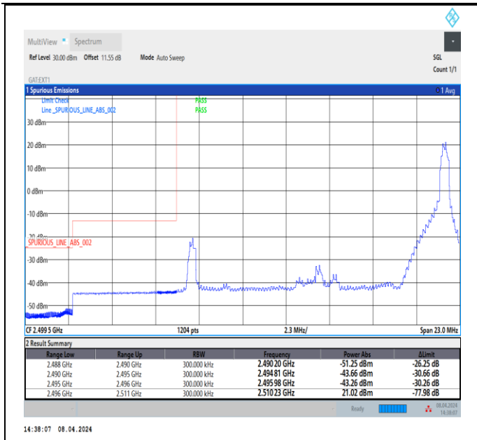
Band41_15MHz_64QAM_39725_1RB#74
