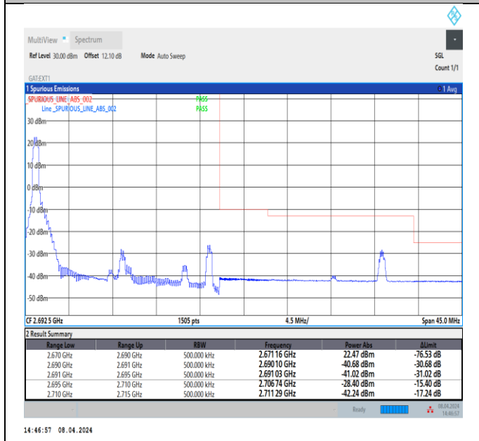
Band41_20MHz_16QAM_41490_1RB#0
