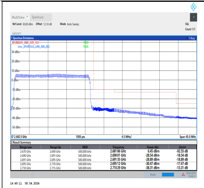
Band41_20MHz_16QAM_41490_100RB#0
