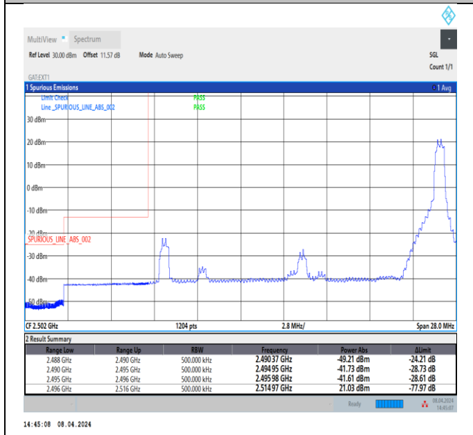
Band41_20MHz_64QAM_39750_1RB#99
