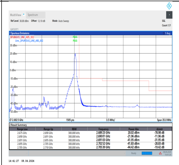
Band41_15MHz_64QAM_41515_1RB#74
