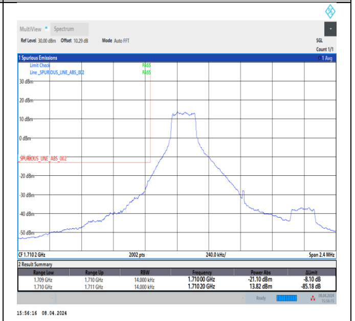
Band66_1.4MHz_QPSK_131979_1RB#0
