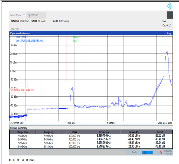
Band41_15MHz_QPSK_39725_1RB#74
