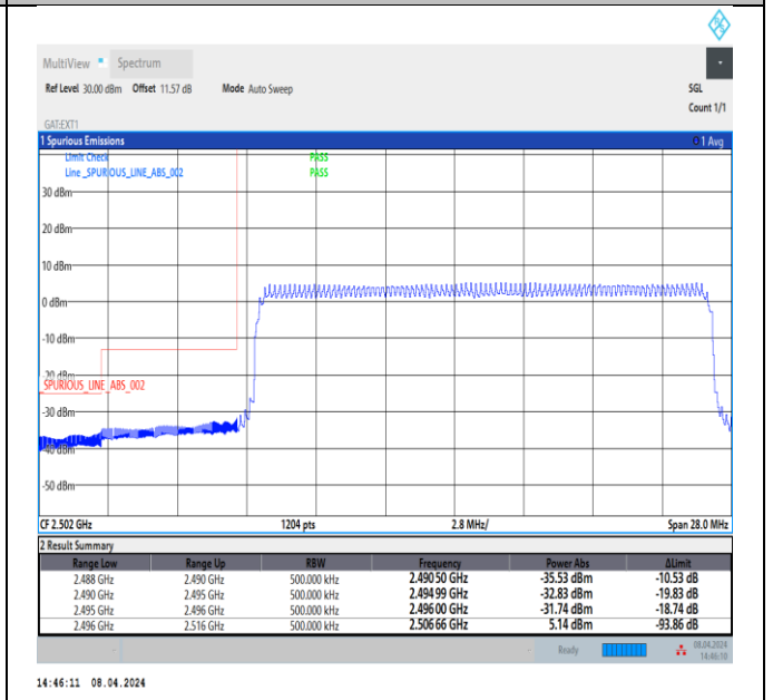
Band41_20MHz_64QAM_39750_100RB#0
