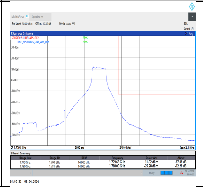
Band66_1.4MHz_64QAM_132665_1RB#5
