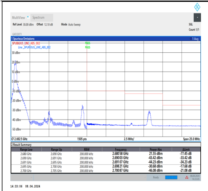
Band41_10MHz_64QAM_41540_1RB#0
