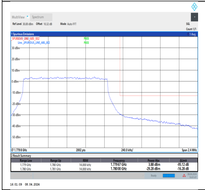
Band66_1.4MHz_16QAM_132665_6RB#0
