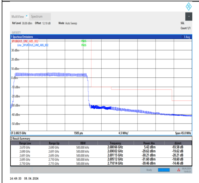
Band41_20MHz_64QAM_41490_100RB#0
