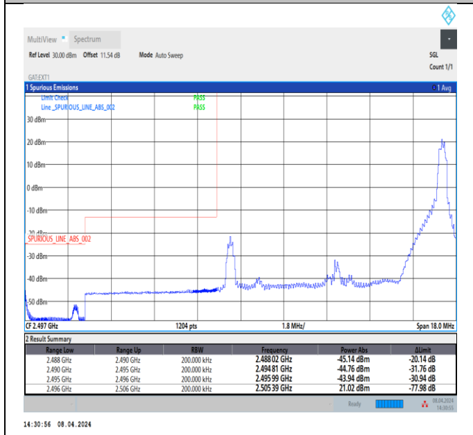
Band41_10MHz_64QAM_39700_1RB#49
