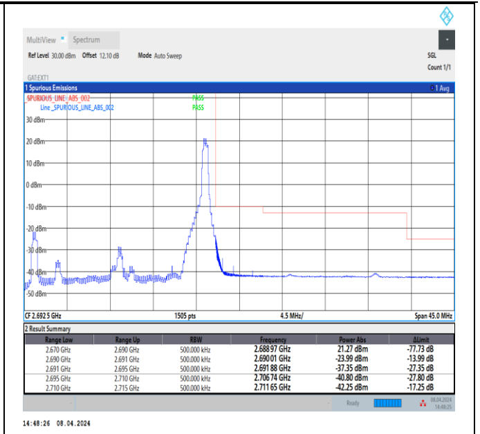
Band41_20MHz_64QAM_41490_1RB#99
