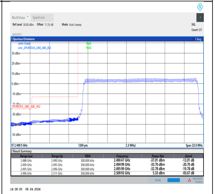
Band41_15MHz_16QAM_39725_75RB#0
