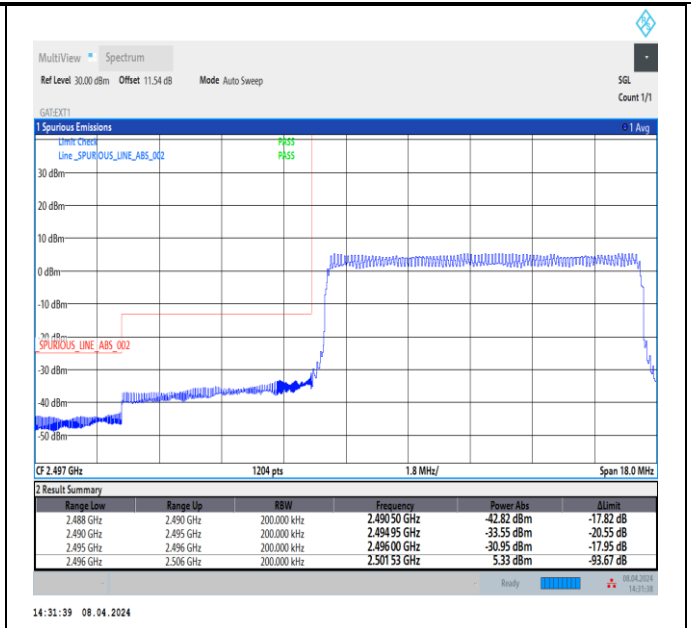
Band41_10MHz_16QAM_39700_50RB#0
