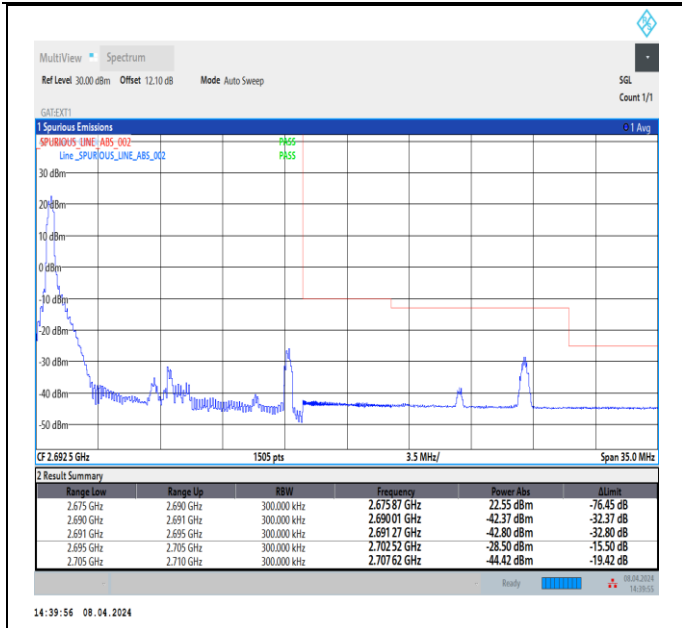
Band41_15MHz_16QAM_41515_1RB#0
