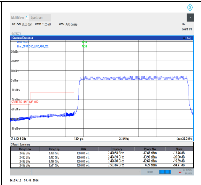
Band41_15MHz_64QAM_39725_75RB#0
