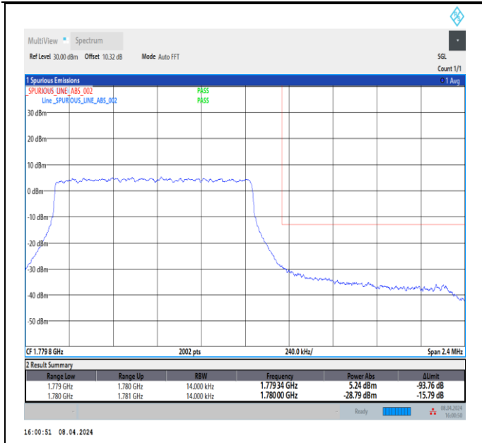
Band66_1.4MHz_QPSK_132665_6RB#0
