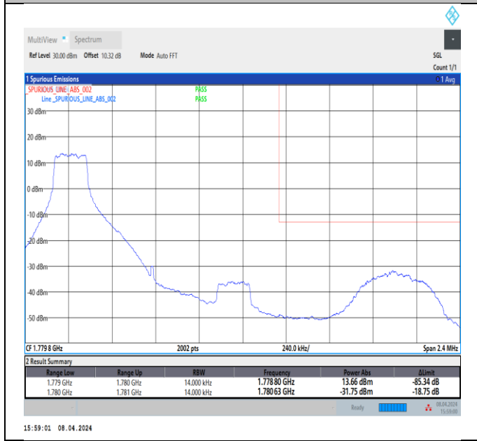
Band66_1.4MHz_QPSK_132665_1RB#0
