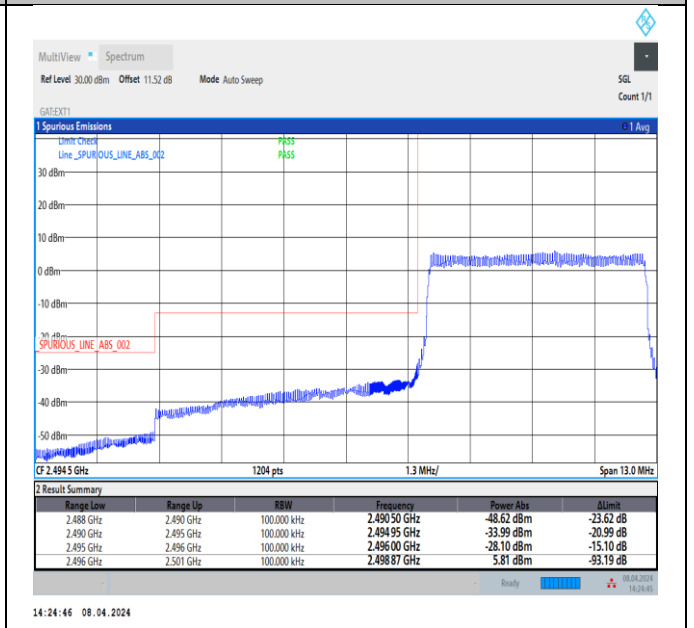
Band41_5MHz_16QAM_39675_25RB#0
