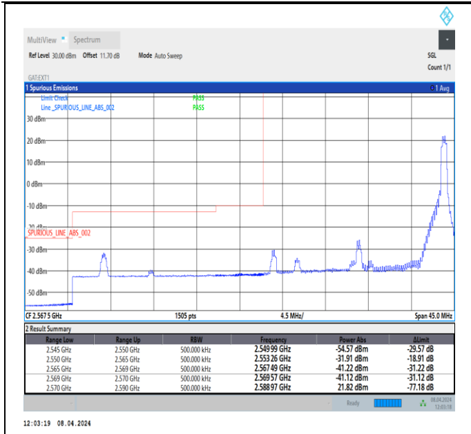
Band38_20MHz_16QAM_37850_1RB#99
