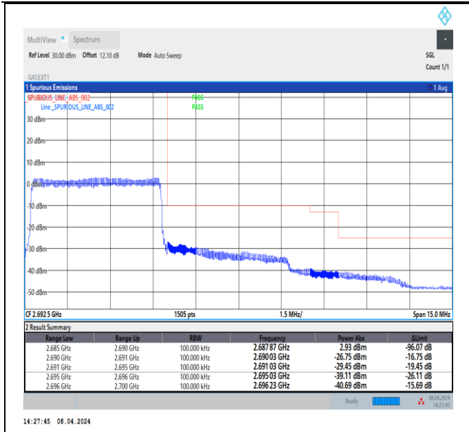
Band41_5MHz_QPSK_41565_25RB#0
