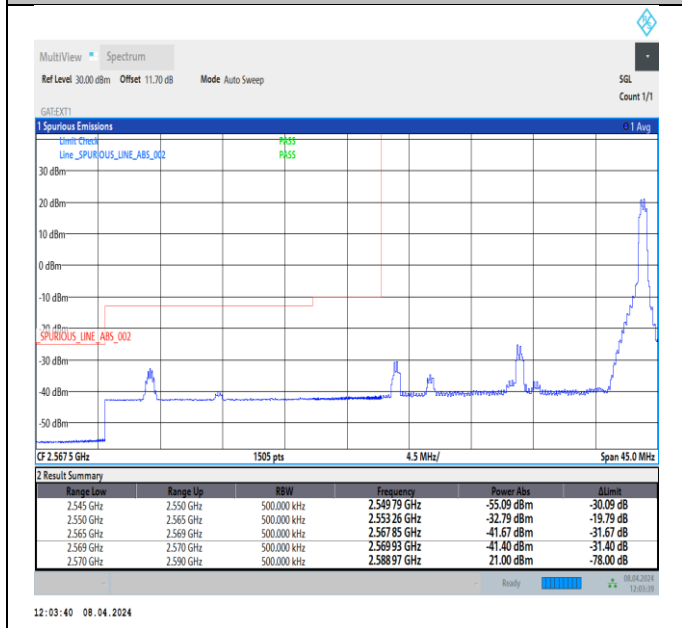
Band38_20MHz_64QAM_37850_1RB#99
