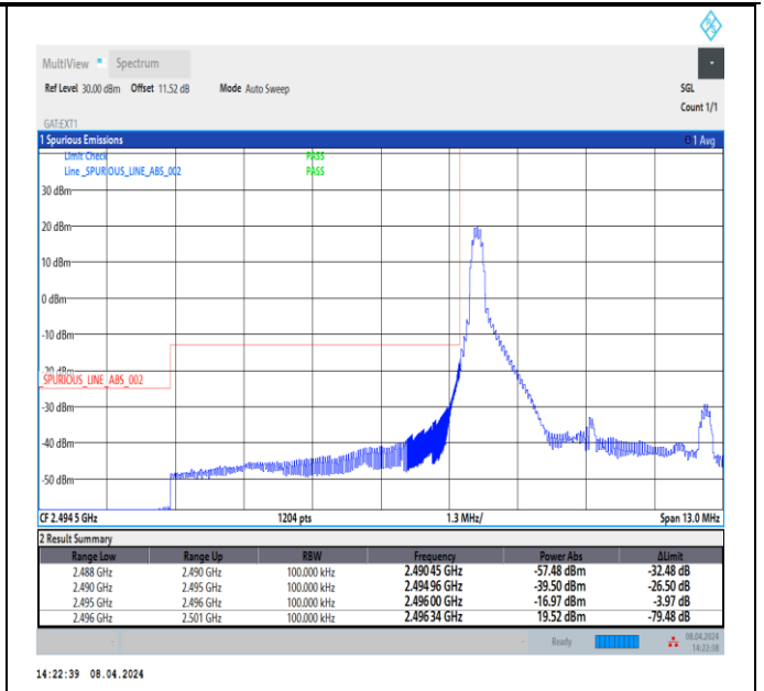
Band41_5MHz_16QAM_39675_1RB#0
