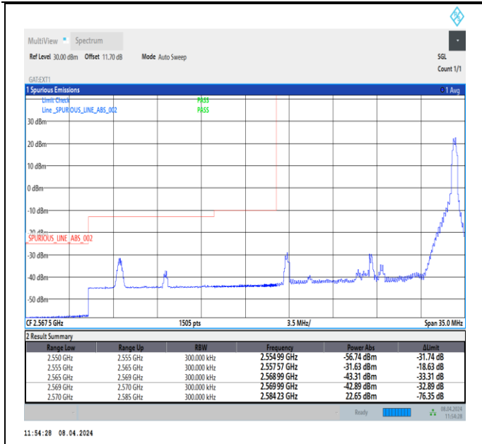
Band38_15MHz_QPSK_37825_1RB#74
