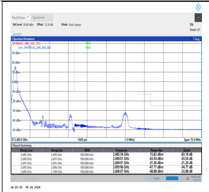
Band41_5MHz_16QAM_41565_1RB#0
