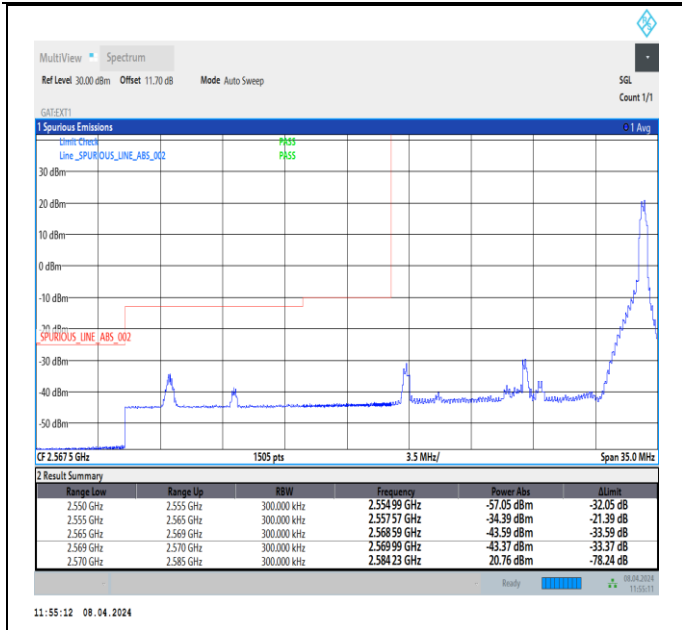
Band38_15MHz_64QAM_37825_1RB#74
