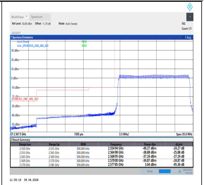
Band38_15MHz_64QAM_37825_75RB#0
