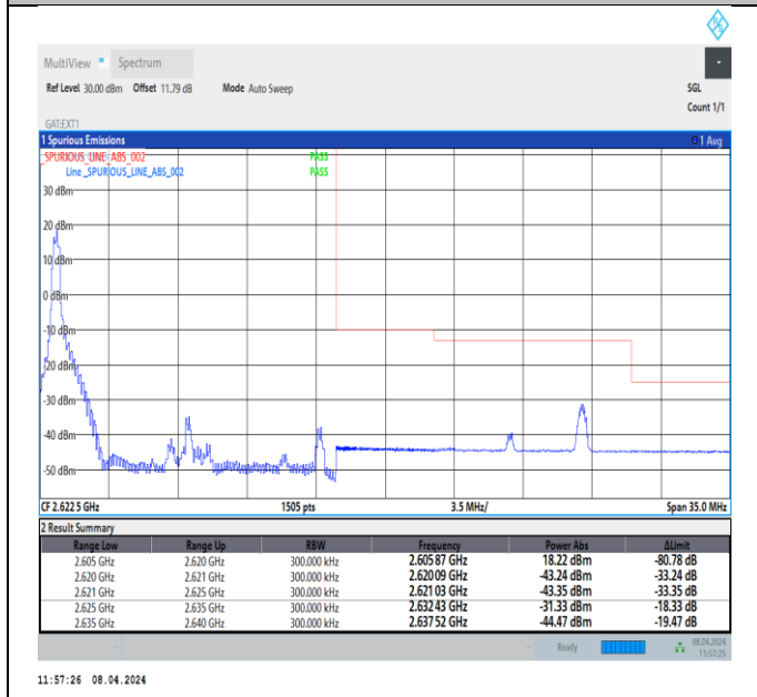
Band38_15MHz_64QAM_38175_1RB#0
