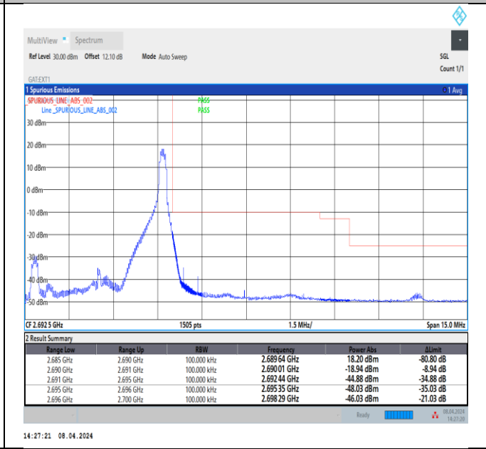
Band41_5MHz_64QAM_41565_1RB#24
