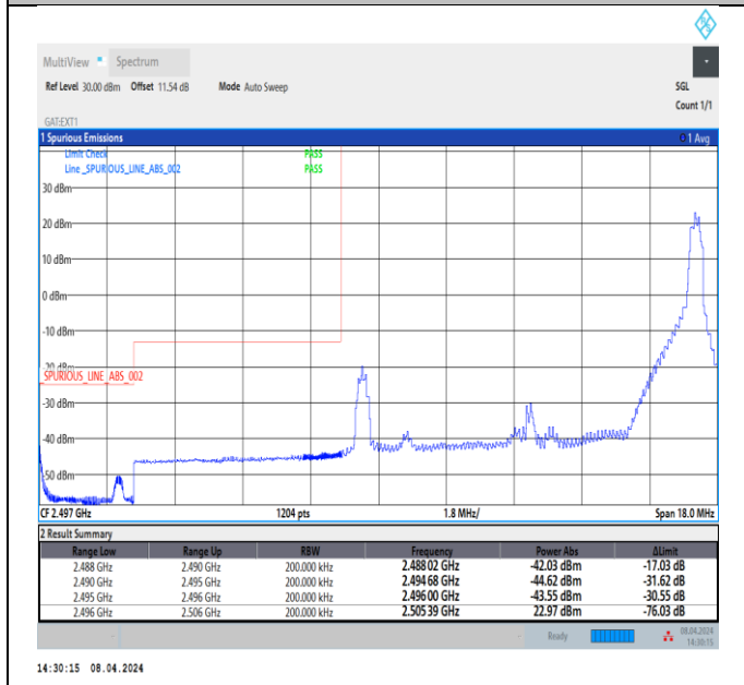
Band41_10MHz_QPSK_39700_1RB#49
