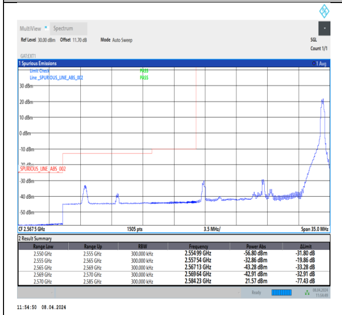
Band38_15MHz_16QAM_37825_1RB#74
