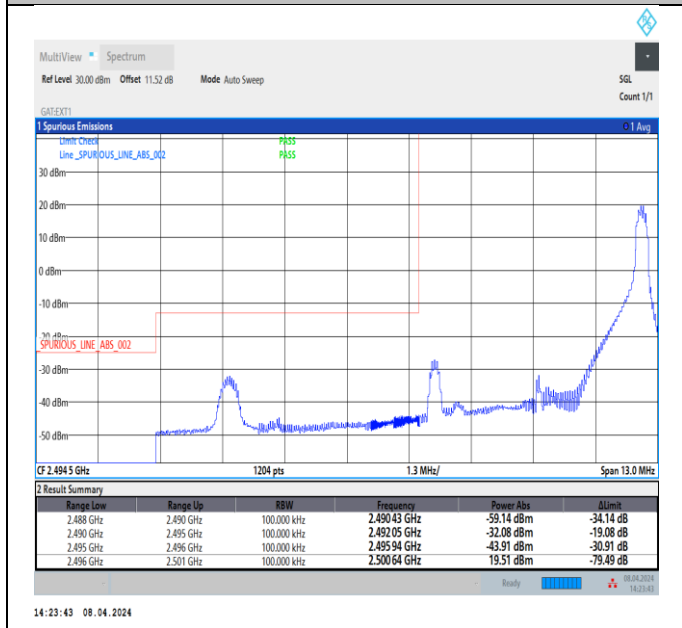
Band41_5MHz_16QAM_39675_1RB#24
