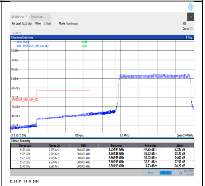
Band38_15MHz_16QAM_37825_75RB#0
