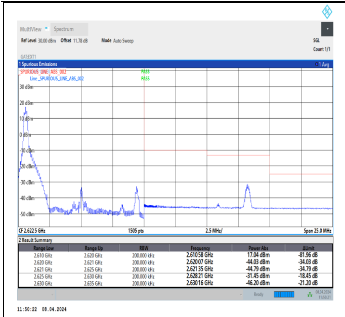
Band38_10MHz_64QAM_38200_1RB#0
