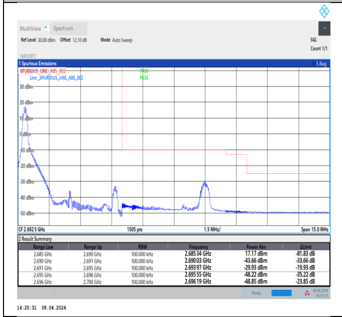
Band41_5MHz_QPSK_41565_1RB#0
