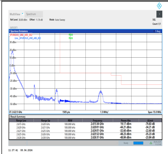
Band38_5MHz_16QAM_38225_1RB#0
