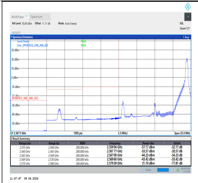
Band38_10MHz_16QAM_37800_1RB#49
