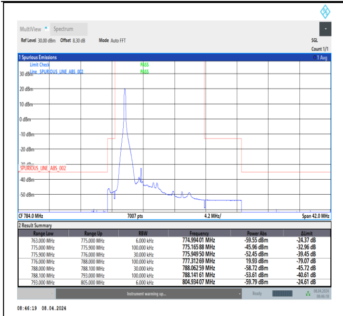
Band13_5MHz_64QAM_23205_1RB#0
