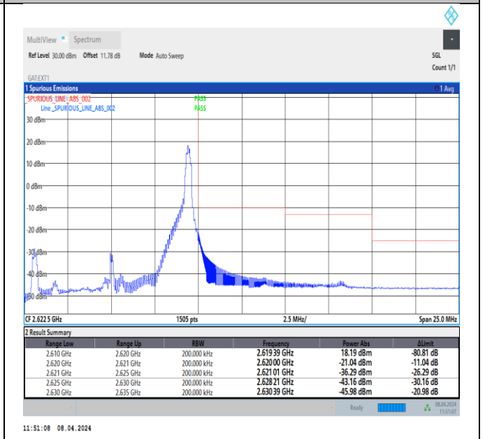
Band38_10MHz_16QAM_38200_1RB#49
