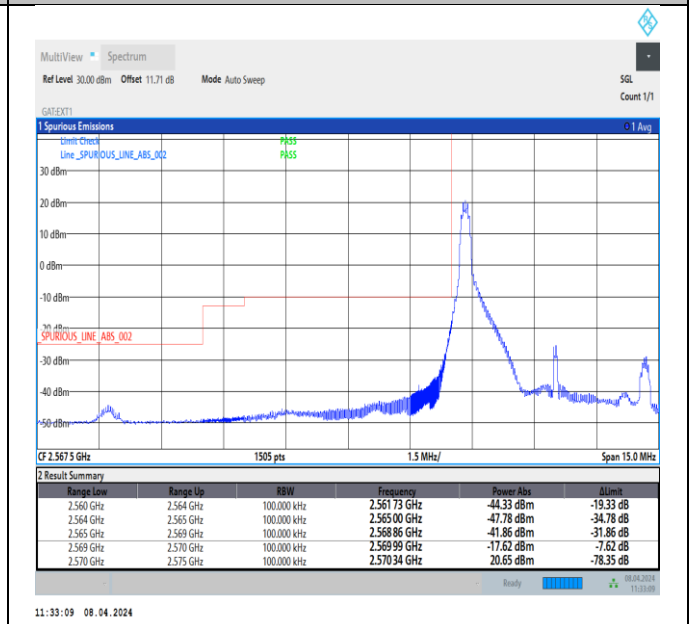
Band38_5MHz_QPSK_3775_1RB#0
