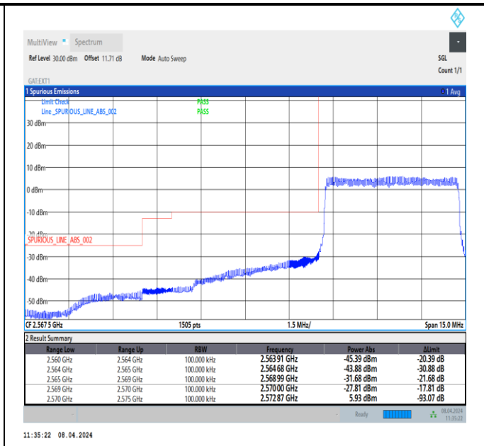
Band38_5MHz_QPSK_37775_25RB#0
