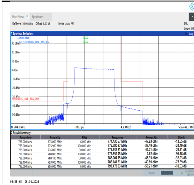
Band13_10MHz_64QAM_23230_50RB#0
