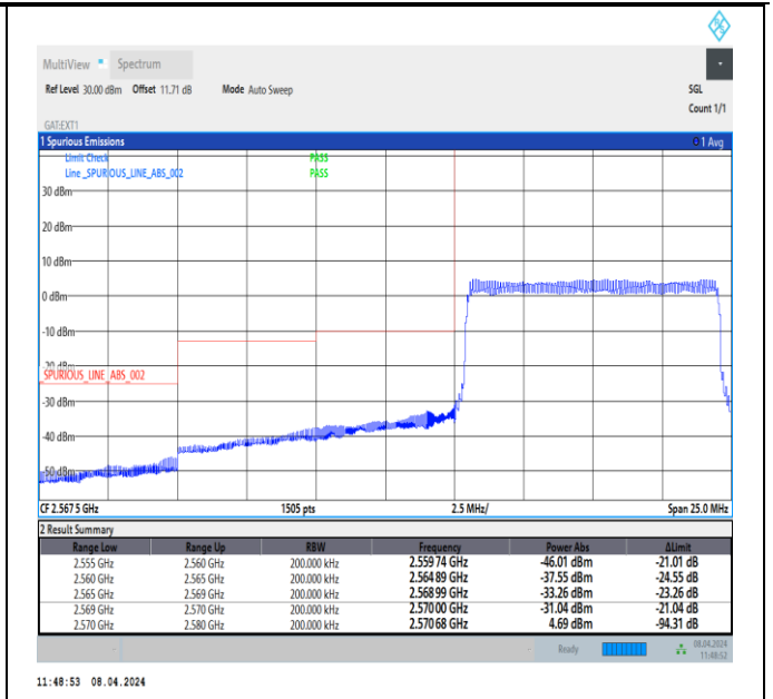
Band38_10MHz_16QAM_37800_50RB#0
