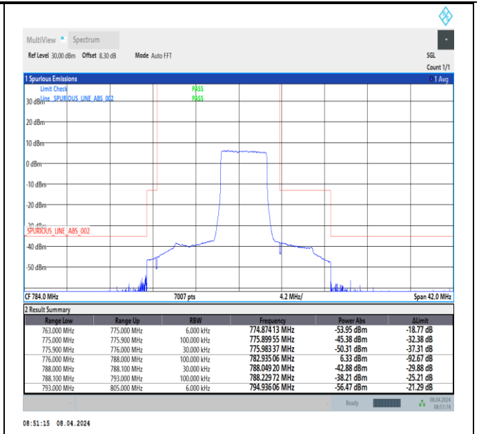
Band13_5MHz_QPSK_23255_25RB#0
