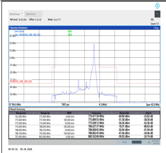
Band13_5MHz_64QAM_23255_1RB#24
