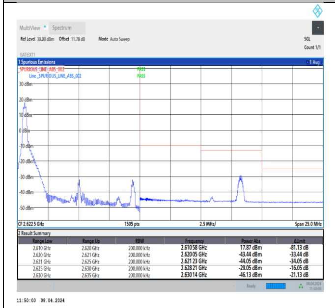
Band38_10MHz_16QAM_38200_1RB#0
