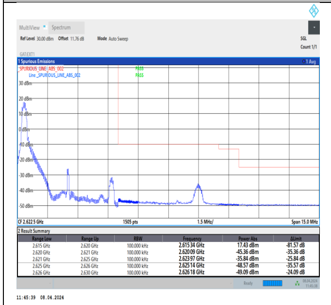
Band38_5MHz_64QAM_38225_1RB#0
