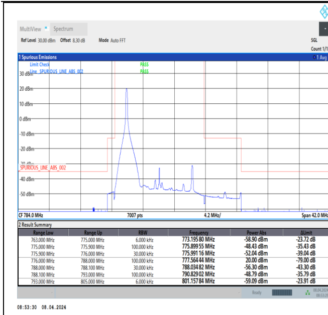
Band13_10MHz_64QAM_23230_1RB#0
