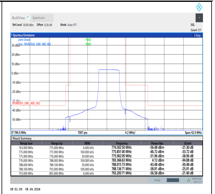
Band13_5MHz_64QAM_23255_25RB#0
