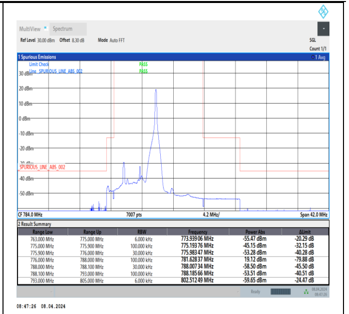
Band13_5MHz_64QAM_23205_1RB#24
