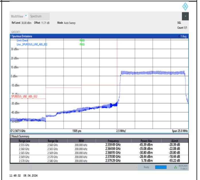
Band38_10MHz_QPSK_37800_50RB#0
