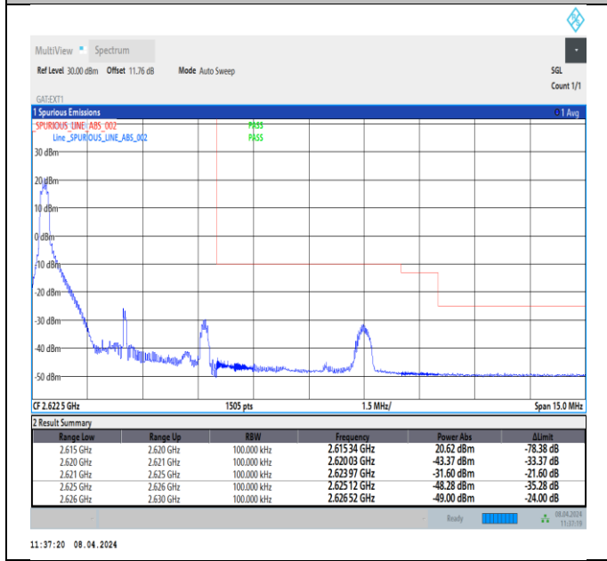
Band38_5MHz_QPSK_38225_1RB#0
