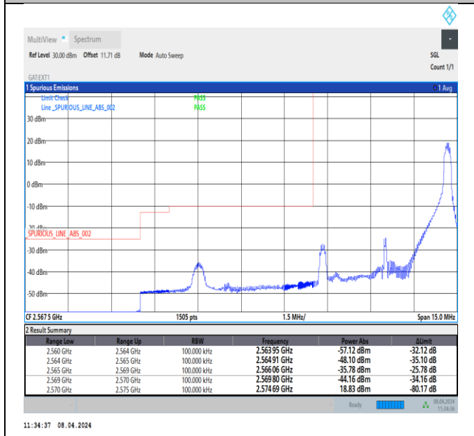
Band38_5MHz_16QAM_37775_1RB#24
