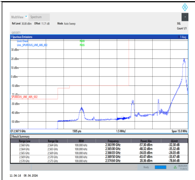
Band38_5MHz_QPSK_37775_1RB#24
