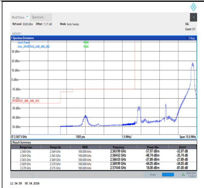
Band38_5MHz_64QAM_37775_1RB#24
