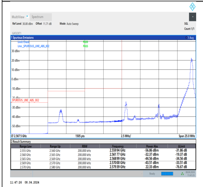
Band38_10MHz_QPSK_37800_1RB#49
