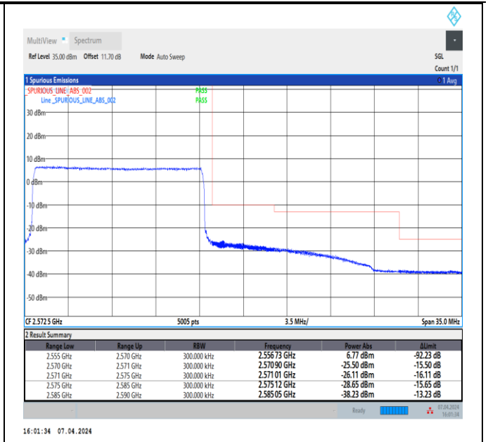
Band7_15MHz_QPSK_21375_75RB#0
