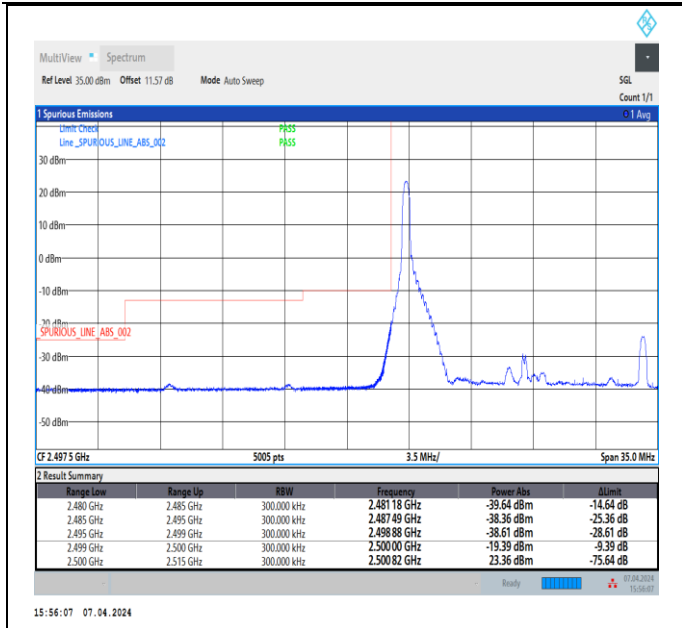
Band7_15MHz_QPSK_20825_1RB#0
