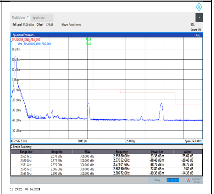
Band7_15MHz_QPSK_21375_1RB#0
