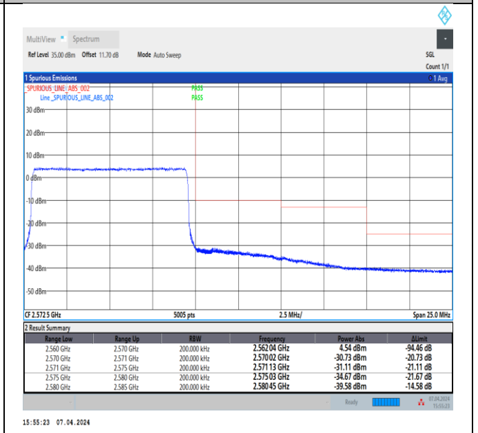
Band7_10MHz_64QAM_21400_50RB#0
