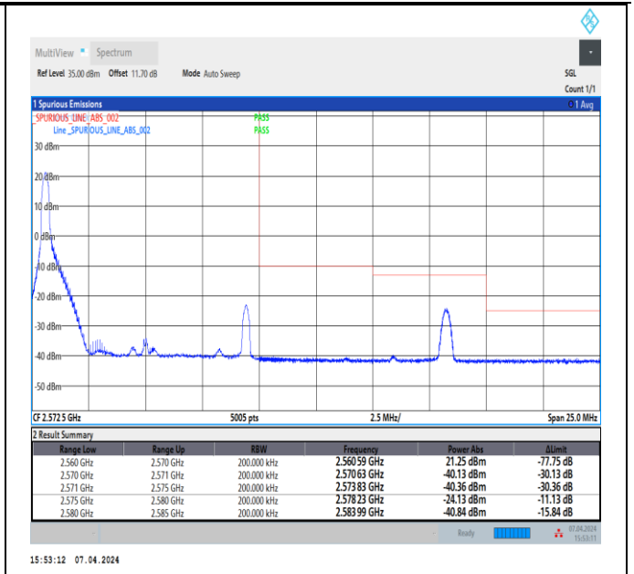
Band7_10MHz_64QAM_21400_1RB#0
