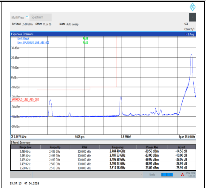
Band7_15MHz_QPSK_20825_1RB#74
