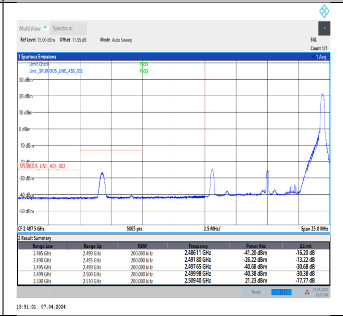
Band7_10MHz_64QAM_20800_1RB#49
