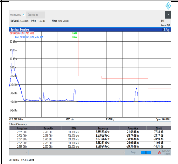
Band7_15MHz_64QAM_21375_1RB#0
