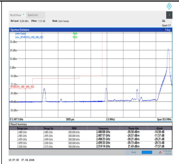
Band7_15MHz_64QAM_20825_1RB#74
