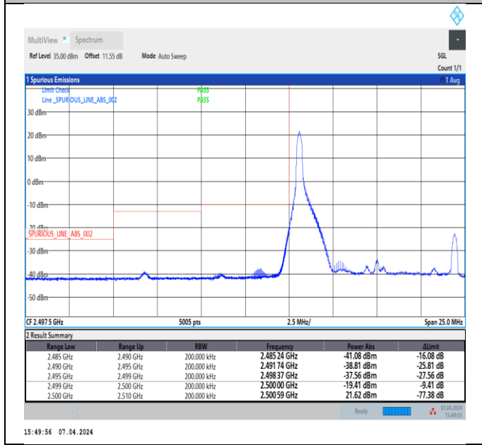
Band7_10MHz_64QAM_20800_1RB#0
