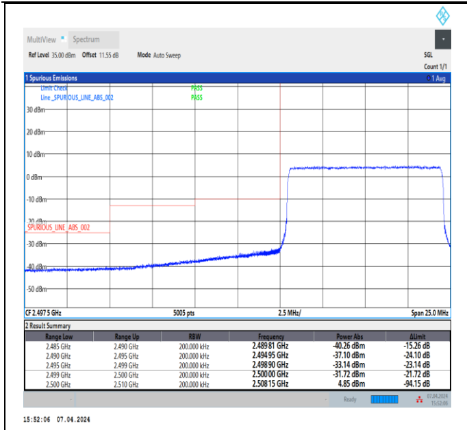
Band7_10MHz_64QAM_20800_50RB#0
