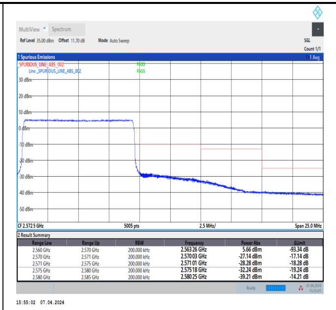
Band7_10MHz_16QAM_21400_50RB#0
