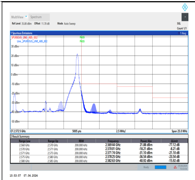
Band7_10MHz_16QAM_21400_1RB#49
