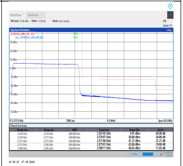
Band7_20MHz_64QAM_21350_100RB#0
