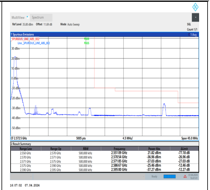
Band7_20MHz_64QAM_21350_1RB#0
