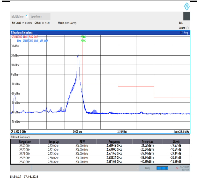
Band7_10MHz_64QAM_21400_1RB#49
