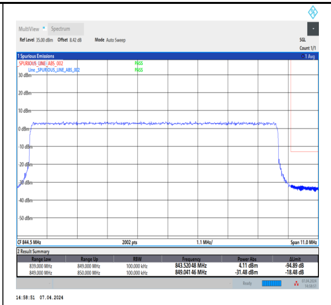
Band5_10MHz_16QAM_20600_50RB#0
