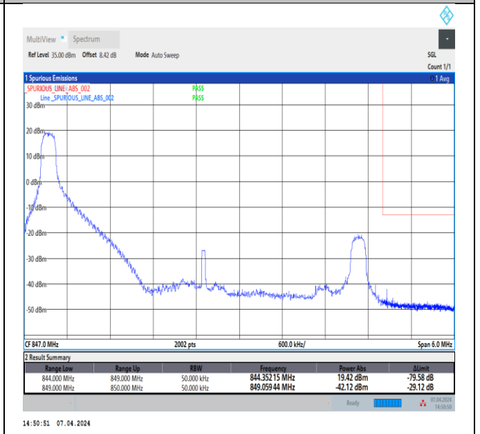
Band5_5MHz_QPSK_20625_1RB#0
