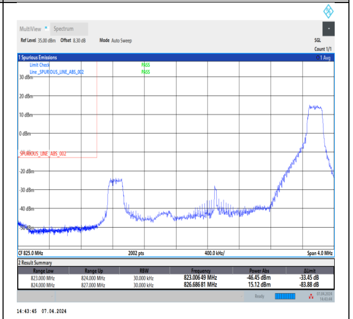
Band5_3MHz_64QAM_20415_1RB#14
