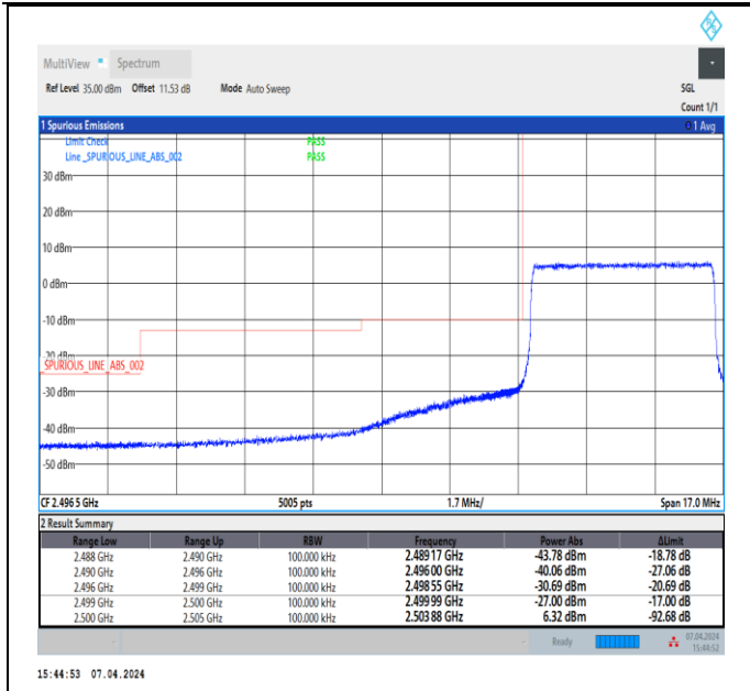
Band7_5MHz_16QAM_20775_25RB#0
