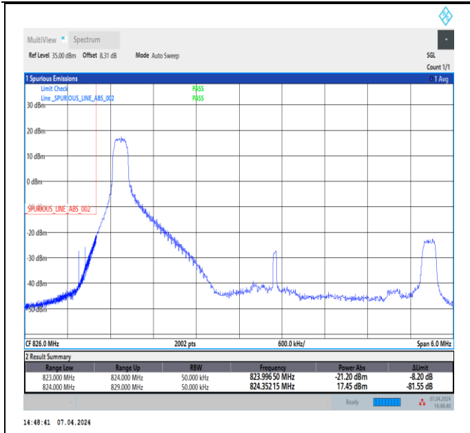
Band5_5MHz_64QAM_20425_1RB#0
