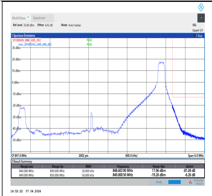
Band5_5MHz_64QAM_20625_1RB#24
