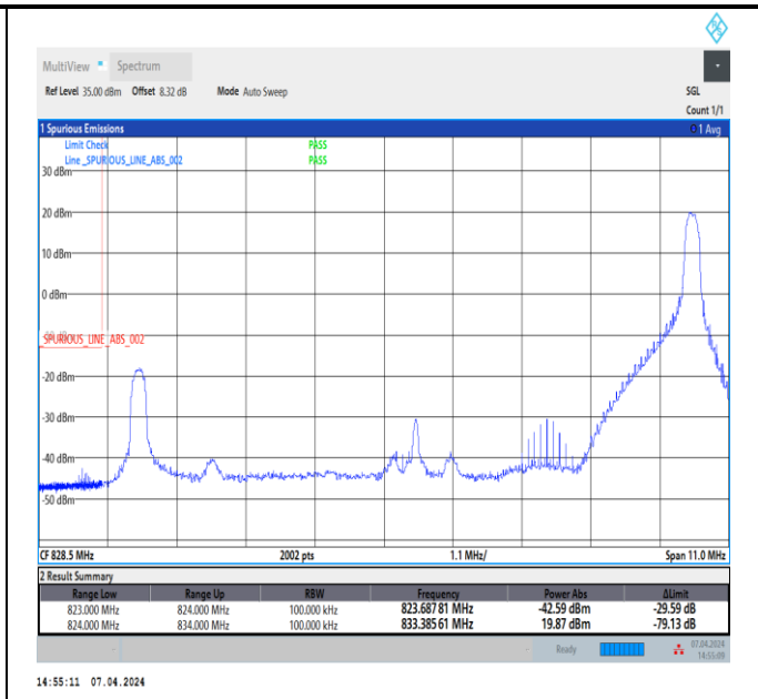
Band5_10MHz_16QAM_20450_1RB#49
