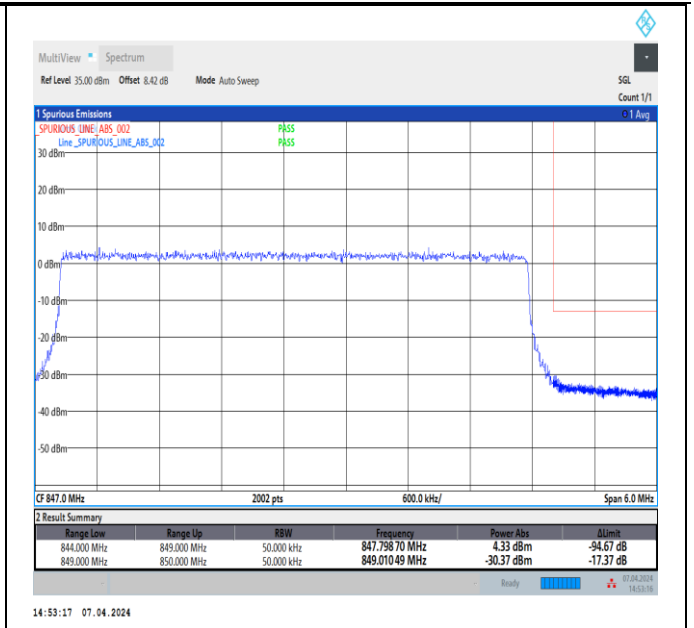
Band5_5MHz_64QAM_20625_25RB#0
