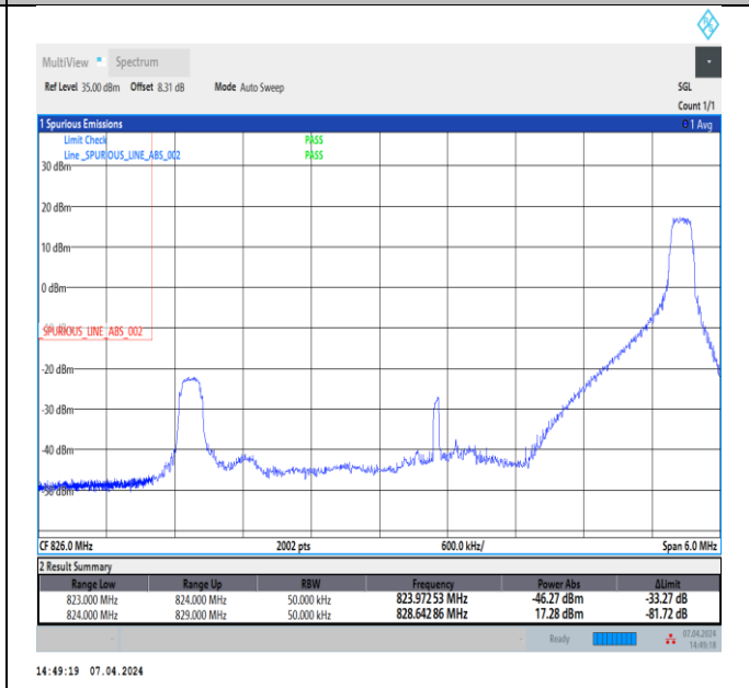
Band5_5MHz_16QAM_20425_1RB#24
