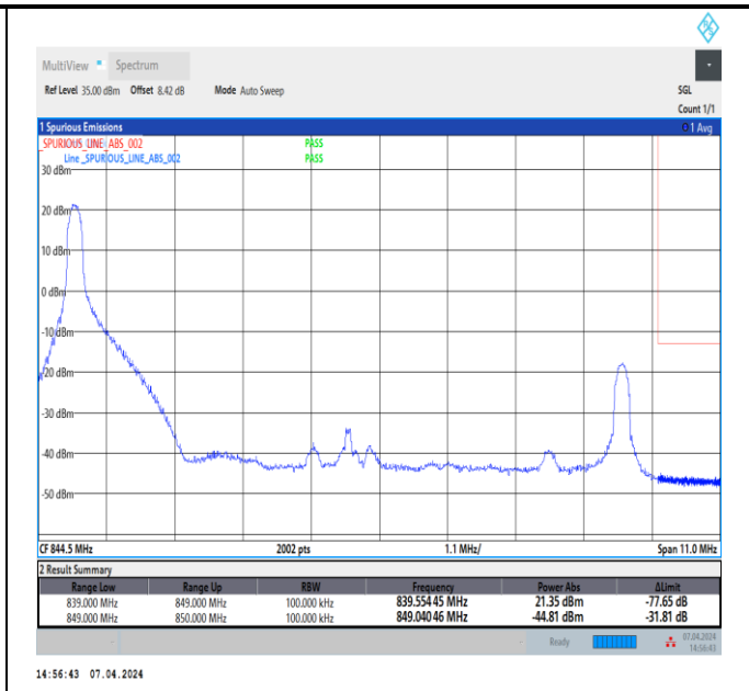
Band5_10MHz_QPSK_20600_1RB#0
