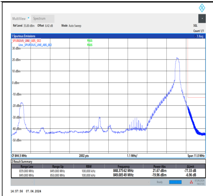
Band5_10MHz_16QAM_20600_1RB#49
