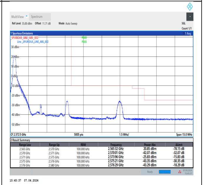
Band7_5MHz_QPSK_21425_1RB#0
