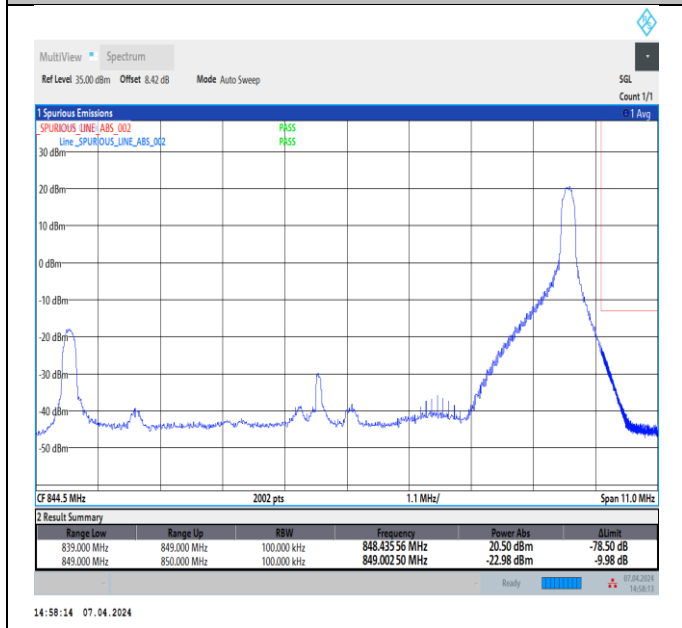
Band5_10MHz_64QAM_20600_1RB#49
