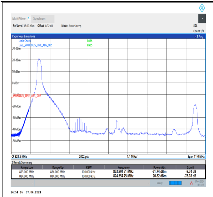
Band5_10MHz_16QAM_20450_1RB#0
