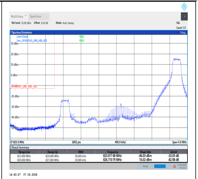
Band5_3MHz_16QAM_20415_1RB#14
