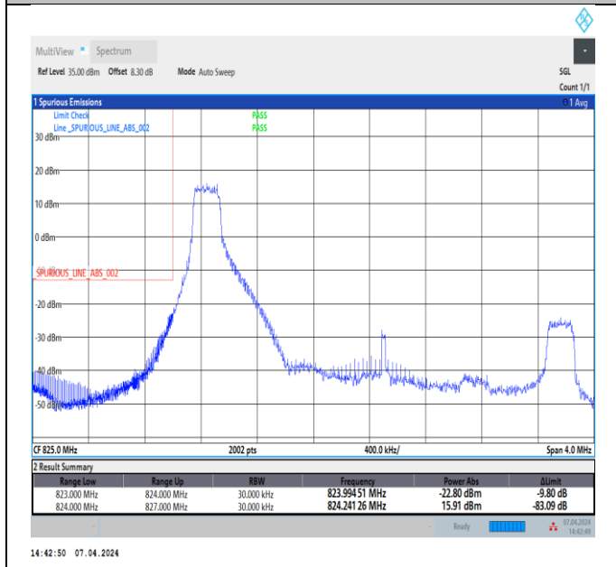
Band5_3MHz_64QAM_20415_1RB#0
