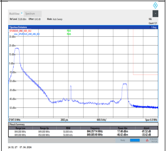
Band5_5MHz_64QAM_20625_1RB#0
