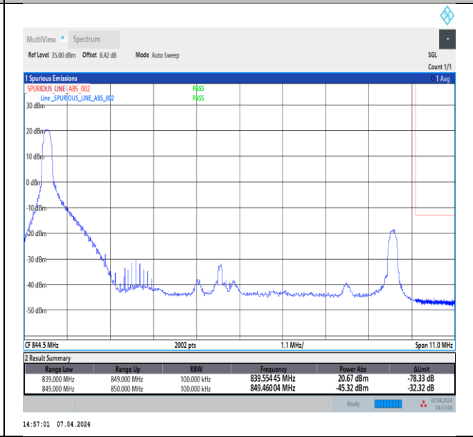
Band5_10MHz_16QAM_20600_1RB#0
