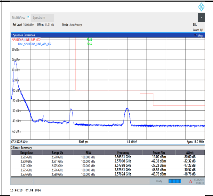
Band7_5MHz_64QAM_21425_1RB#0
