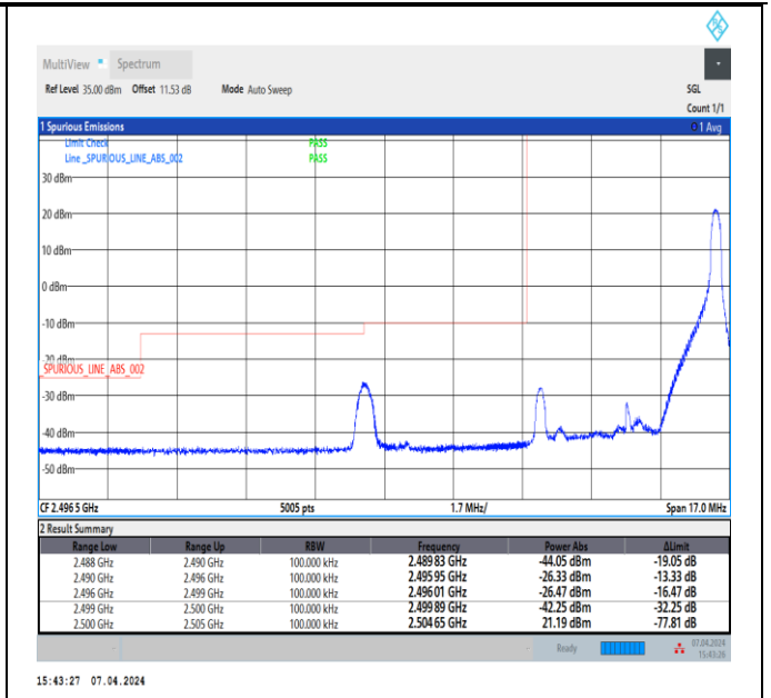
Band7_5MHz_QPSK_20775_1RB#24
