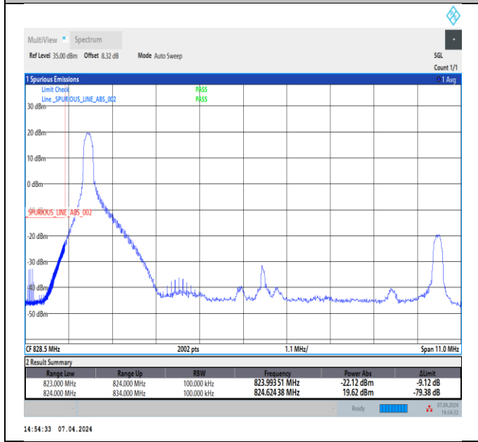
Band5_10MHz_64QAM_20450_1RB#0
