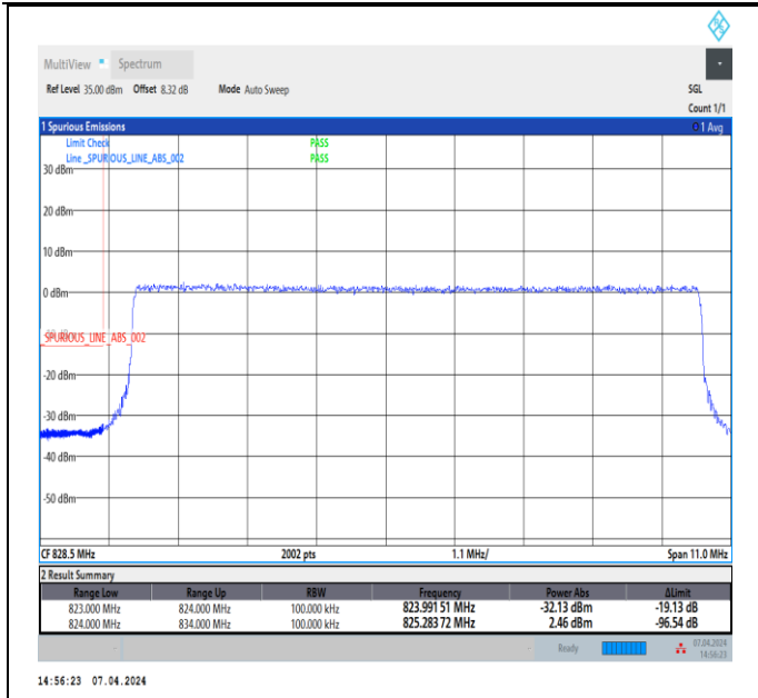
Band5_10MHz_64QAM_20450_50RB#0
