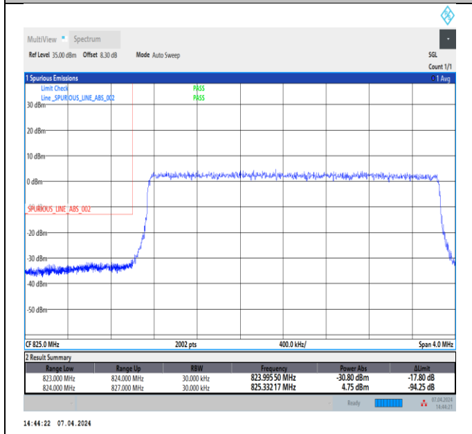
Band5_3MHz_16QAM_20415_15RB#0
