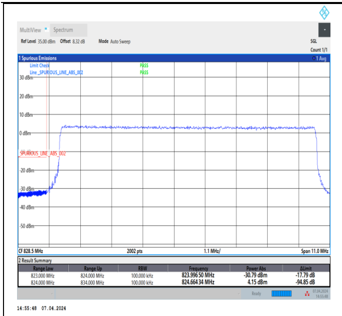
Band5_10MHz_QPSK_20450_50RB#0
