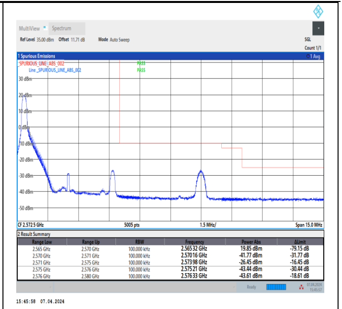
Band7_5MHz_16QAM_21425_1RB#0
