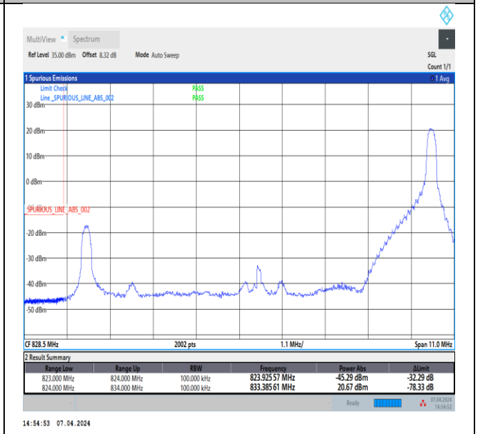
Band5_10MHz_QPSK_20450_1RB#49
