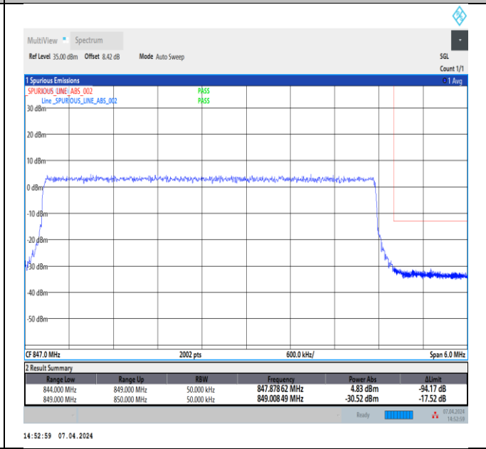
Band5_5MHz_16QAM_20625_25RB#0
