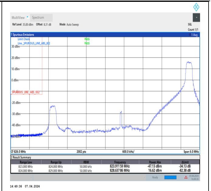
Band5_5MHz_64QAM_20425_1RB#24
