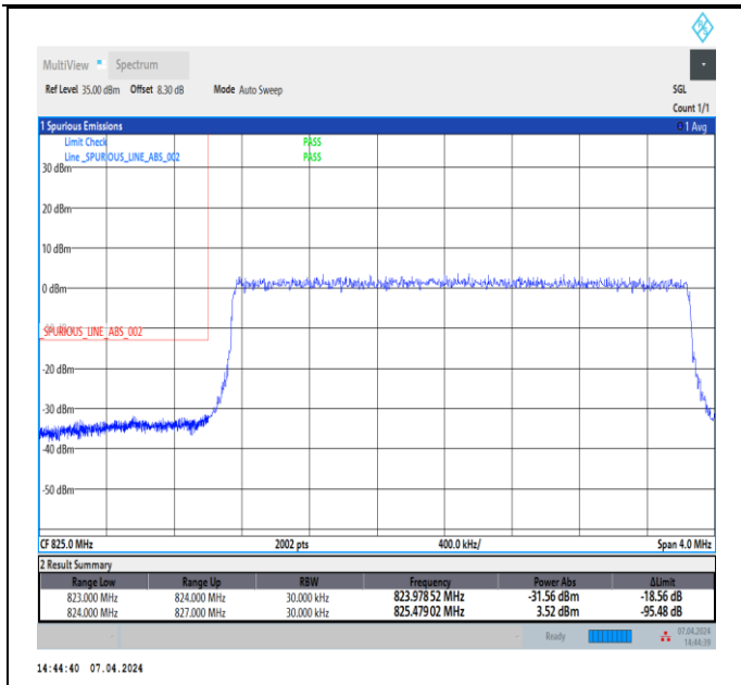
Band5_3MHz_64QAM_20415_15RB#0
