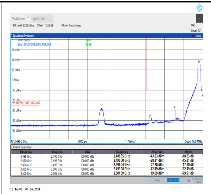
Band7_5MHz_64QAM_20775_1RB#24
