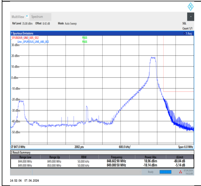
Band5_5MHz_16QAM_20625_1RB#24
