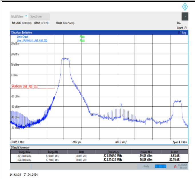
Band5_3MHz_16QAM_20415_1RB#0
