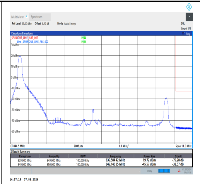
Band5_10MHz_64QAM_20600_1RB#0
