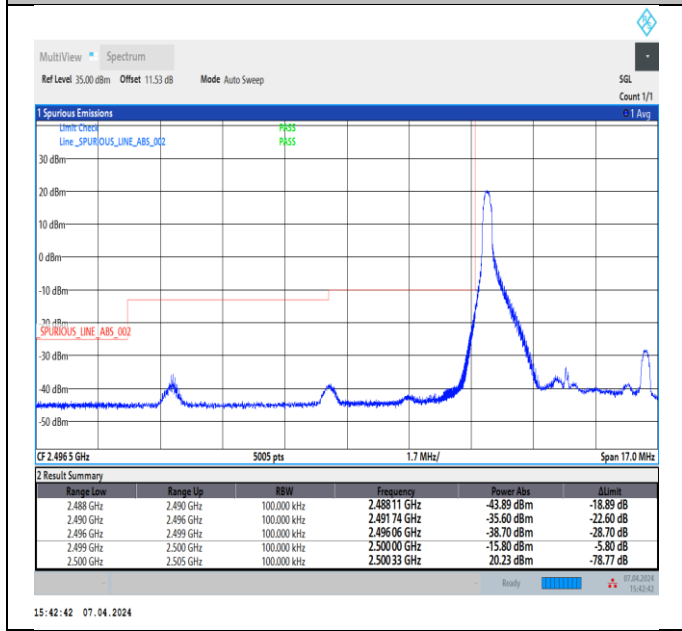
Band7_5MHz_16QAM_20775_1RB#0
