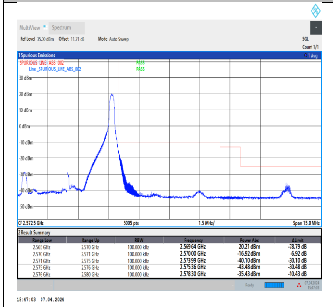
Band7_5MHz_16QAM_21425_1RB#24
