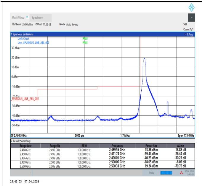
Band7_5MHz_64QAM_20775_1RB#0
