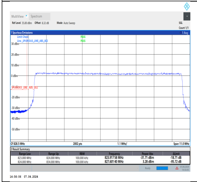
Band5_10MHz_16QAM_20450_50RB#0
