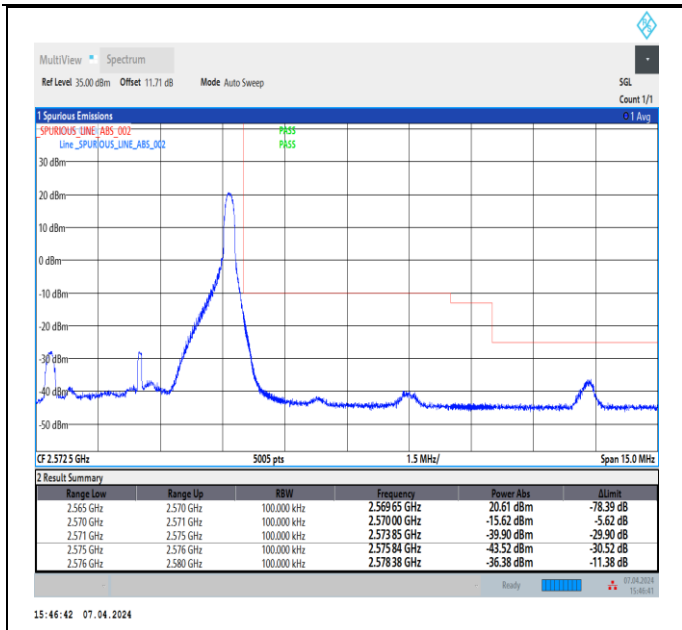
Band7_5MHz_QPSK_21425_1RB#24
