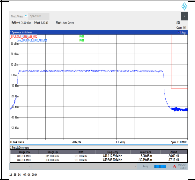
Band5_10MHz_QPSK_20600_50RB#0
