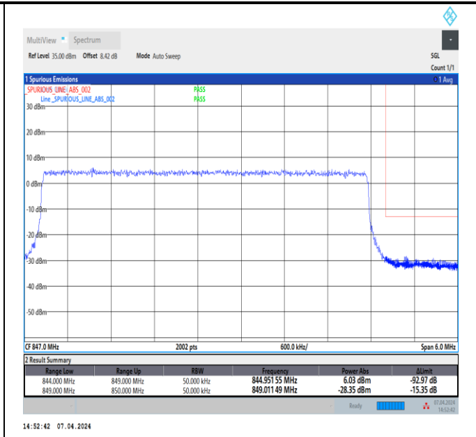
Band5_5MHz_QPSK_20625_25RB#0
