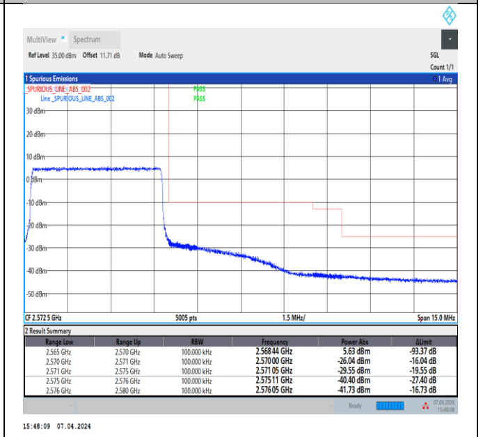
Band7_5MHz_16QAM_21425_25RB#0
