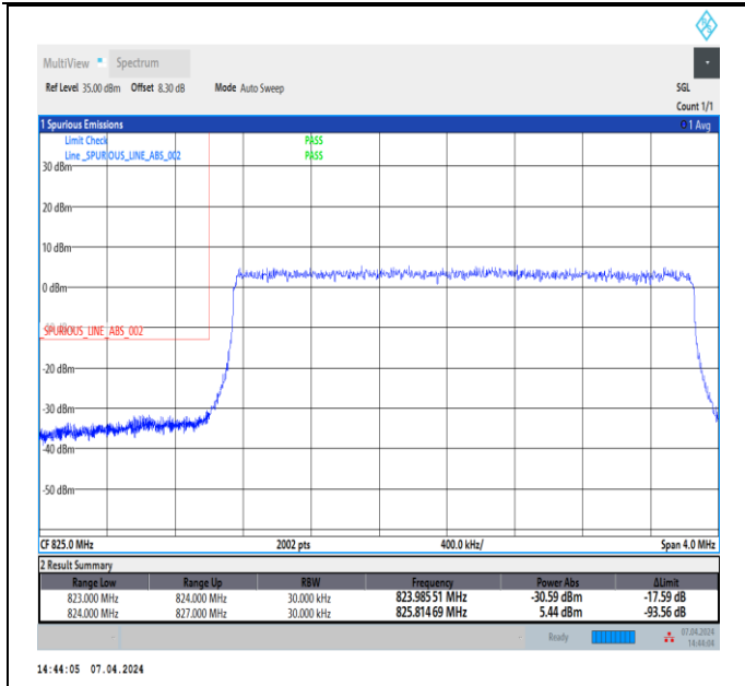
Band5_3MHz_QPSK_20415_15RB#0
