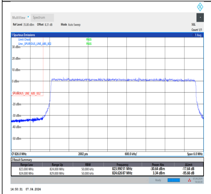
Band5_5MHz_64QAM_20425_25RB#0
