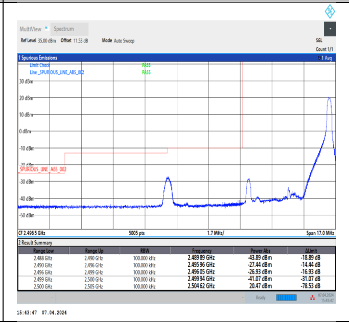
Band7_5MHz_16QAM_20775_1RB#24
