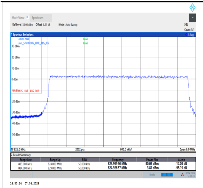
Band5_5MHz_16QAM_20425_25RB#0
