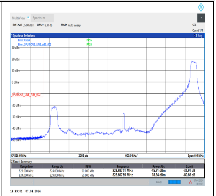
Band5_5MHz_QPSK_20425_1RB#24
