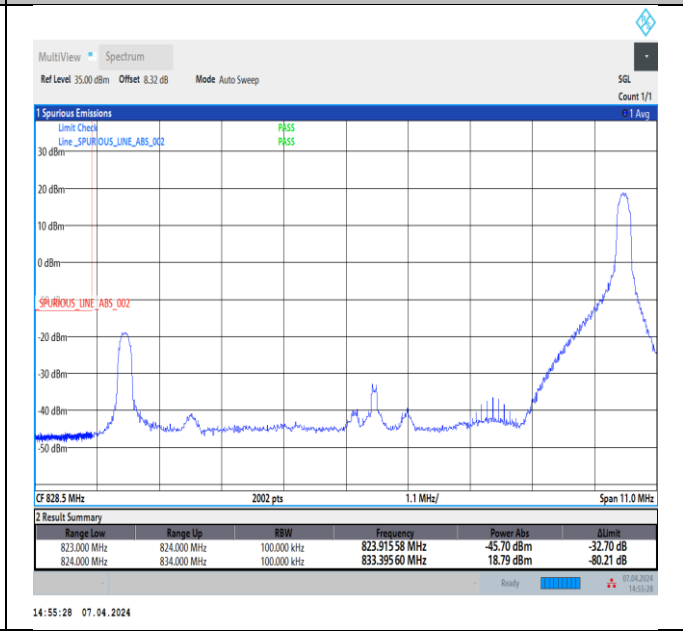
Band5_10MHz_64QAM_20450_1RB#49
