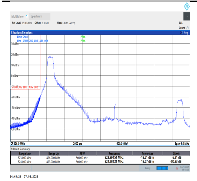
Band5_5MHz_16QAM_20425_1RB#0
