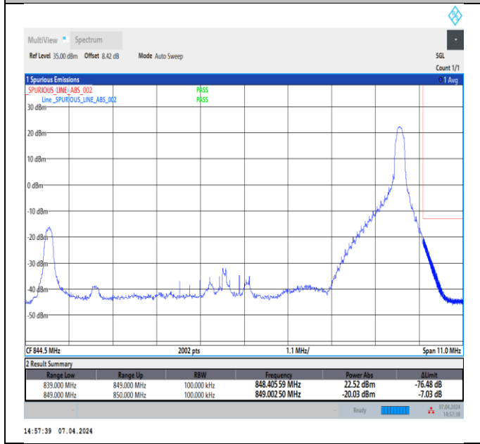
Band5_10MHz_QPSK_20600_1RB#49
