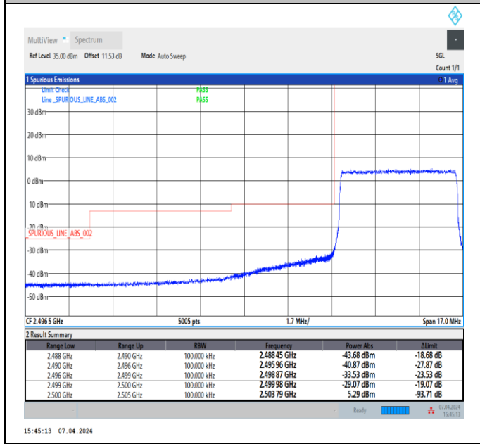
Band7_5MHz_64QAM_20775_25RB#0
