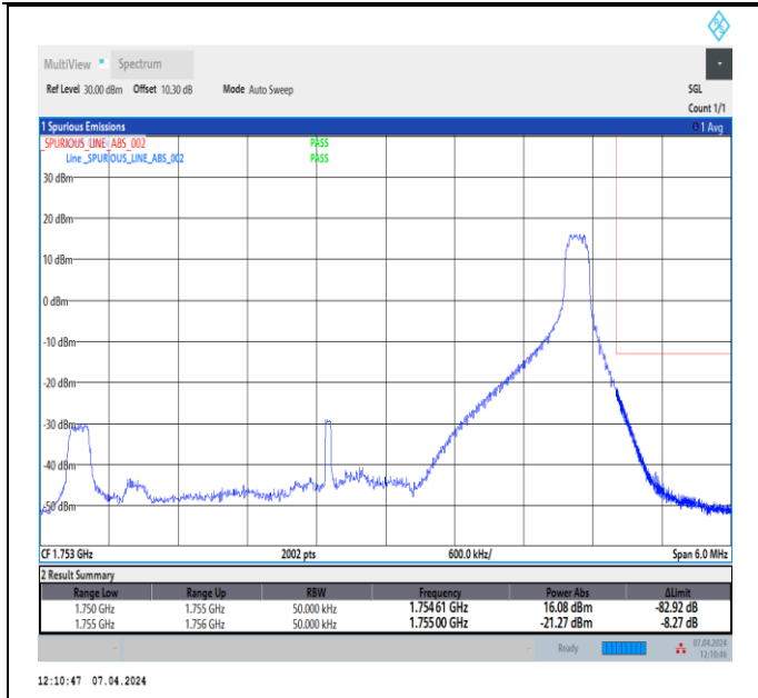
Band4_5MHz_64QAM_20375_1RB#24
