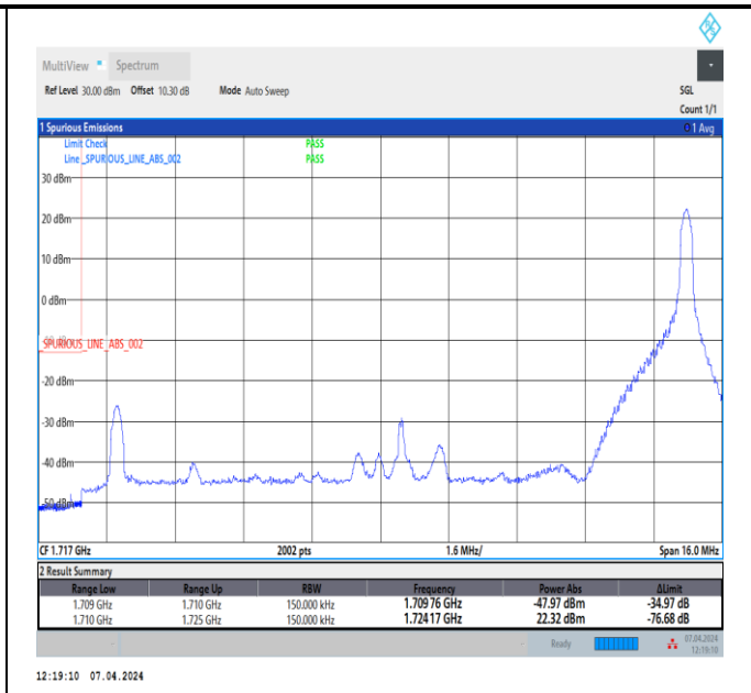
Band4_15MHz_QPSK_2025_1RB#74
