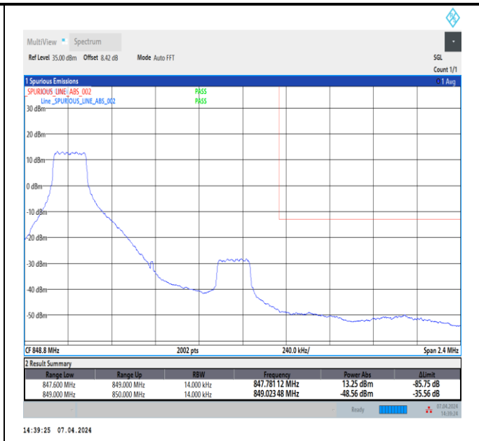
Band5_1.4MHz_16QAM_20643_1RB#0
