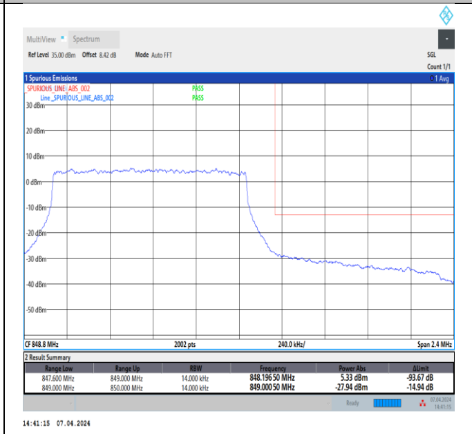
Band5_1.4MHz_16QAM_20643_6RB#0
