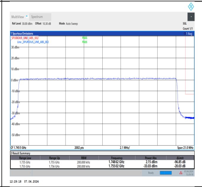
Band4_20MHz_64QAM_20300_100RB#0
