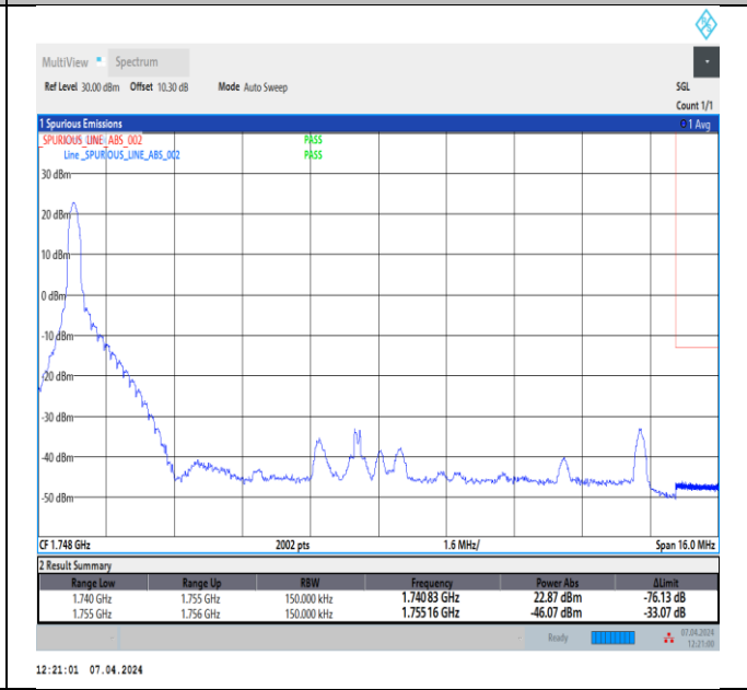
Band4_15MHz_QPSK_20325_1RB#0
