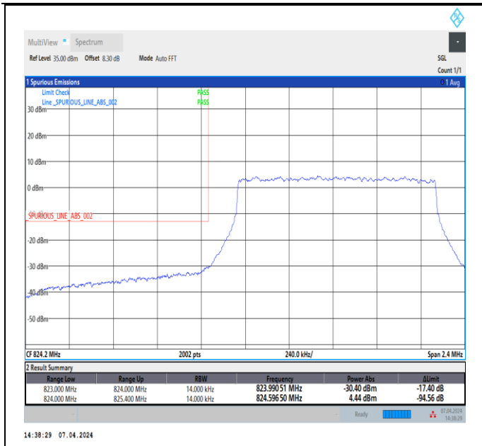
Band5_1.4MHz_16QAM_20407_6RB#0
