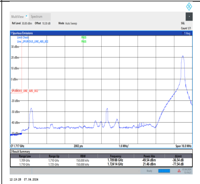
Band4_15MHz_16QAM_20025_1RB#74
