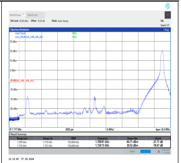
Band4_15MHz_64QAM_20025_1RB#74
