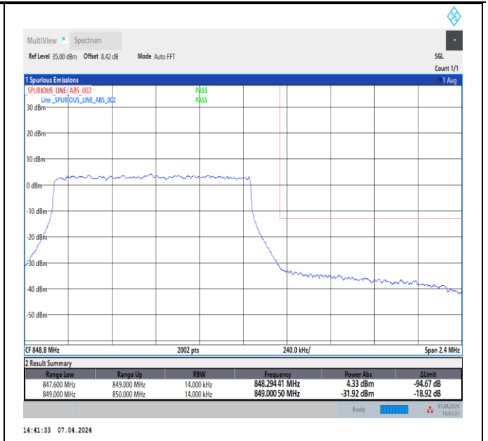
Band5_1.4MHz_64QAM_20643_6RB#0
