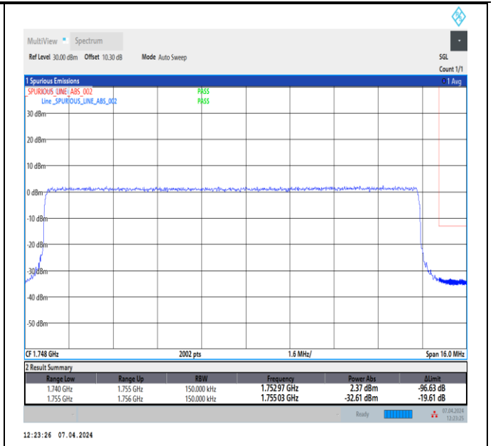
Band4_15MHz_64QAM_20325_75RB#0
