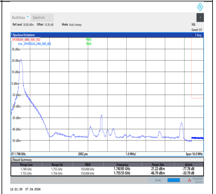
Band4_15MHz_64QAM_20325_1RB#0
