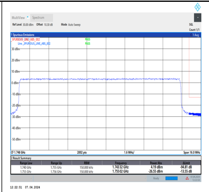
Band4_15MHz_QPSK_20325_75RB#0
