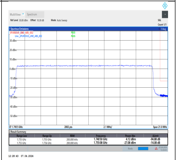
Band4_20MHz_QPSK_20300_100RB#0
