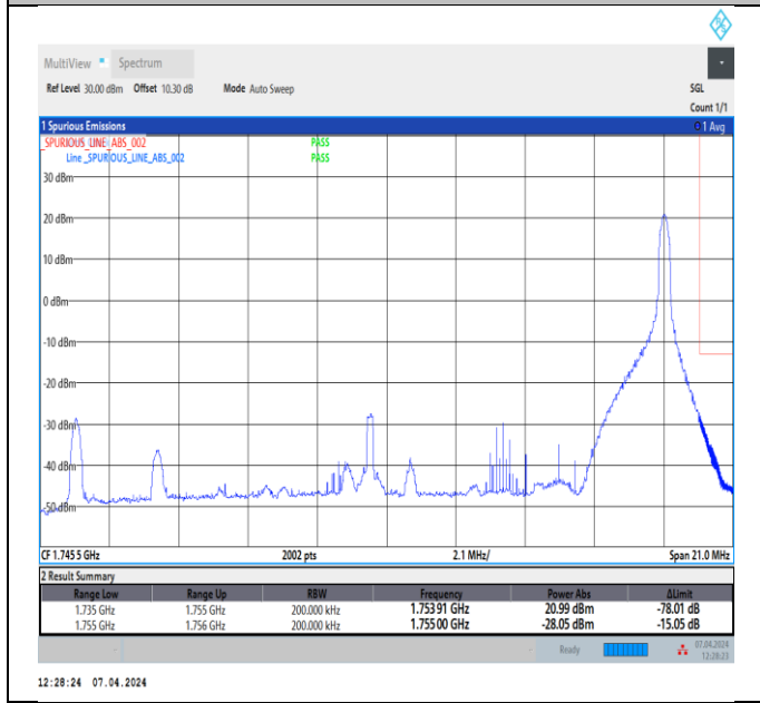
Band4_20MHz_64QAM_20300_1RB#99
