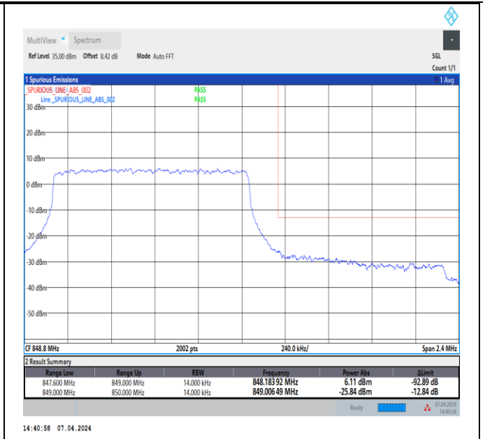
Band5_1.4MHz_QPSK_20643_6RB#0
