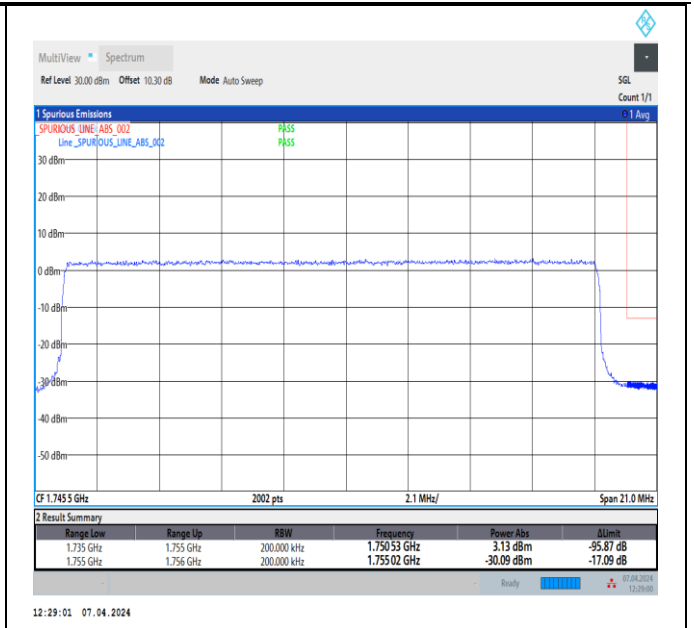
Band4_20MHz_16QAM_20300_100RB#0
