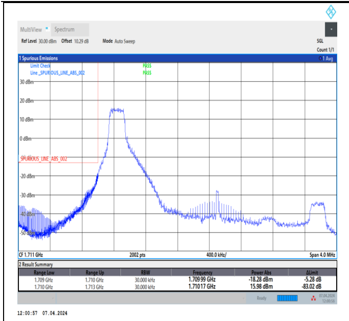
Band4_3MHz_16QAM_19965_1RB#0
