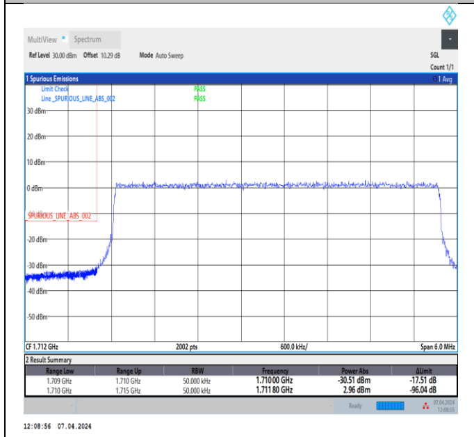
Band4_5MHz_64QAM_19975_25RB#0
