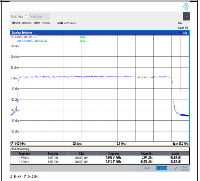
Band2_20MHz_64QAM_19100_100RB#0
