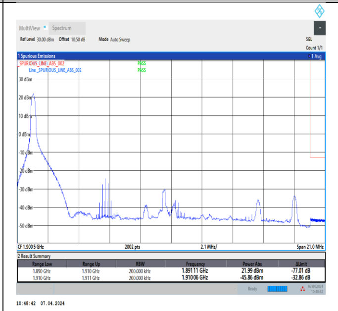
Band2_20MHz_16QAM_19100_1RB#0
