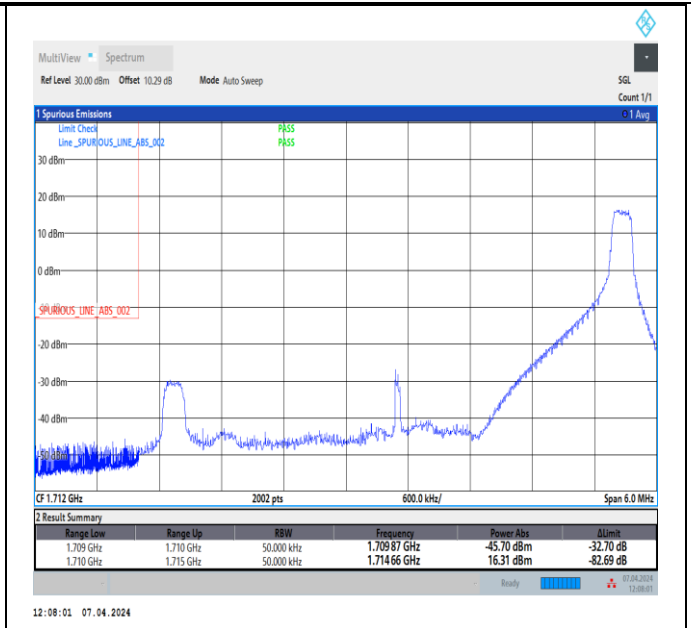
Band4_5MHz_64QAM_19975_1RB#24
