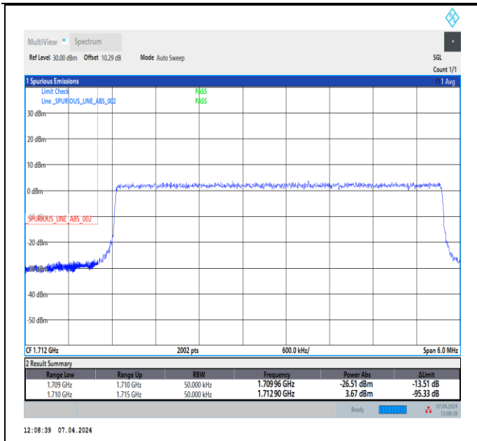
Band4_5MHz_16QAM_19975_25RB#0
