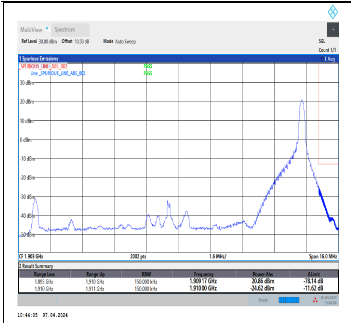
Band2_15MHz_64QAM_19125_1RB#74
