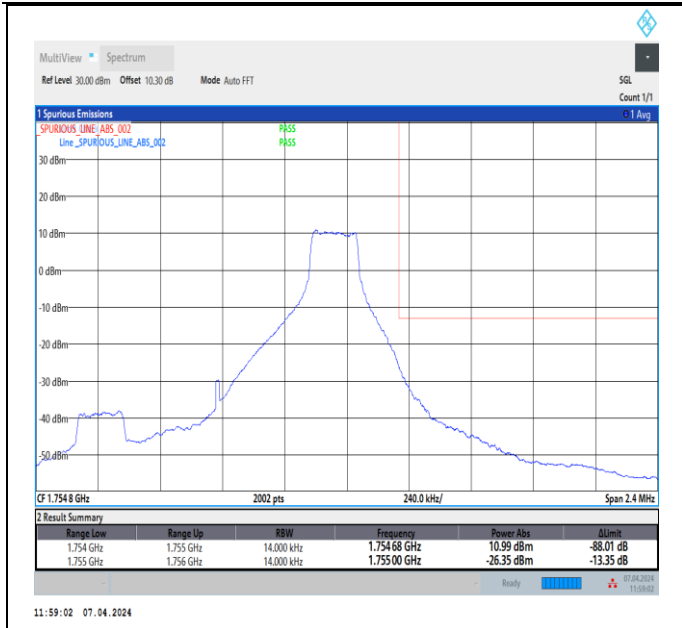
Band4_1.4MHz_64QAM_20393_1RB#5
