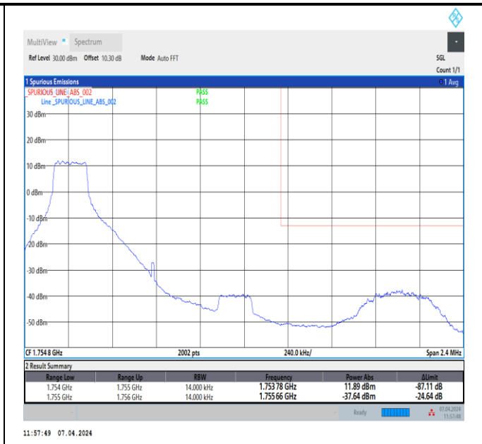
Band4_1.4MHz_16QAM_20393_1RB#0
