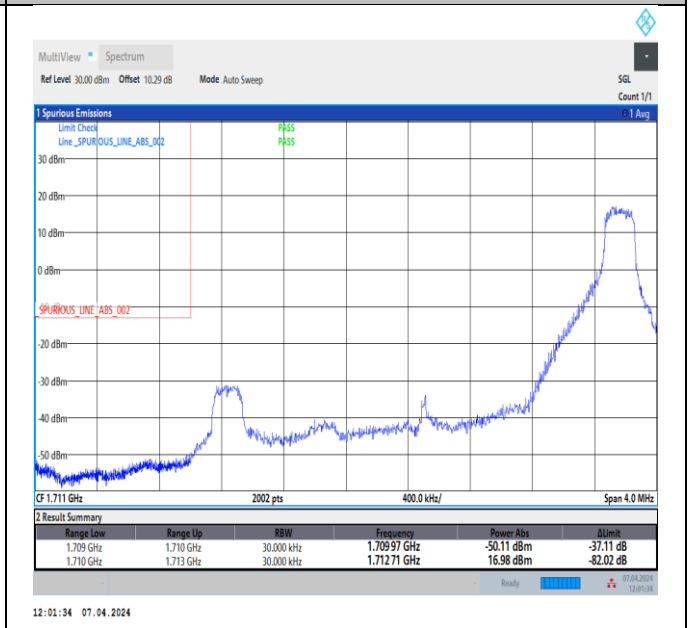
Band4_3MHz_QPSK_19965_1RB#14
