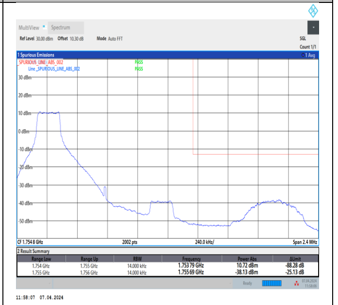
Band4_1.4MHz_64QAM_20393_1RB#0
