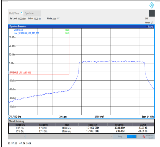
Band4_1.4MHz_64QAM_19957_6RB#0
