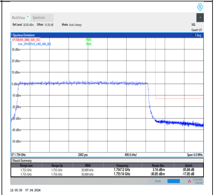
Band4_3MHz_64QAM_20385_15RB#0
