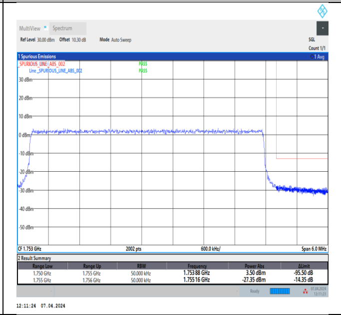
Band4_5MHz_16QAM_20375_25RB#0
