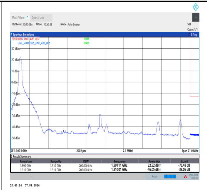
Band2_20MHz_QPSK_19100_1RB#0
