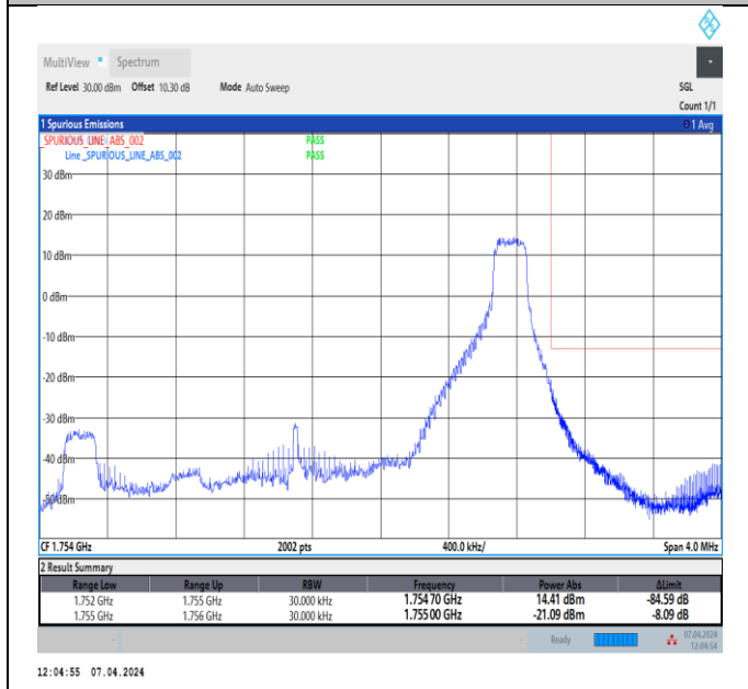
Band4_3MHz_64QAM_20385_1RB#14
