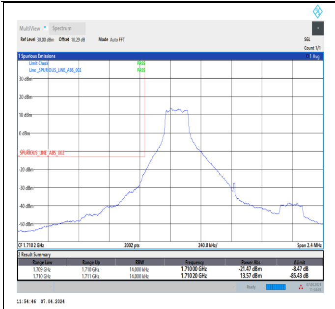
Band4_1.4MHz_QPSK_19957_1RB#0
