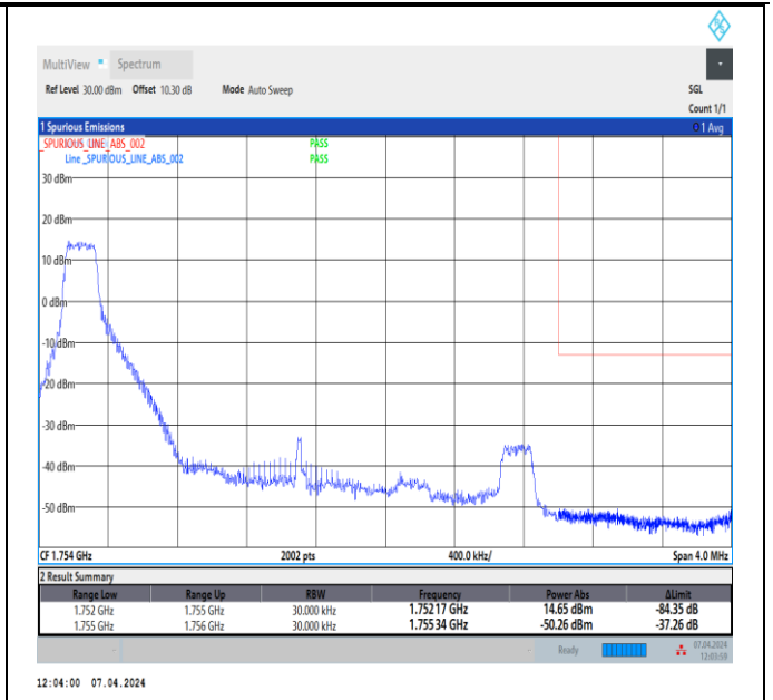
Band4_3MHz_64QAM_20385_1RB#0
