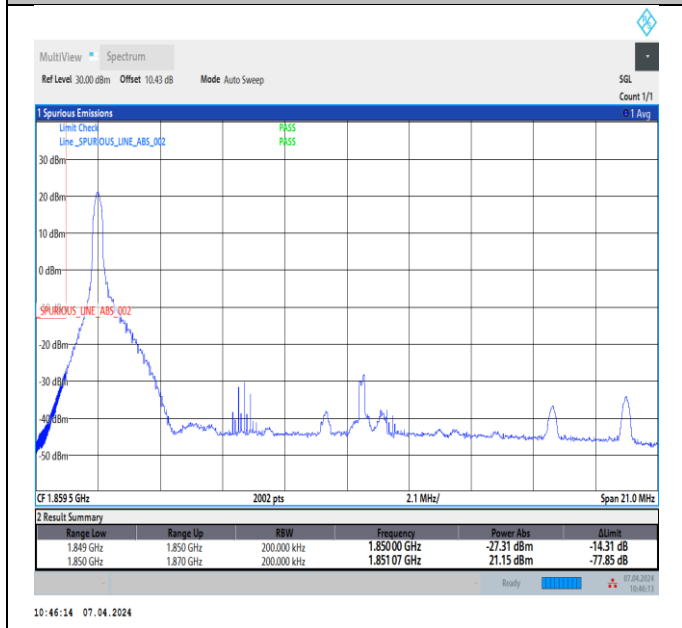
Band2_20MHz_64QAM_18700_1RB#0
