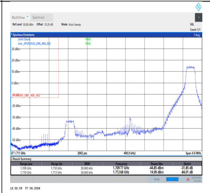
Band4_3MHz_64QAM_19965_1RB#14
