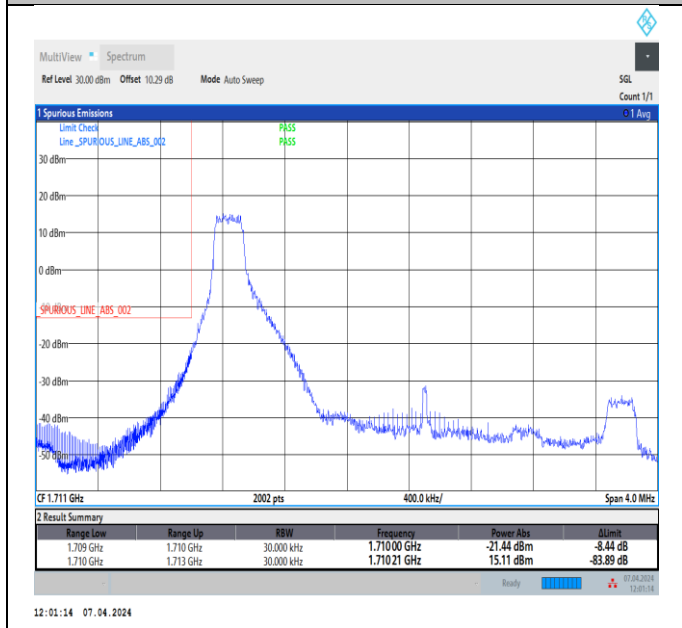
Band4_3MHz_64QAM_19965_1RB#0
