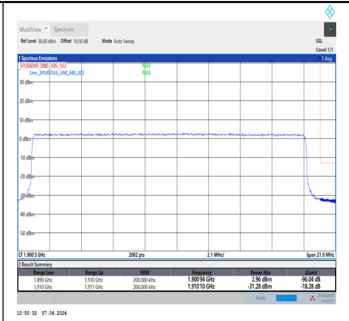
Band2_20MHz_16QAM_19100_100RB#0
