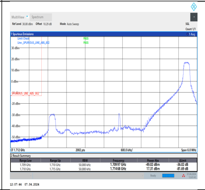
Band4_5MHz_16QAM_19975_1RB#24
