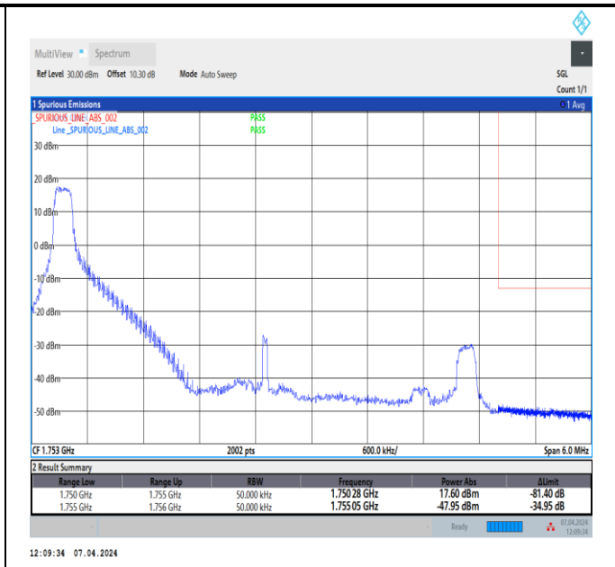
Band4_5MHz_16QAM_20375_1RB#0
