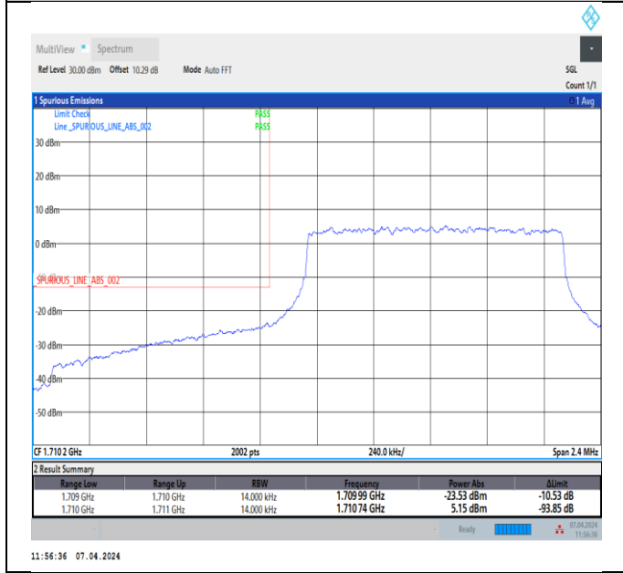
Band4_1.4MHz_QPSK_19957_6RB#0
