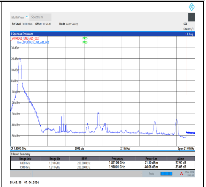
Band2_20MHz_64QAM_19100_1RB#0
