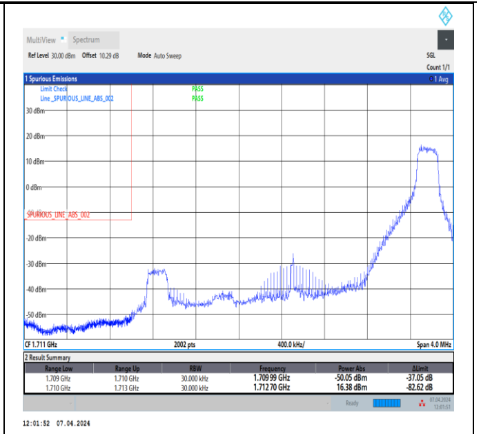
Band4_3MHz_16QAM_19965_1RB#14
