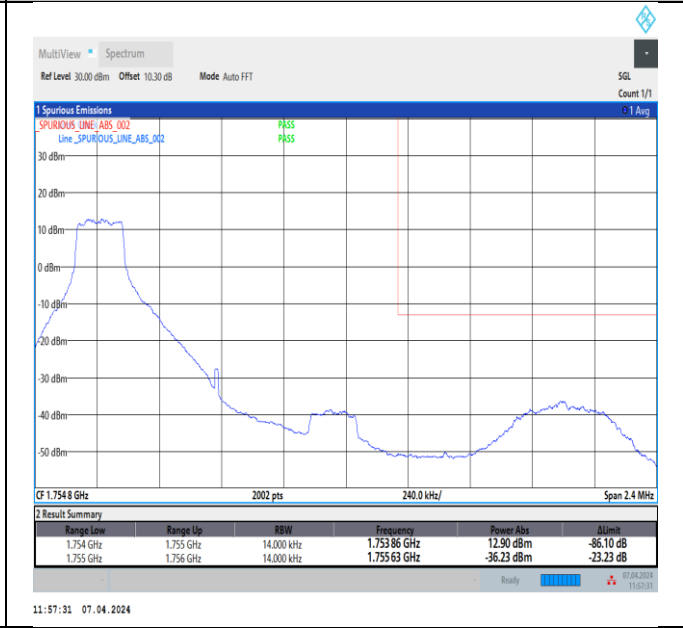
Band4_1.4MHz_QPSK_20393_1RB#0
