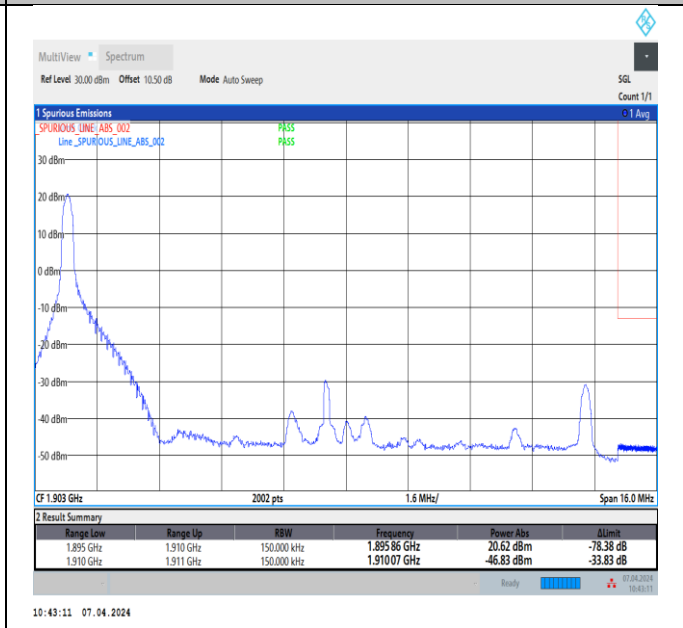
Band2_15MHz_64QAM_19125_1RB#0
