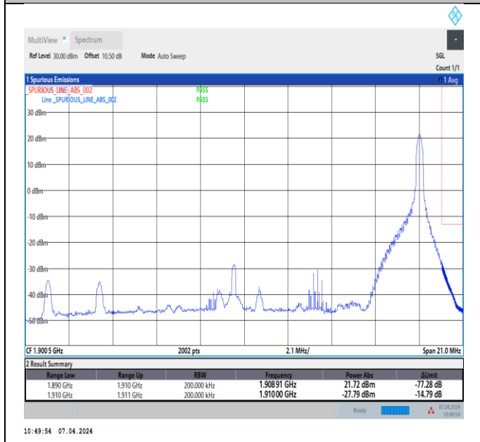
Band2_20MHz_64QAM_19100_1RB#99
