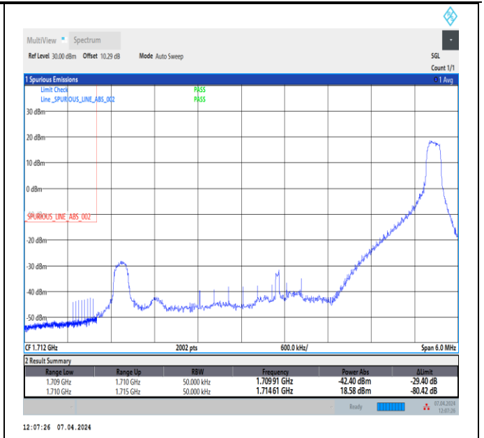
Band4_5MHz_QPSK_19975_1RB#24
