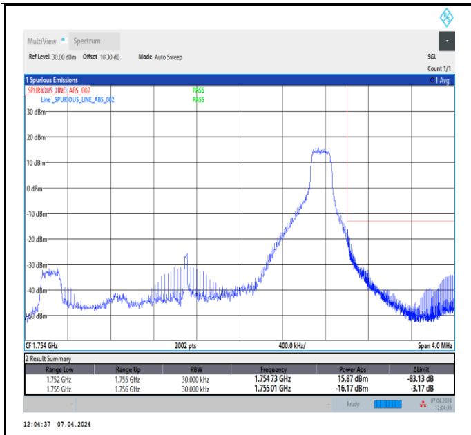
Band4_3MHz_16QAM_20385_1RB#14
