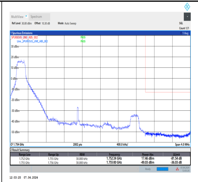
Band4_3MHz_QPSK_20385_1RB#0
