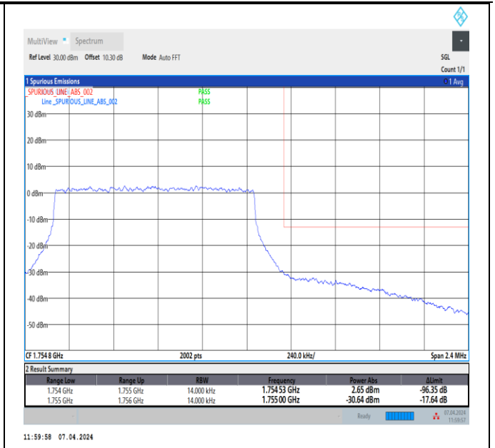
Band4_1.4MHz_64QAM_20393_6RB#0
