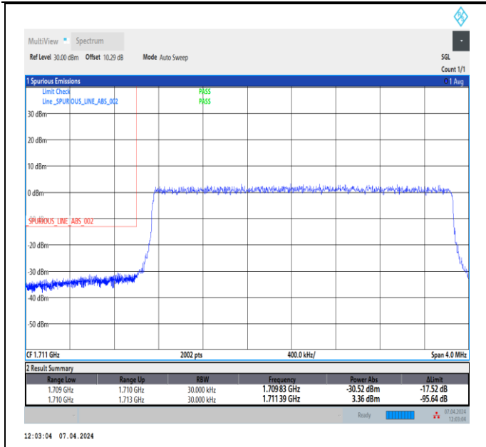
Band4_3MHz_64QAM_19965_15RB#0
