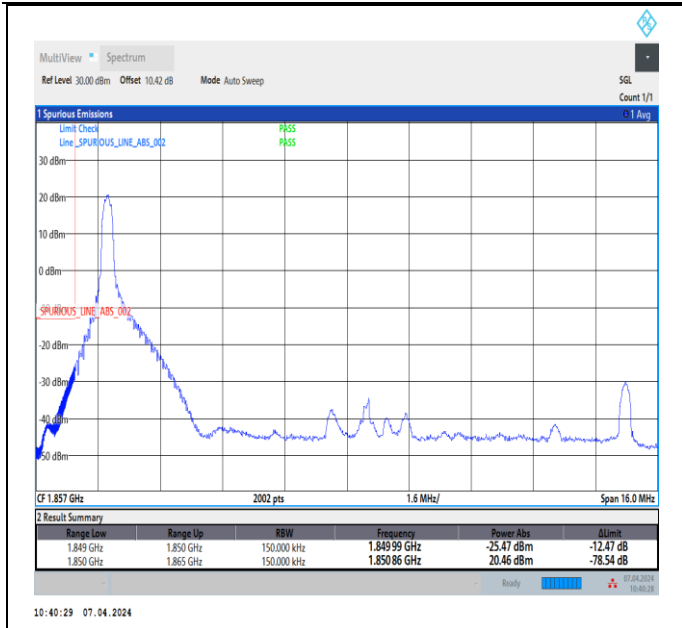
Band2_15MHz_64QAM_18675_1RB#0
