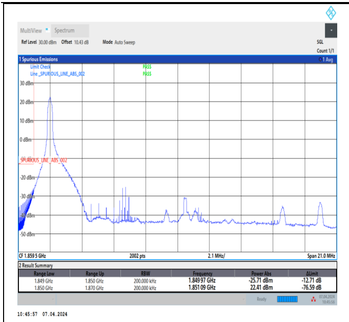
Band2_20MHz_16QAM_18700_1RB#0
