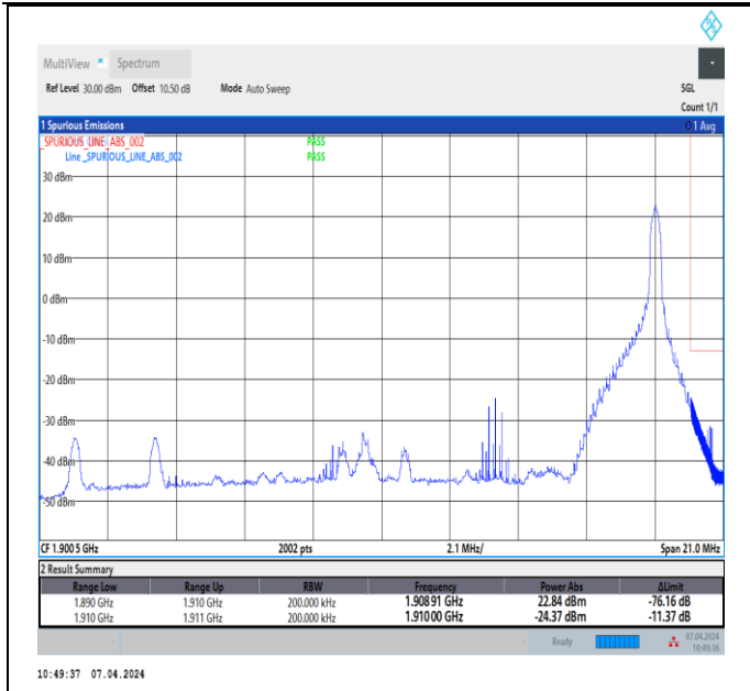
Band2_20MHz_16QAM_19100_1RB#99
