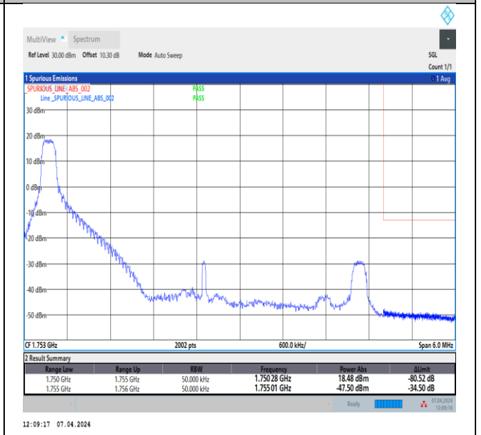
Band4_5MHz_QPSK_20375_1RB#0
