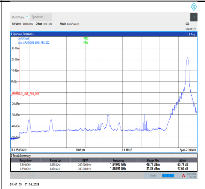
Band2_20MHz_64QAM_18700_1RB#99
