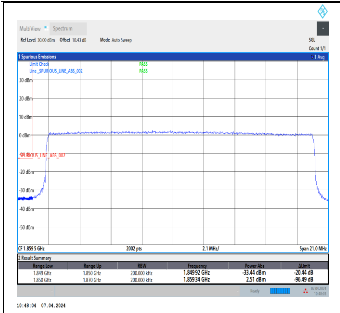
Band2_20MHz_64QAM_18700_100RB#0
