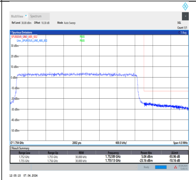
Band4_3MHz_QPSK_20385_15RB#0
