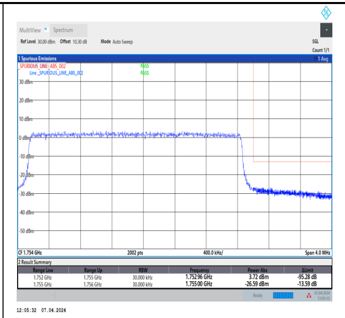
Band4_3MHz_16QAM_20385_15RB#0
