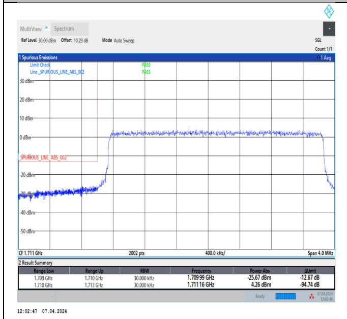
Band4_3MHz_16QAM_19965_15RB#0
