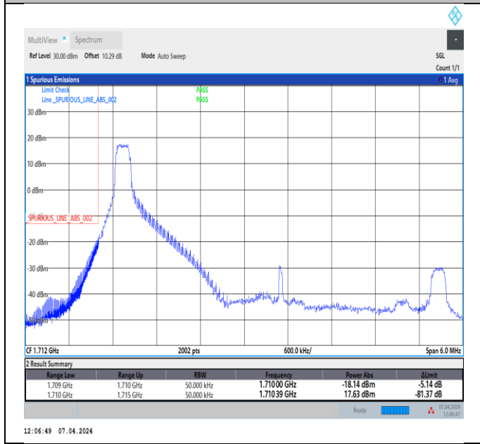
Band4_5MHz_16QAM_19975_1RB#0
