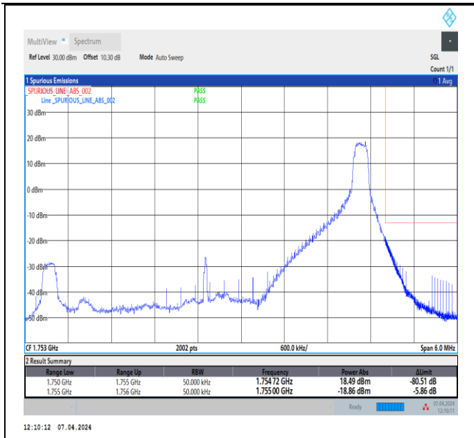
Band4_5MHz_QPSK_20375_1RB#24
