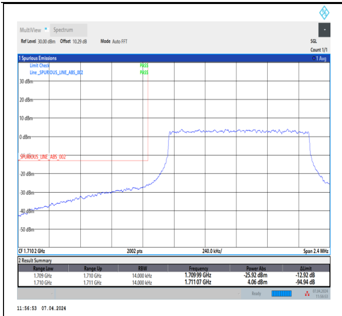
Band4_1.4MHz_16QAM_19957_6RB#0
