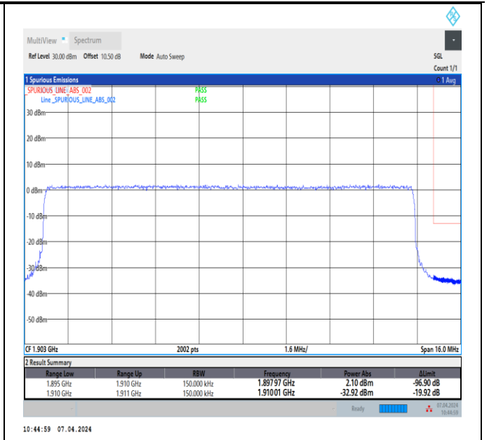
Band2_15MHz_64QAM_19125_75RB#0
