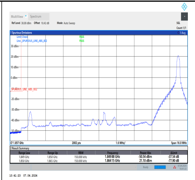
Band2_15MHz_64QAM_18675_1RB#74
