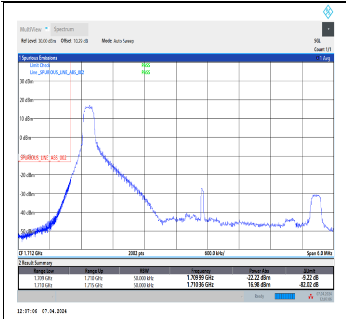
Band4_5MHz_64QAM_19975_1RB#0
