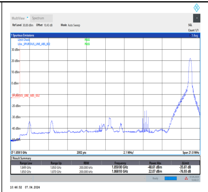
Band2_20MHz_16QAM_18700_1RB#99
