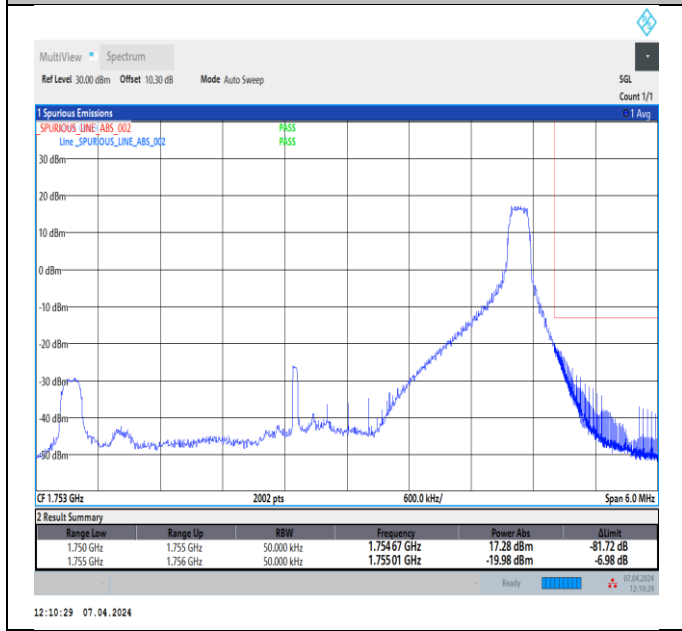
Band4_5MHz_16QAM_20375_1RB#24
