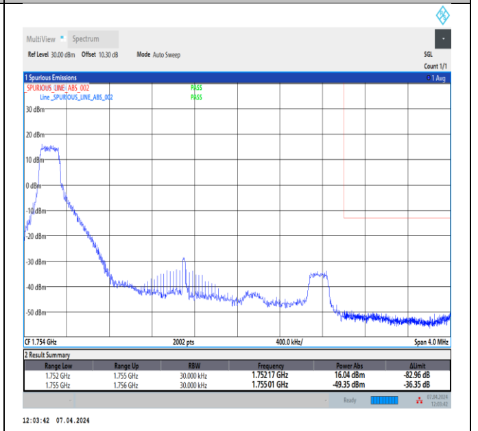
Band4_3MHz_16QAM_20385_1RB#0
