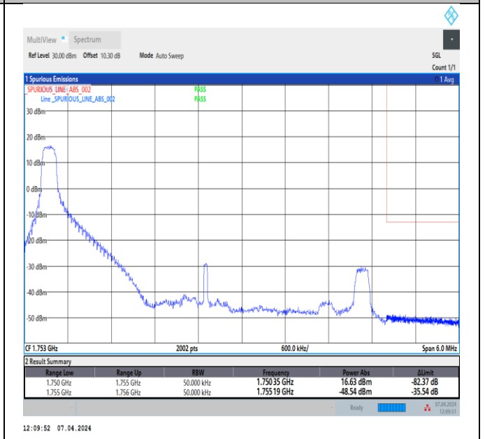
Band4_5MHz_64QAM_20375_1RB#0
