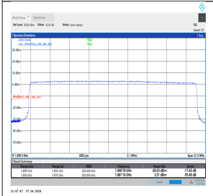
Band2_20MHz_16QAM_18700_100RB#0
