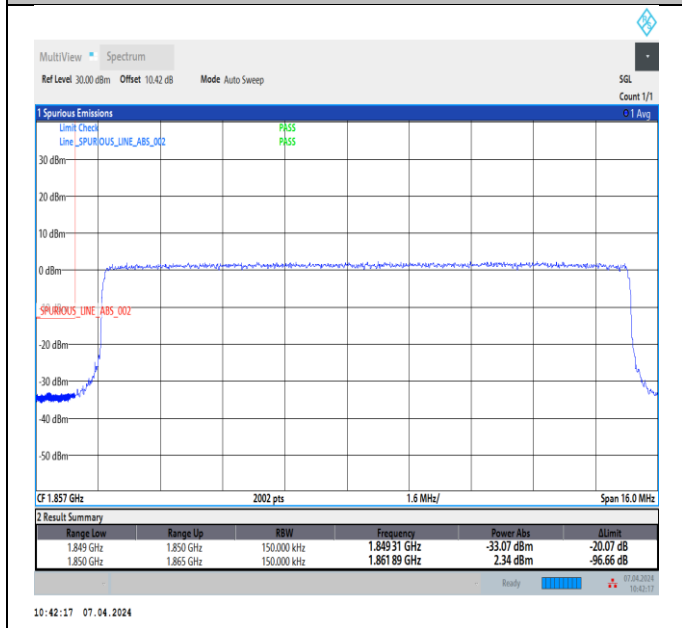
Band2_15MHz_64QAM_18675_75RB#0
