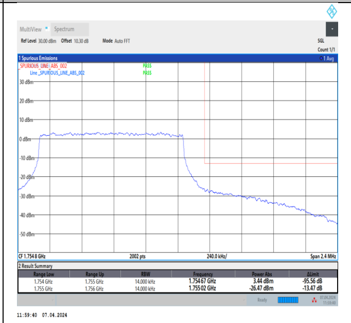
Band4_1.4MHz_16QAM_20393_6RB#0
