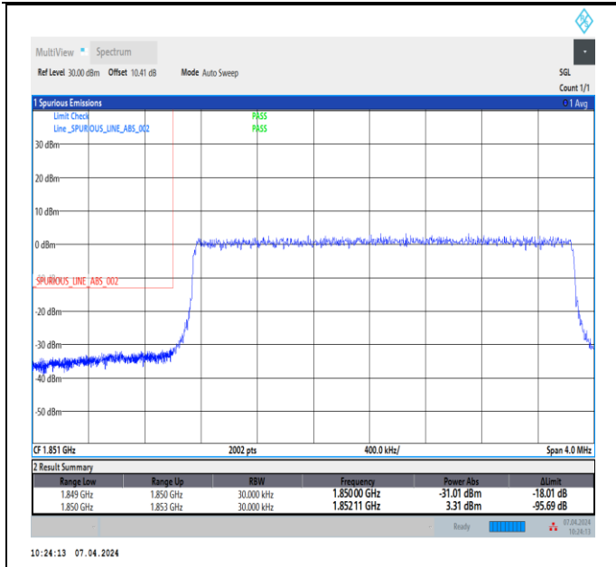
Band2_3MHz_64QAM_18615_15RB#0
