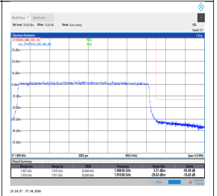
Band2_3MHz_64QAM_19185_15RB#0
