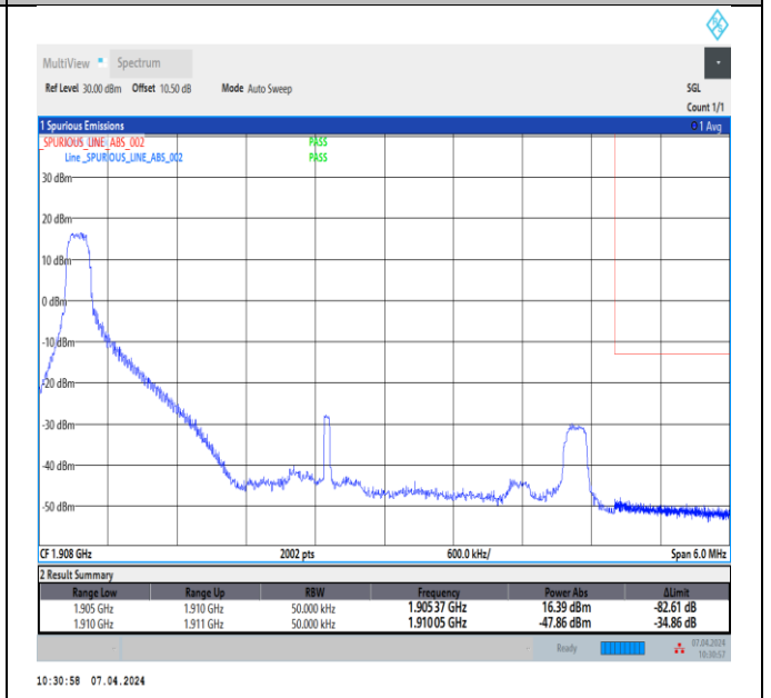
Band2_5MHz_64QAM_19175_1RB#0
