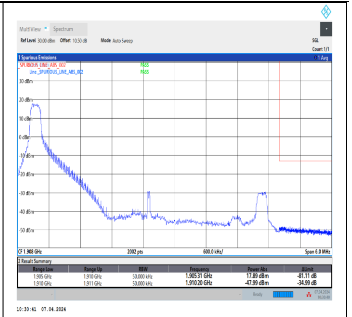
Band2_5MHz_16QAM_19175_1RB#0
