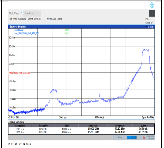
Band2_3MHz_QPSK_18615_1RB#14
