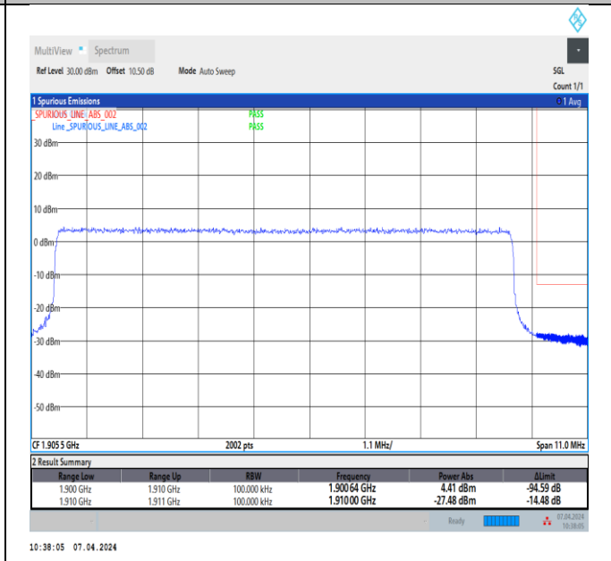
Band2_10MHz_QPSK_19150_50RB#0
