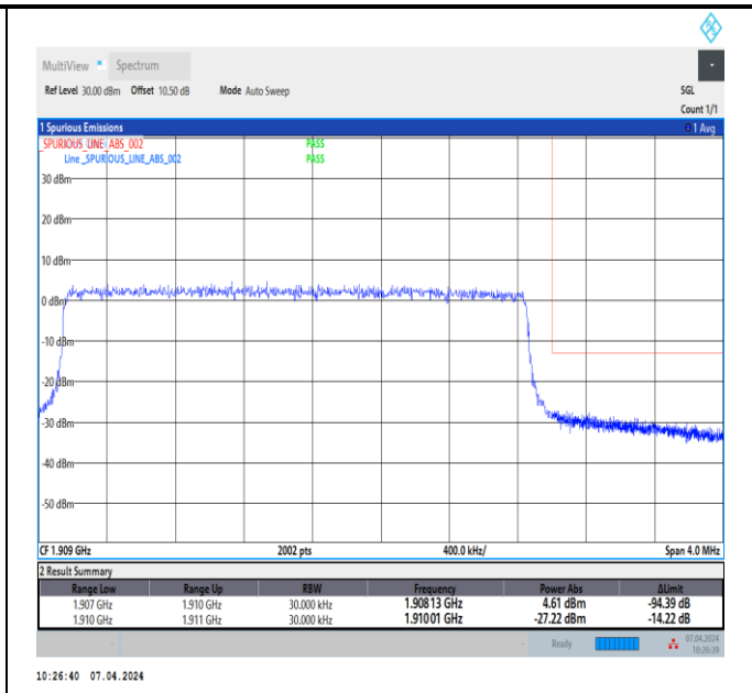
Band2_3MHz_16QAM_19185_15RB#0
