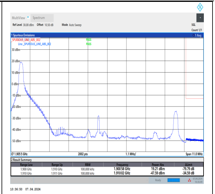
Band2_10MHz_64QAM_19150_1RB#0
