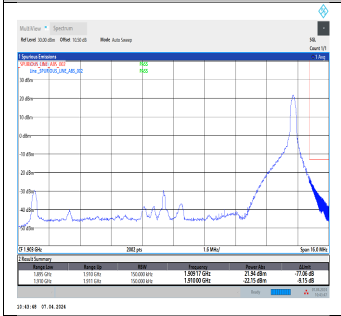
Band2_15MHz_16QAM_19125_1RB#74
