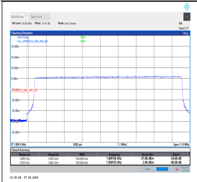
Band2_10MHz_64QAM_18650_50RB#0
