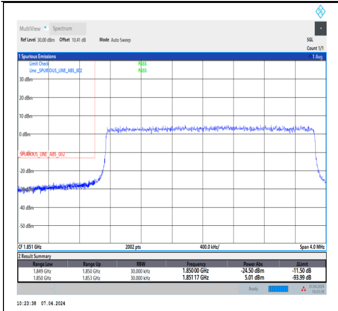
Band2_3MHz_QPSK_18615_15RB#0
