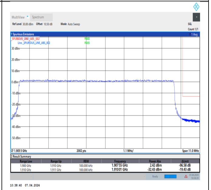
Band2_10MHz_64QAM_19150_50RB#0
