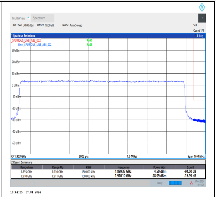
Band2_15MHz_QPSK_19125_75RB#0
