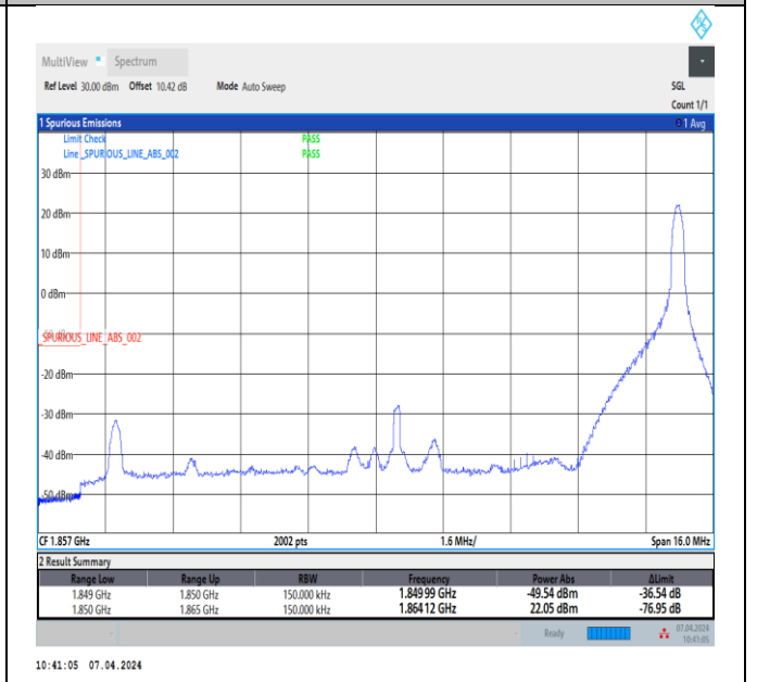
Band2_15MHz_16QAM_18675_1RB#74
