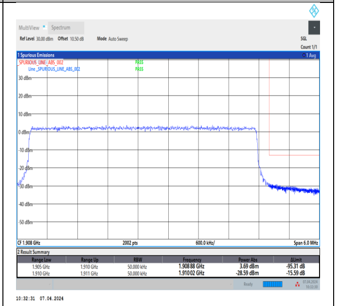
Band2_5MHz_16QAM_19175_25RB#0
