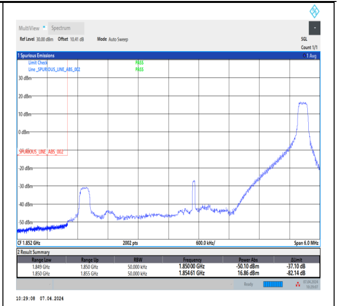
Band2_5MHz_64QAM_18625_1RB#24
