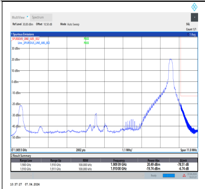
Band2_10MHz_16QAM_19150_1RB#49
