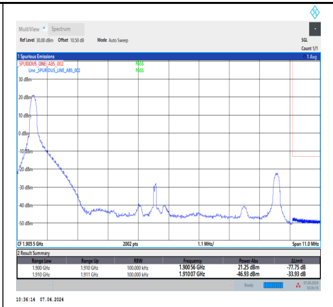
Band2_10MHz_QPSK_19150_1RB#0
