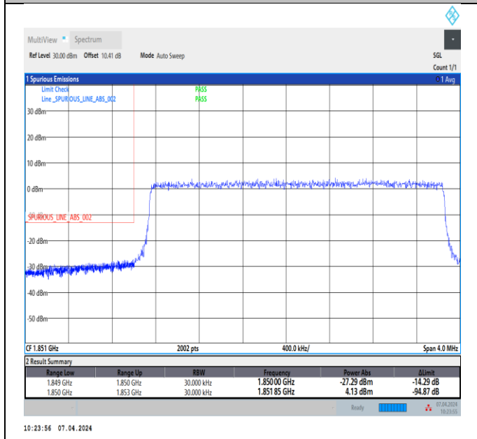
Band2_3MHz_16QAM_18615_15RB#0
