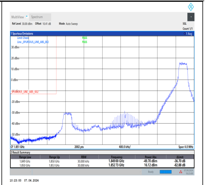
Band2_3MHz_16QAM_18615_1RB#14
