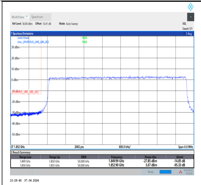
Band2_5MHz_16QAM_18625_25RB#0
