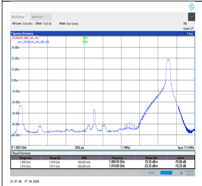
Band2_10MHz_64QAM_19150_1RB#49
