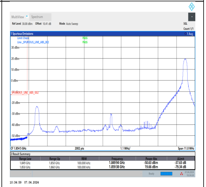
Band2_10MHz_64QAM_18650_1RB#49
