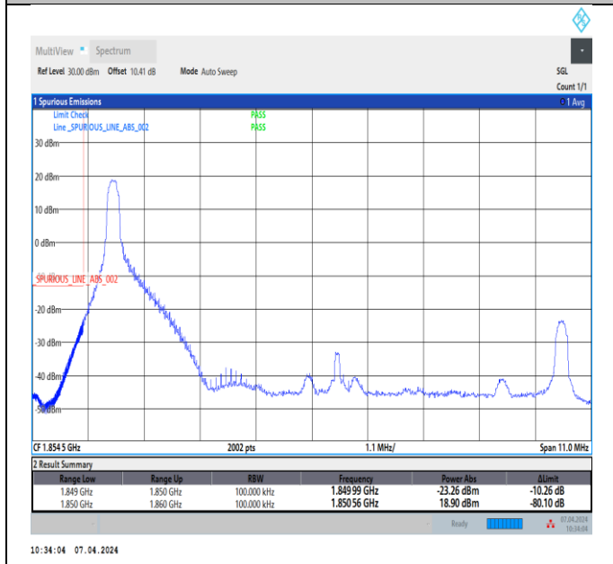
Band2_10MHz_64QAM_18650_1RB#0
