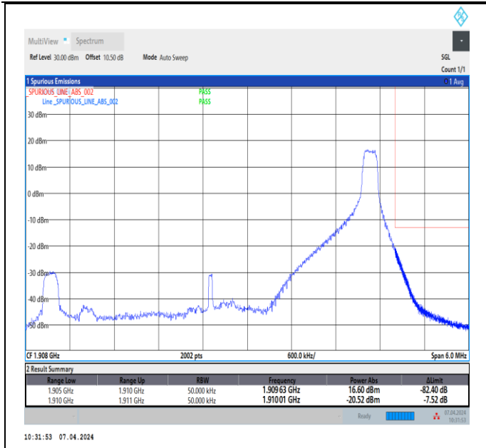
Band2_5MHz_64QAM_19175_1RB#24
