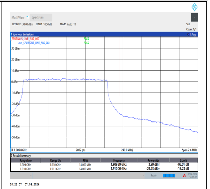
Band2_1.4MHz_64QAM_19193_6RB#0
