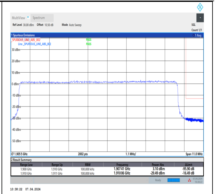
Band2_10MHz_16QAM_19150_50RB#0
