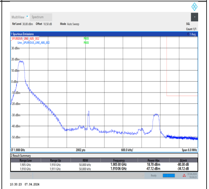
Band2_5MHz_QPSK_19175_1RB#0
