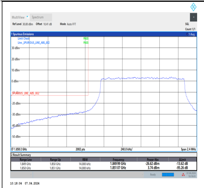
Band2_1.4MHz_16QAM_18607_6RB#0
