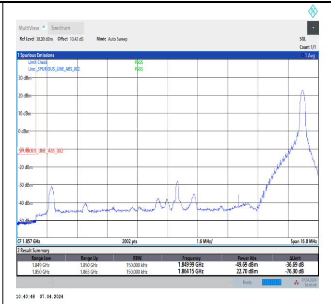
Band2_15MHz_QPSK_18675_1RB#74
