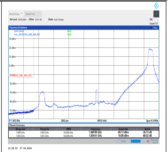
Band2_5MHz_QPSK_18625_1RB#24
