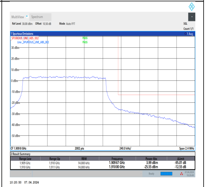
Band2_1.4MHz_16QAM_19193_6RB#0
