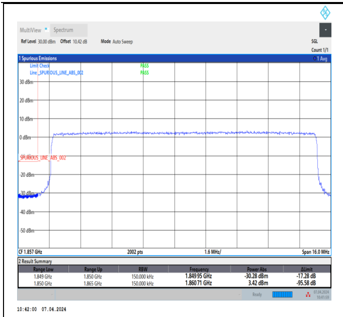
Band2_15MHz_16QAM_18675_75RB#0
