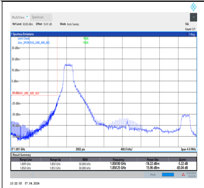
Band2_3MHz_16QAM_18615_1RB#0
