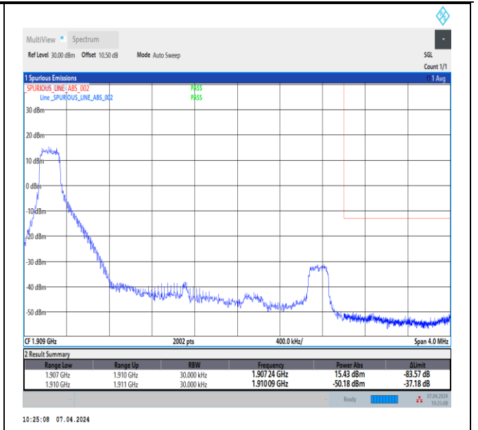
Band2_3MHz_64QAM_19185_1RB#0
