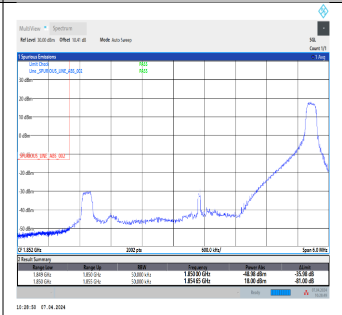
Band2_5MHz_16QAM_18625_1RB#24
