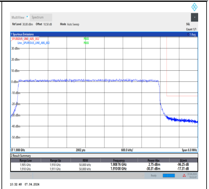
Band2_5MHz_64QAM_19175_25RB#0
