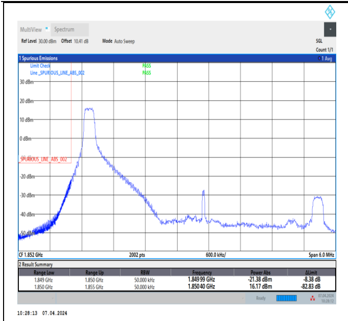
Band2_5MHz_64QAM_18625_1RB#0
