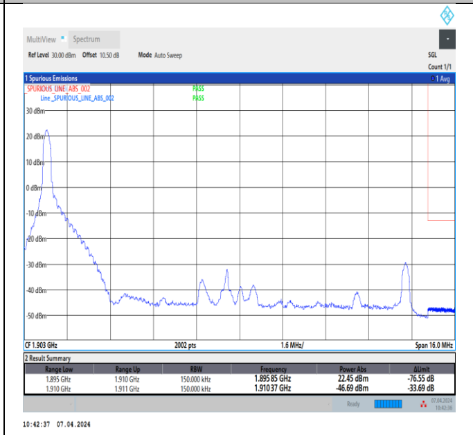
Band2_15MHz_QPSK_19125_1RB#0
