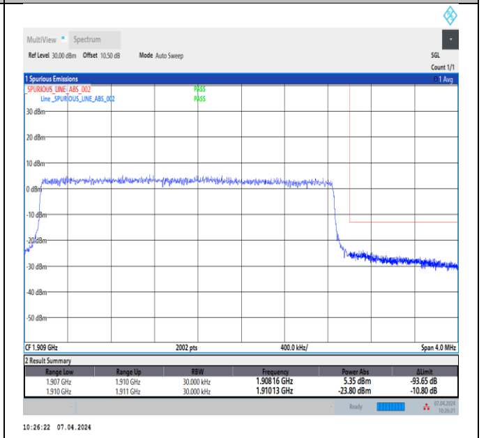
Band2_3MHz_QPSK_19185_15RB#0
