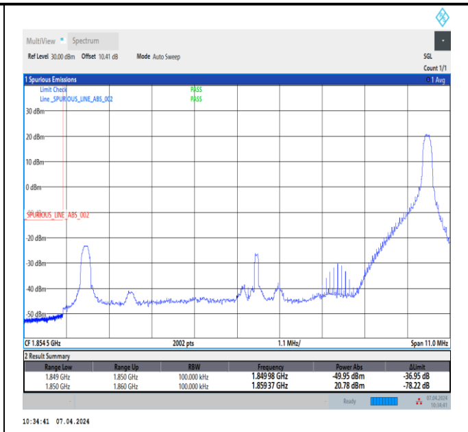
Band2_10MHz_16QAM_18650_1RB#49
