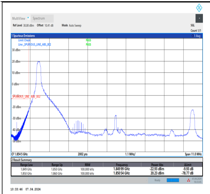
Band2_10MHz_16QAM_18650_1RB#0
