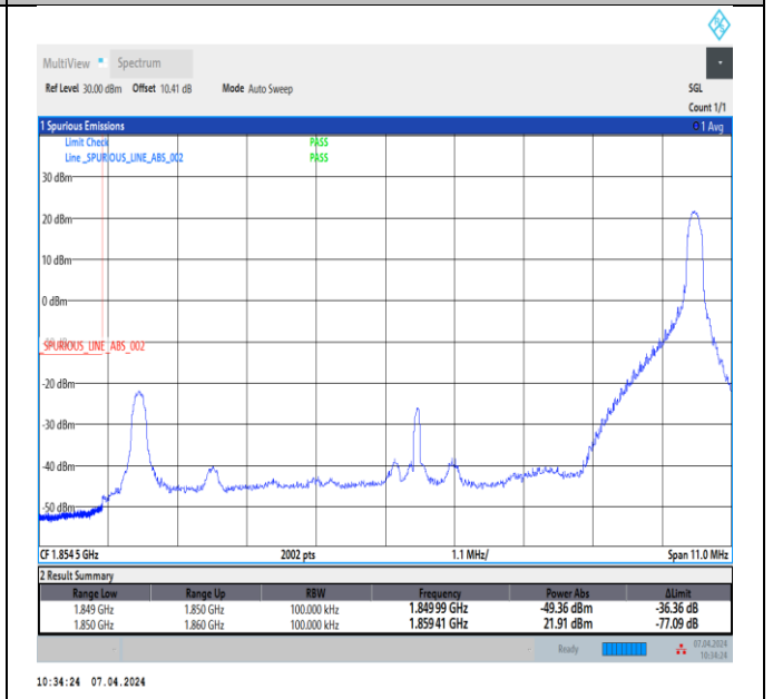
Band2_10MHz_QPSK_18650_1RB#49
