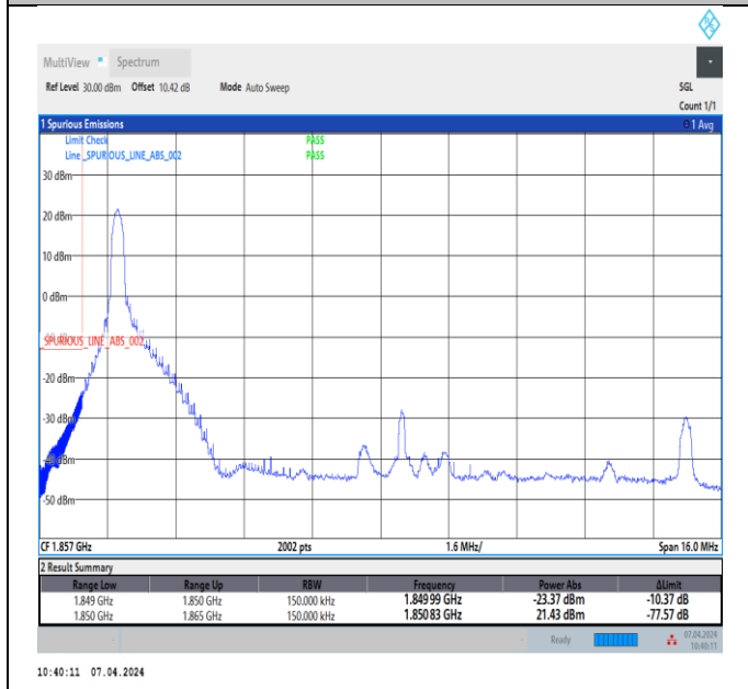
Band2_15MHz_16QAM_18675_1RB#0
