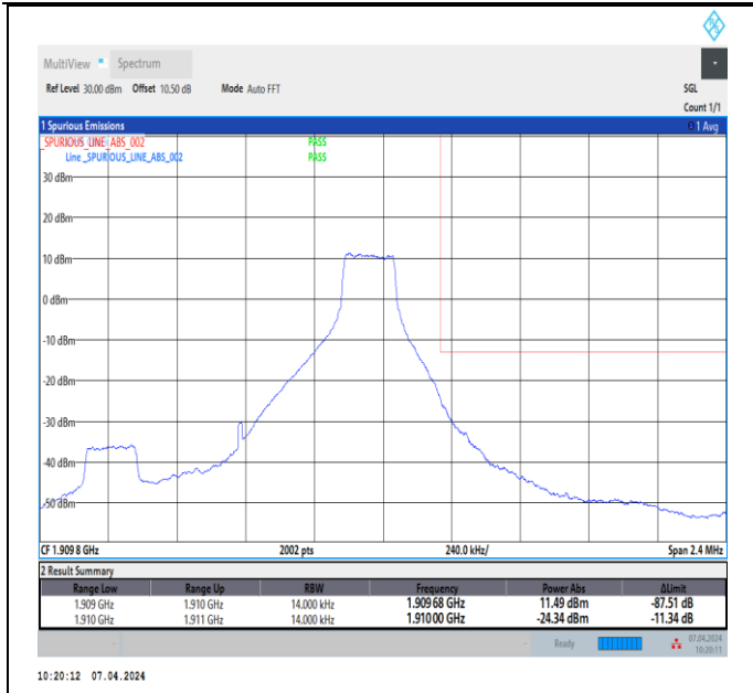
Band2_1.4MHz_64QAM_19193_1RB#5
