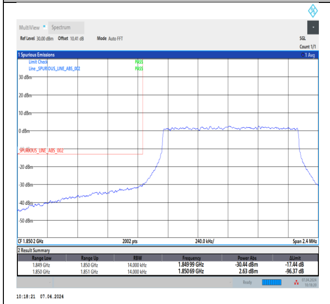
Band2_1.4MHz_64QAM_18607_6RB#0
