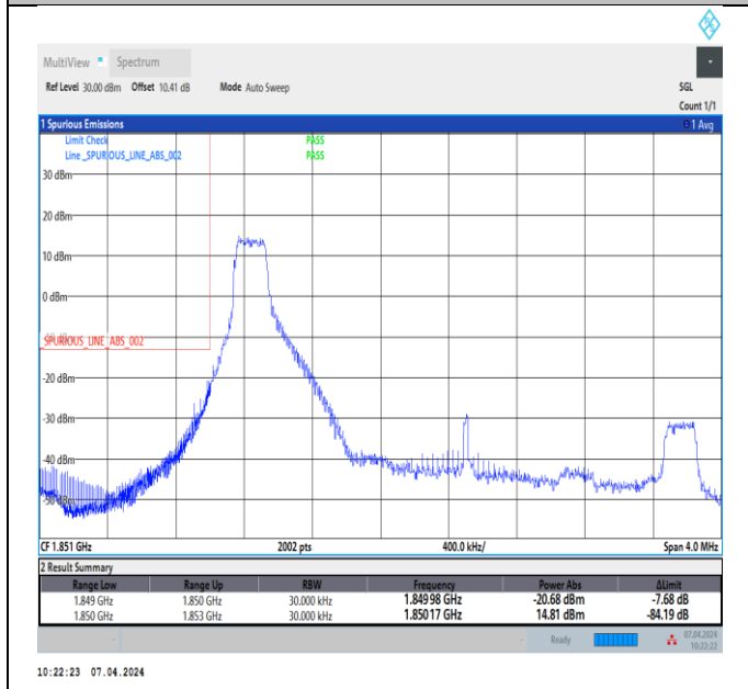
Band2_3MHz_64QAM_18615_1RB#0
