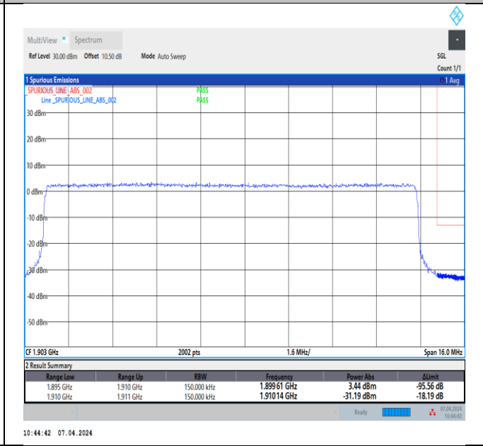
Band2_15MHz_16QAM_19125_75RB#0
