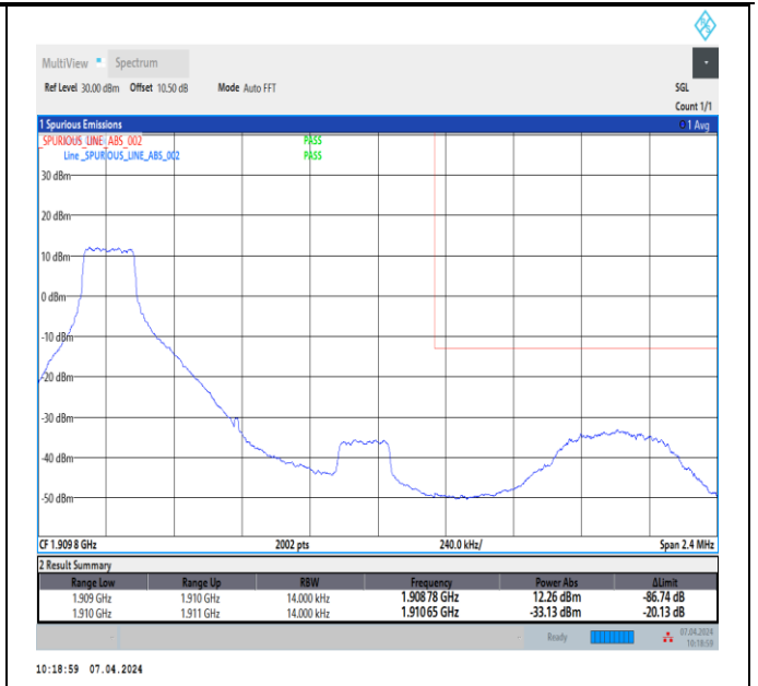
Band2_1.4MHz_16QAM_19193_1RB#0
