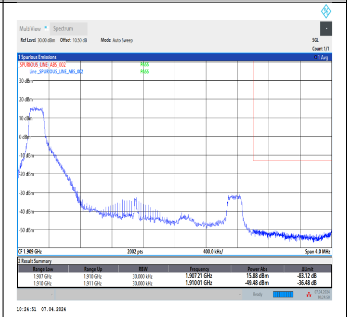
Band2_3MHz_16QAM_19185_1RB#0
