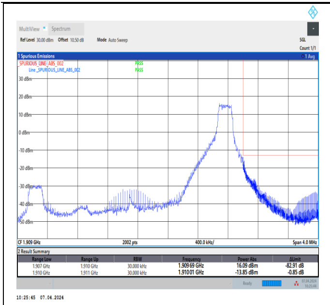
Band2_3MHz_16QAM_19185_1RB#14
