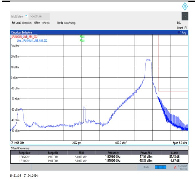
Band2_5MHz_16QAM_19175_1RB#24
