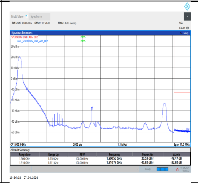
Band2_10MHz_16QAM_19150_1RB#0
