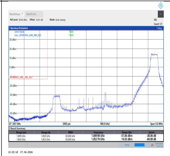
Band2_3MHz_64QAM_18615_1RB#14
