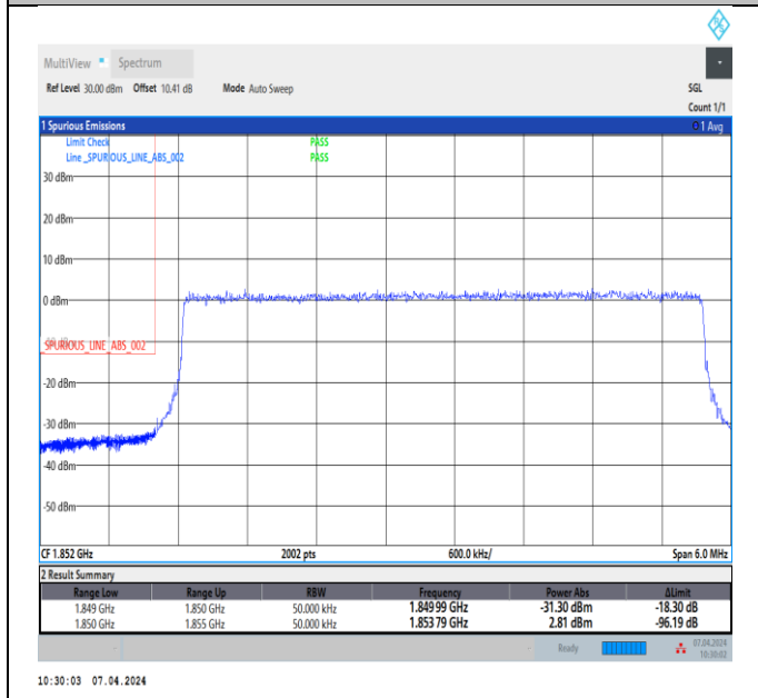
Band2_5MHz_64QAM_18625_25RB#0
