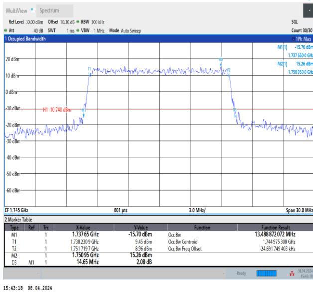
Band66-15MHz-16QAM-132322-75RB#0-PASS
