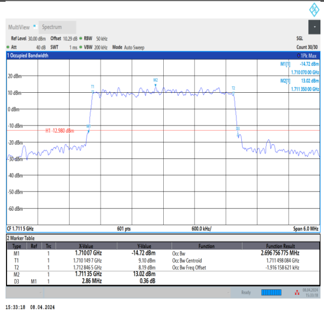
Band66-3MHz-64QAM-131987-15RB#0-PASS
