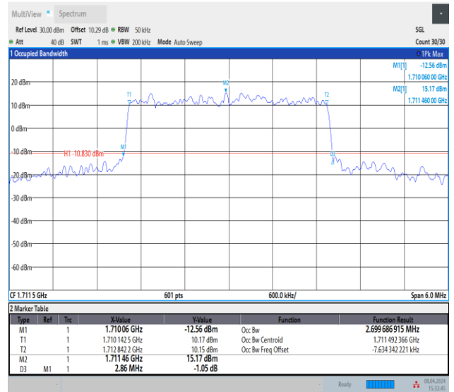
Band66-3MHz-QPSK-131987-15RB#0-PASS
