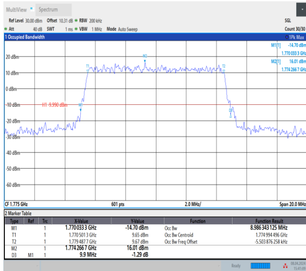
Band66-10MHz-16QAM-132622-50RB#0-PASS
