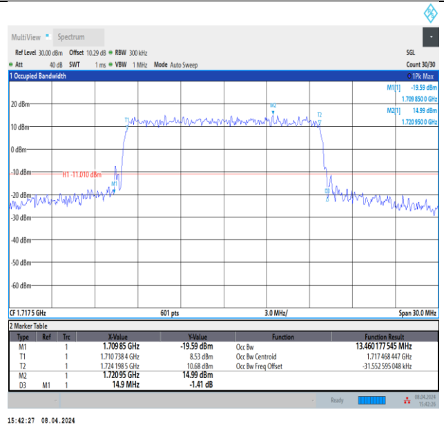
Band66-15MHz-16QAM-132047-75RB#0-PASS
