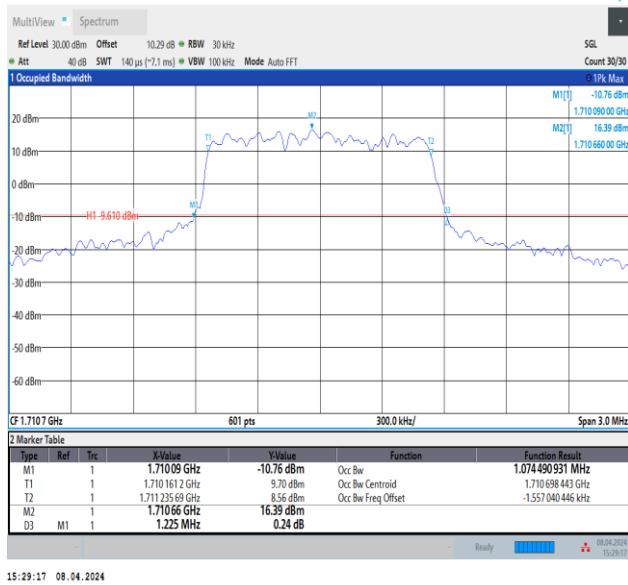
Band66-1.4MHz-QPSK-131979-6RB#0-PASS
