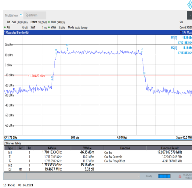
Band66-20MHz-64QAM-132072-100RB#0-PASS
