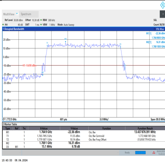
Band66-15MHz-QPSK-132597-75RB#0-PASS
