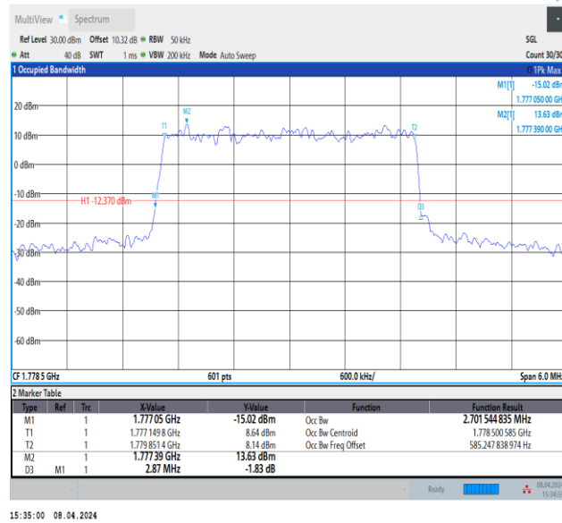
Band66-3MHz-64QAM-132657-15RB#0-PASS
