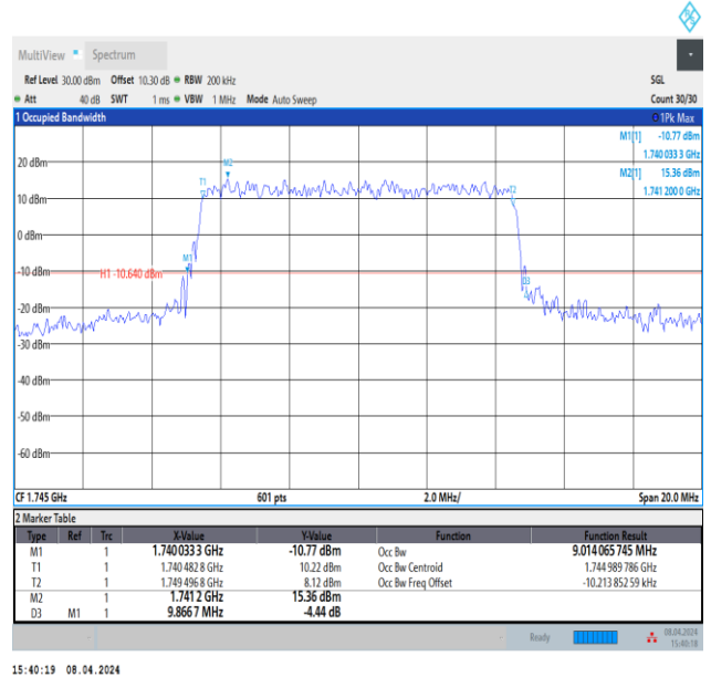
Band66-10MHz-16QAM-132322-50RB#0-PASS
