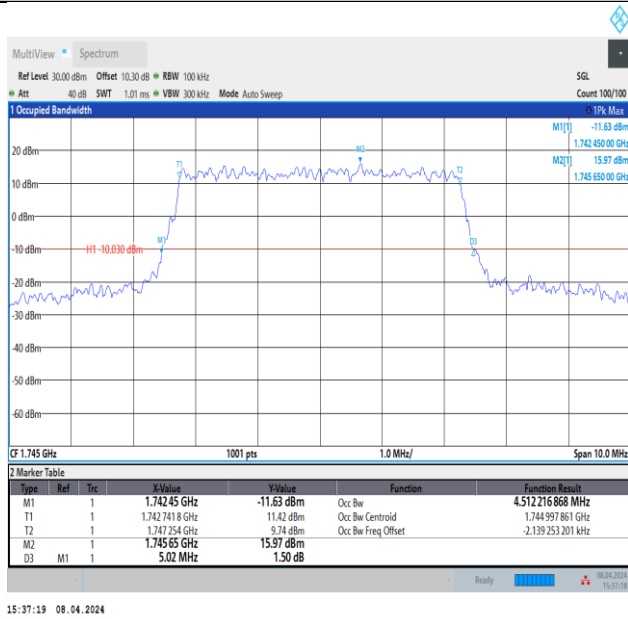
Band66-5MHz-16QAM-132322-25RB#0-PASS
