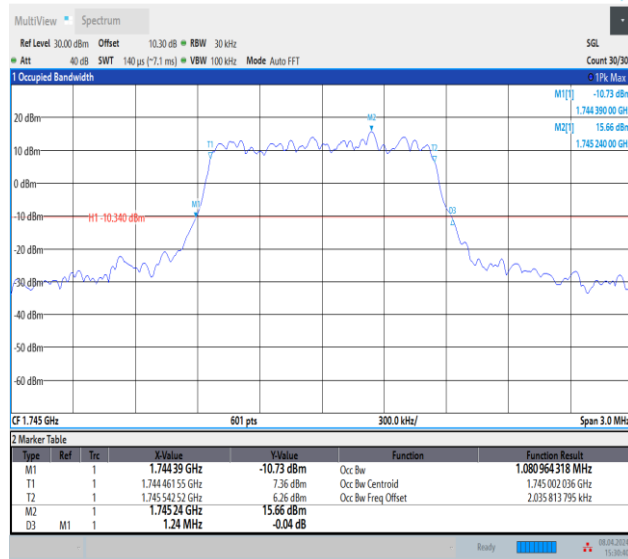
Band66-1.4MHz-64QAM-132322-6RB#0-PASS
