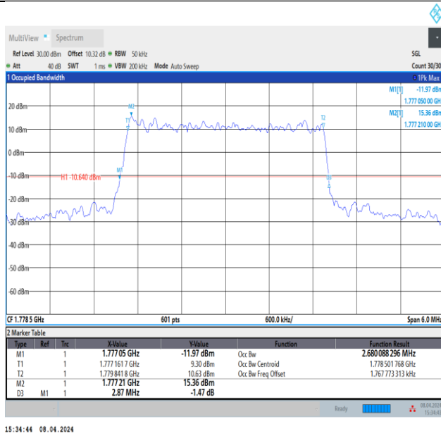
Band66-3MHz-16QAM-132657-15RB#0-PASS
