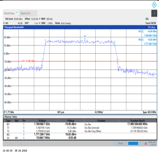
Band66-20MHz-QPSK-132572-100RB#0-PASS
