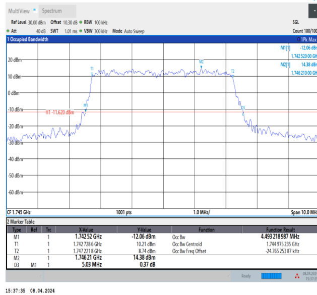
Band66-5MHz-64QAM-132322-25RB#0-PASS
