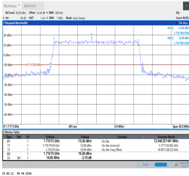
Band66-15MHz-QPSK-132047-75RB#0-PASS
