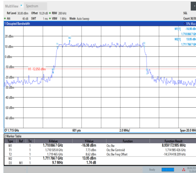
Band66-10MHz-64QAM-132022-50RB#0-PASS
