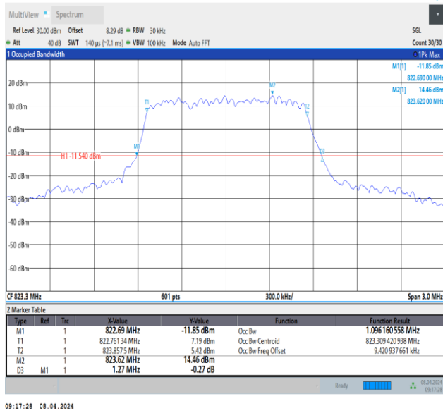
26(814-824)-1.4MHz-64QAM-26783-6RB#0-PASS
