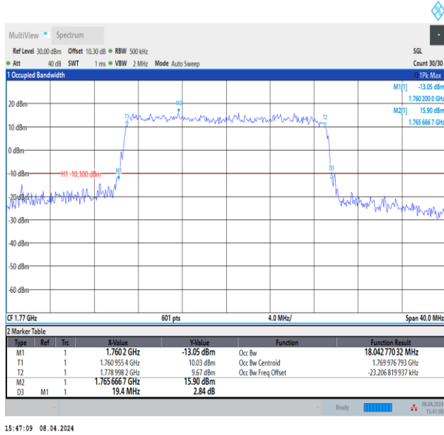
Band66-20MHz-16QAM-132572-100RB#0-PASS
