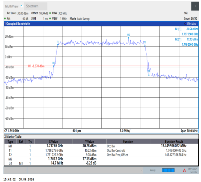
Band66-15MHz-QPSK-132322-75RB#0-PASS
