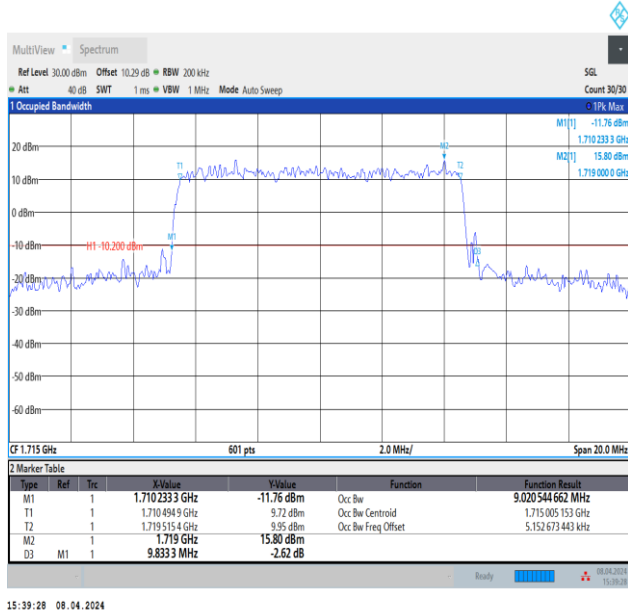
Band66-10MHz-16QAM-132022-50RB#0-PASS
