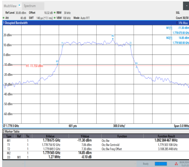
Band66-1.4MHz-64QAM-132665-6RB#0-PASS
