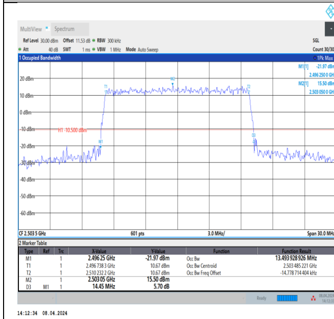
Band41-15MHz-QPSK-39725-75RB#0-PASS
