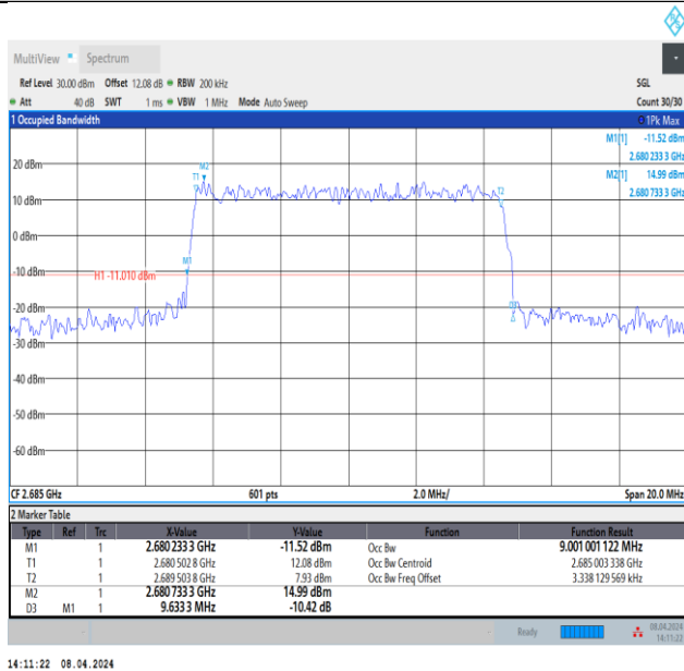
Band41-10MHz-16QAM-41540-50RB#0-PASS
