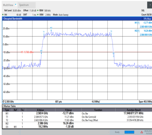
Band41-20MHz-64QAM-40620-100RB#0-PASS
