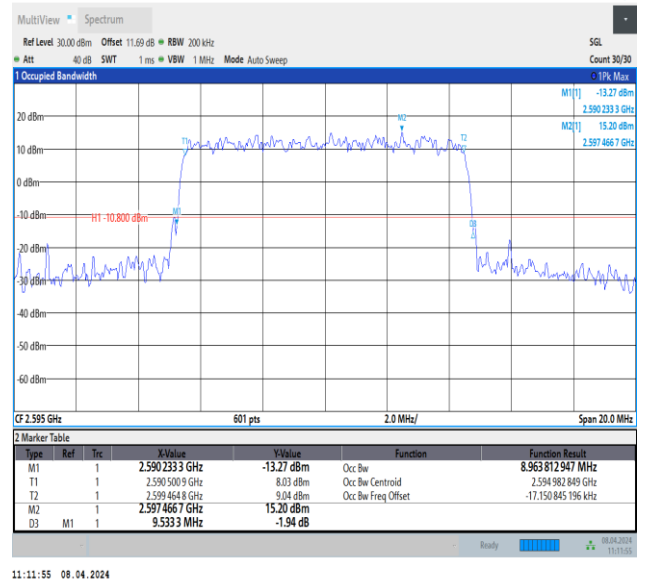
Band38-10MHz-16QAM-38000-50RB#0-PASS
