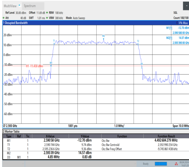
Band41-5MHz-16QAM-40620-25RB#0-PASS
