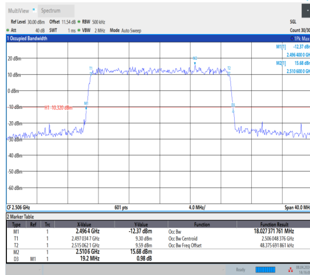
Band41-20MHz-64QAM-39750-100RB#0-PASS
