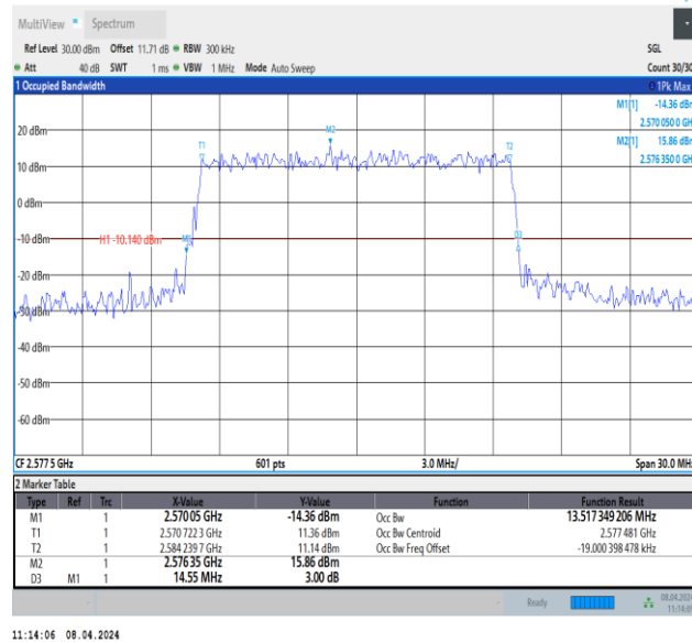
Band38-15MHz-16QAM-37825-75RB#0-PASS
