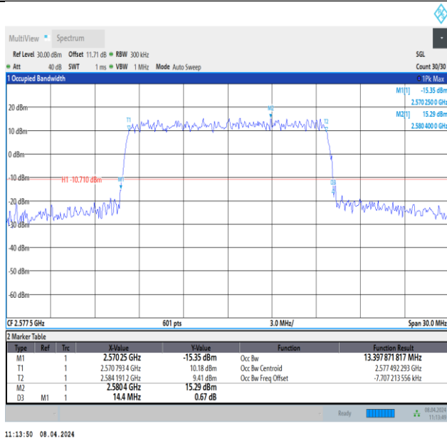
Band38-15MHz-QPSK-37825-75RB#0-PASS
