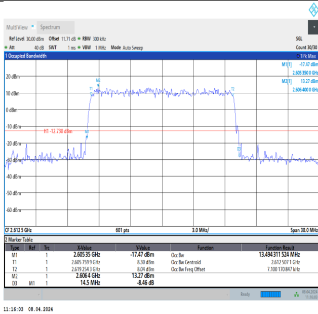
Band38-15MHz-64QAM-38175-75RB#0-PASS
