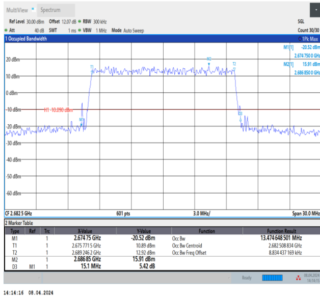
Band41-15MHz-QPSK-41515-75RB#0-PASS
