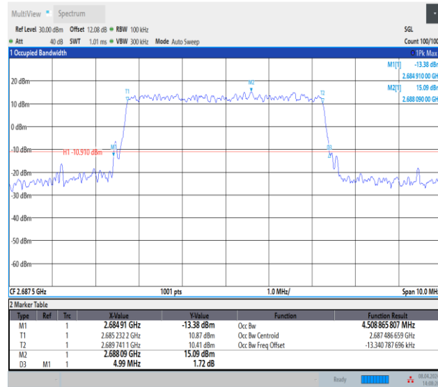
Band41-5MHz-16QAM-41565-25RB#0-PASS
