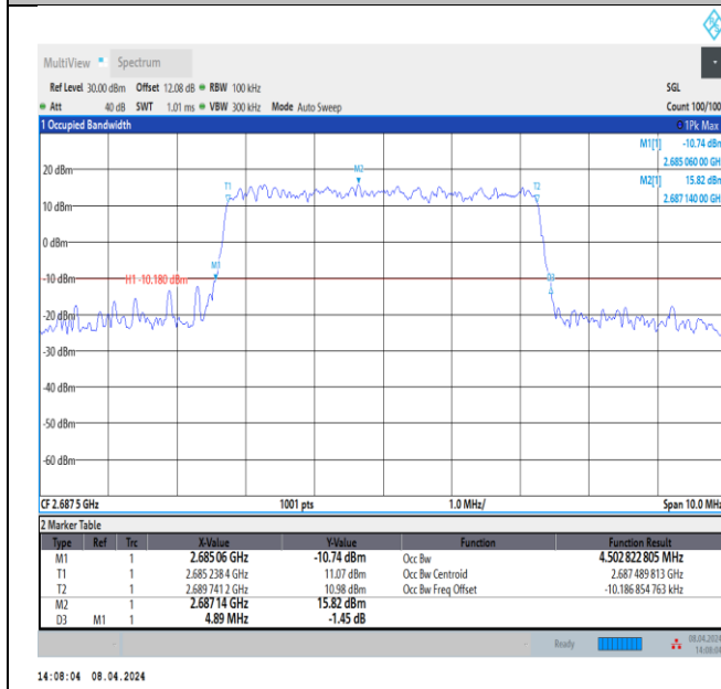
Band41-5MHz-QPSK-41565-25RB#0-PASS
