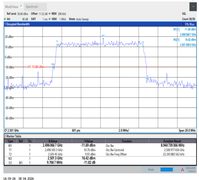
Band41-10MHz-QPSK-39700-50RB#0-PASS
