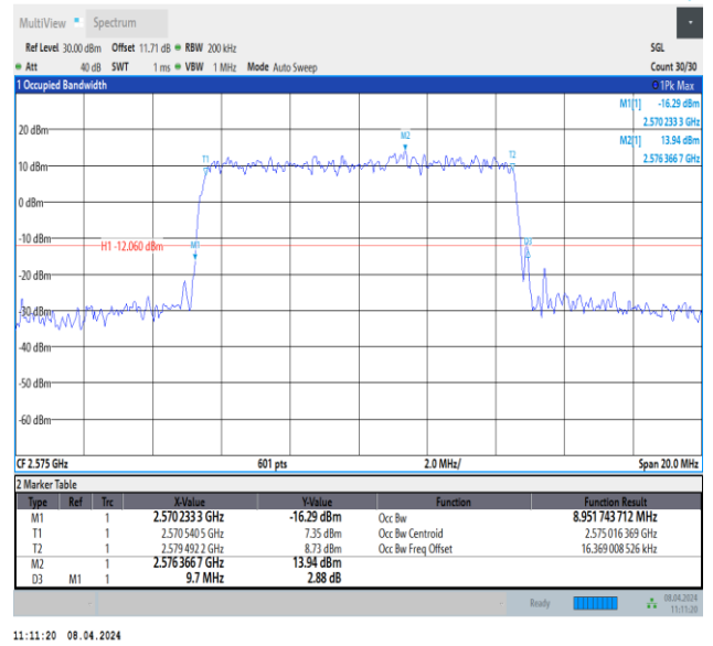
Band38-10MHz-64QAM-37800-50RB#0-PASS
