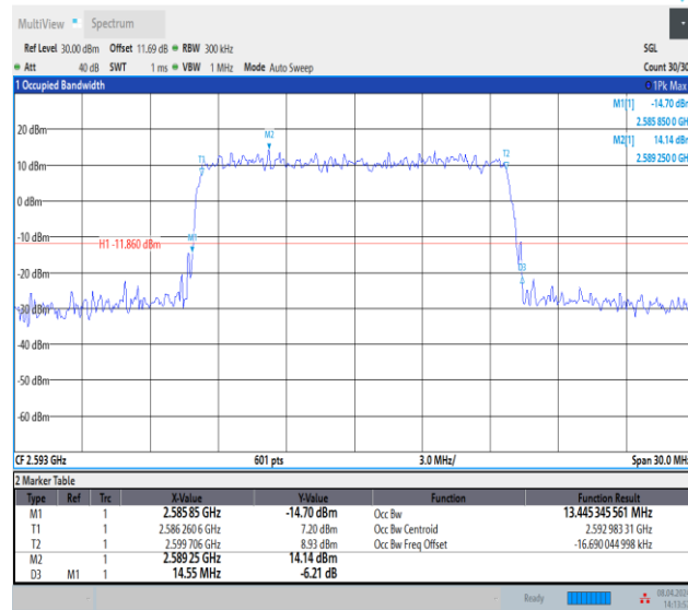
Band41-15MHz-64QAM-40620-75RB#0-PASS
