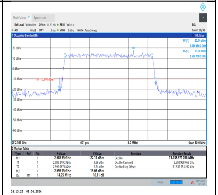
Band41-15MHz-QPSK-40620-75RB#0-PASS
