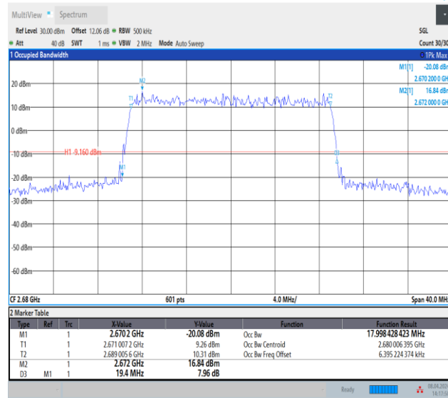
Band41-20MHz-64QAM-41490-100RB#0-PASS
