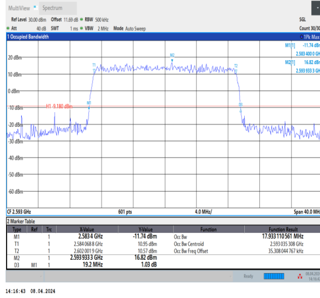
Band41-20MHz-16QAM-40620-100RB#0-PASS
