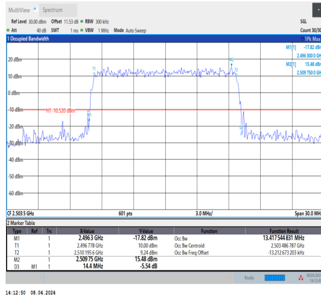
Band41-15MHz-16QAM-39725-75RB#0-PASS
