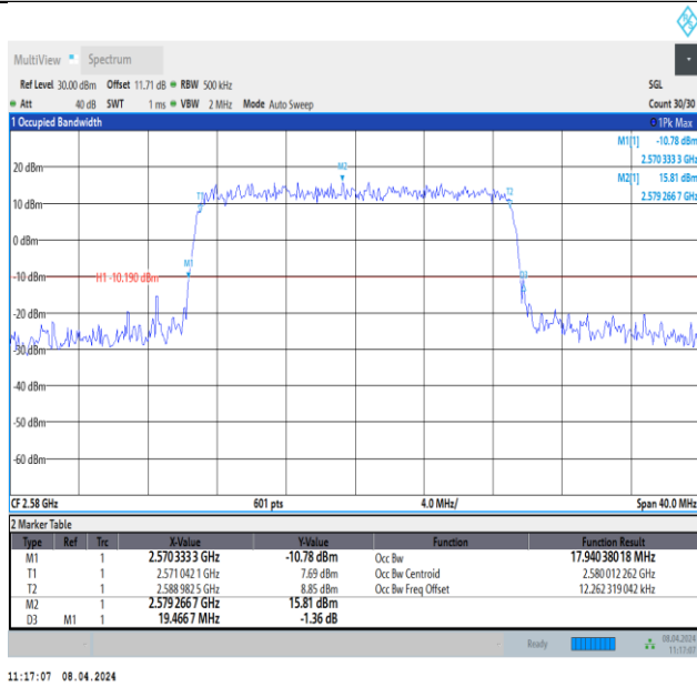
Band38-20MHz-16QAM-37850-100RB#0-PASS
