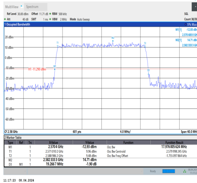
Band38-20MHz-64QAM-37850-100RB#0-PASS
