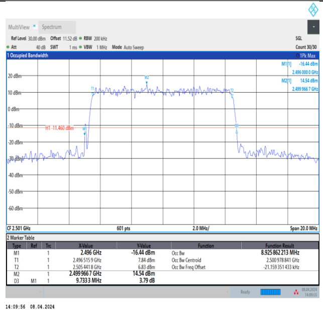
Band41-10MHz-64QAM-39700-50RB#0-PASS
