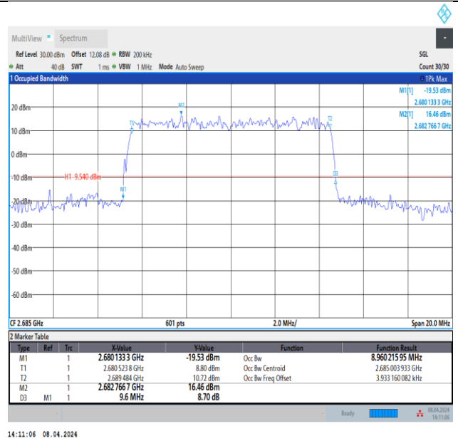
Band41-10MHz-QPSK-41540-50RB#0-PASS
