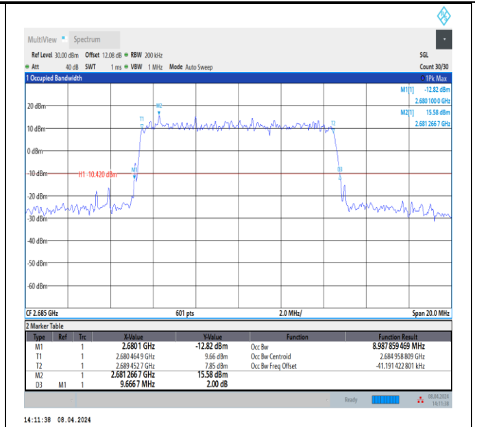
Band41-10MHz-64QAM-41540-50RB#0-PASS
