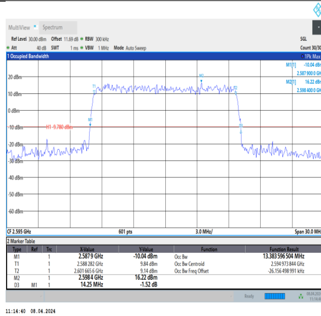
Band38-15MHz-QPSK-38000-75RB#0-PASS
