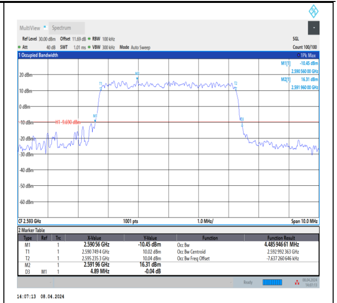
Band41-5MHz-QPSK-40620-25RB#0-PASS
