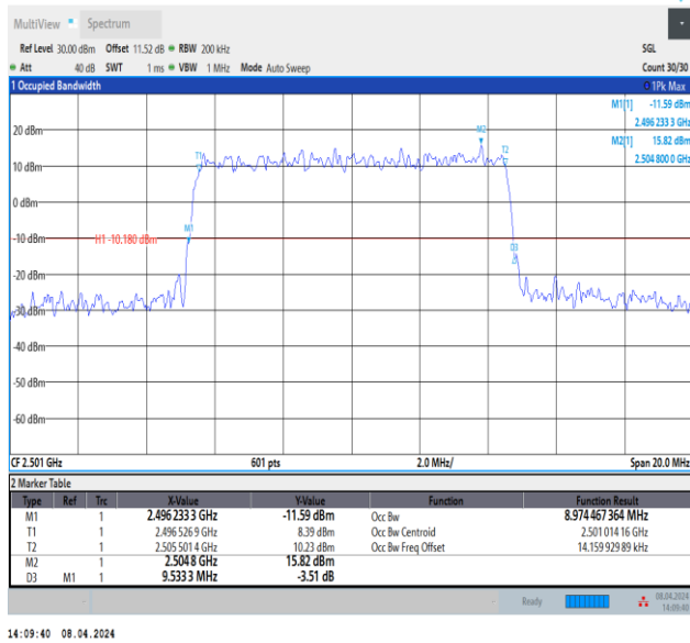
Band41-10MHz-16QAM-39700-50RB#0-PASS
