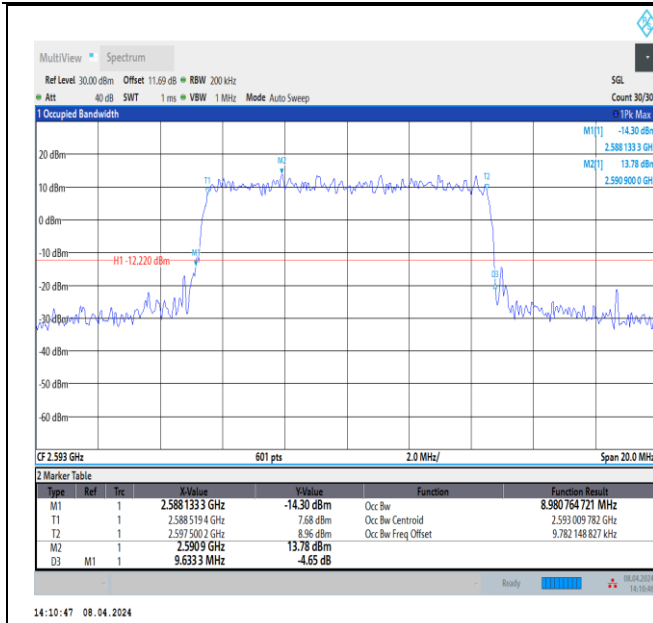
Band41-10MHz-64QAM-40620-50RB#0-PASS
