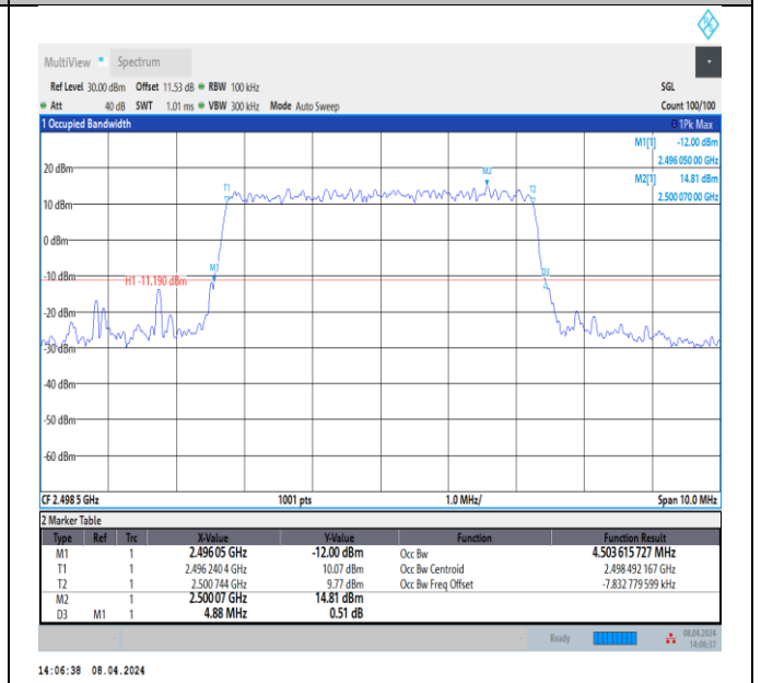
Band41-5MHz-16QAM-39675-25RB#0-PASS
