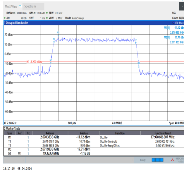
Band41-20MHz-QPSK-41490-100RB#0-PASS
