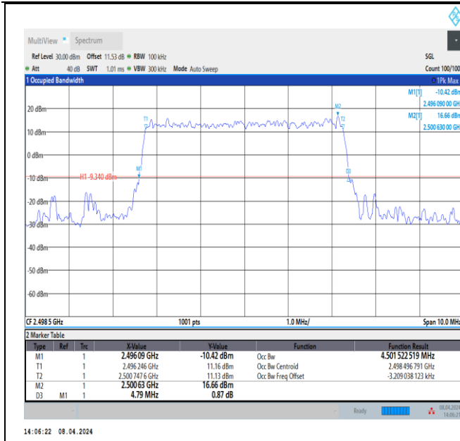
Band41-5MHz-QPSK-39675-25RB#0-PASS
