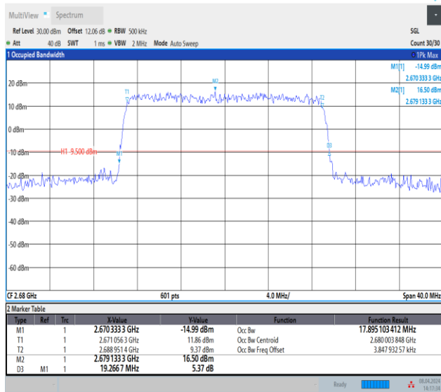
Band41-20MHz-16QAM-41490-100RB#0-PASS
