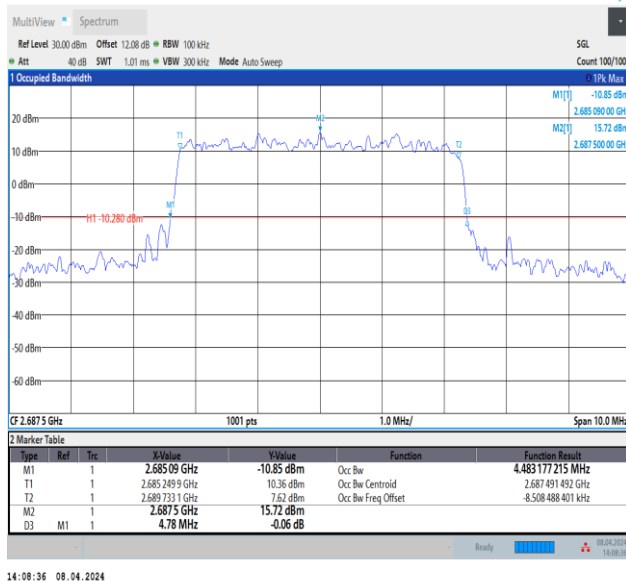
Band41-5MHz-64QAM-41565-25RB#0-PASS
