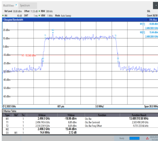
Band41-15MHz-64QAM-39725-75RB#0-PASS
