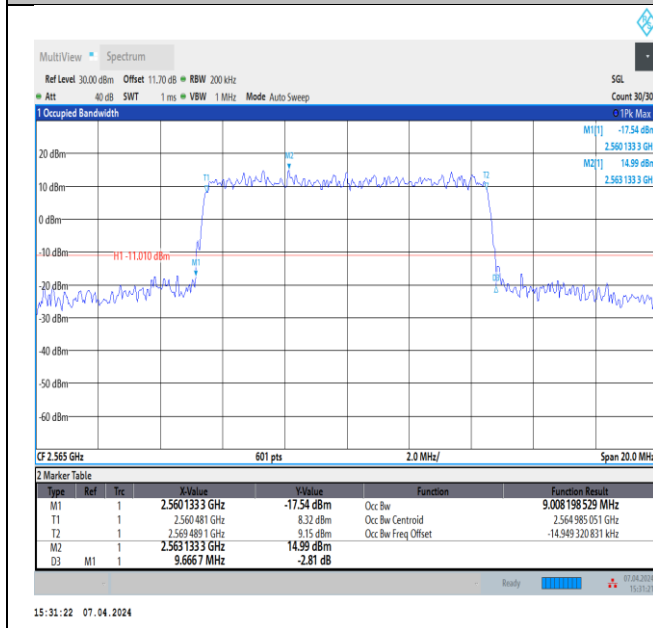
Band7-10MHz-16QAM-21400-50RB#0-PASS
