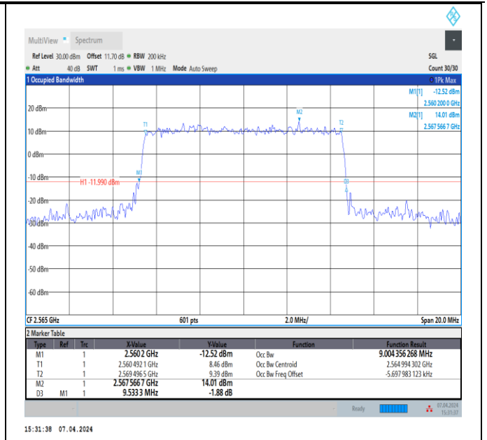
Band7-10MHz-64QAM-21400-50RB#0-PASS
