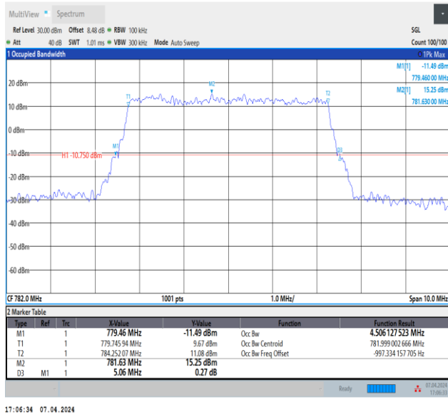
Band13-5MHz-16QAM-23230-25RB#0-PASS
