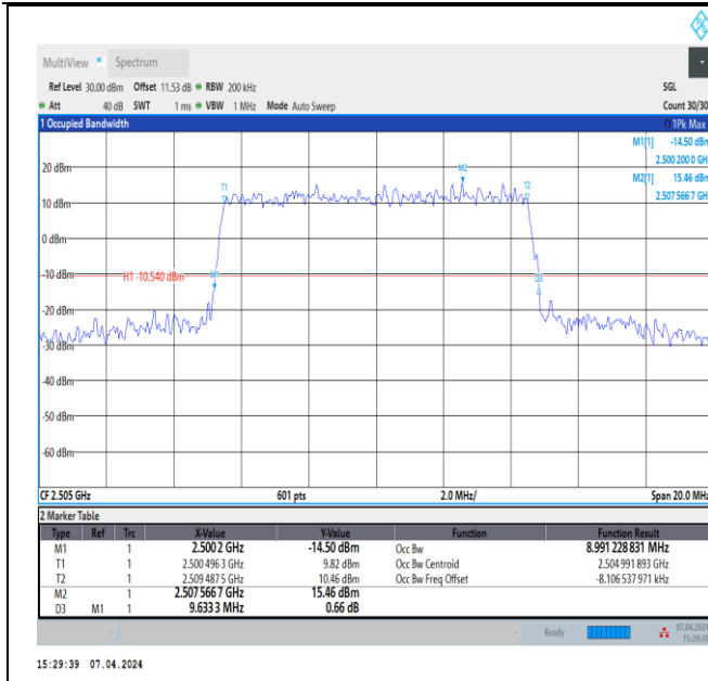
Band7-10MHz-16QAM-20800-50RB#0-PASS
