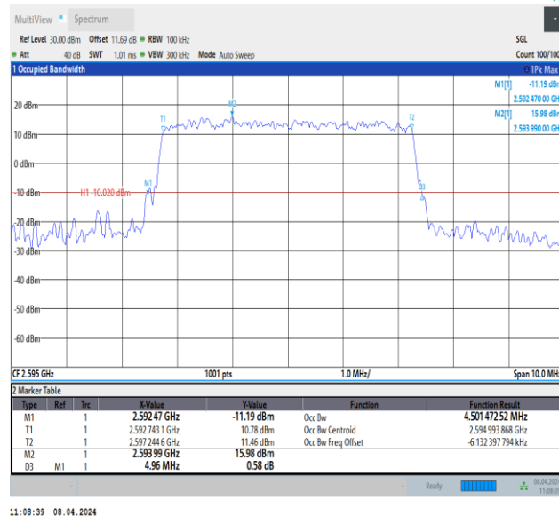
Band38-5MHz-QPSK-38000-25RB#0-PASS
