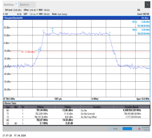
Band13-5MHz-16QAM-23255-25RB#0-PASS
