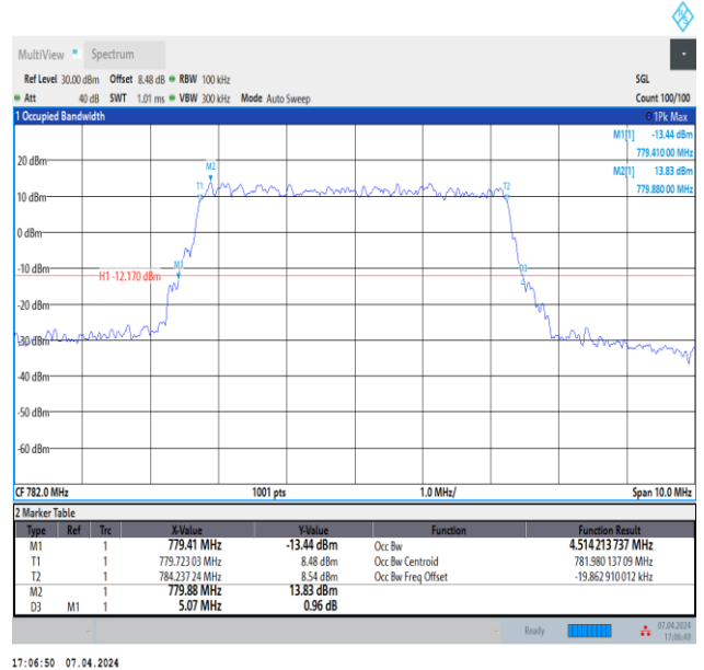
Band13-5MHz-64QAM-23230-25RB#0-PASS
