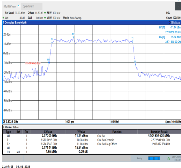
Band38-5MHz-QPSK-37775-25RB#0-PASS
