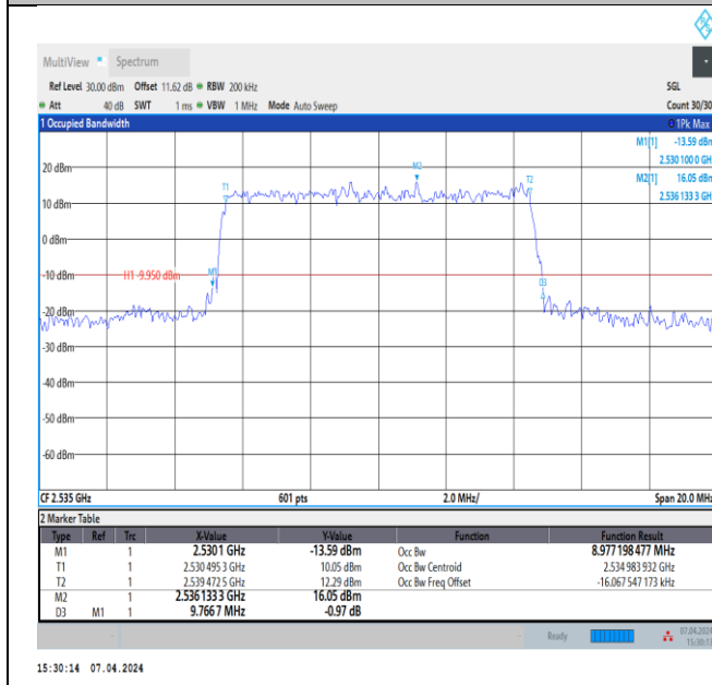
Band7-10MHz-QPSK-21100-50RB#0-PASS
