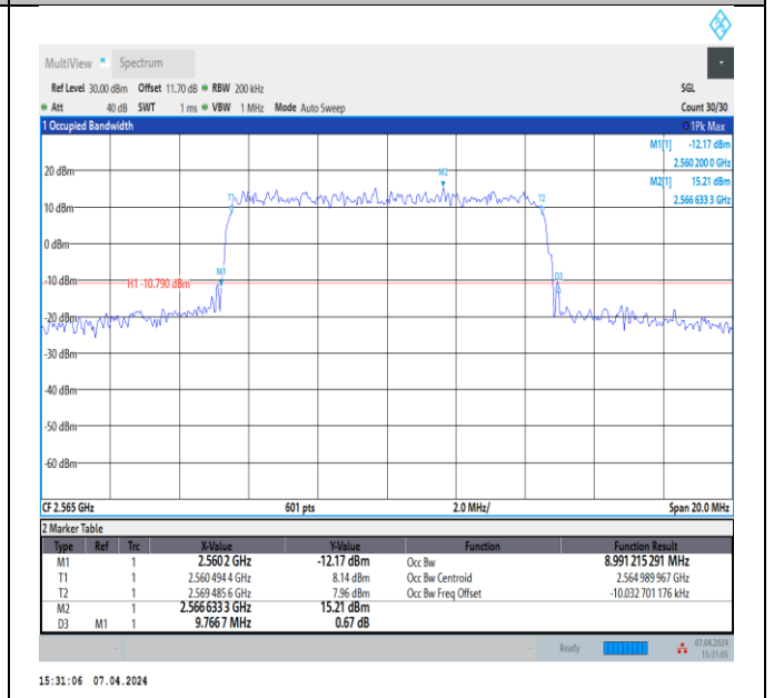
Band7-10MHz-QPSK-21400-50RB#0-PASS
