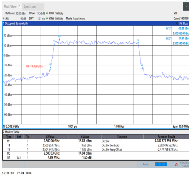
Band7-5MHz-QPSK-20775-25RB#0-PASS
