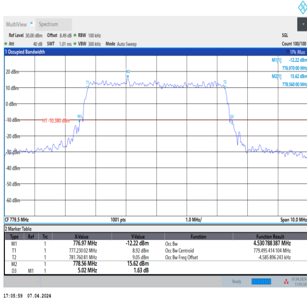
Band13-5MHz-64QAM-23205-25RB#0-PASS
