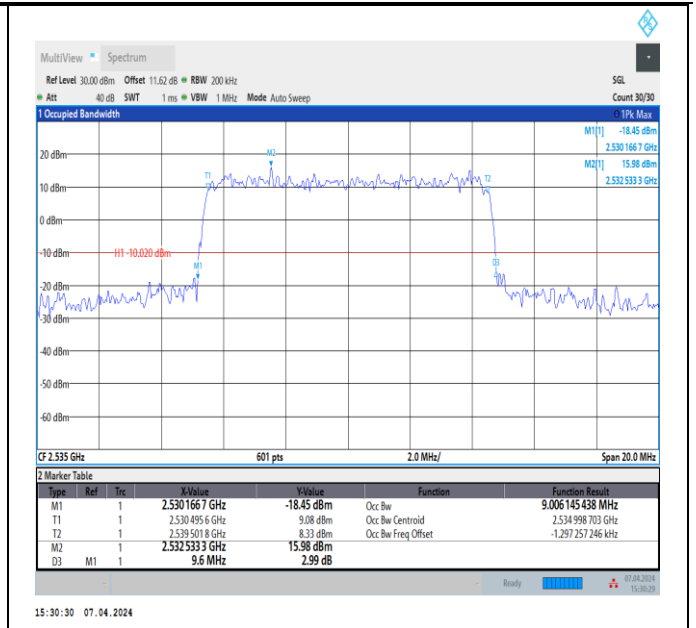
Band7-10MHz-16QAM-21100-50RB#0-PASS
