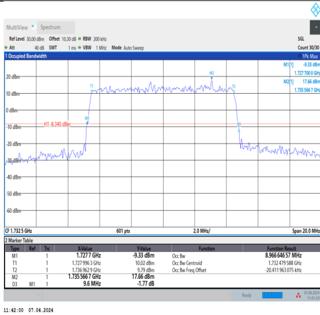
Band4-10MHz-QPSK-20175-50RB#0-PASS
