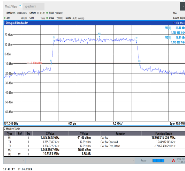
Band4-20MHz-QPSK-20300-100RB#0-PASS
