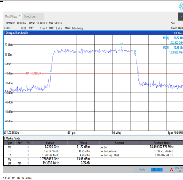
Band4-20MHz-16QAM-20175-100RB#0-PASS
