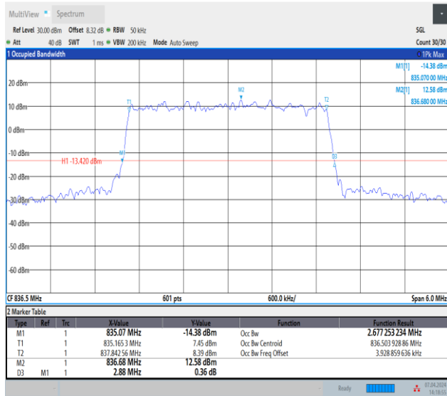
Band5-3MHz-64QAM-20525-15RB#0-PASS
