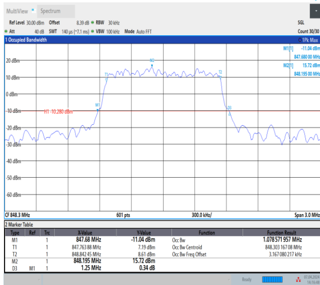
Band5-1.4MHz-64QAM-20643-6RB#0-PASS
