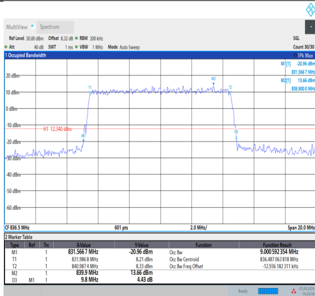
Band5-10MHz-16QAM-20600-50RB#0-PASS
