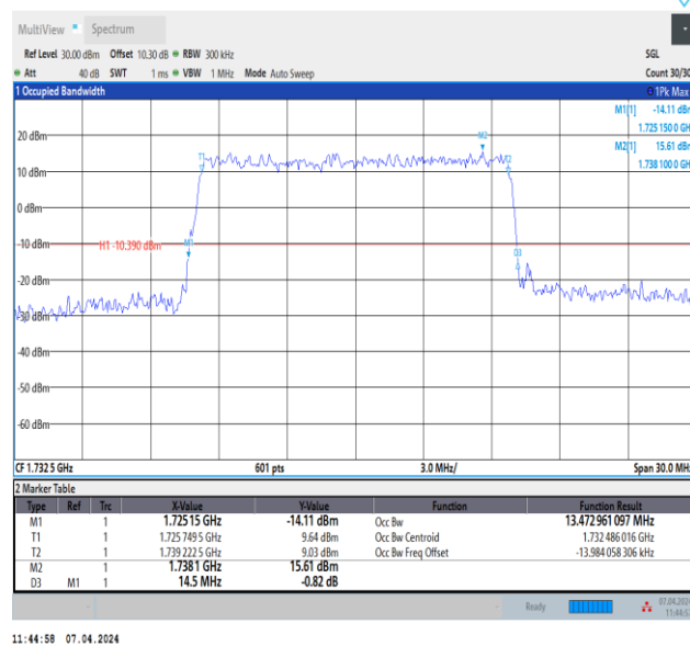
Band4-15MHz-QPSK-20175-75RB#0-PASS
