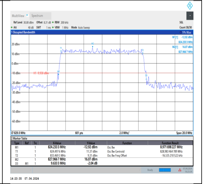
Band5-10MHz-QPSK-20450-50RB#0-PASS
