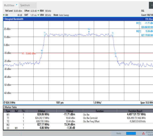
Band5-5MHz-16QAM-20425-25RB#0-PASS
