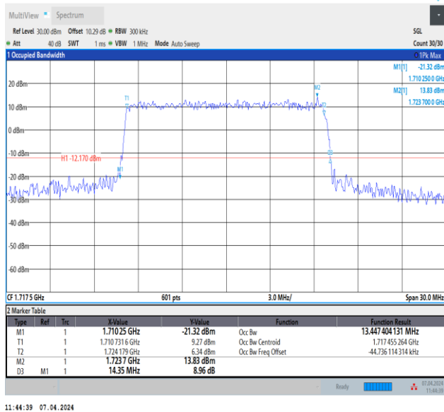
Band4-15MHz-64QAM-20025-75RB#0-PASS
