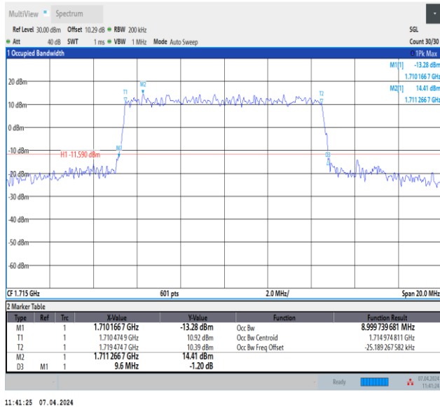
Band4-10MHz-16QAM-20000-50RB#0-PASS
