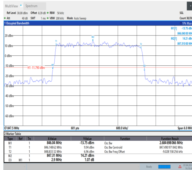
Band5-3MHz-64QAM-20635-15RB#0-PASS
