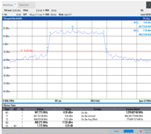
Band5-1.4MHz-QPSK-20643-6RB#0-PASS
