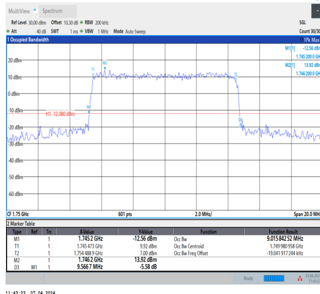
Band4-10MHz-64QAM-20350-50RB#0-PASS
