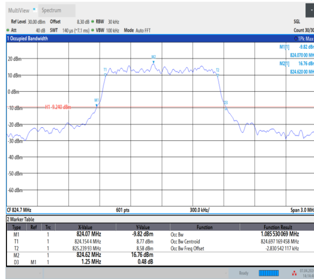
Band5-1.4MHz-16QAM-20407-6RB#0-PASS
