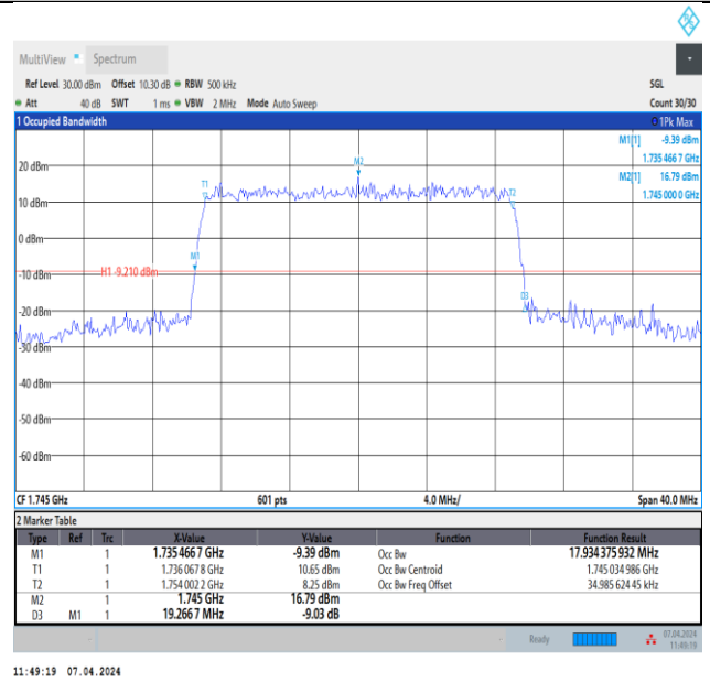
Band4-20MHz-64QAM-20300-100RB#0-PASS
