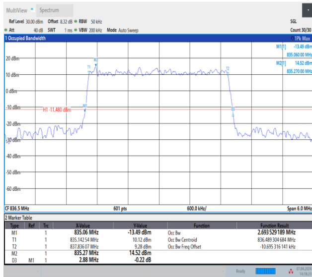
Band5-3MHz-QPSK-20525-15RB#0-PASS
