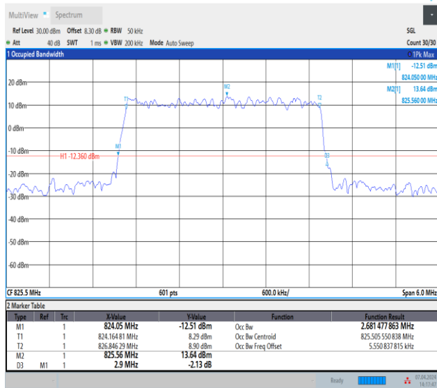
Band5-3MHz-16QAM-20415-15RB#0-PASS
