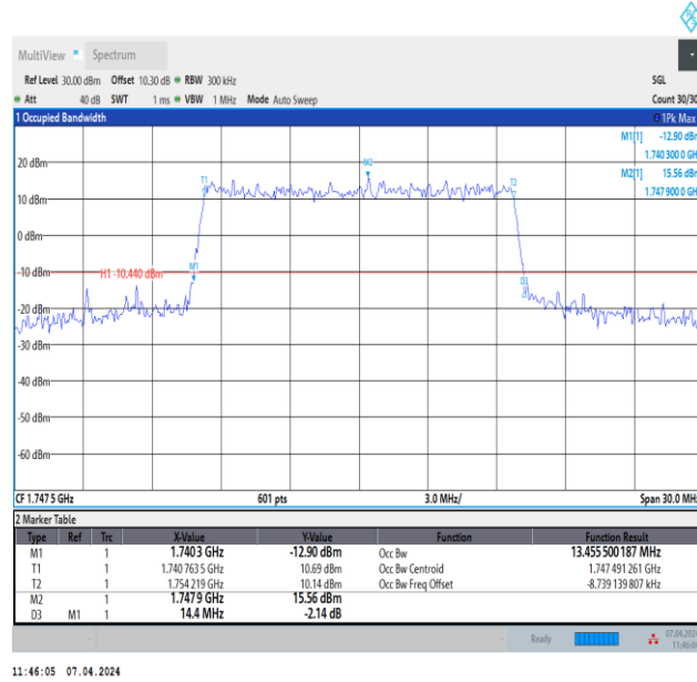
Band4-15MHz-16QAM-20325-75RB#0-PASS
