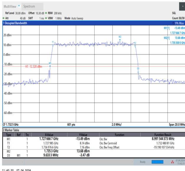
Band4-10MHz-64QAM-20175-50RB#0-PASS
