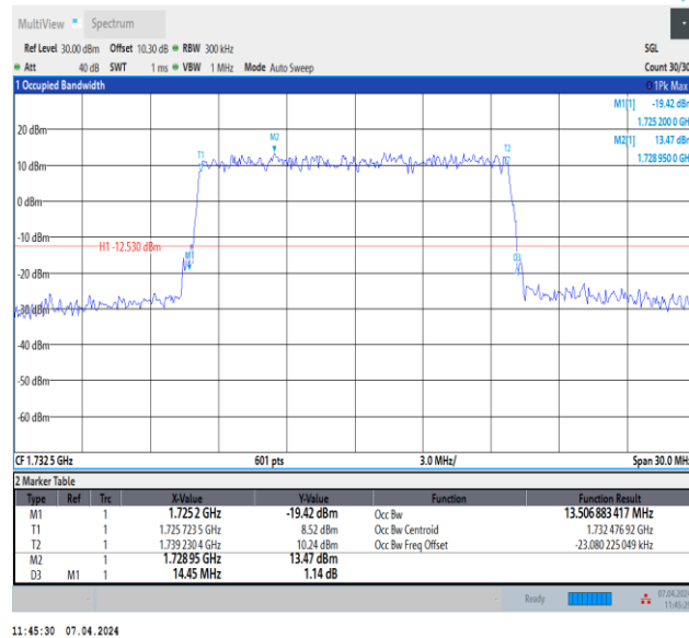
Band4-15MHz-64QAM-20175-75RB#0-PASS
