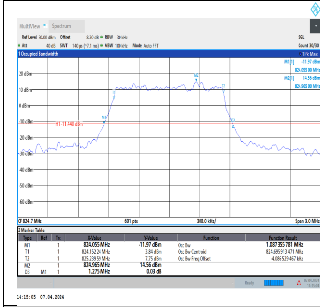
Band5-1.4MHz-64QAM-20407-6RB#0-PASS
