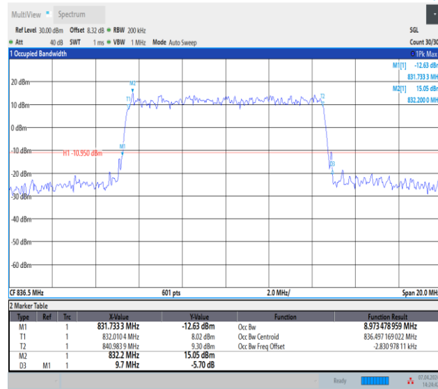
Band5-10MHz-16QAM-20525-50RB#0-PASS
