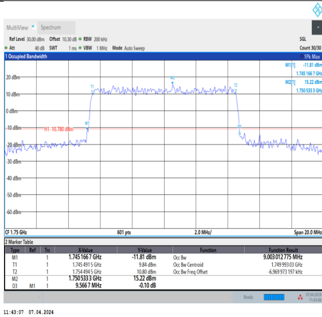
Band4-10MHz-16QAM-20350-50RB#0-PASS
