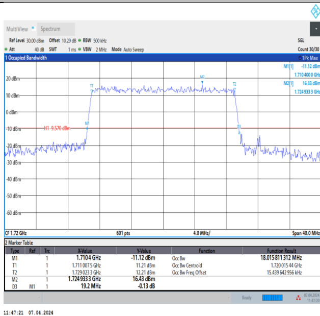
Band4-20MHz-16QAM-20050-100RB#0-PASS
