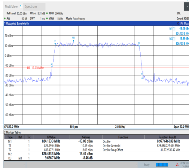
Band5-10MHz-64QAM-20450-50RB#0-PASS
