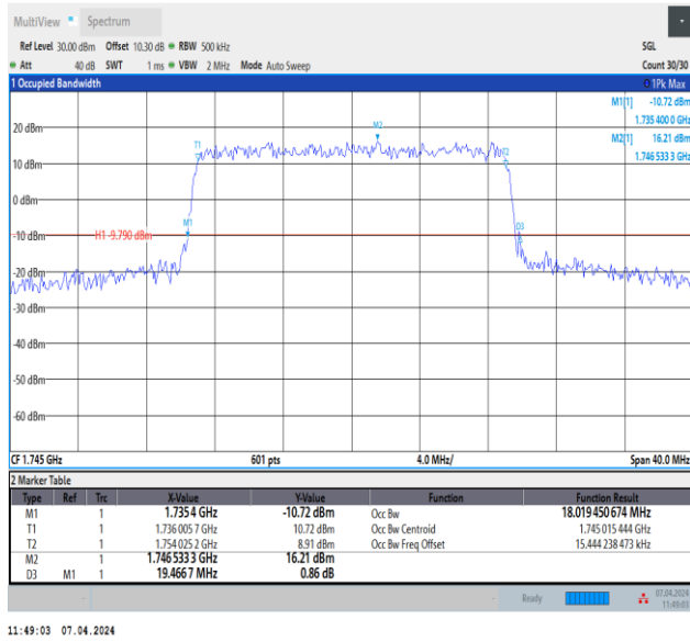
Band4-20MHz-16QAM-20300-100RB#0-PASS
