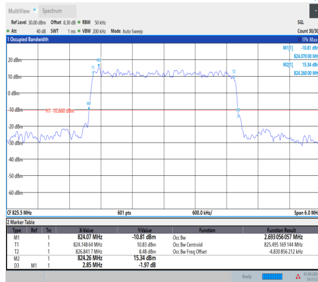
Band5-3MHz-QPSK-20415-15RB#0-PASS
