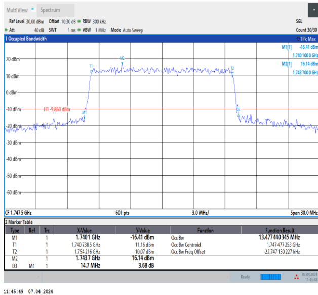
Band4-15MHz-QPSK-20325-75RB#0-PASS
