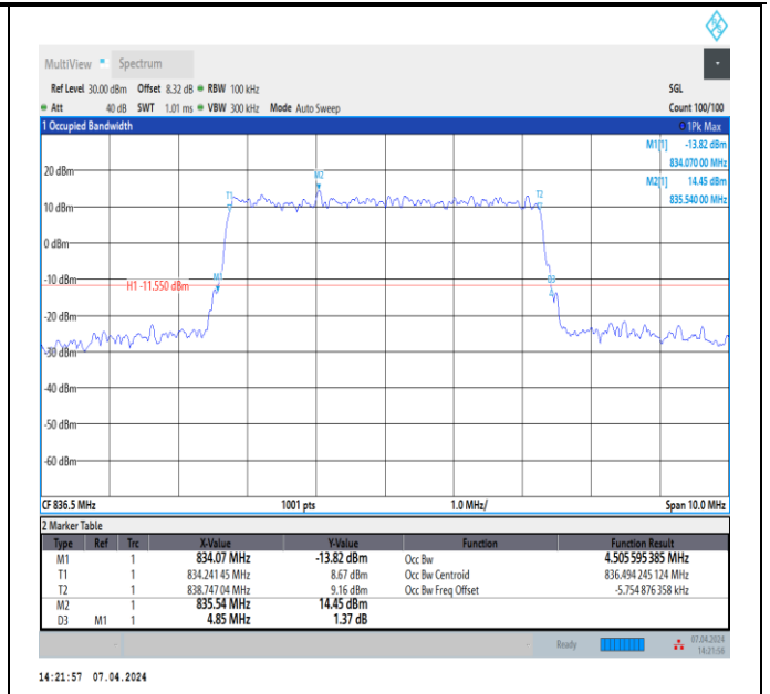
Band5-5MHz-64QAM-20525-25RB#0-PASS
