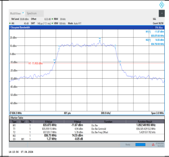
Band5-1.4MHz-64QAM-20525-6RB#0-PASS
