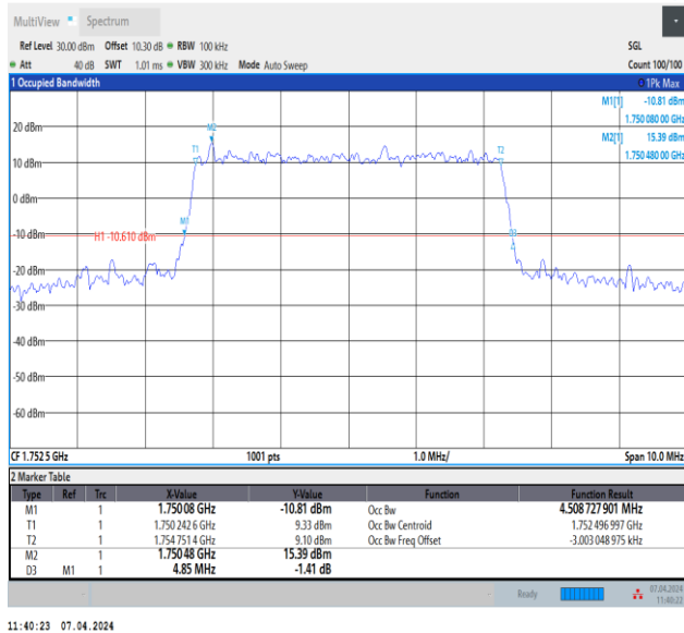
Band4-5MHz-64QAM-20375-25RB#0-PASS
