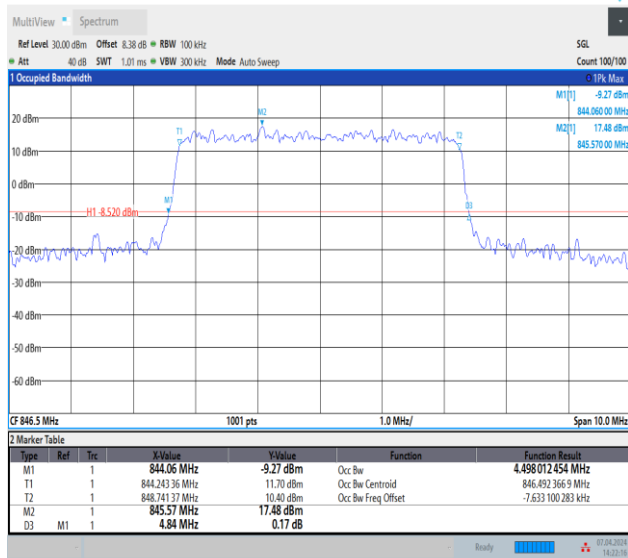
Band5-5MHz-QPSK-20625-25RB#0-PASS
