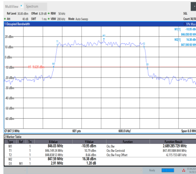
Band5-3MHz-QPSK-20635-15RB#0-PASS
