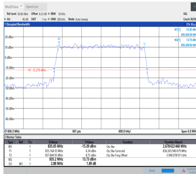
Band5-3MHz-16QAM-20525-15RB#0-PASS
