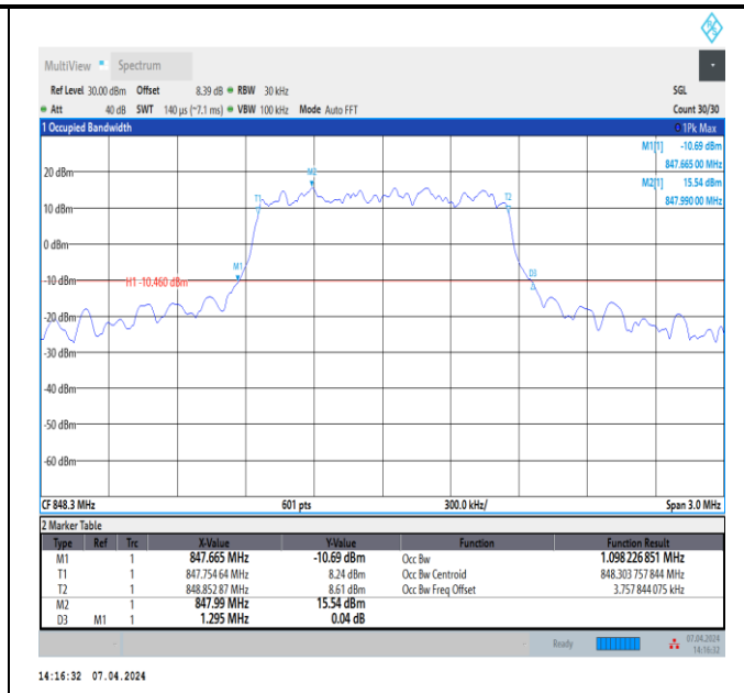
Band5-1.4MHz-16QAM-20643-6RB#0-PASS
