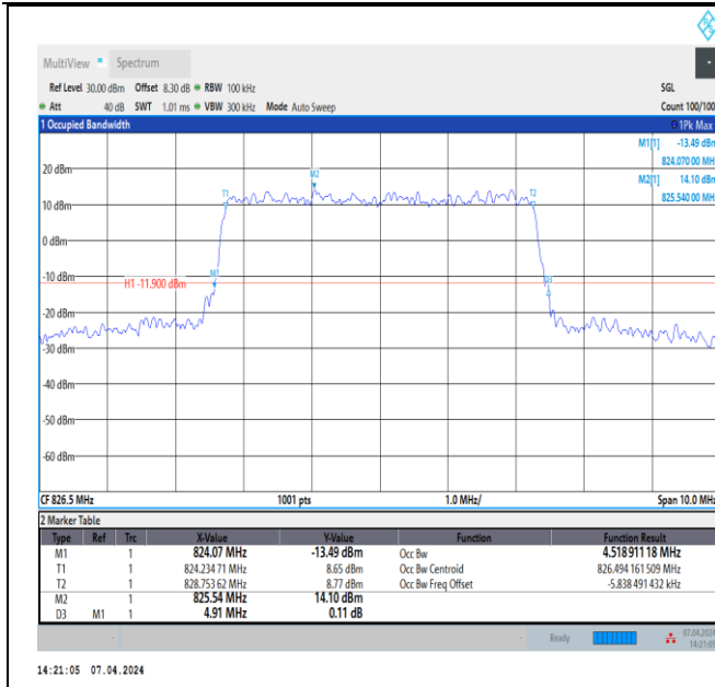
Band5-5MHz-64QAM-20425-25RB#0-PASS
