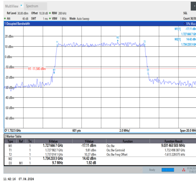
Band4-10MHz-16QAM-20175-50RB#0-PASS
