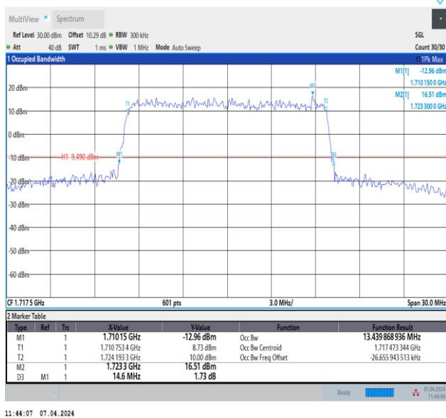
Band4-15MHz-QPSK-20025-75RB#0-PASS
