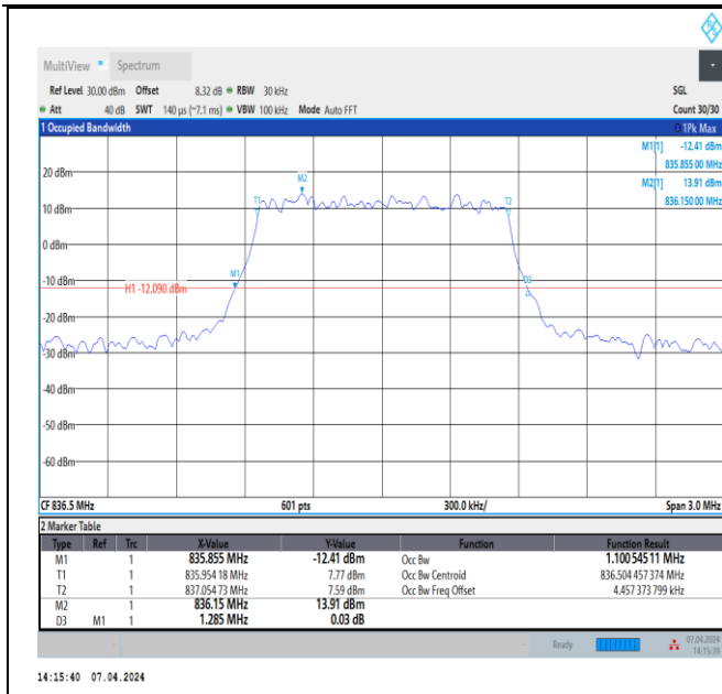
Band5-1.4MHz-16QAM-20525-6RB#0-PASS
