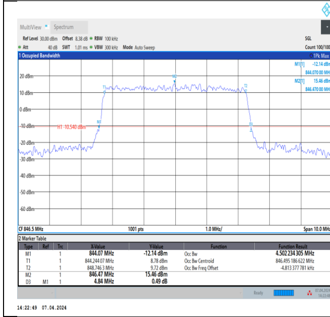
Band5-5MHz-64QAM-20625-25RB#0-PASS
