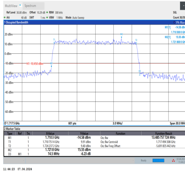
Band4-15MHz-16QAM-20025-75RB#0-PASS
