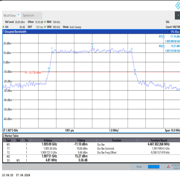
Band2-5MHz-64QAM-19175-25RB#0-PASS
