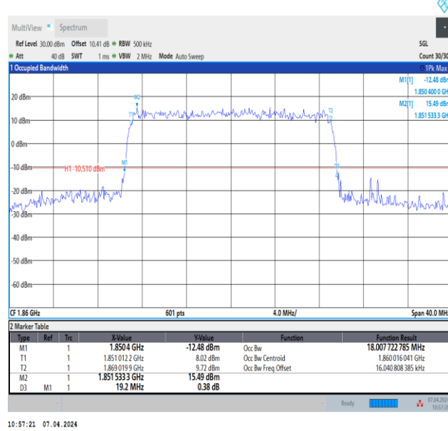
Band2-20MHz-64QAM-18700-100RB#0-PASS
