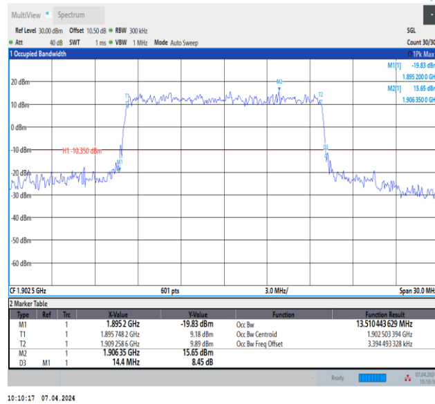
Band2-15MHz-16QAM-19125-75RB#0-PASS
