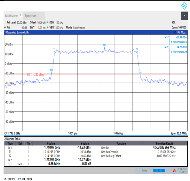
Band4-5MHz-16QAM-19975-25RB#0-PASS
