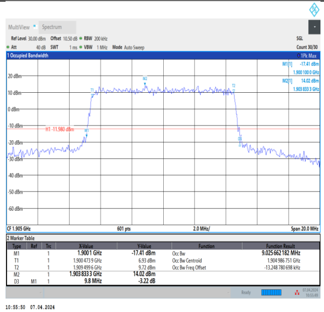
Band2-10MHz-64QAM-19150-50RB#0-PASS
