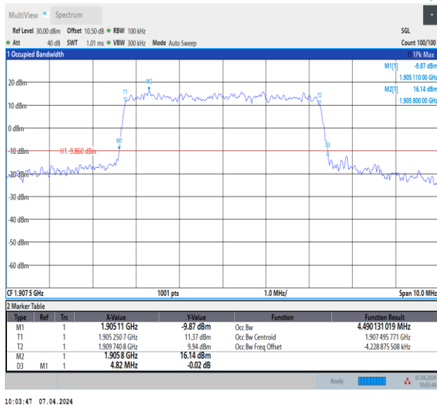
Band2-5MHz-QPSK-19175-25RB#0-PASS
