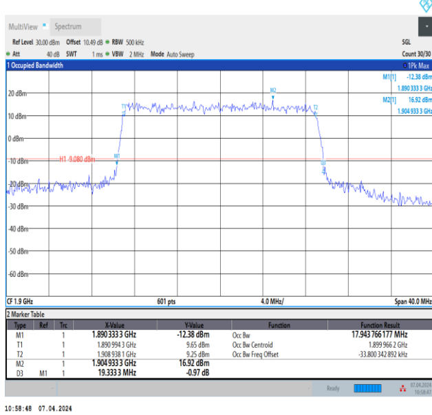
Band2-20MHz-16QAM-19100-100RB#0-PASS
