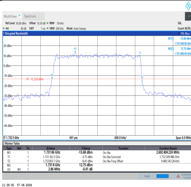
Band4-3MHz-64QAM-20175-15RB#0-PASS
