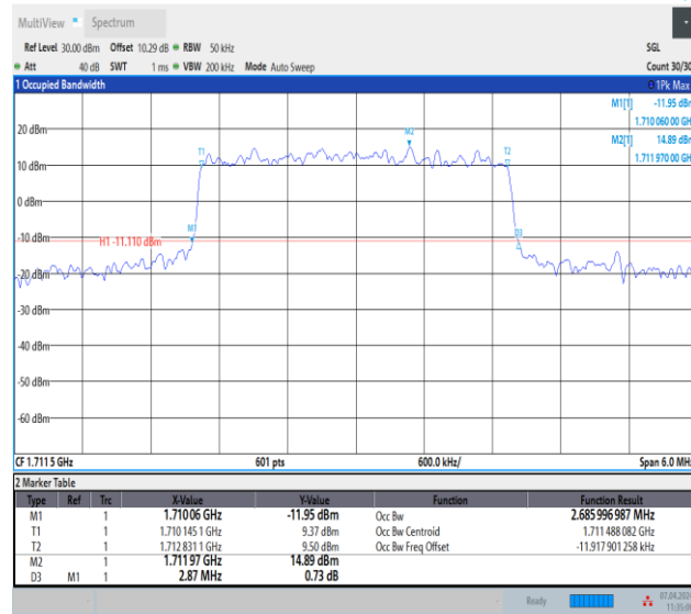
Band4-3MHz-QPSK-19965-15RB#0-PASS
