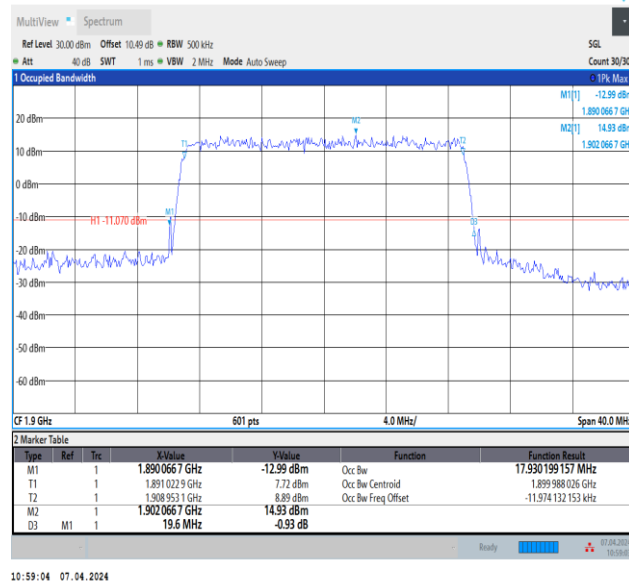
Band2-20MHz-64QAM-19100-100RB#0-PASS
