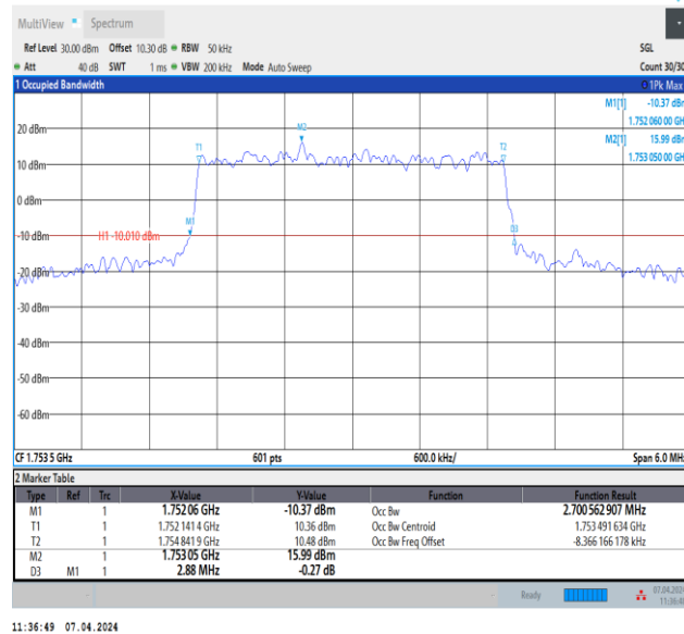
Band4-3MHz-QPSK-20385-15RB#0-PASS
