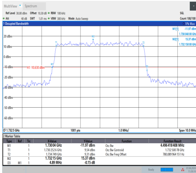
Band4-5MHz-16QAM-20175-25RB#0-PASS
