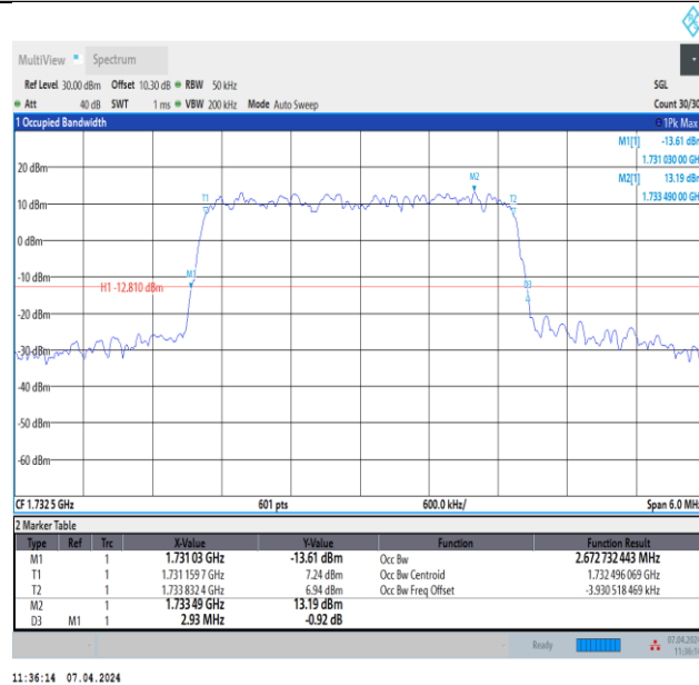
Band4-3MHz-16QAM-20175-15RB#0-PASS
