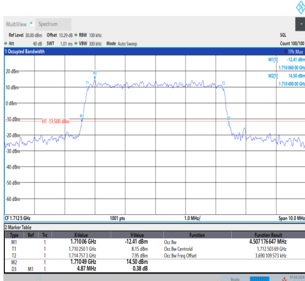
Band4-5MHz-16QAM-20175-25RB#0-PASS
