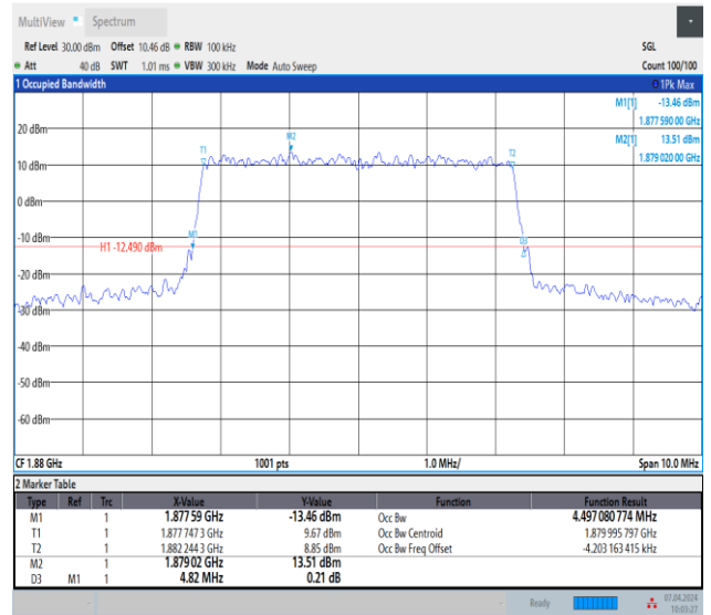
Band2-5MHz-64QAM-18900-25RB#0-PASS
