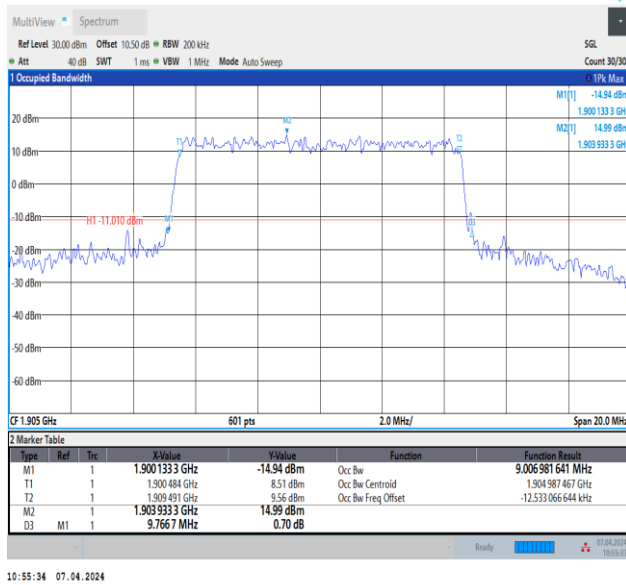
Band2-10MHz-16QAM-19150-50RB#0-PASS
