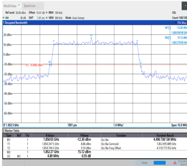
Band2-5MHz-64QAM-18625-25RB#0-PASS
