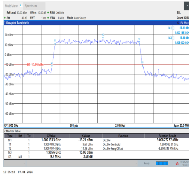
Band2-10MHz-QPSK-19150-50RB#0-PASS
