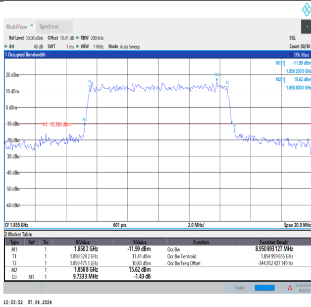
Band2-10MHz-16QAM-18650-50RB#0-PASS
