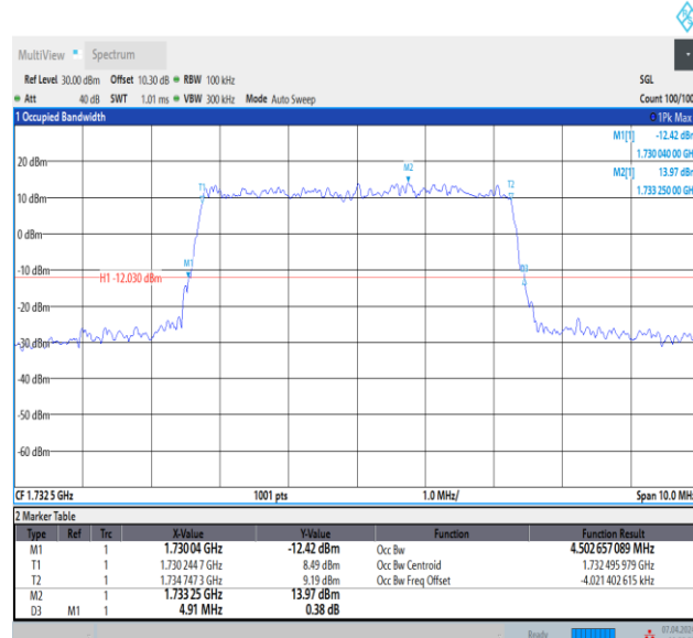
Band4-5MHz-16QAM-20375-25RB#0-PASS
