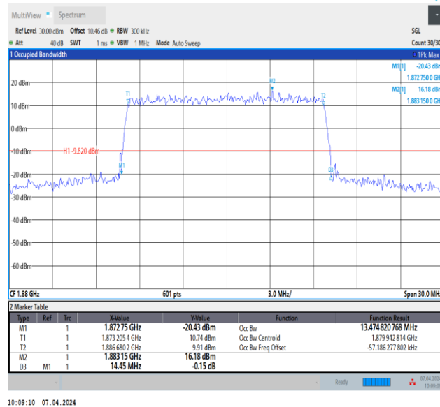
Band2-15MHz-QPSK-18900-75RB#0-PASS
