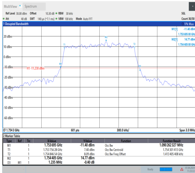
Band4-1.4MHz-64QAM-20393-6RB#0-PASS
