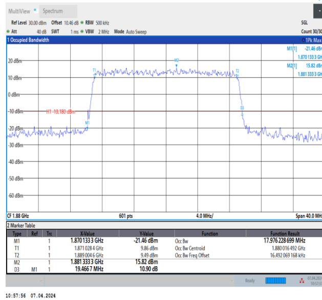
Band2-20MHz-16QAM-18900-100RB#0-PASS
