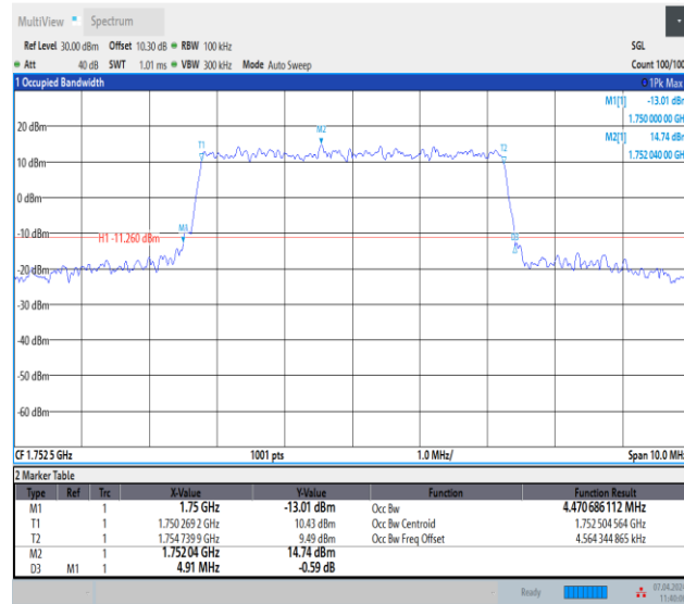
Band4-5MHz-16QAM-20375-25RB#0-PASS
