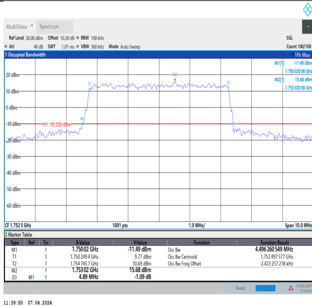
Band4-5MHz-QPSK-20375-25RB#0-PASS
