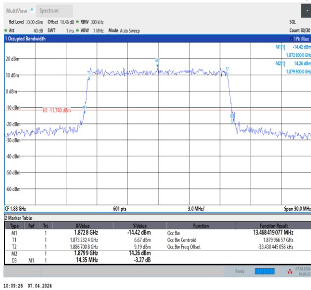
Band2-15MHz-16QAM-18900-75RB#0-PASS
