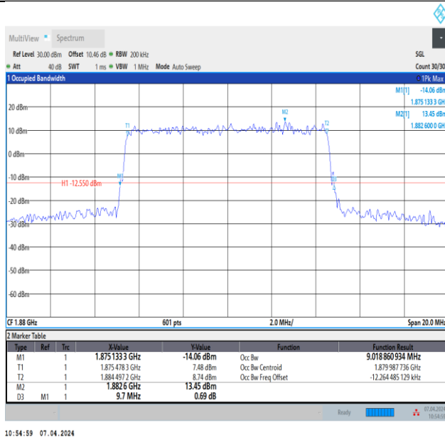
Band2-10MHz-64QAM-18900-50RB#0-PASS
