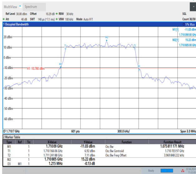
Band4-1.4MHz-64QAM-19957-6RB#0-PASS
