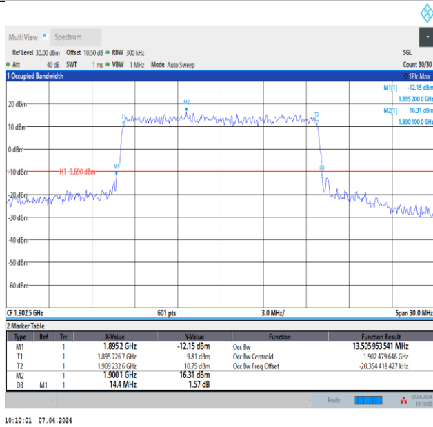
Band2-15MHz-QPSK-19125-75RB#0-PASS
