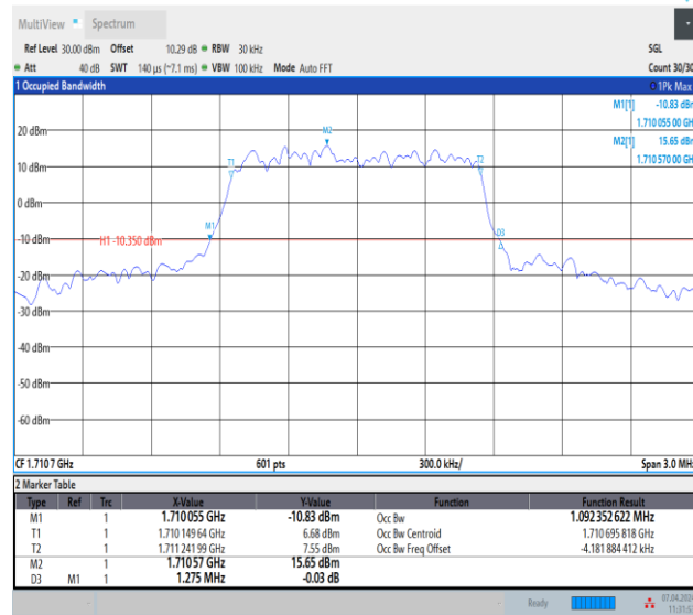
Band4-1.4MHz-16QAM-19957-6RB#0-PASS
