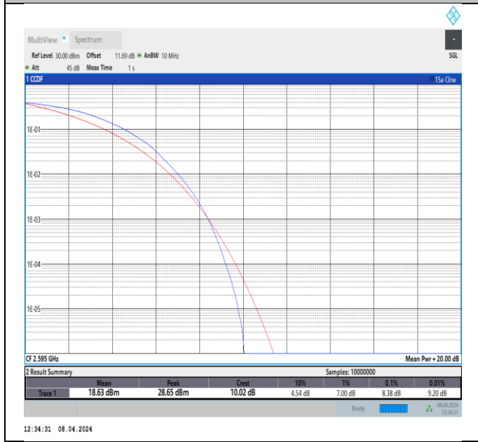
Band38-10MHz-64QAM-38000-50RB#0-PASS
