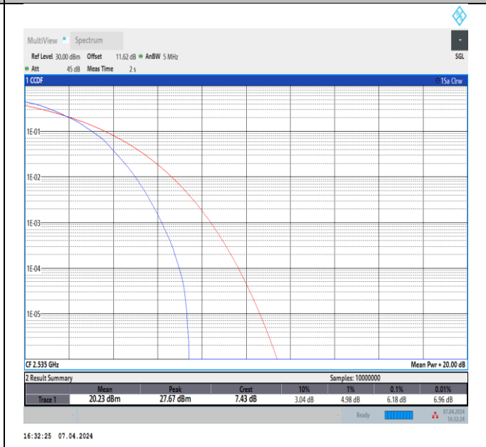
Band7-5MHz-64QAM-21100-25RB#0-PASS
