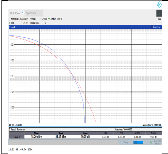
Band38-5MHz-64QAM-37775-25RB#0-PASS
