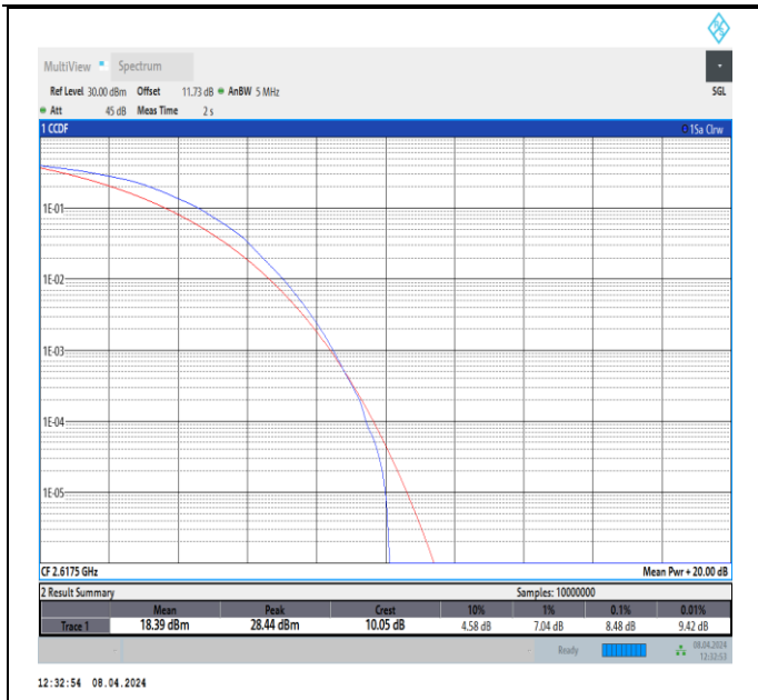
Band38-5MHz-64QAM-38225-25RB#0-PASS
