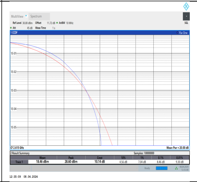
Band38-10MHz-64QAM-38200-50RB#0-PASS
