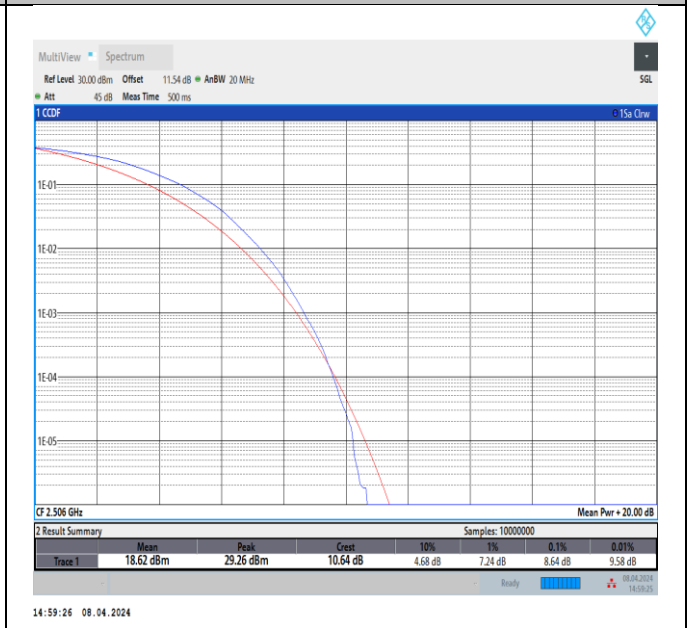
Band41-20MHz-64QAM-39750-100RB#0-PASS
