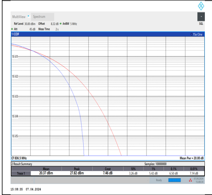
Band5-3MHz-64QAM-20525-15RB#0-PASS
