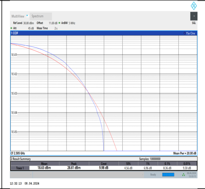
Band38-5MHz-64QAM-38000-25RB#0-PASS
