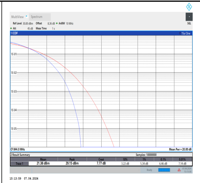
Band5-10MHz-64QAM-20600-50RB#0-PASS
