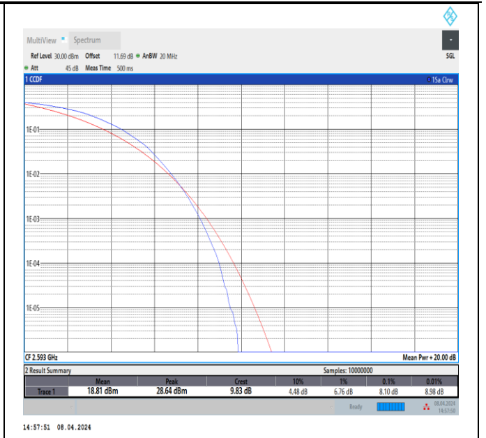
Band41-15MHz-64QAM-40620-75RB#0-PASS
