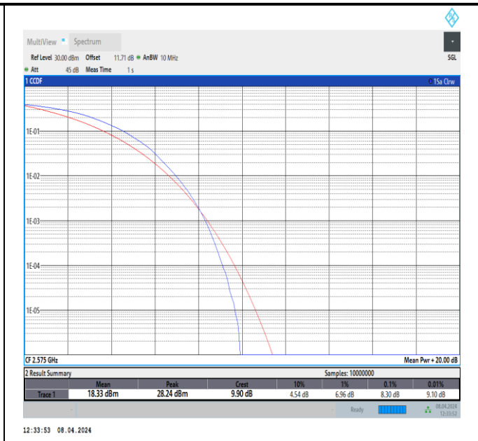
Band38-10MHz-64QAM-37800-50RB#0-PASS
