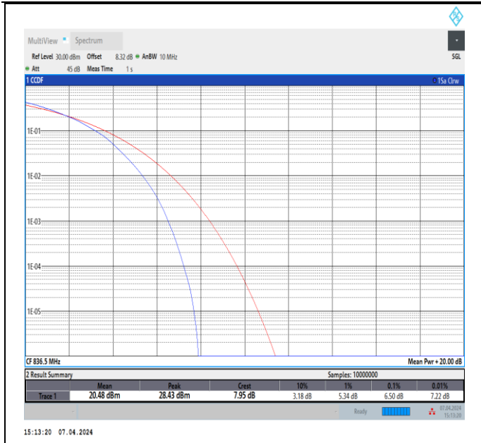
Band5-10MHz-64QAM-20525-50RB#0-PASS
