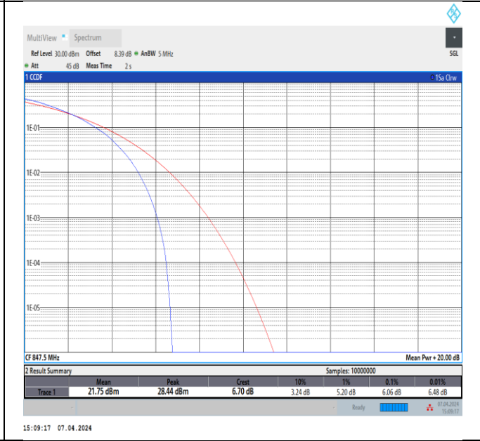
Band5-3MHz-64QAM-20635-15RB#0-PASS
