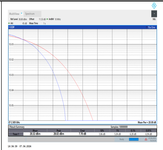
Band7-10MHz-64QAM-20800-50RB#0-PASS
