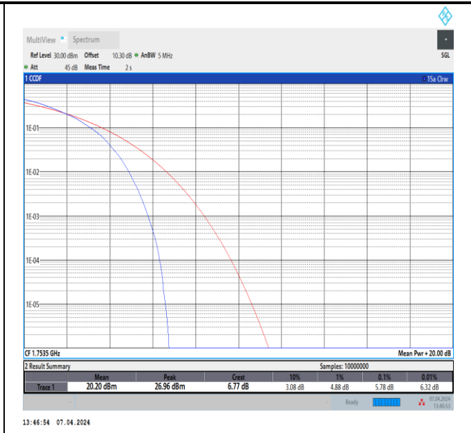
Band4-3MHz-64QAM-20385-15RB#0-PASS
