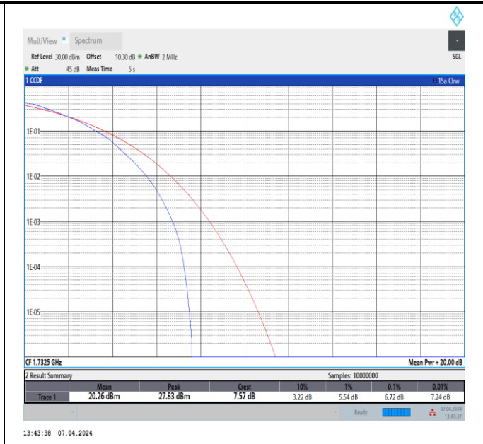
Band4-1.4MHz-64QAM-20175-6RB#0-PASS
