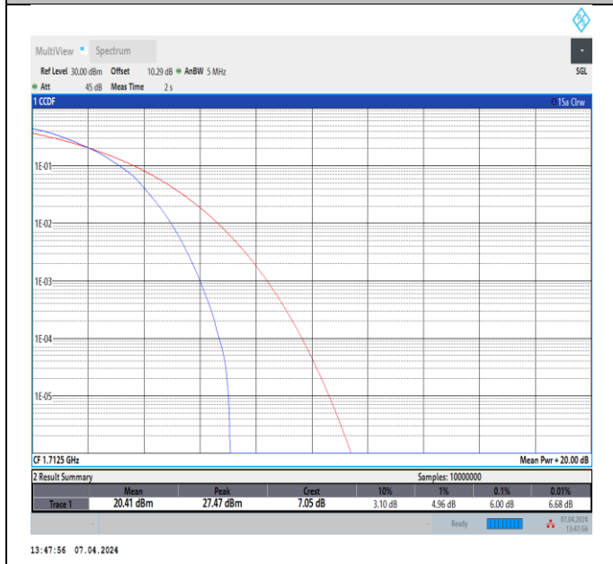
Band4-5MHz-64QAM-19975-25RB#0-PASS
