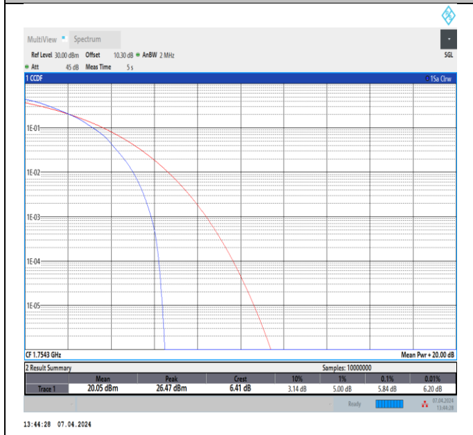
Band4-1.4MHz-64QAM-20393-6RB#0-PASS
