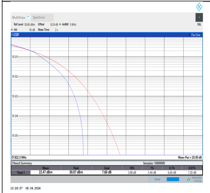
26(814-824)-3MHz-16QAM-26775-15RB#0-PASS
