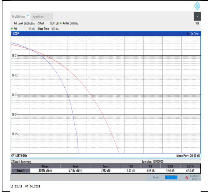
Band2-15MHz-64QAM-18675-75RB#0-PASS
