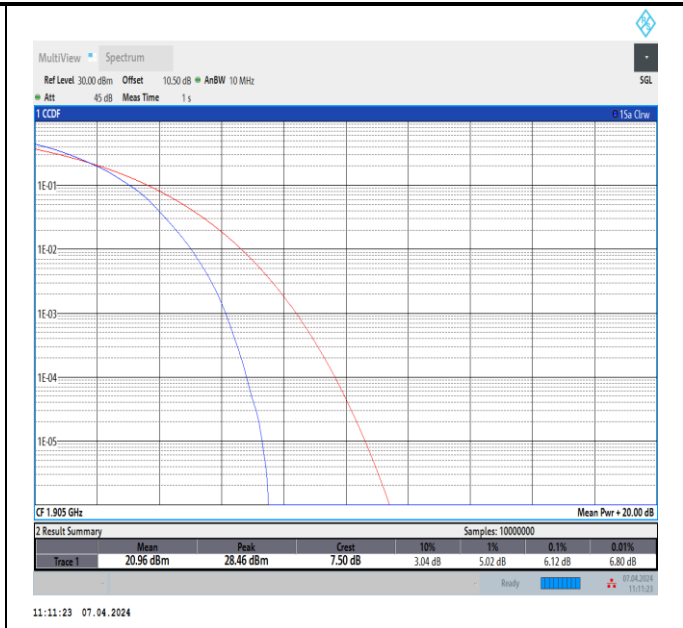
Band2-10MHz-64QAM-19150-50RB#0-PASS
