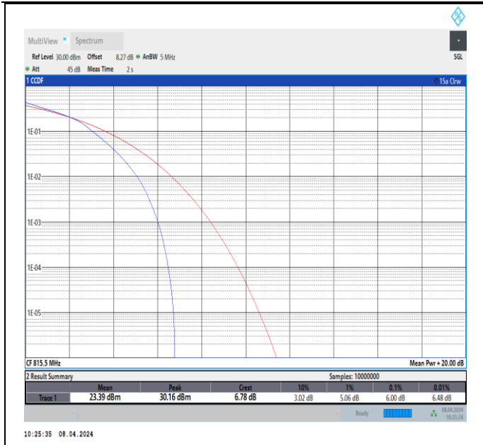
26(814-824)-3MHz-16QAM-26705-15RB#0-PASS
