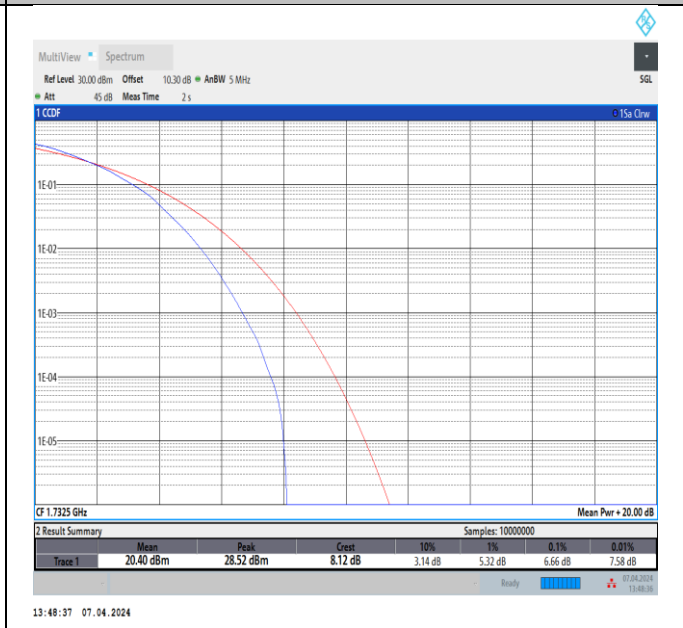
Band4-5MHz-64QAM-20175-25RB#0-PASS
