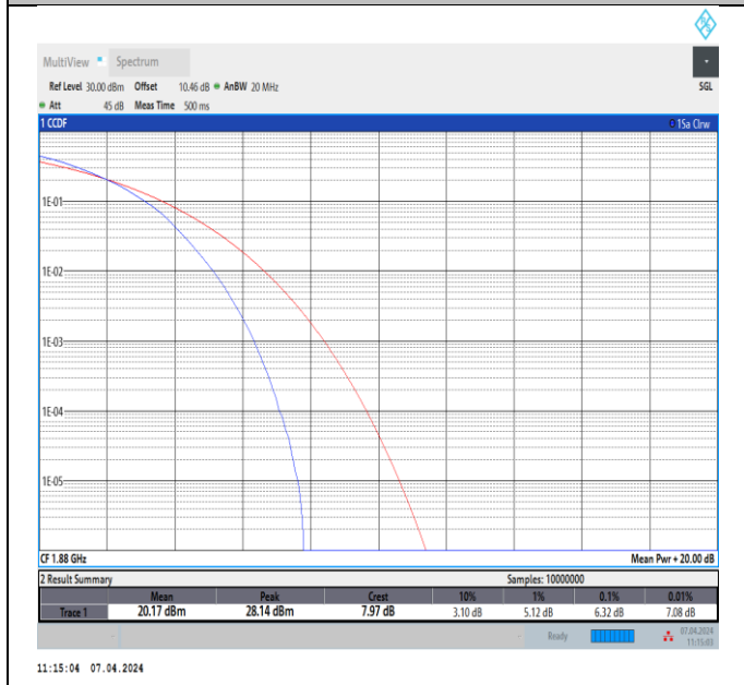
Band2-20MHz-64QAM-18900-100RB#0-PASS
