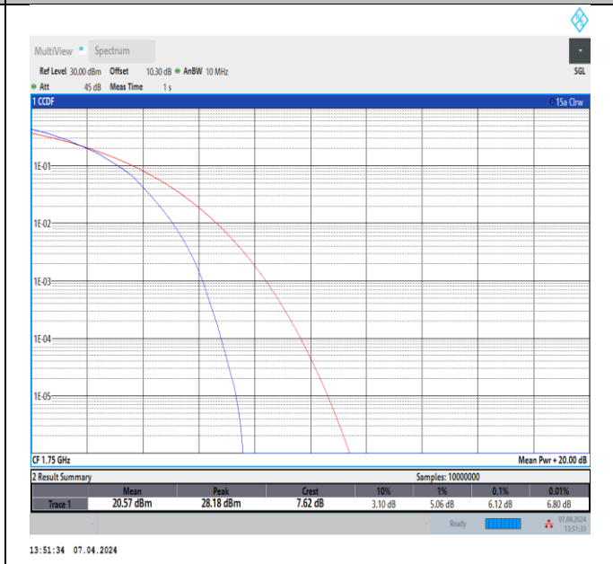
Band4-10MHz-64QAM-20350-50RB#0-PASS
