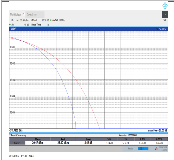
Band4-10MHz-64QAM-20175-50RB#0-PASS
