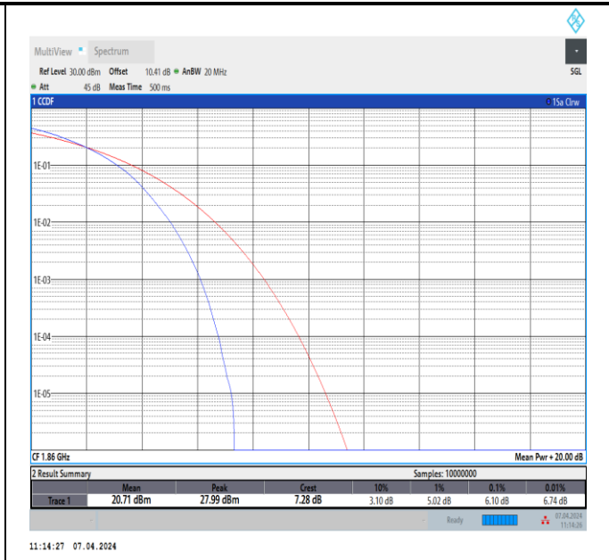
Band2-20MHz-64QAM-18700-100RB#0-PASS
