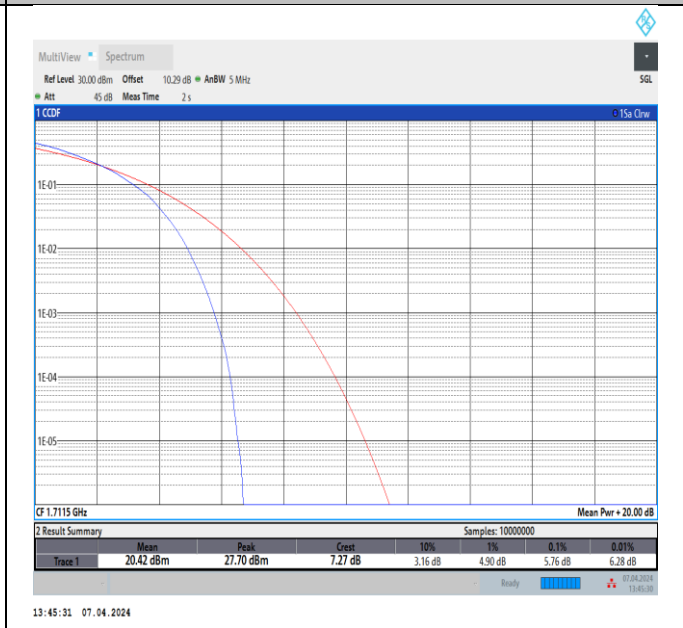
Band4-3MHz-64QAM-19965-15RB#0-PASS
