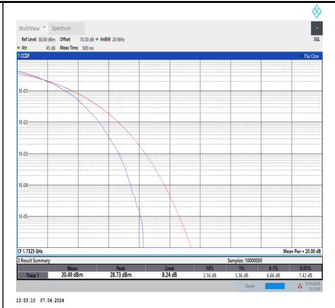
Band4-15MHz-64QAM-20175-75RB#0-PASS
