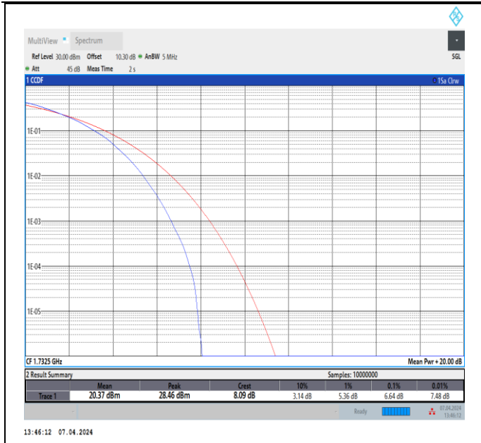
Band4-3MHz-64QAM-20175-15RB#0-PASS
