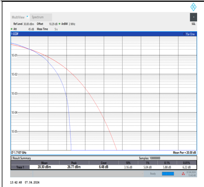
Band4-1.4MHz-64QAM-19957-6RB#0-PASS
