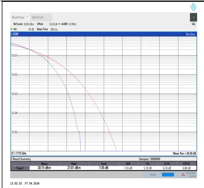
Band4-15MHz-64QAM-20025-75RB#0-PASS
