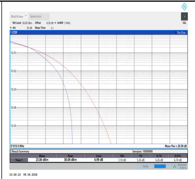
26(814-824)-3MHz-16QAM-26740-15RB#0-PASS
