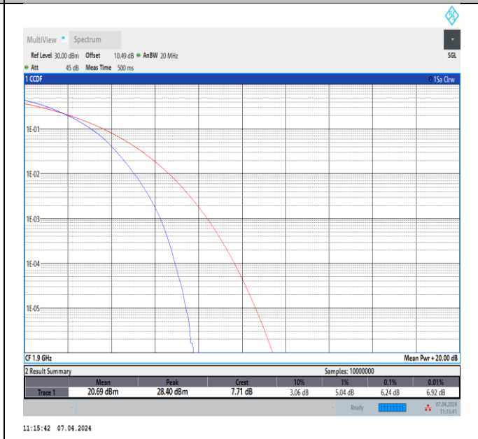
Band2-20MHz-64QAM-19100-100RB#0-PASS
