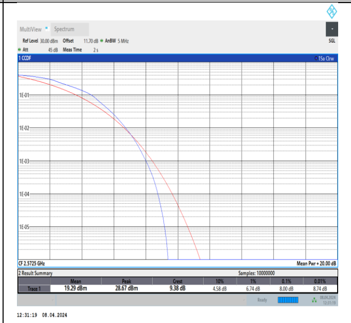
Band38-5MHz-16QAM-37775-25RB#0-PASS
