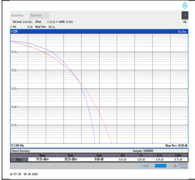
Band41-15MHz-16QAM-40620-75RB#0-PASS
