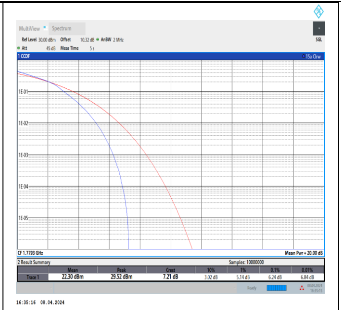
Band66-1.4MHz-16QAM-132665-6RB#0-PASS
