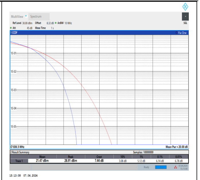
Band5-10MHz-16QAM-20525-50RB#0-PASS
