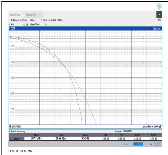
Band41-10MHz-16QAM-41540-50RB#0-PASS
