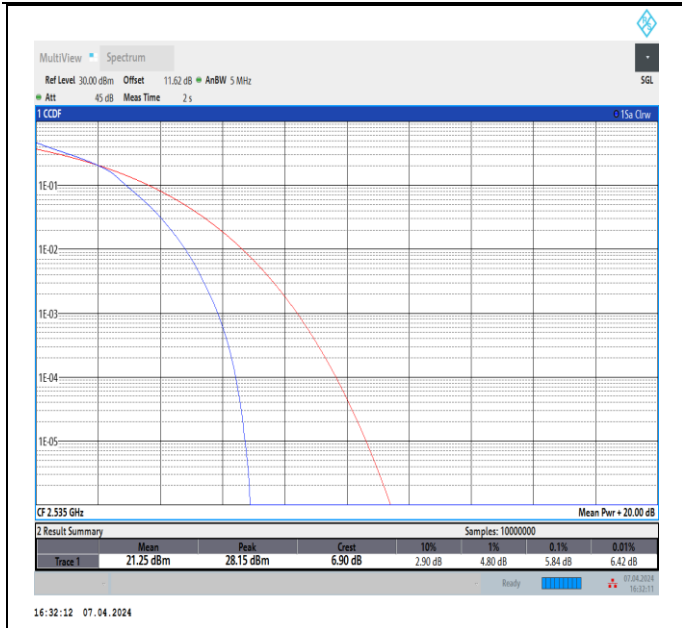
Band7-5MHz-16QAM-21100-25RB#0-PASS
