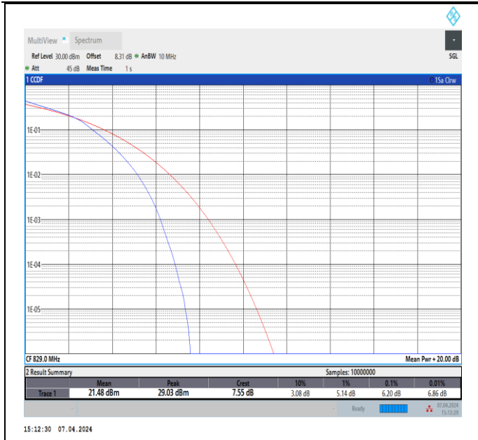
Band5-10MHz-16QAM-20450-50RB#0-PASS
