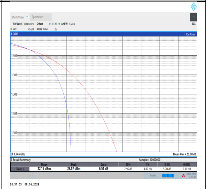
Band66-3MHz-16QAM-132322-15RB#0-PASS
