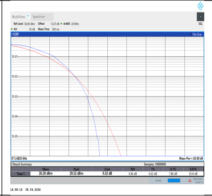
Band41-15MHz-16QAM-41515-75RB#0-PASS
