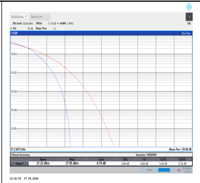
Band7-5MHz-16QAM-21425-25RB#0-PASS
