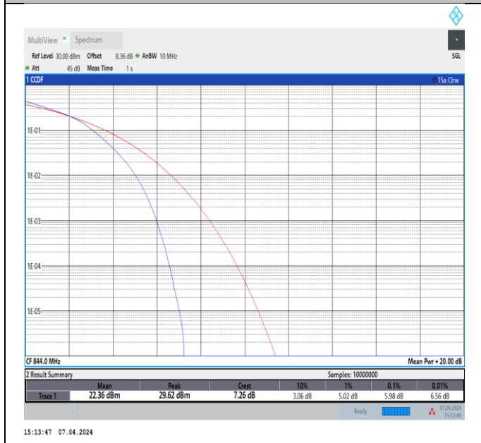
Band5-10MHz-16QAM-20600-50RB#0-PASS
