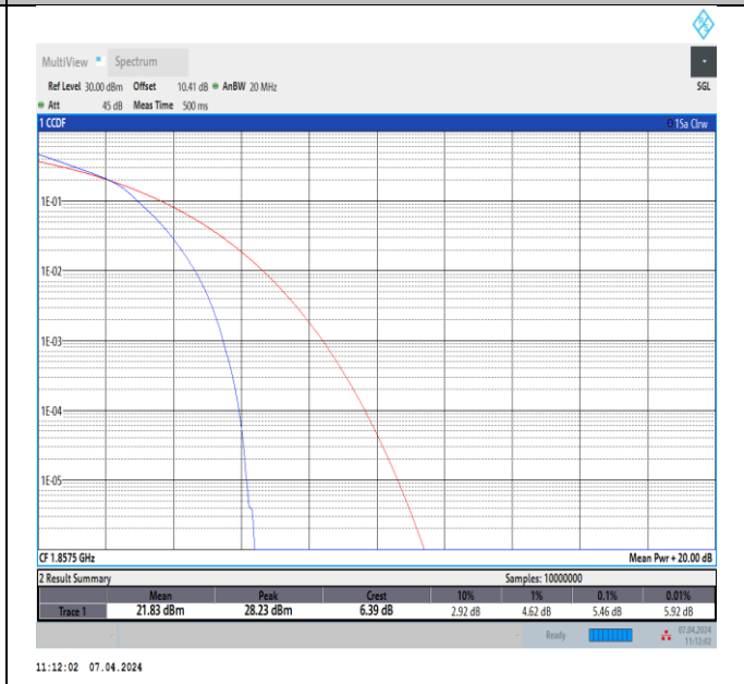
Band2-15MHz-16QAM-18675-75RB#0-PASS
