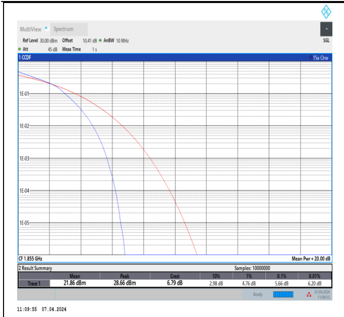
Band2-10MHz-16QAM-18650-50RB#0-PASS
