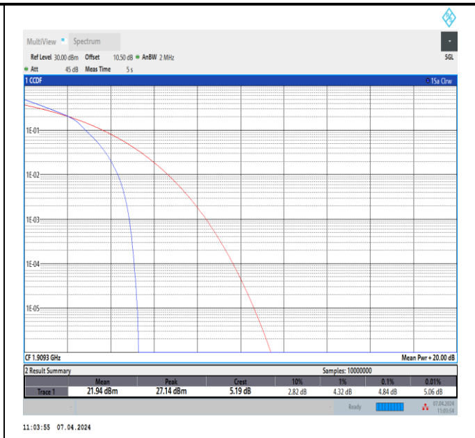
Band2-1.4MHz-16QAM-19193-6RB#0-PASS
