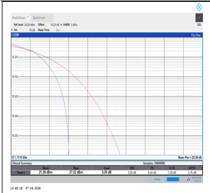
Band4-3MHz-16QAM-19965-15RB#0-PASS
