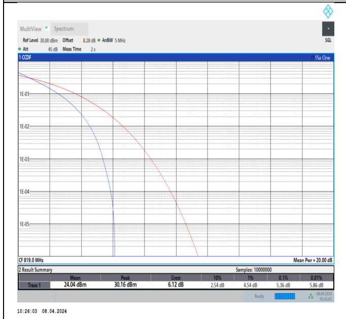
26(814-824)-3MHz-QPSK-26740-15RB#0-PASS
