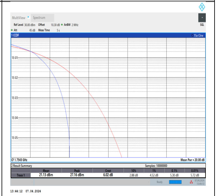
Band4-1.4MHz-16QAM-20393-6RB#0-PASS
