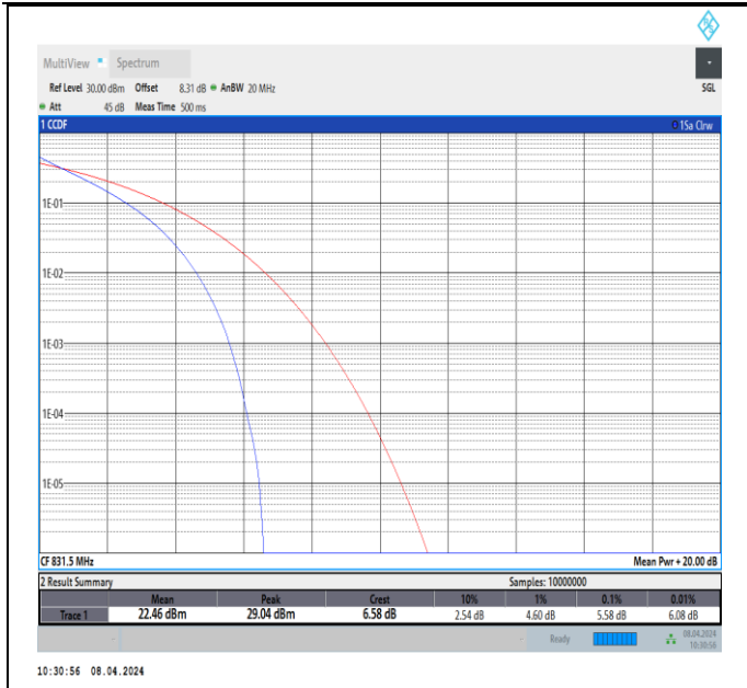
26(824-849)-15MHz-QPSK-26865-75RB#0-PASS
