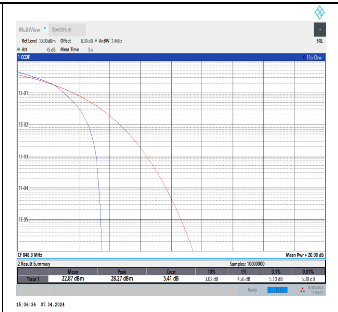
Band5-1.4MHz-16QAM-20643-6RB#0-PASS
