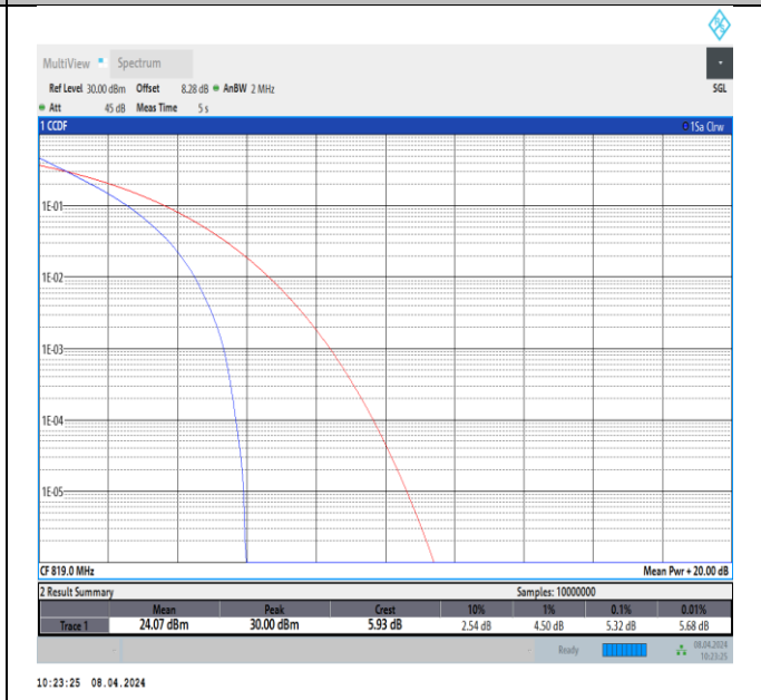
26(814-824)-1.4MHz-QPSK-26740-6RB#0-PASS
