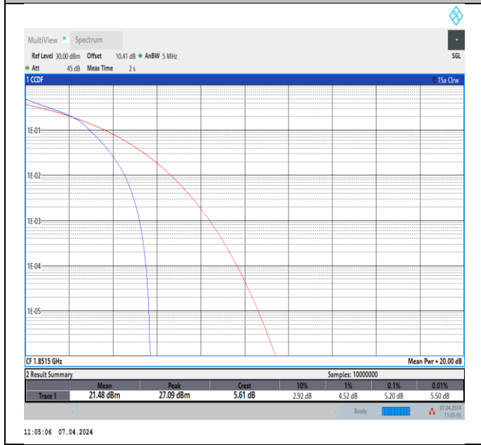
Band2-3MHz-16QAM-18615-15RB#0-PASS
