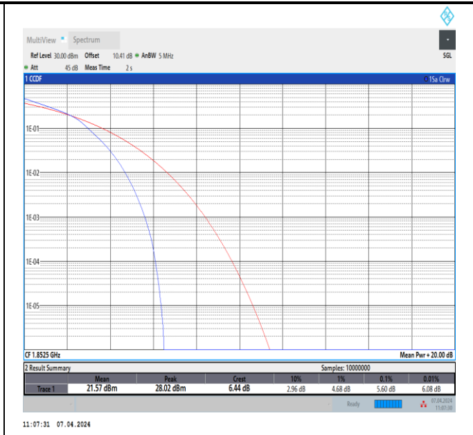
Band2-5MHz-16QAM-18625-25RB#0-PASS
