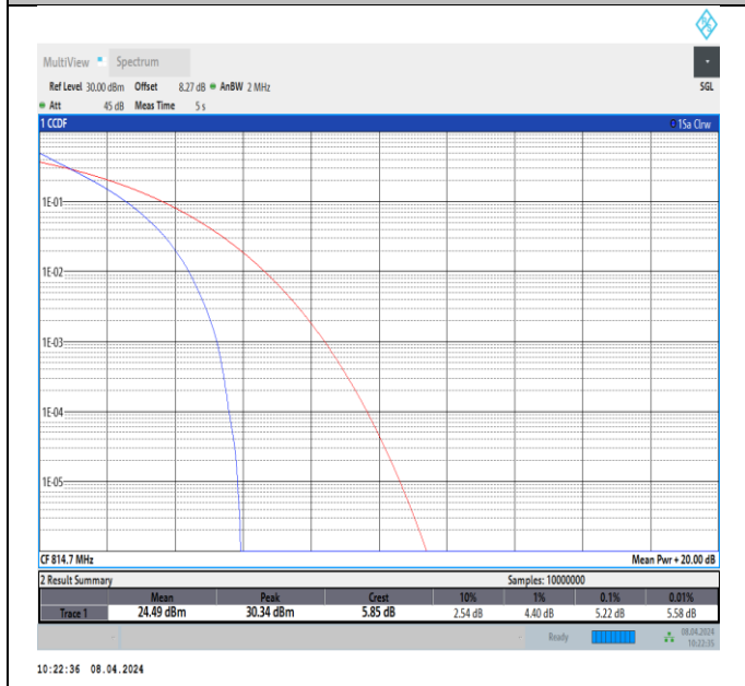
26(814-824)-1.4MHz-QPSK-26697-6RB#0-PASS
