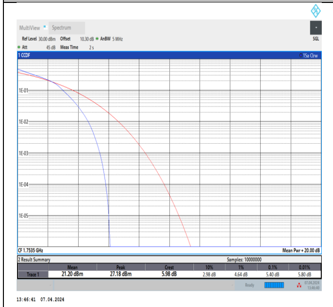
Band4-3MHz-16QAM-20385-15RB#0-PASS
