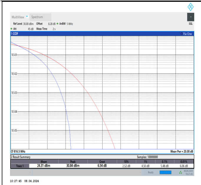
26(814-824)-5MHz-QPSK-26715-25RB#0-PASS
