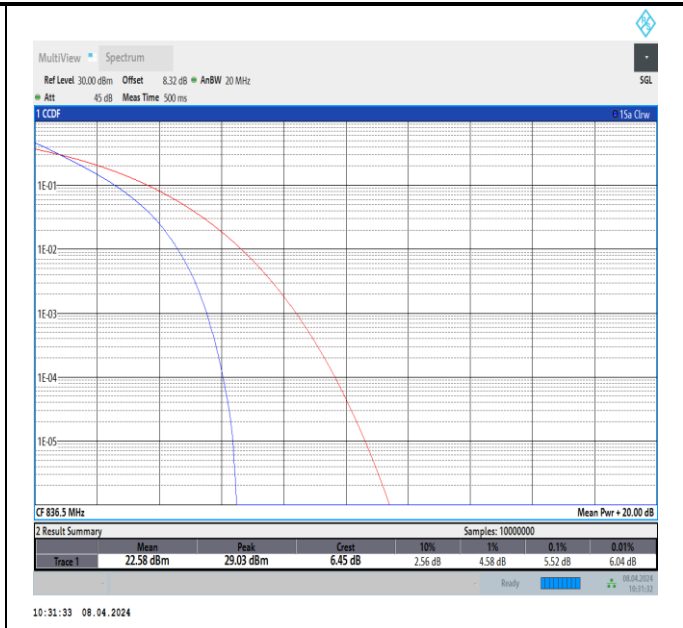
26(824-849)-15MHz-QPSK-26915-75RB#0-PASS
