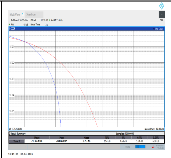
Band4-5MHz-16QAM-20375-25RB#0-PASS
