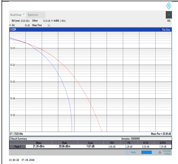
Band4-1.4MHz-16QAM-20175-6RB#0-PASS
