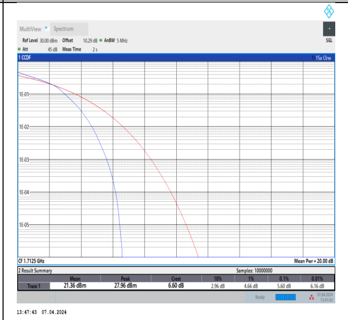
Band4-5MHz-16QAM-19975-25RB#0-PASS
