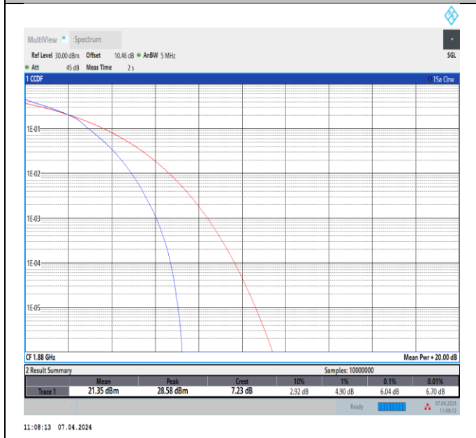
Band2-5MHz-16QAM-18900-25RB#0-PASS
