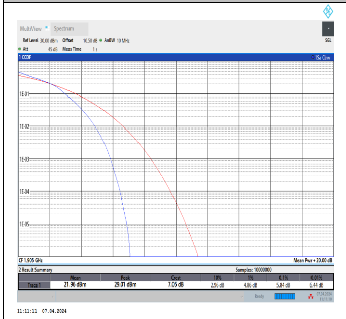
Band2-10MHz-16QAM-19150-50RB#0-PASS
