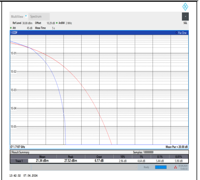
Band4-1.4MHz-16QAM-19957-6RB#0-PASS
