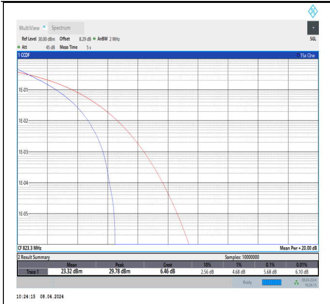
26(814-824)-1.4MHz-QPSK-26783-6RB#0-PASS
