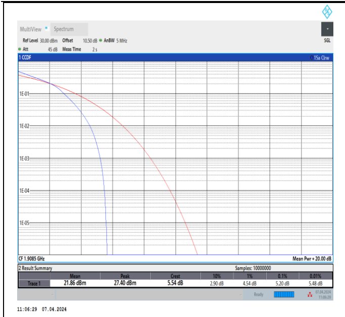
Band2-3MHz-16QAM-19185-15RB#0-PASS
