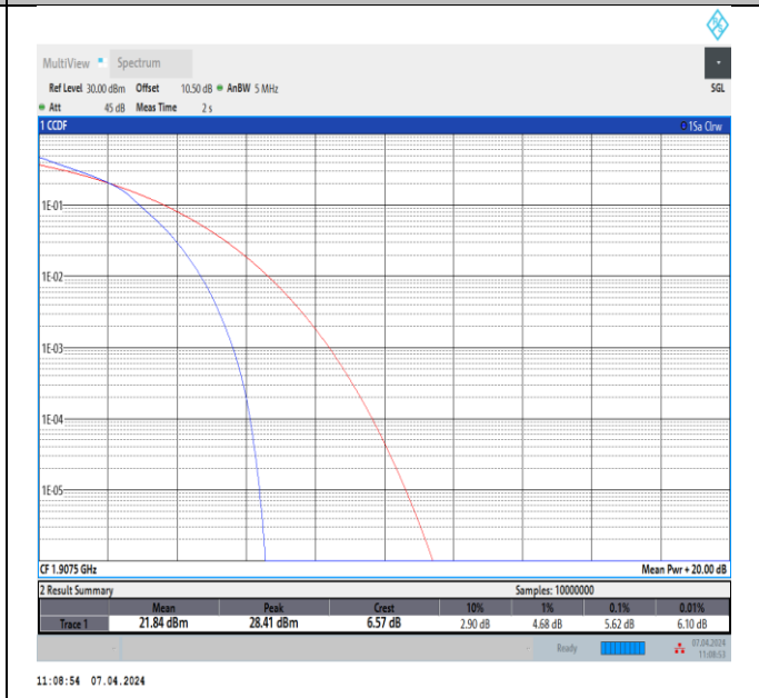
Band2-5MHz-16QAM-19175-25RB#0-PASS
