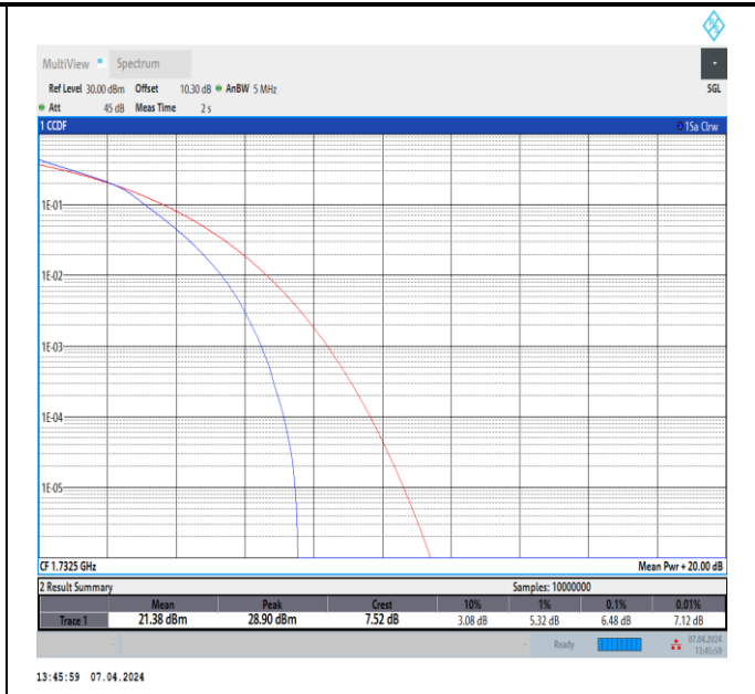
Band4-3MHz-16QAM-20175-15RB#0-PASS
