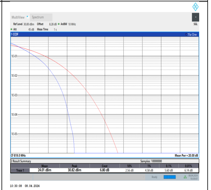
26(814-824)-10MHz-QPSK-26740-50RB#0-PASS
