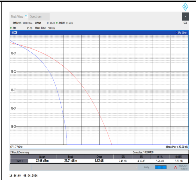
Band66-20MHz-QPSK-132572-100RB#0-PASS
