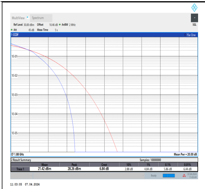
Band2-1.4MHz-16QAM-18900-6RB#0-PASS
