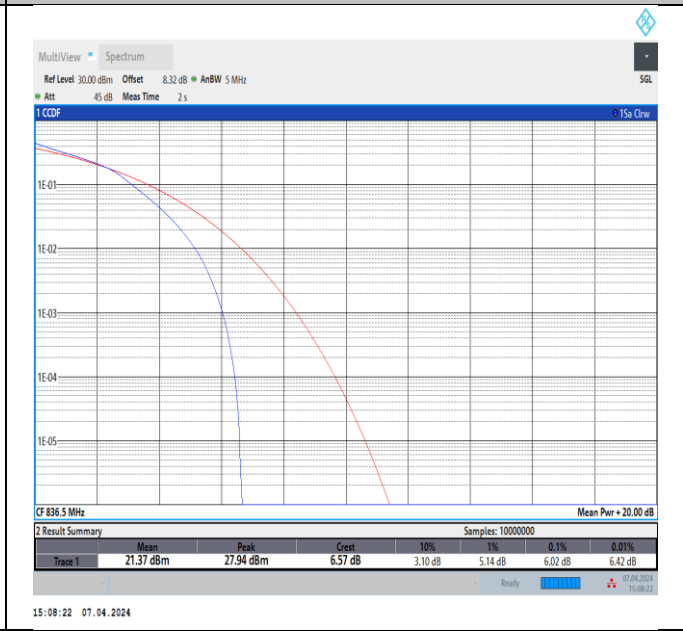
Band5-3MHz-16QAM-20525-15RB#0-PASS
