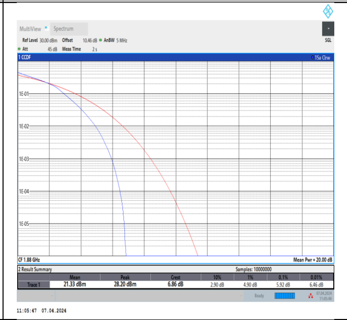
Band2-3MHz-16QAM-18900-15RB#0-PASS
