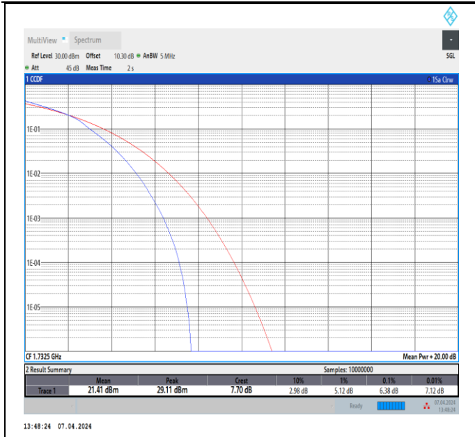
Band4-5MHz-16QAM-20175-25RB#0-PASS
