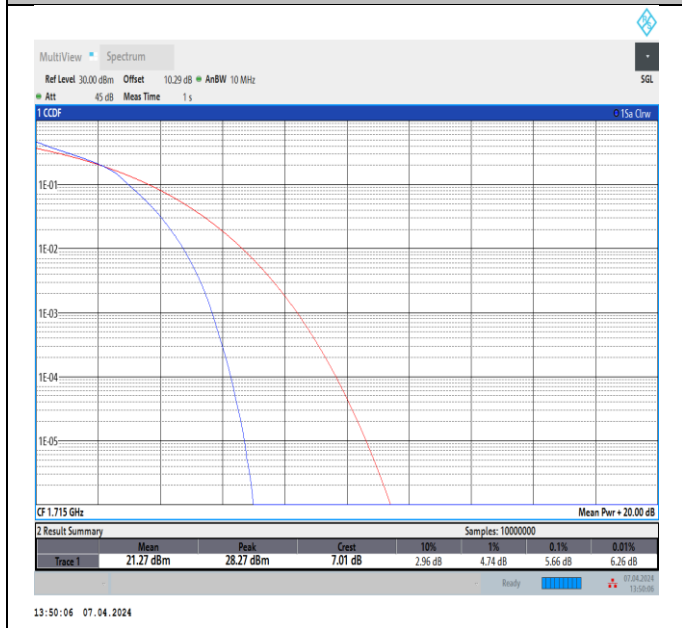
Band4-10MHz-16QAM-20000-50RB#0-PASS
