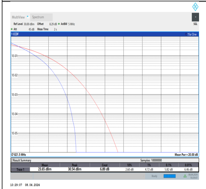
26(814-824)-5MHz-QPSK-26765-25RB#0-PASS
