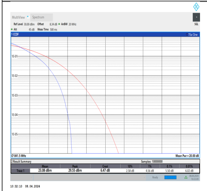
26(824-849)-15MHz-QPSK-26965-75RB#0-PASS
