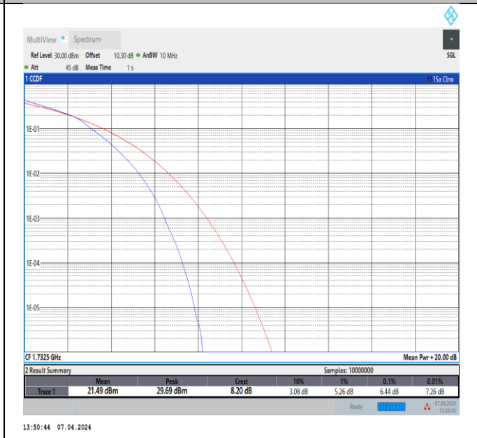
Band4-10MHz-16QAM-20175-50RB#0-PASS
