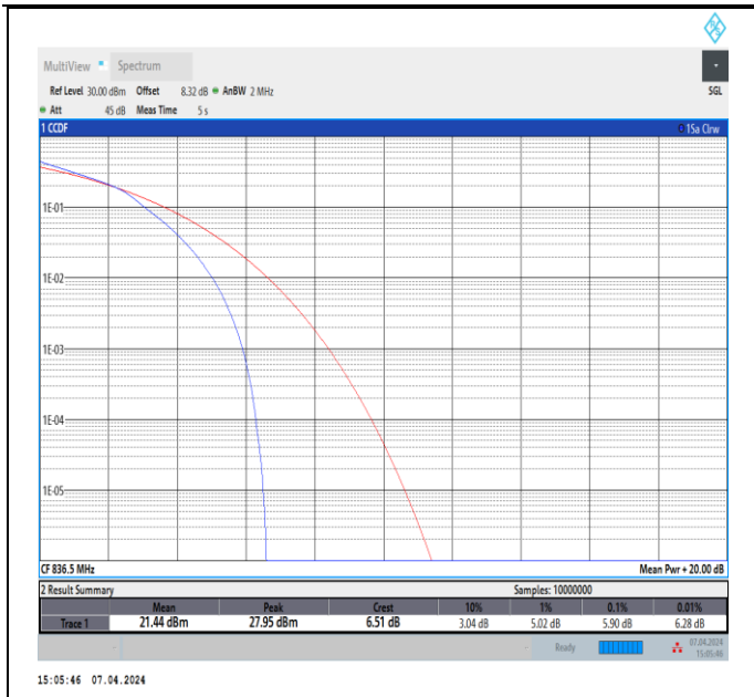
Band5-1.4MHz-16QAM-20525-6RB#0-PASS
