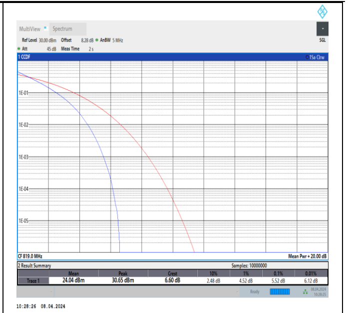
26(814-824)-5MHz-QPSK-26740-25RB#0-PASS
