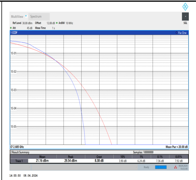
Band41-10MHz-QPSK-41540-50RB#0-PASS
