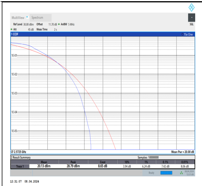
Band38-5MHz-QPSK-37775-25RB#0-PASS
