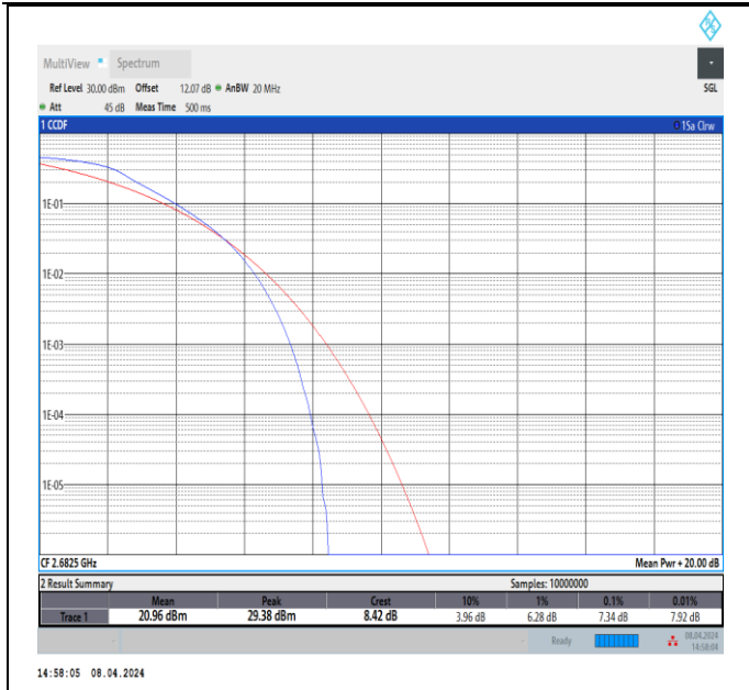
Band41-15MHz-QPSK-41515-75RB#0-PASS
