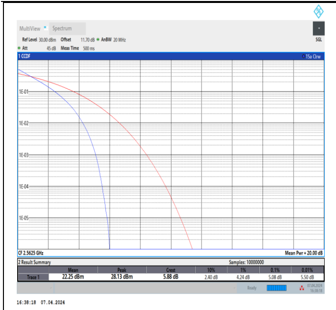
Band7-15MHz-QPSK-21375-75RB#0-PASS
