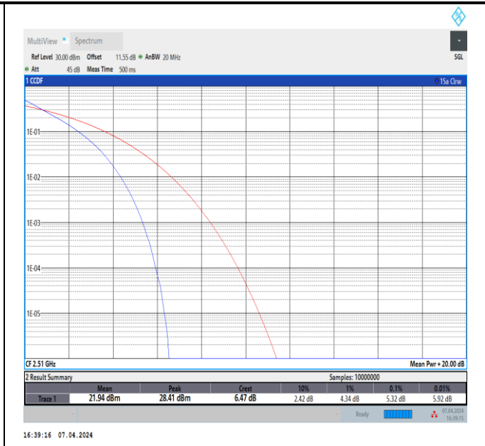
Band7-20MHz-QPSK-20850-100RB#0-PASS
