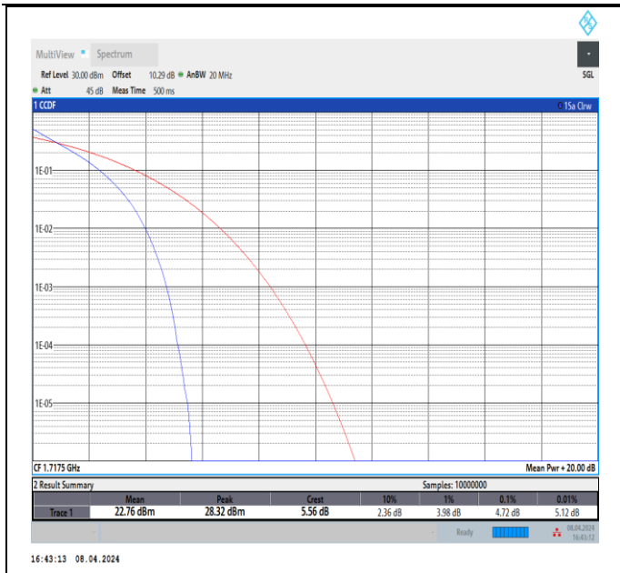
Band66-15MHz-QPSK-132047-75RB#0-PASS
