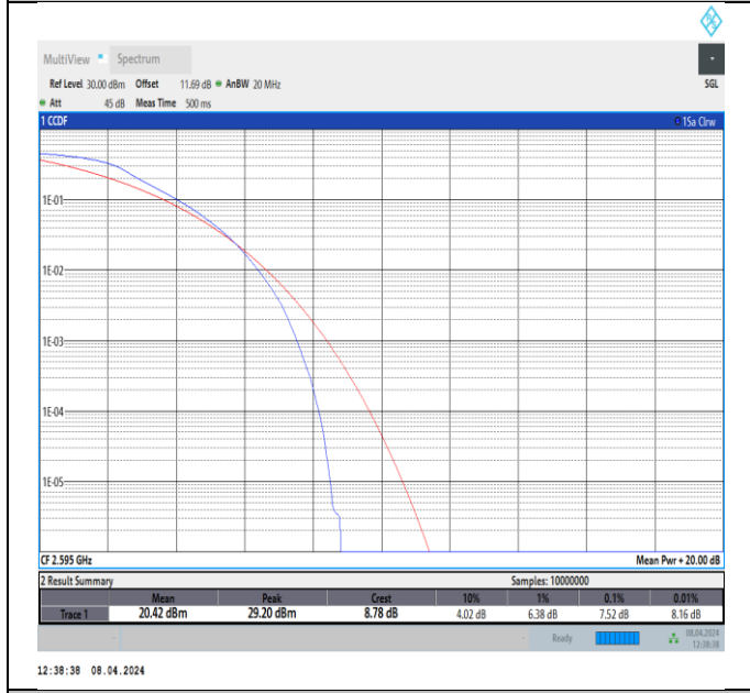
Band38-20MHz-QPSK-38000-100RB#0-PASS
