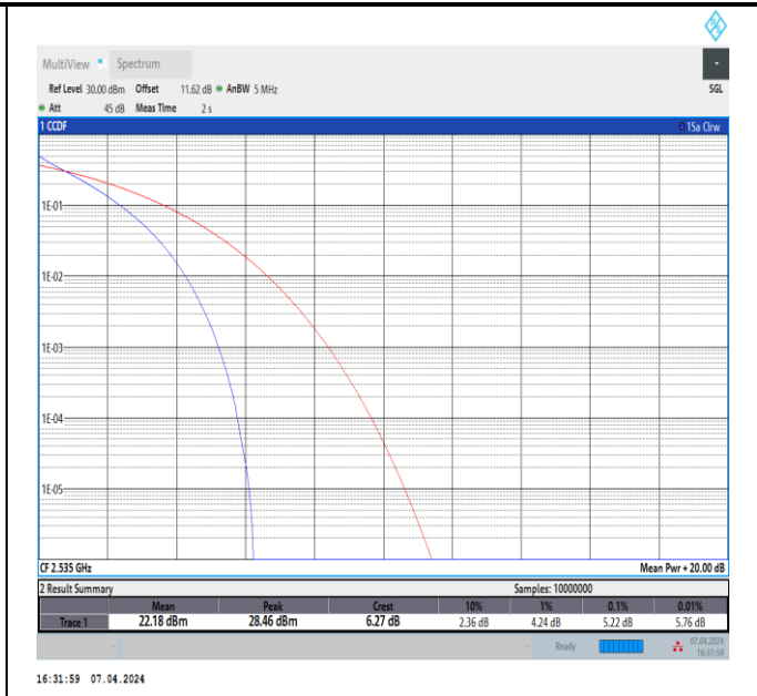
Band7-5MHz-QPSK-21100-25RB#0-PASS
