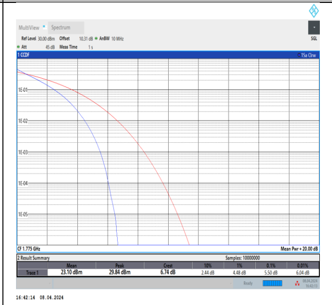
Band66-10MHz-QPSK-132622-50RB#0-PASS
