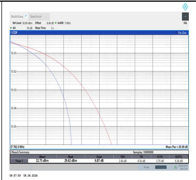
Band 13-5MHz-QPSK-23230-25RB#0-PASS
