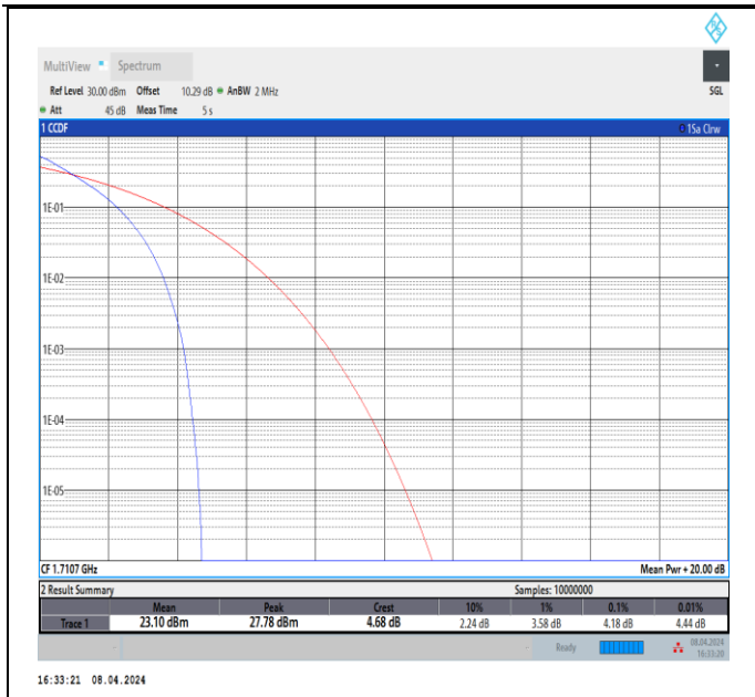
Band66-1.4MHz-QPSK-131979-6RB#0-PASS
