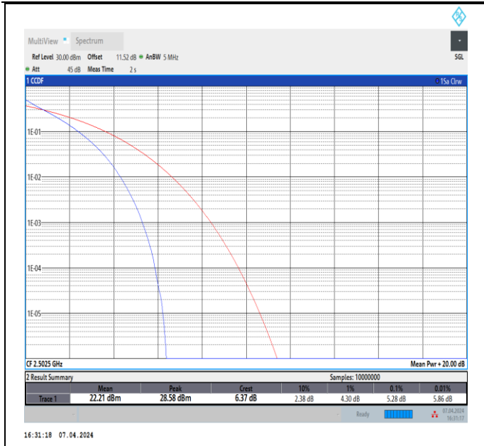
Band7-5MHz-QPSK-20775-25RB#0-PASS
