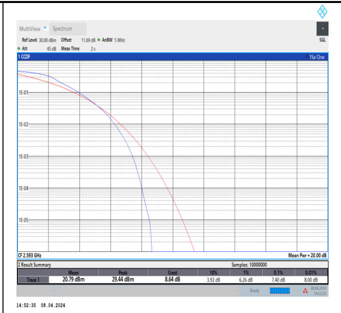
Band41-5MHz-QPSK-40620-25RB#0-PASS
