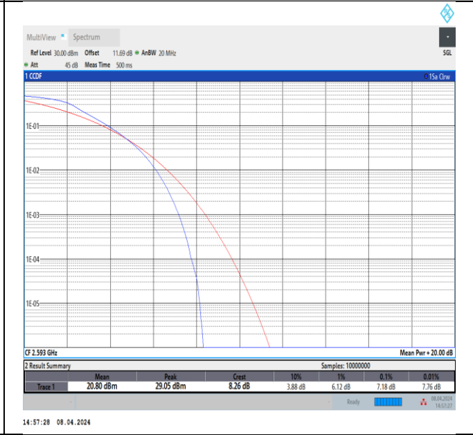
Band41-15MHz-QPSK-40620-75RB#0-PASS
