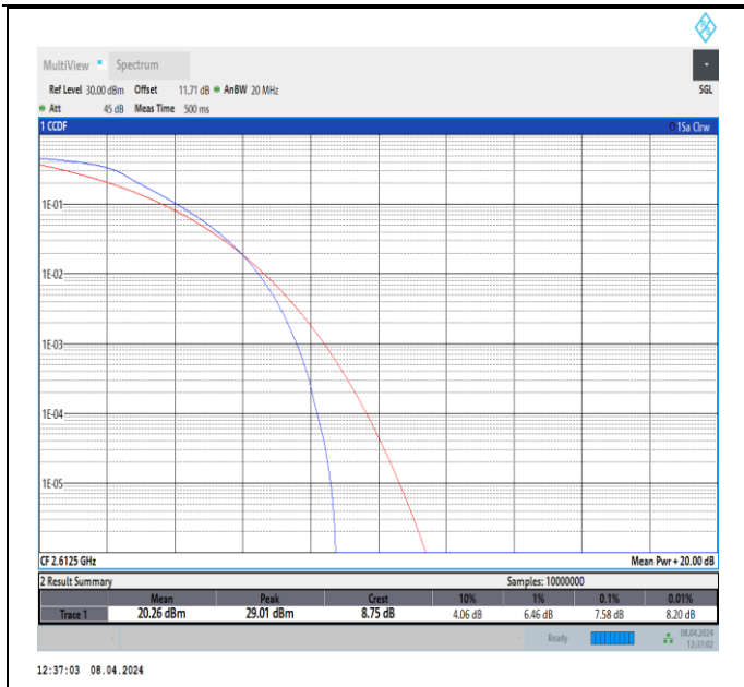
Band38-15MHz-QPSK-38175-75RB#0-PASS
