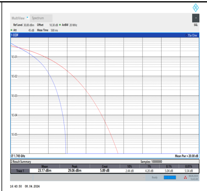
Band66-15MHz-QPSK-132322-75RB#0-PASS
