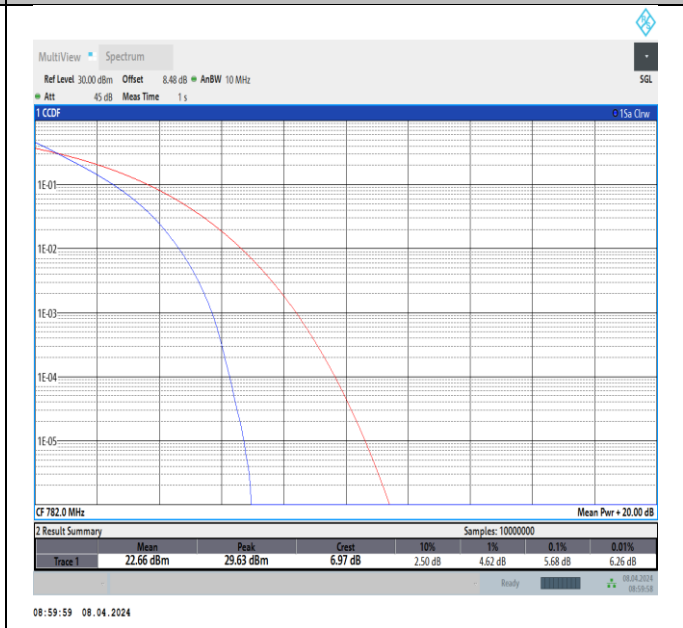
Band 13-10MHz-QPSK-23230-50RB#0-PASS
