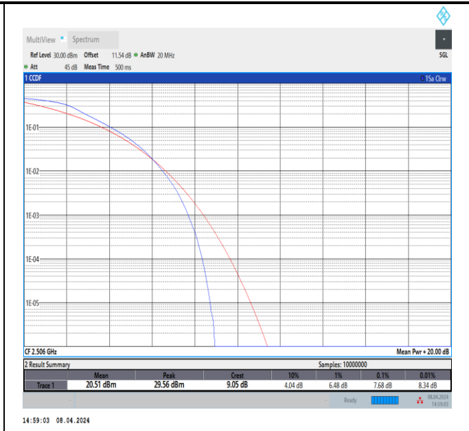
Band41-20MHz-QPSK-39750-100RB#0-PASS
