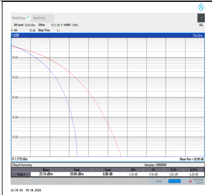
Band66-5MHz-QPSK-132647-25RB#0-PASS
