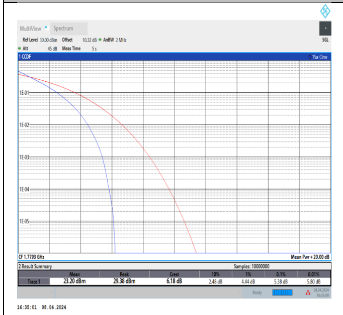
Band66-1.4MHz-QPSK-132665-6RB#0-PASS
