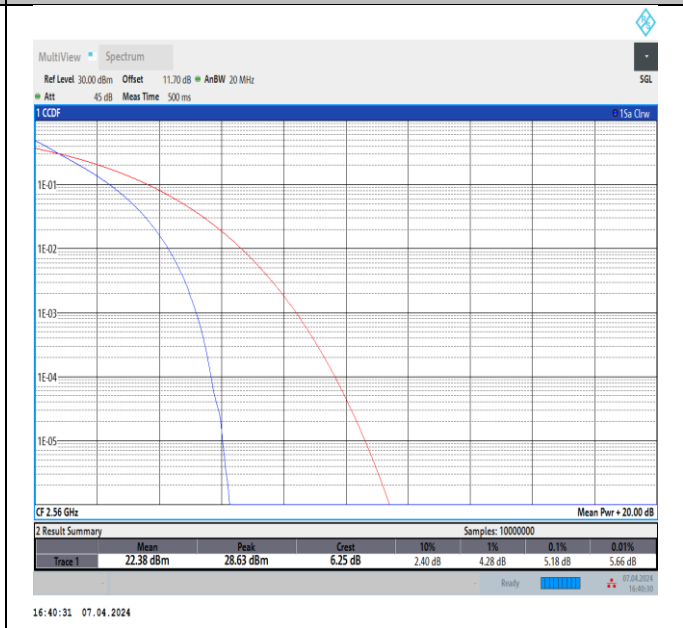
Band7-20MHz-QPSK-21350-100RB#0-PASS
