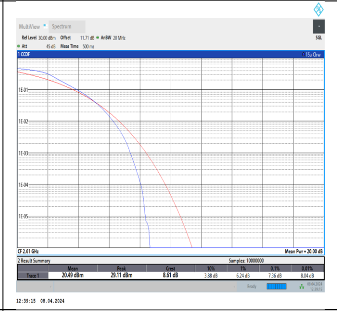
Band38-20MHz-QPSK-38150-100RB#0-PASS
