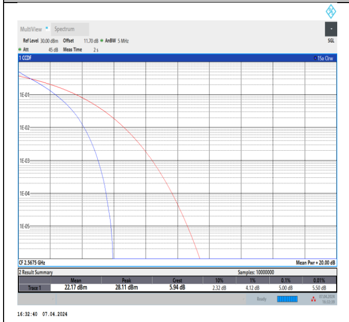
Band7-5MHz-QPSK-21425-25RB#0-PASS
