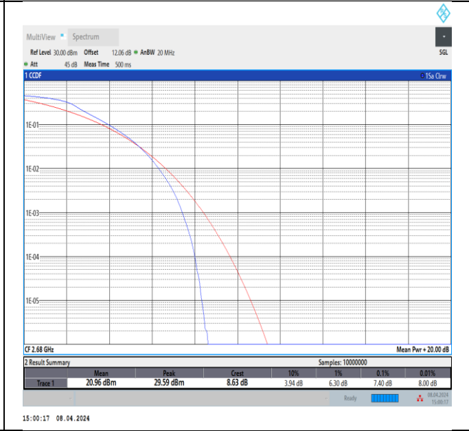
Band41-20MHz-QPSK-41490-100RB#0-PASS
