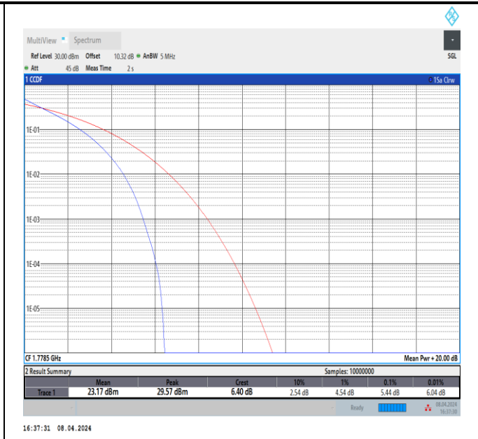
Band66-3MHz-QPSK-132657-15RB#0-PASS
