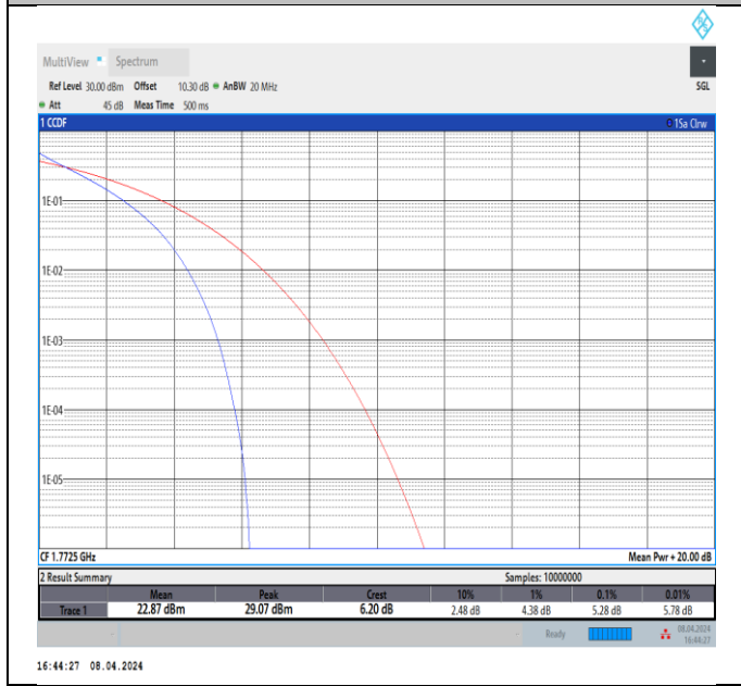
Band66-15MHz-QPSK-132597-75RB#0-PASS
