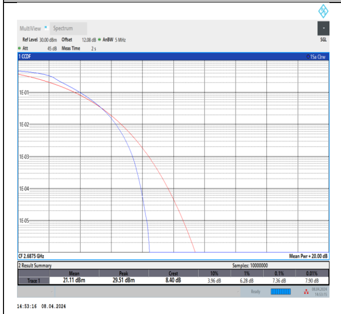
Band41-5MHz-QPSK-41565-25RB#0-PASS
