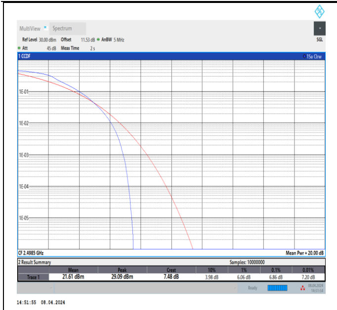
Band41-5MHz-QPSK-39675-25RB#0-PASS
