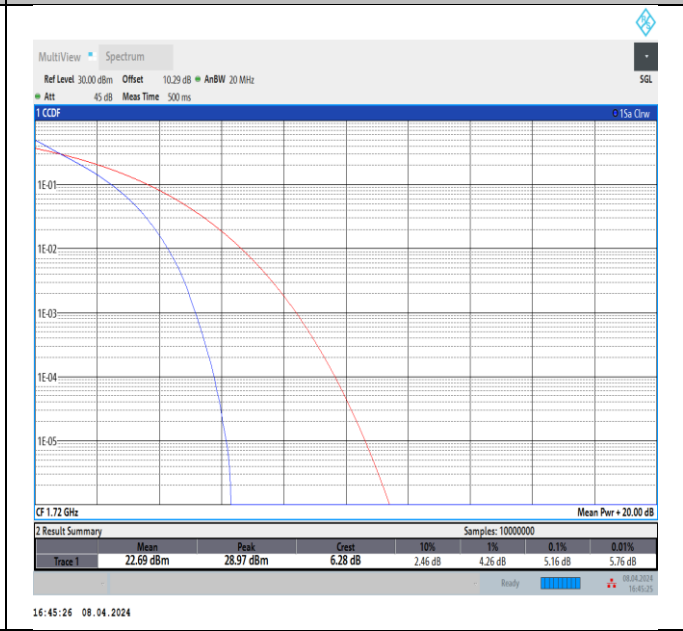
Band66-20MHz-QPSK-132072-100RB#0-PASS
