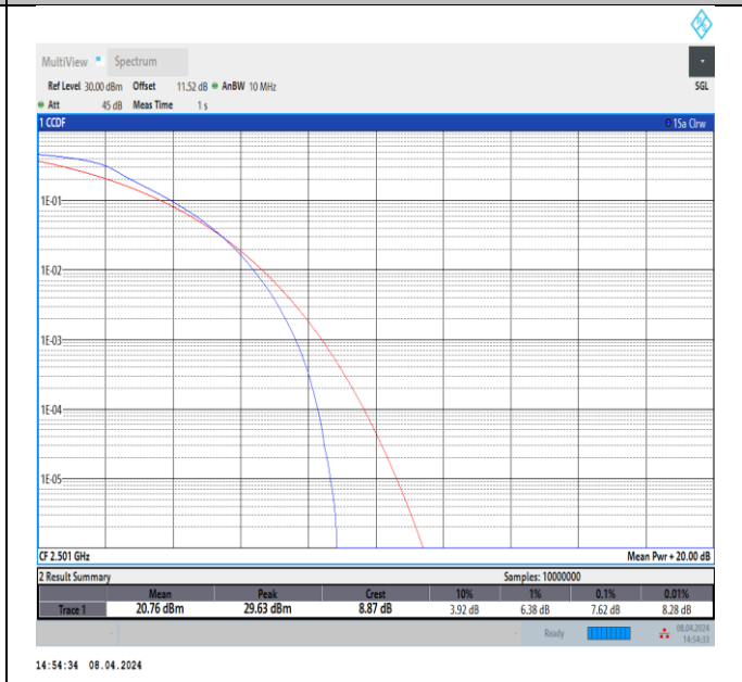
Band41-10MHz-QPSK-39700-50RB#0-PASS
