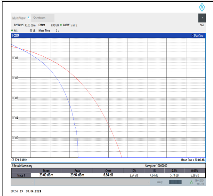
Band 13-5MHz-QPSK-23205-25RB#0-PASS
