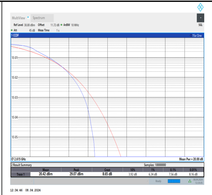
Band38-10MHz-QPSK-38200-50RB#0-PASS
