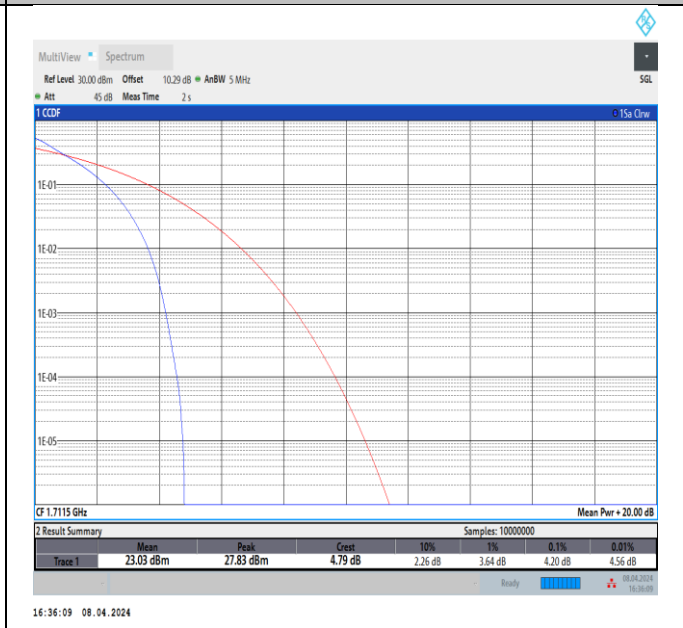
Band66-3MHz-QPSK-131987-15RB#0-PASS
