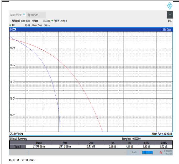
Band7-15MHz-QPSK-20825-75RB#0-PASS
