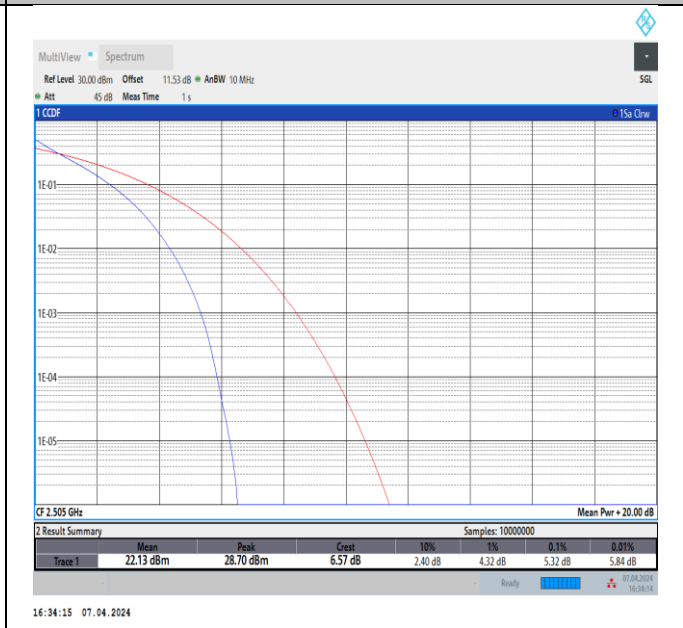
Band7-10MHz-QPSK-20800-50RB#0-PASS
