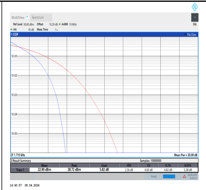
Band66-10MHz-QPSK-132022-50RB#0-PASS
