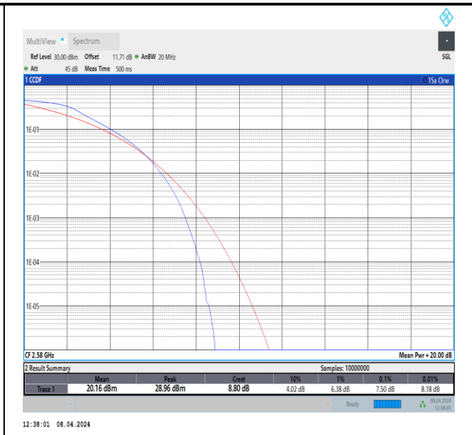
Band38-20MHz-QPSK-37850-100RB#0-PASS
