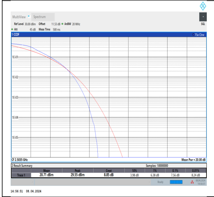
Band41-15MHz-QPSK-39725-75RB#0-PASS
