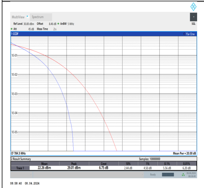
Band 13-5MHz-QPSK-23255-25RB#0-PASS
