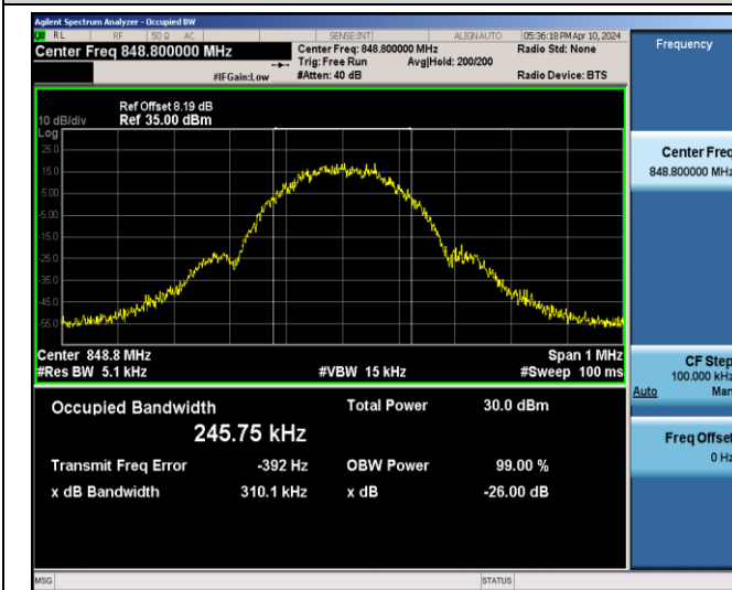
EGPRS850-251-8-0.3101
