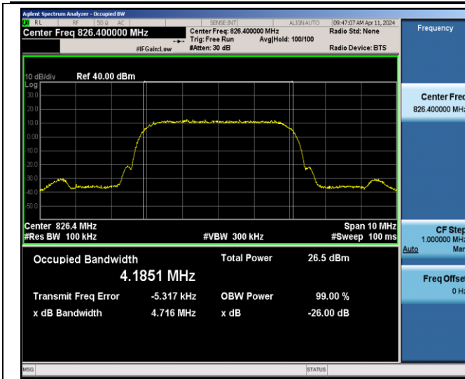
Band5-4132-4.716
