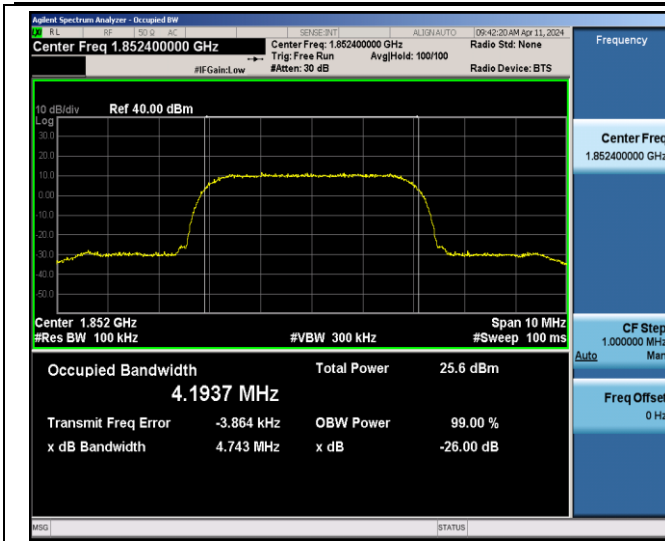
Band2-9262-4.743
