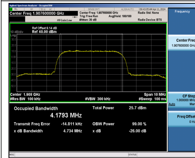
Band2-9538-4.734
