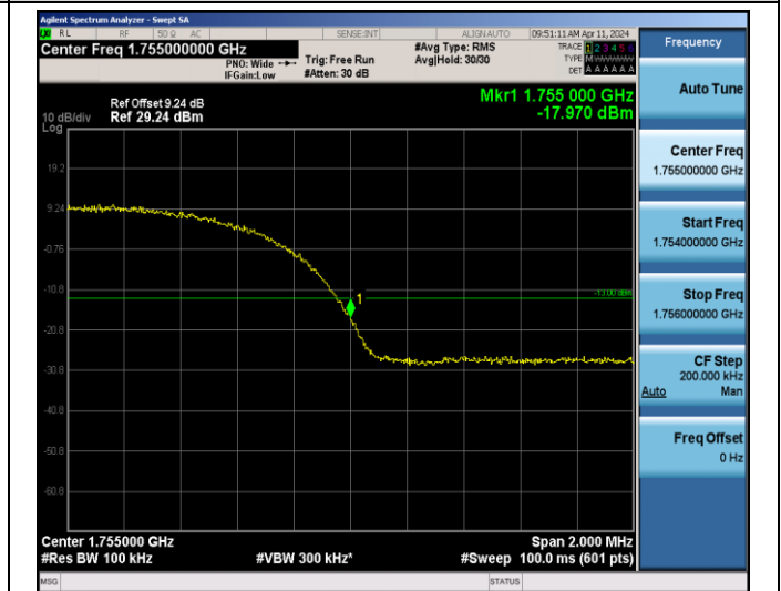
Band4-1513
