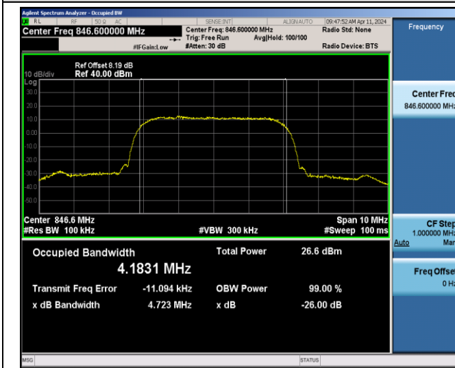
Band5-4233-4.723
