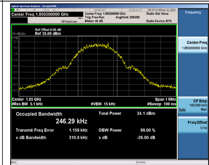
GSM1900-512-0-0.3109
