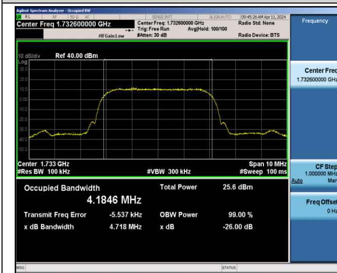
Band4-1413-4.718
