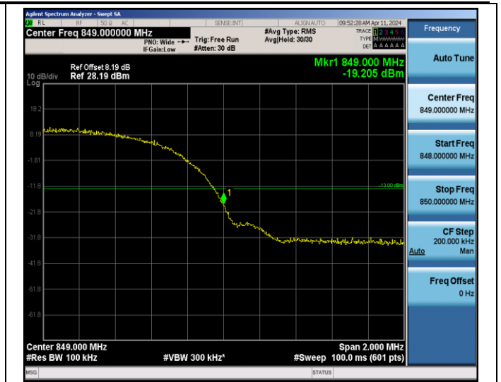
Band5-4233
