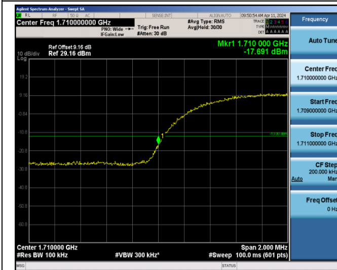
Band4-1312
