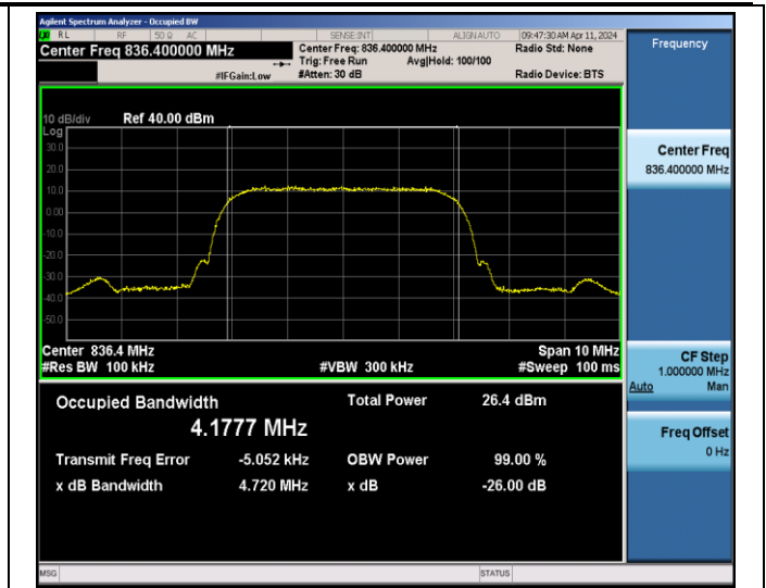
Band5-4182-4.720
