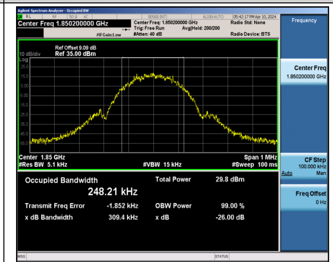
EGPRS1900-512-2-0.3094
