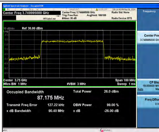
1-N78-3700-3800-PC2-30-90-M-8-CP-64QAM-Outer_Full-245@0-Ant23-87.175-90.40-≤90-PASS
