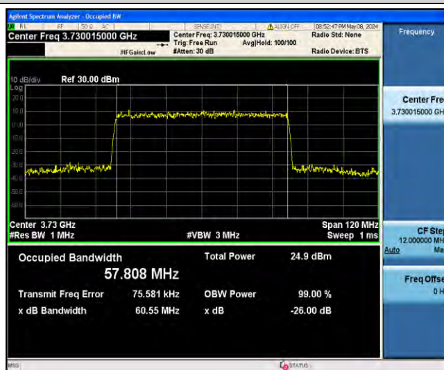
1-N78-3700-3800-PC2-30-60-L-5-DFT-256QAM-Outer_Full-162@0-Ant23-57.808-60.55-≤60-PASS
