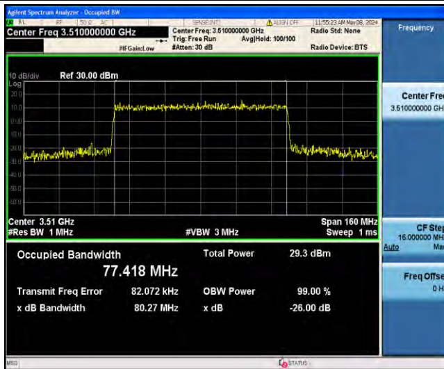
1-N78-3450-3550-PC2-30-80-H-6-CP-QPSK-Outer_Full-217@0-Ant23-77.418-80.27-≤80-PASS
