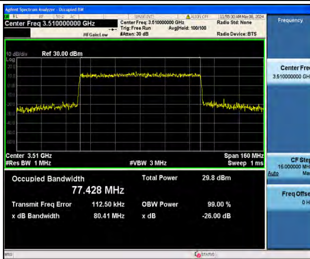
1-N78-3450-3550-PC2-30-80-H-7-CP-16QAM-Outer_Full-217@0-Ant23-77.428-80.41-≤80-PASS
