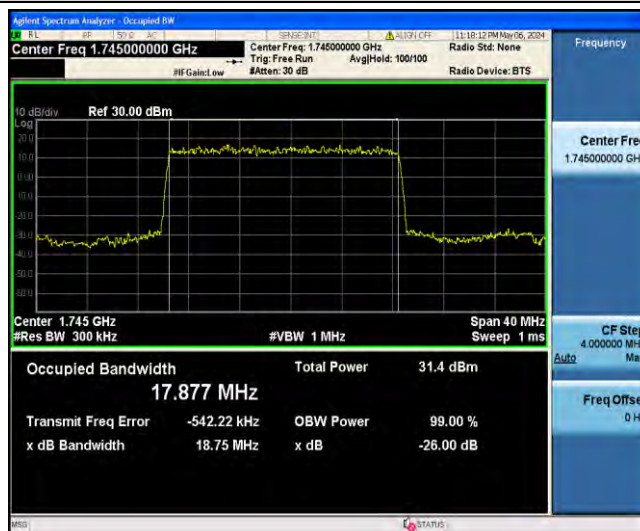
1-N66-PC3-15-20-M-2-DFT-PI2BPSK-Outer_Full-100@0-Ant31-17.877-18.75-≤20-PASS
