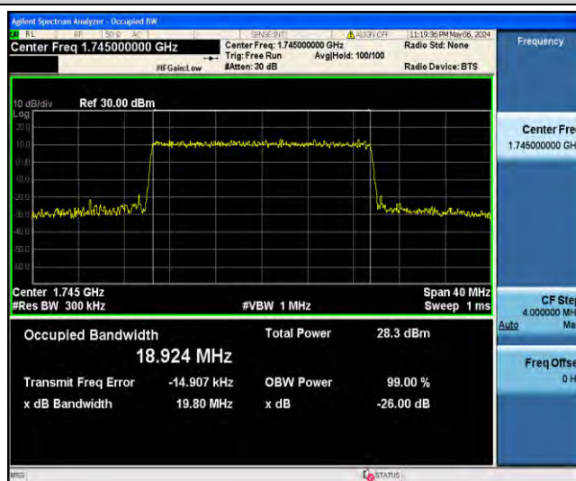
1-N66-PC3-15-20-M-8-CP-64QAM-Outer_Full-106@0-Ant31-18.924-19.80-≤20-PASS
