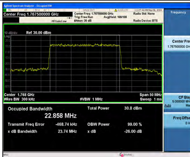
1-N66-PC3-15-25-H-1-DFT-QPSK-Outer_Full-128@0-Ant31-22.858-23.74-≤25-PASS
