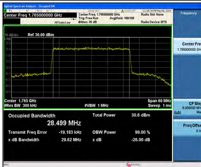
1-N66-PC3-15-30-H-1-DFT-QPSK-Outer_Full-160@0-Ant31-28.499-29.62-<30-PASS
