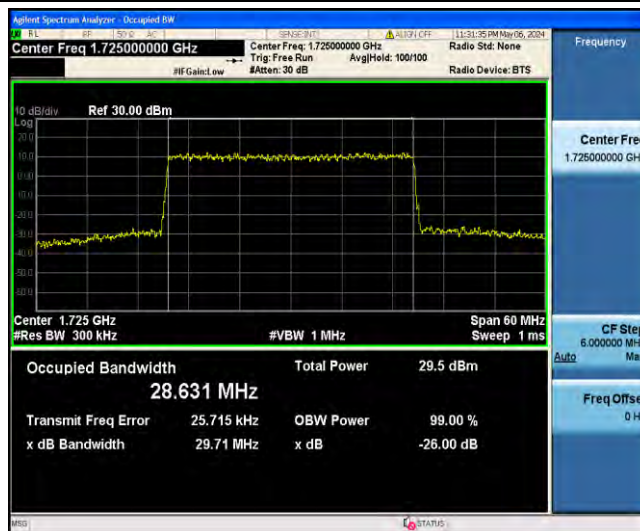
1-N66-PC3-15-30-L-4-DFT-64QAM-Outer_Full-160@0-Ant31-28.631-29.71-≤30-PASS
