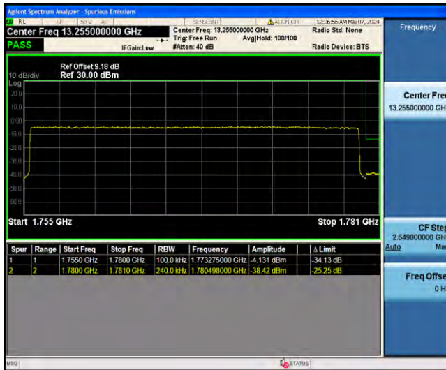
1-N66-PC3-15-25-H-6-CP-QPSK-Outer_Full-133@0-Ant31-1780.50-25.22--38.42-PASS
