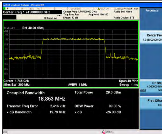
1-N66-PC3-15-20-M-7-CP-16QAM-Outer_Full-106@0-Ant31-18.853-19.79-≤20-PASS
