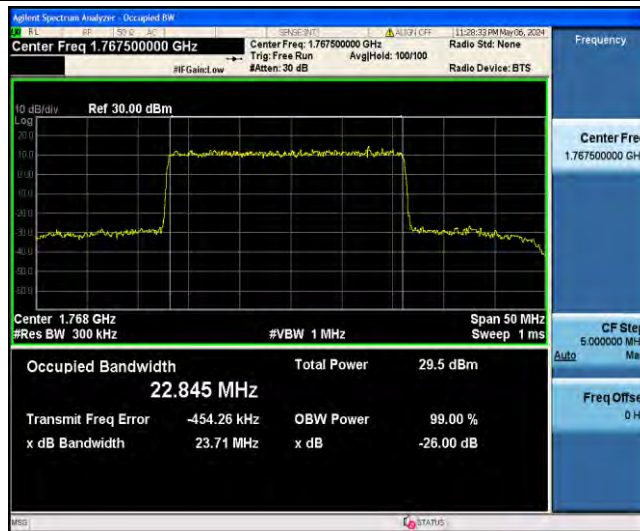
1-N66-PC3-15-25-H-3-DFT-16QAM-Outer_Full-128@0-Ant31-22.845-23.71-≤25-PASS
