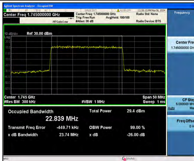
1-N66-PC3-15-25-M-4-DFT-64QAM-Outer_Full-128@0-Ant31-22.839-23.74-≤25-PASS
