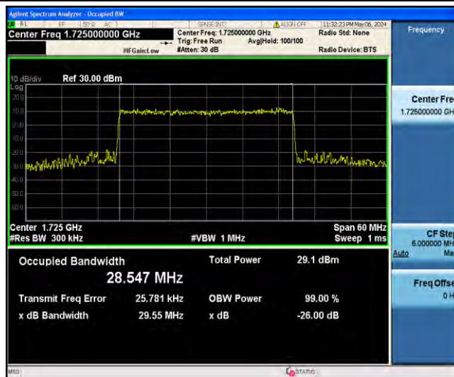
1-N66-PC3-15-30-L-7-CP-16QAM-Outer_Full-160@0-Ant31-28.547-29.55-≤30-PASS
