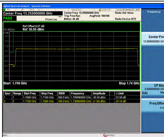
1-N66-PC3-15-30-L-6-CP-QPSK-Outter_Full-160@0-Ant31-1710.00-23.58--36.58-PASS
