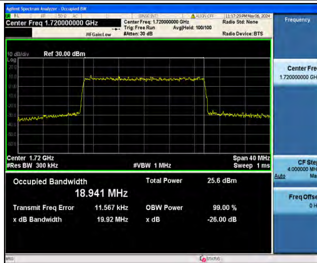
1-N66-PC3-15-20-L-9-CP-256QAM-Outer_Full-106@0-Ant31-18.941-19.92-≤20-PASS
