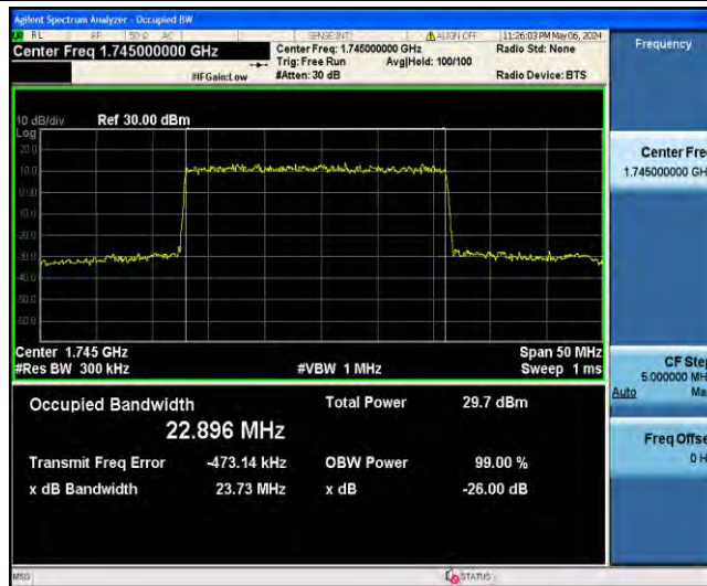
1-N66-PC3-15-25-M-3-DFT-16QAM-Outer_Full-128@0-Ant31-22.896-23.73-≤25-PASS
