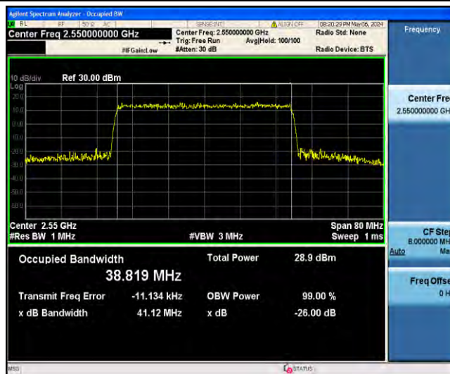
1-N7-PC3-15-40-H-4-DFT-64QAM-Outer_Full-216@0-Ant31-38.819-41.12-≤40-PASS
