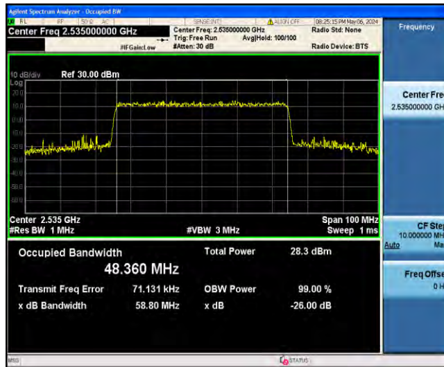
1-N7-PC3-15-50-M-7-CP-16QAM-Outer_Full-270@0-Ant31-48.360-58.80-≤50-PASS
