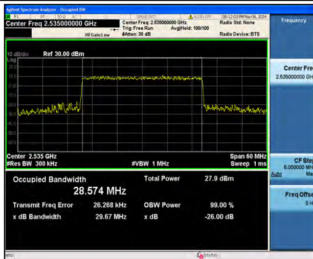
1-N7-PC3-15-30-M-7-CP-16QAM-Outer_Full-160@0-Ant31-28.574-29.67-≤30-PASS
