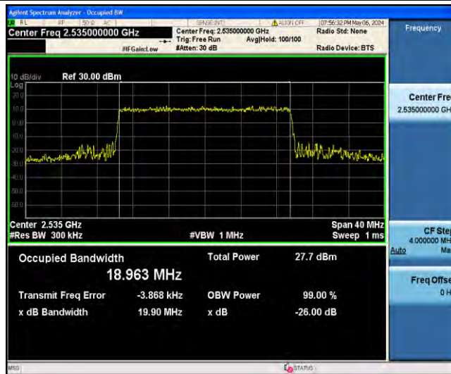
1-N7-PC3-15-20-M-6-CP-QPSK-Outer_Full-106@0-Ant31-18.963-19.90-≤20-PASS
