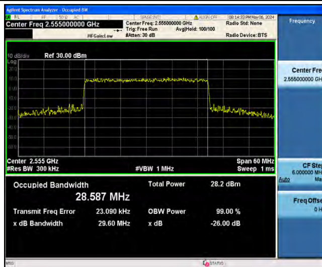
1-N7-PC3-15-30-H-7-CP-16QAM-Outer_Full-160@0-Ant31-28.587-29.60-<30-PASS
