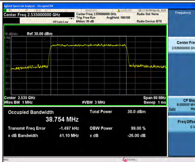
1-N7-PC3-15-40-M-1-DFT-QPSK-Outer_Full-216@0-Ant31-38.754-41.10-<40-PASS
