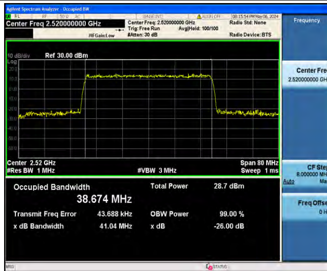
1-N7-PC3-15-40-L-3-DFT-16QAM-Outer_Full-216@0-Ant31-38.674-41.04-≤40-PASS
