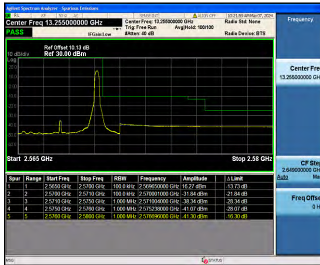
1-N7-PC3-15-5-H-5-CP-QPSK-Edge_1RB_Right-1@24-Ant31-2576.70-16.30--41.30-PASS
