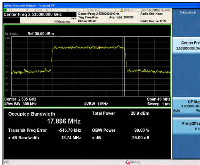
1-N7-PC3-15-20-M-3-DFT-16QAM-Outer_Full-100@0-Ant31-17.896-18.74-≤20-PASS
