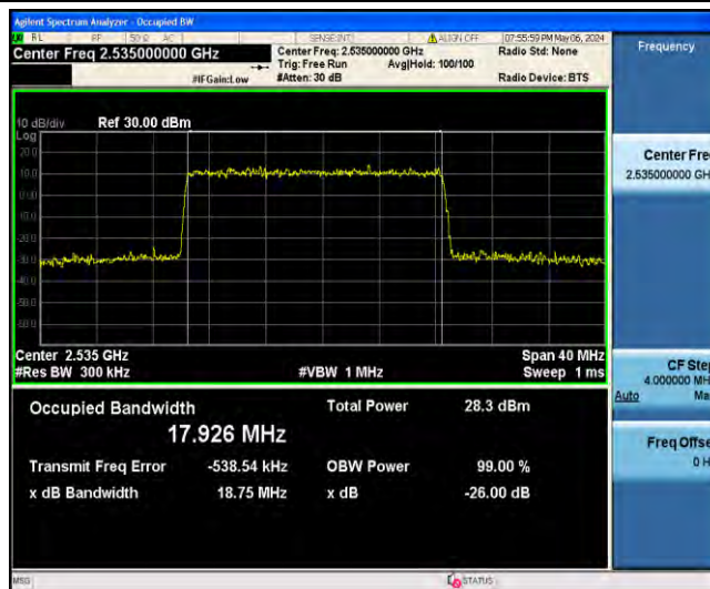
1-N7-PC3-15-20-M-4-DFT-64QAM-Outer_Full-100@0-Ant31-17.926-18.75-≤20-PASS
