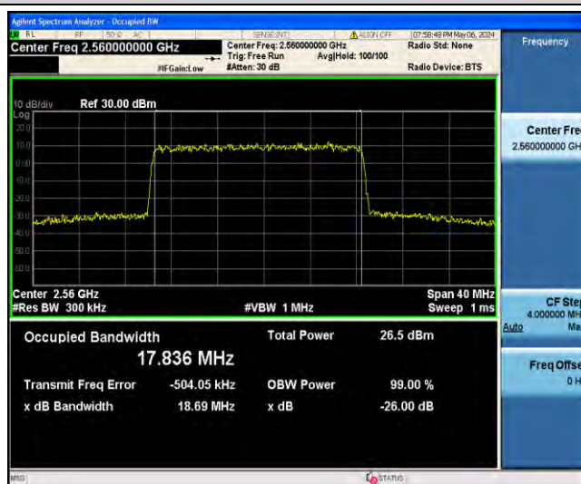
1-N7-PC3-15-20-H-5-DFT-256QAM-Outer_Full-100@0-Ant31-17.836-18.69-<20-PASS
