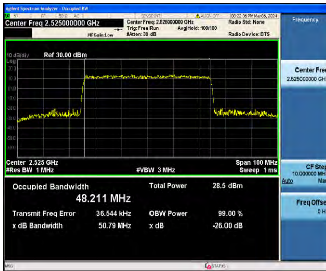
1-N7-PC3-15-50-L-4-DFT-64QAM-Outer_Full-270@0-Ant31-48.211-50.79-≤50-PASS
