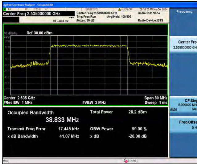
1-N7-PC3-15-40-M-6-CP-QPSK-Outer_Full-216@0-Ant31-38.833-41.07-<40-PASS
