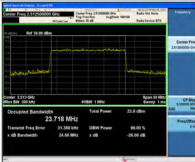
1-N7-PC3-15-25-L-9-CP-256QAM-Outer_Full-133@0-Ant31-23.718-24.66-≤25-PASS
