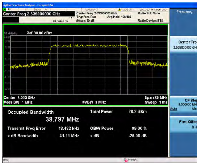
1-N7-PC3-15-40-M-7-CP-16QAM-Outer_Full-216@0-Ant31-38.797-41.11-<40-PASS
