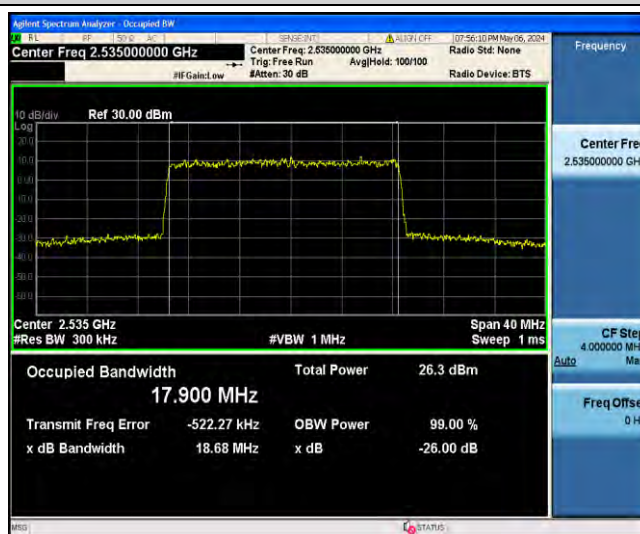
1-N7-PC3-15-20-M-5-DFT-256QAM-Outer_Full-100@0-Ant31-17.900-18.68-≤20-PASS
