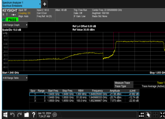
N2(5M)_DFT-s-OFDM_BPSK_Outer_Full_Low_CH
