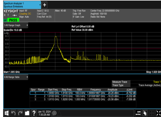
N2(10M)_DFT-s- OFDM_BPSK_Edge_1RB_Right_High_CH
