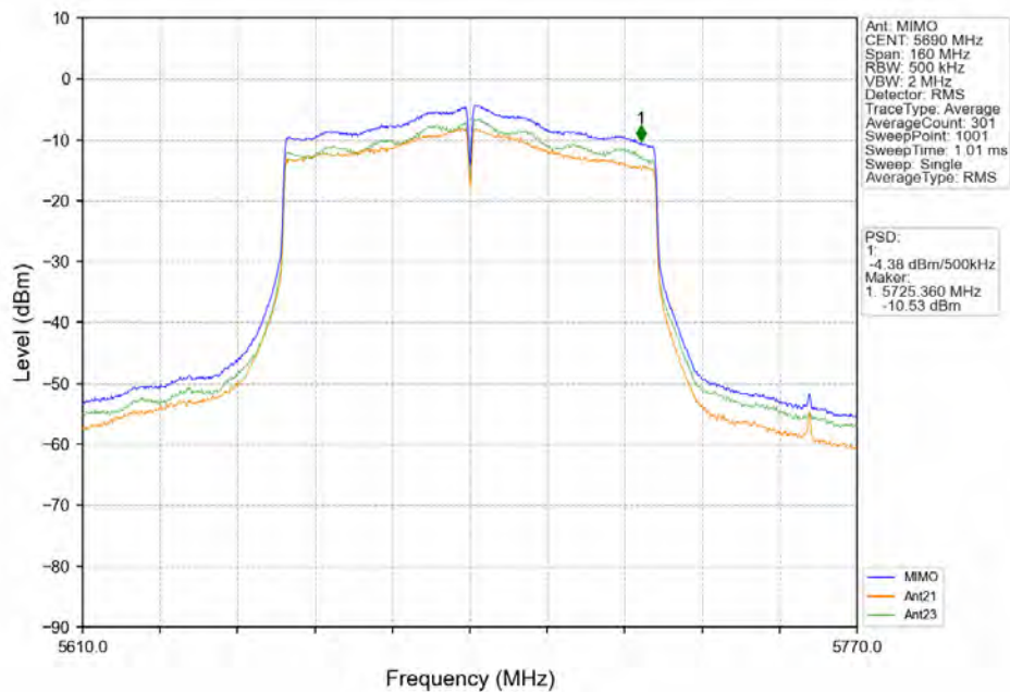
802.11ac(VHT80)_HCH_5690MHz_MIMO_NTNV
