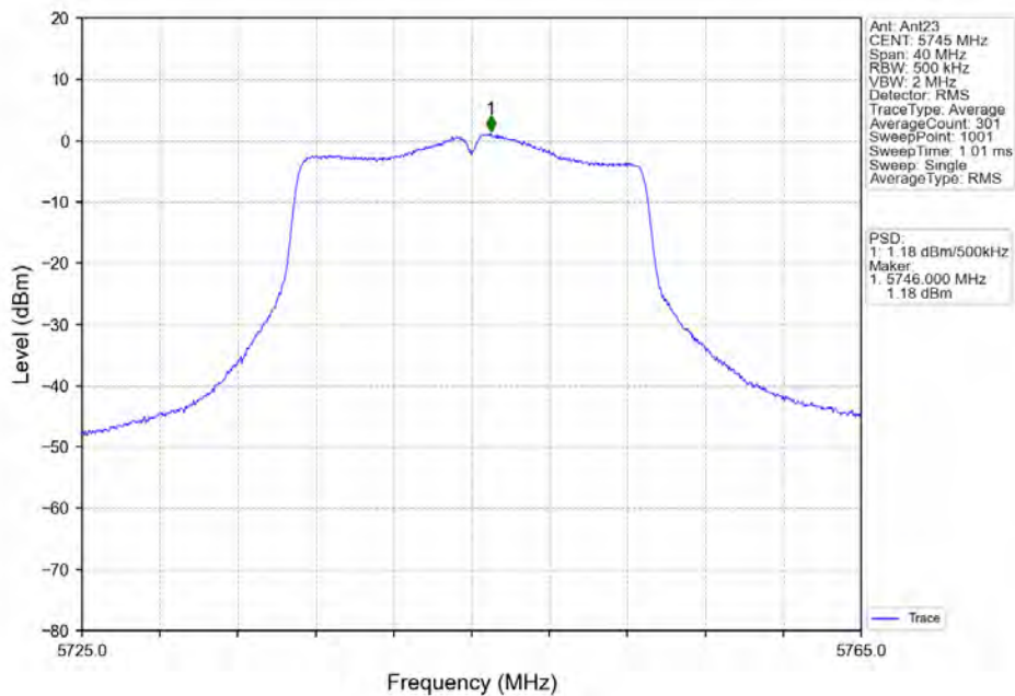
802.11n(HT20) LCH_5745MHz_Ant23_NTNV
