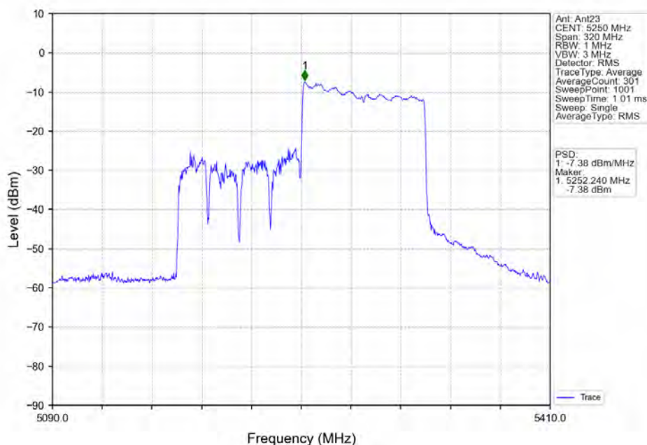
802.11ax(HE160) MCH 5250MHz RU996 Right MIMO NTN
