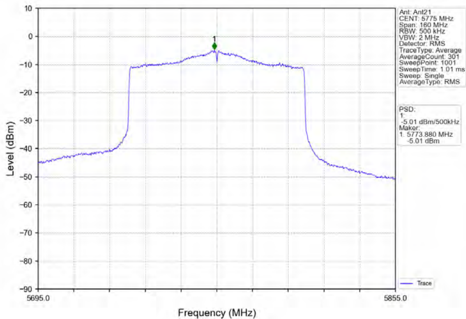
802.11ax(HE80) MCH 5775MHz RU996 Left Ant21 NTN
