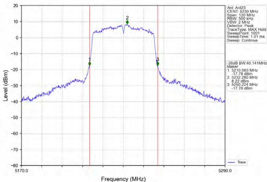
802.11ac(VHT40)_HCH_5230MHz_Ant23_NTNV
