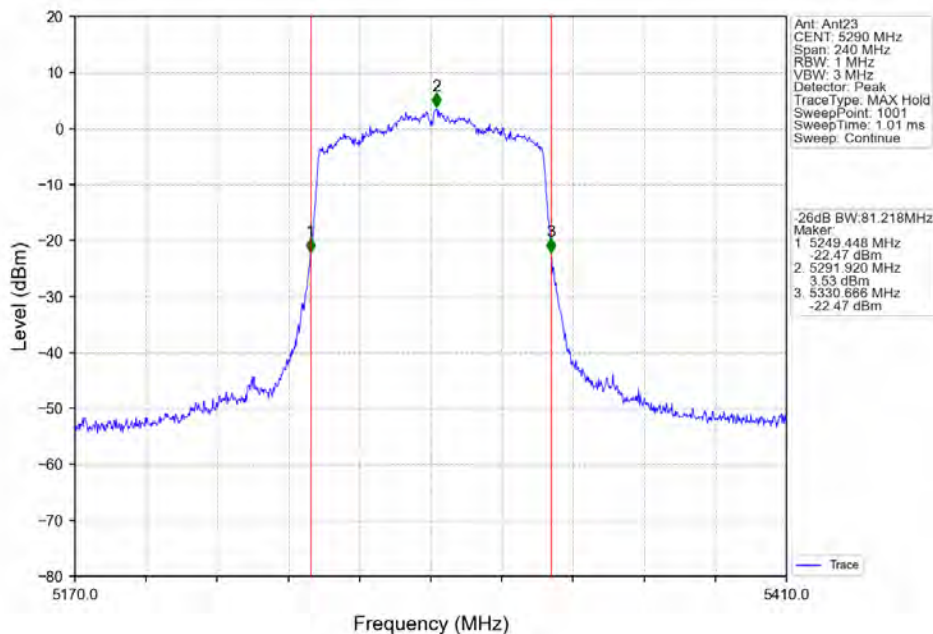
802.11ac(VHT80)_MCH_5290MHz_Ant23_NTNV
