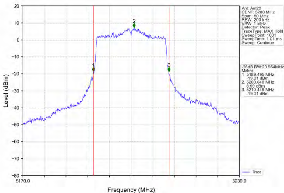
802.11ax(HE20) MCH 5200MHz RU242 Left Ant23 NTN
