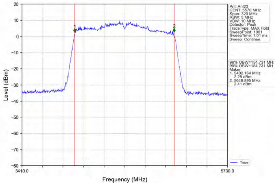
802.11ac(VHT160)_MCH_5570MHz_Ant23_NTNV
