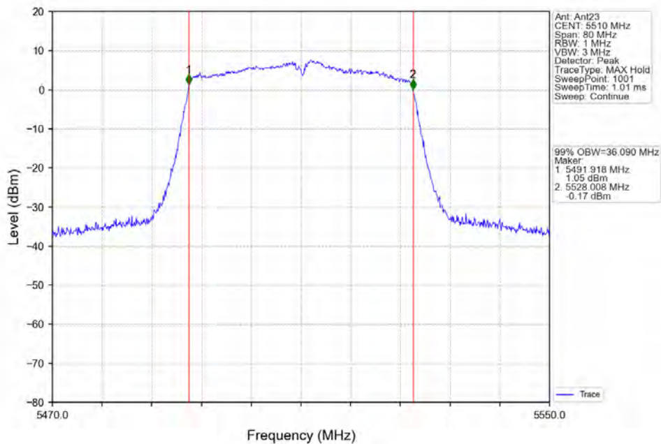
802.11ac(VHT40)_LCH_5510MHz_Ant23_NTNV
