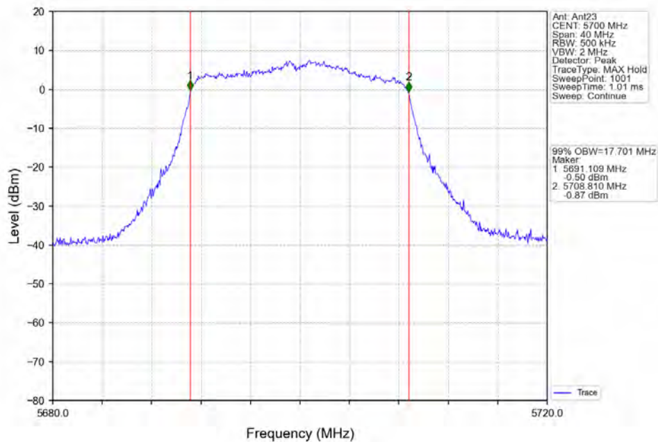
802.11ac(VHT20)_HCH_5700MHz_Ant23_NTNV
