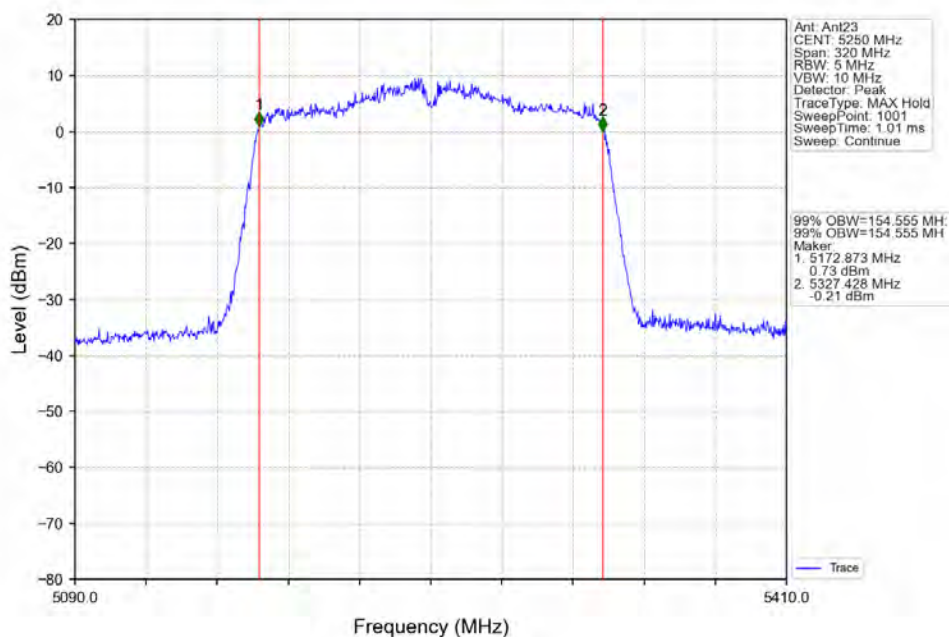
802.11ac(VHT160)_MCH_5250MHz_Ant23_NTNV
