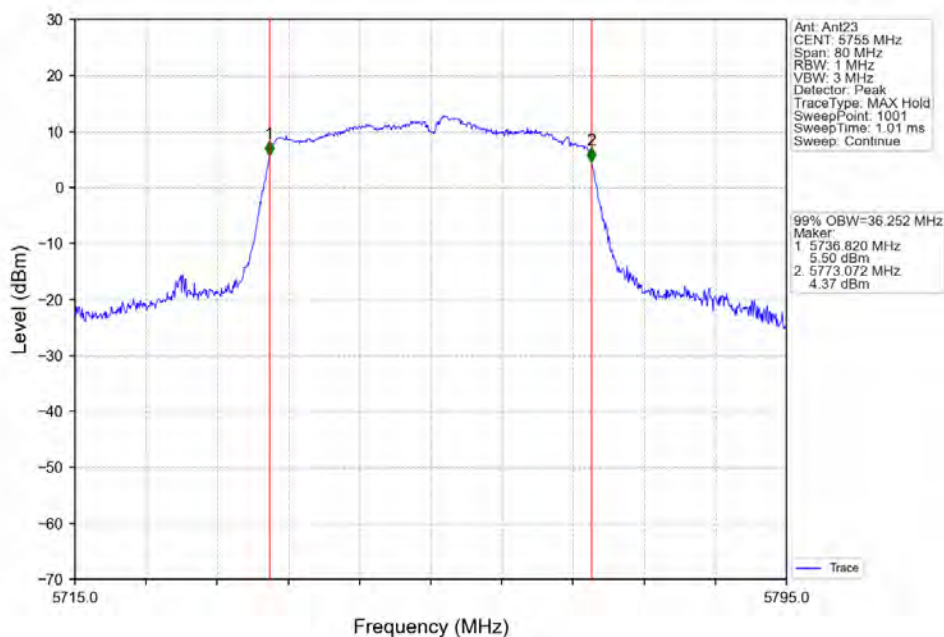
802.11ac(VHT40)_LCH_5755MHz_Ant23_NTNV
