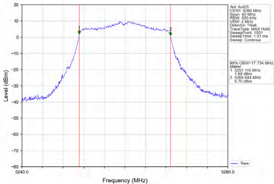
802.11ac(VHT20)_LCH_5260MHz_Ant23_NTNV
