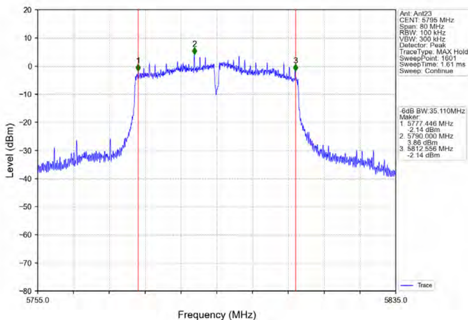
802.11ac(VHT40)_HCH_5795MHz_Ant23_NTNV
