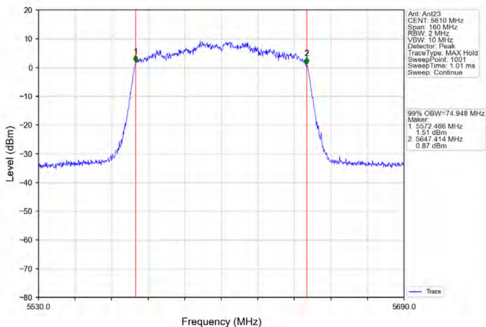
802.11ac(VHT80)_HCH_5610MHz_Ant23_NTNV
