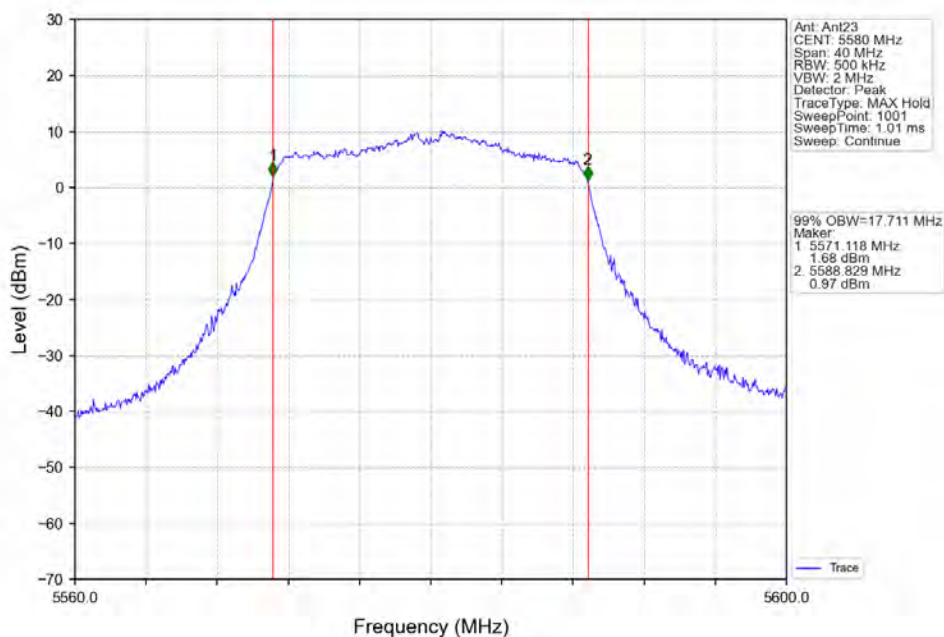
802.11ac(VHT20)_MCH_5580MHz_Ant23_NTNV
