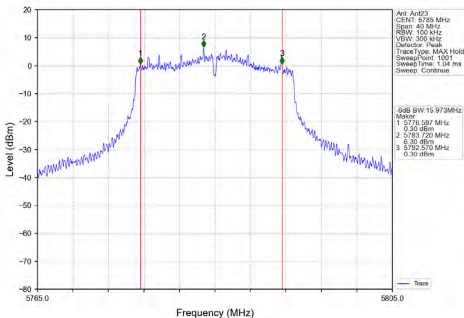
802.11n(HT20)_MCH_5785MHz_Ant23_NTNV
