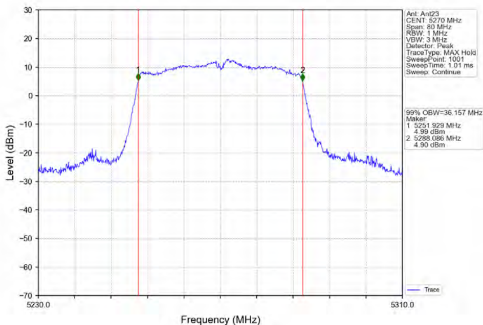
802.11ac(VHT40)_LCH_5270MHz_Ant23_NTNV
