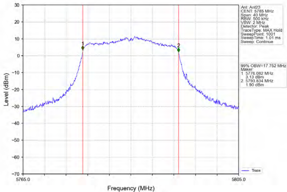
802.11ac(VHT20)_MCH_5785MHz_Ant23_NTNV
