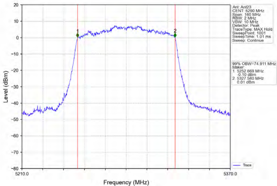
802.11ac(VHT80) MCH_5290MHz_Ant23_NTNV
