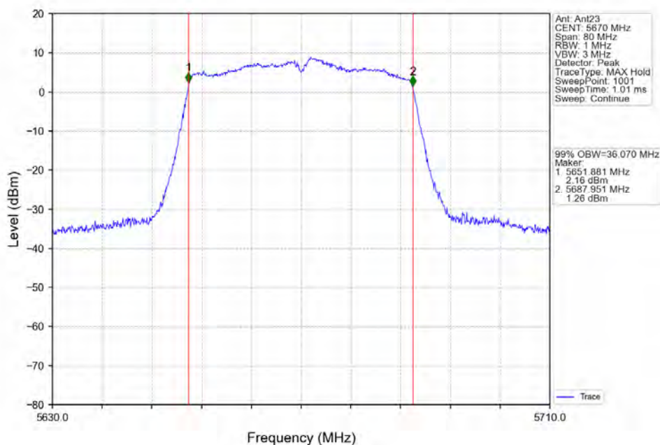
802.11ac(VHT40) HCH_5670MHz_Ant23_NTNV
