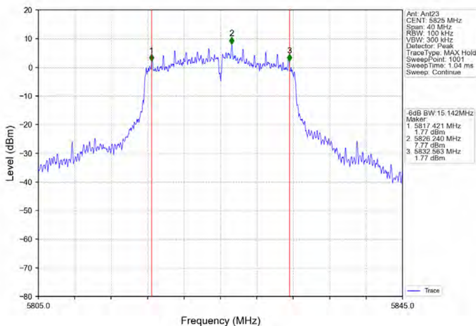
802.11a_HCH_5825MHz_Ant23_NTNV
