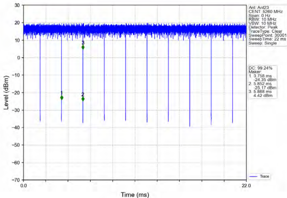
802.11a_LCH_5260MHz_Ant23_NTNV
