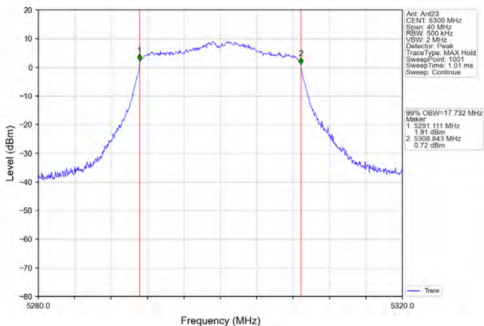
802.11n(HT20)_MCH_5300MHz_Ant23_NTNV
