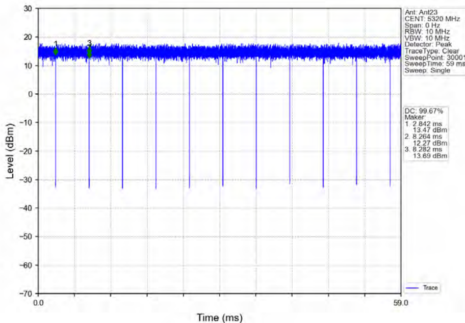
802.11ac(VHT20)_HCH_5320MHz_Ant23_NTNV
