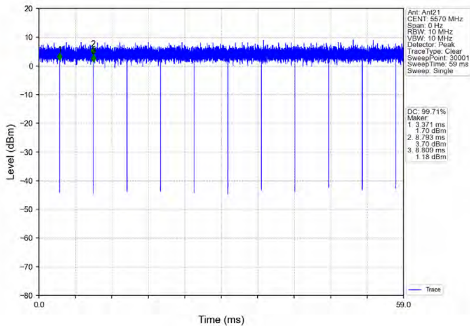
802.11ac(VHT160)_MCH_5570MHz_Ant21_NTNV
