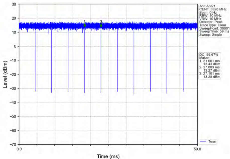
802.11ac(VHT20)_HCH_5320MHz_Ant21_NTNV
