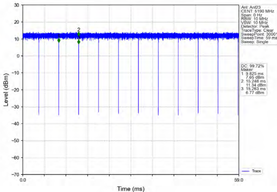
802.11ac(VHT40)_LCH_5190MHz_Ant23_NTNV
