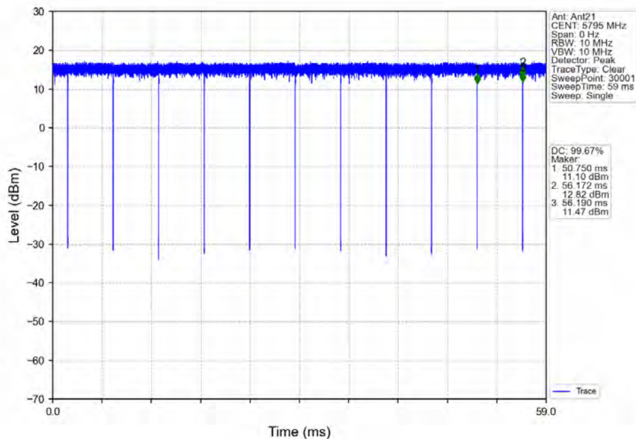
802.11ac(VHT40)_HCH_5795MHz_Ant21_NTNV
