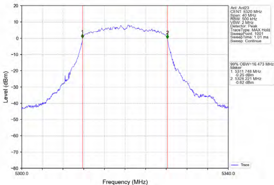
802.11a_HCH_5320MHz_Ant23_NTNV
