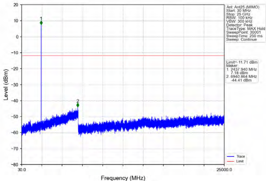
802.11ax(HEW20) MCH 2437MHz RU26 Mid_Ant25 (MIMO) NTN
