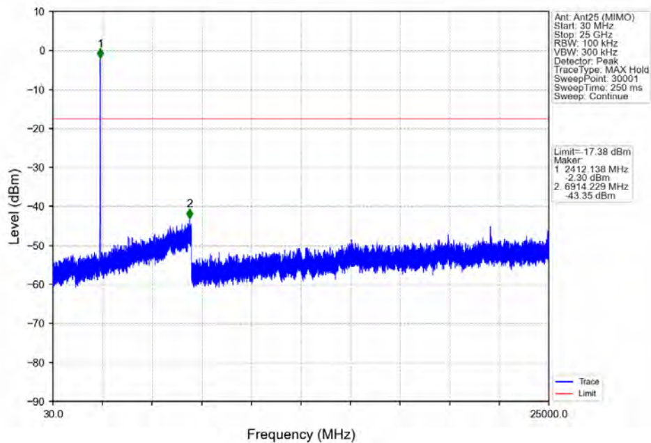
802.11ax(HEW20) LCH_2412MHz_RU242_Left_Ant25 (MIMO) NTN
