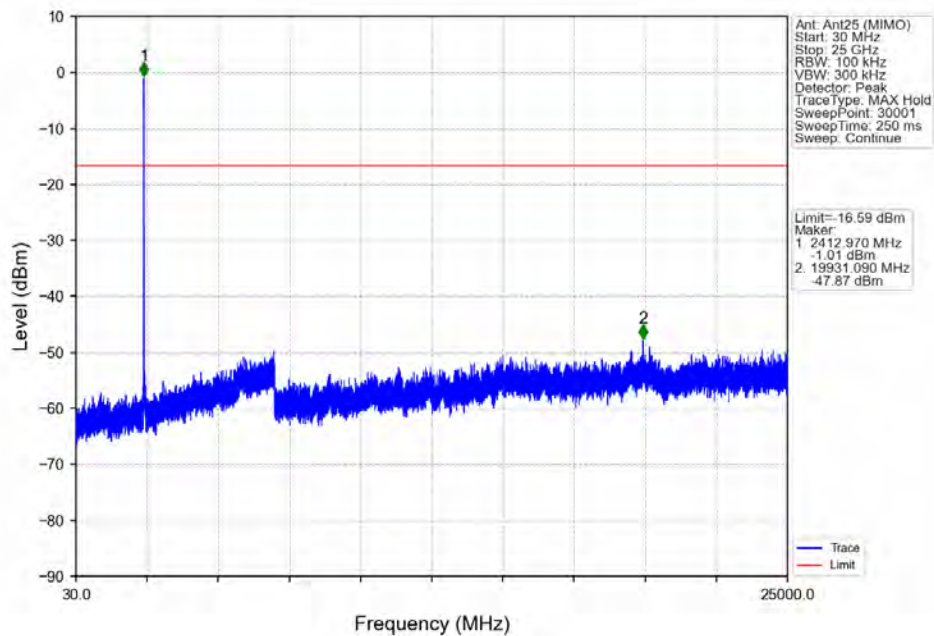
802.11ac(VHT20)_LCH_2412MHz_Ant25 (MIMO)_NTNV
