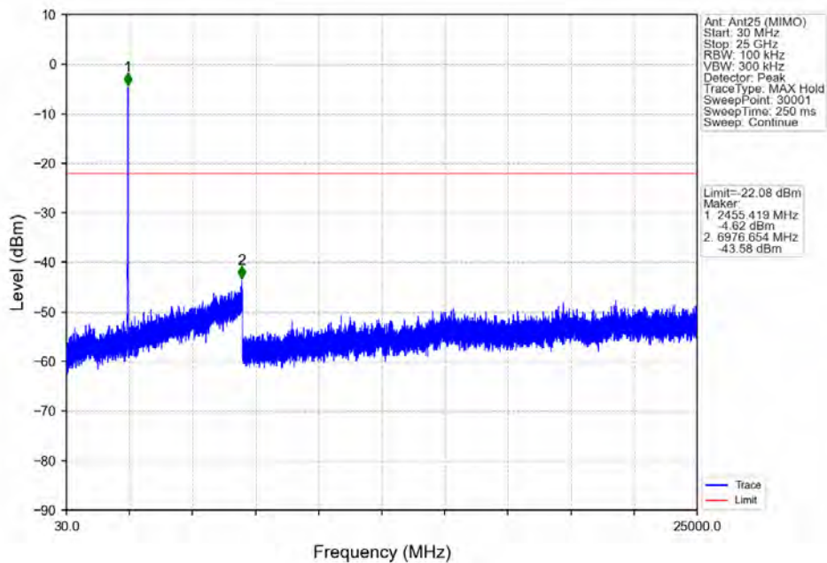
802.11ax(HEW40) HCH 2452MHz RU242 Right Ant25 (MIMO) NTNV
