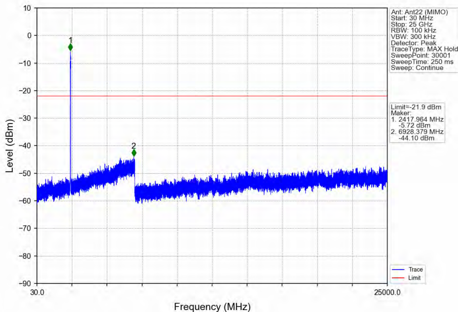
802.11ax(HEW40) LCH 2422MHz RU484 Left Ant22 (MIMO) NTN
