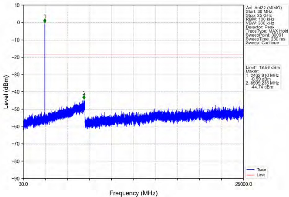
802.11ax(HEW20) HCH 2462MHz RU52 Right Ant22 (MIMO) NTN
