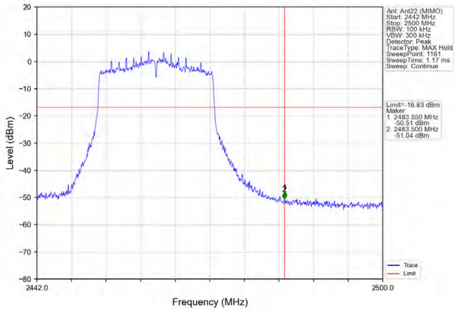
802.11ax(HEW20) HCH 2462MHz RU242 Left Ant22 (MIMO) NTN
