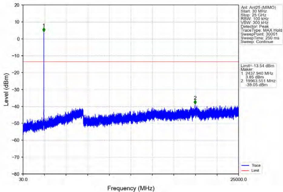
802.11ac(VHT20)_MCH_2437MHz_Ant25 (MIMO)_NTNV
