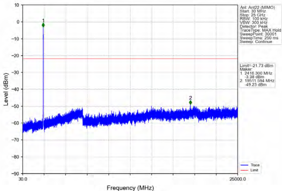
802.11ac(VHT40)_LCH_2422MHz_Ant22 (MIMO)_NTNV
