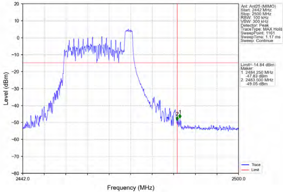
802.11ax(HEW20) HCH 2462MHz RU26 Right Ant25 (MIMO) NTN
