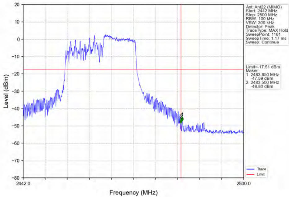
802.11ax(HEW20)_HCH_2462MHz_RU106_Right_Ant22 (MIMO)_NTNV
