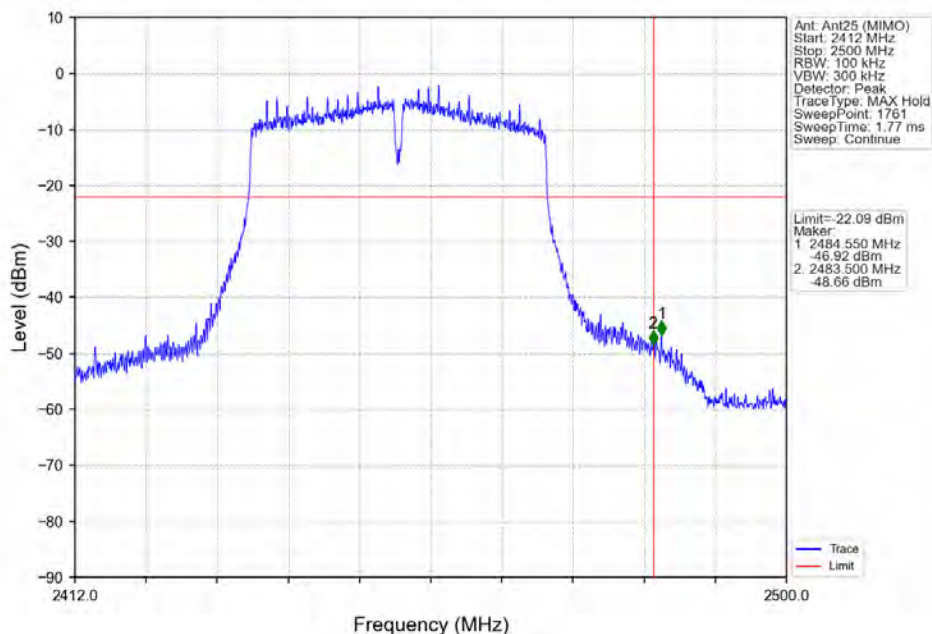
802.11ac(VHT40)_HCH_2452MHz_Ant25 (MIMO)_NTNV
