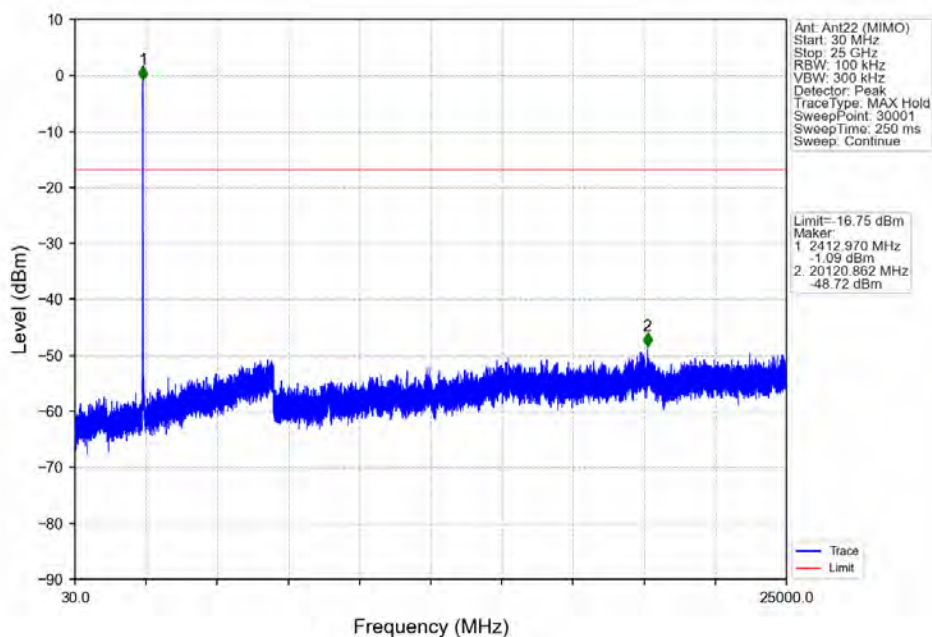
802.11ac(VHT20)_LCH_2412MHz_Ant22 (MIMO)_NTNV
