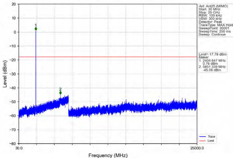
802.11ax(HEW20) LCH 2412MHz RU52 Left Ant25 (MIMO) NTN
