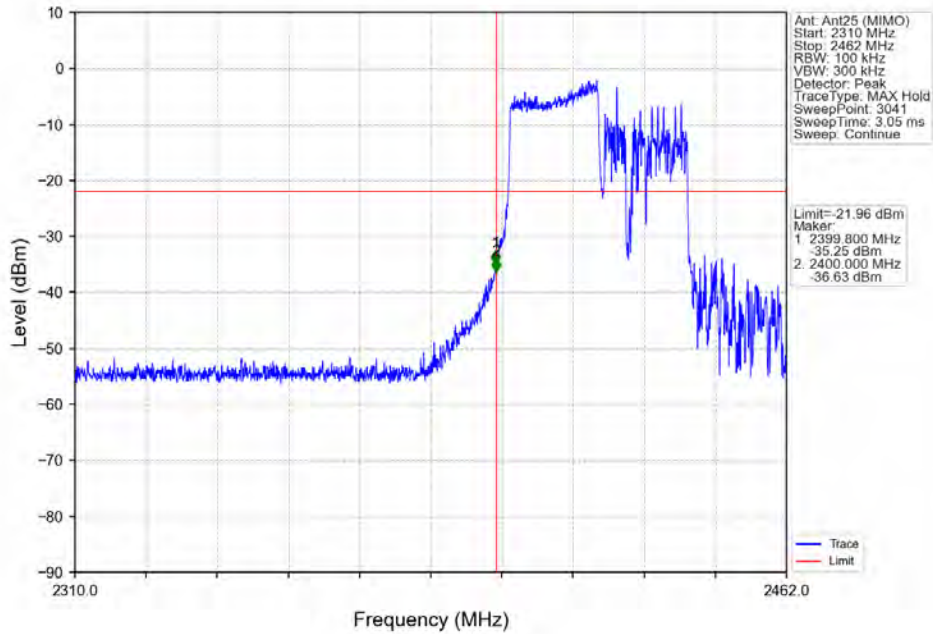
802.11ax(HEW40) LCH_2422MHz_RU242_Left_Ant25 (MIMO) NTN
