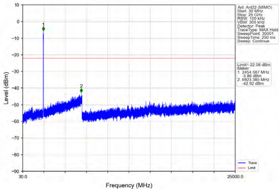
802.11ac(VHT40) HCH 2452MHz Ant22 (MIMO) NTNV
