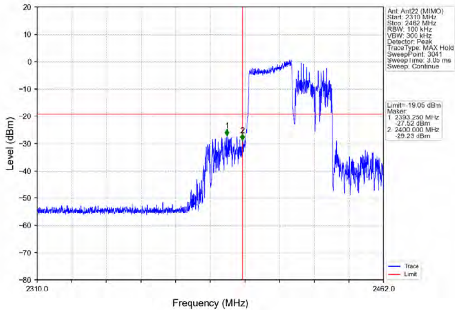
802.11ax(HEW40) LCH_2422MHz_RU242_Left_Ant22 (MIMO) NTN
