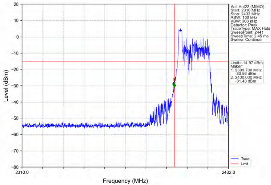
802.11ax(HEW20) LCH 2412MHz RU26 Left Ant22 (MIMO) NTN
