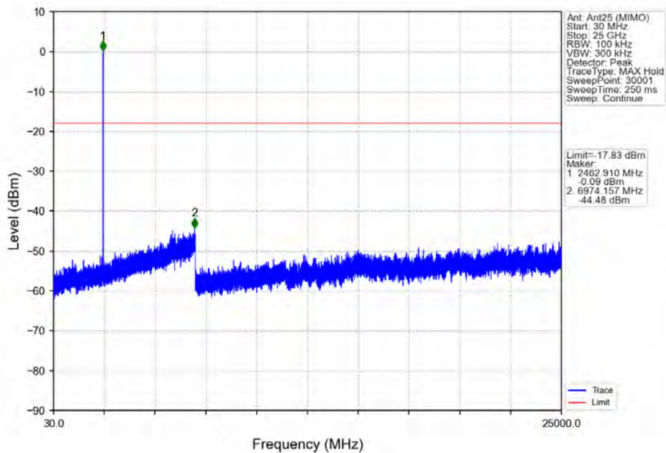
802.11ax(HEW20)_HCH_2462MHz_RU106_Right_Ant25 (MIMO)_NTNV
