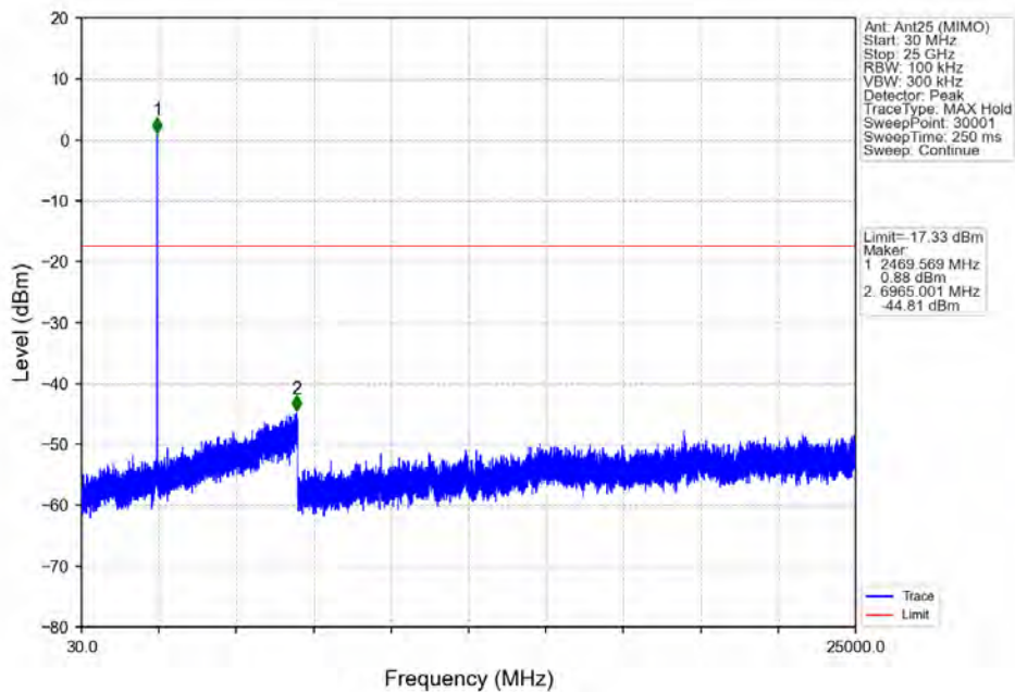
802.11ax(HEW20) HCH 2462MHz RU52 Right Ant25 (MIMO) NTN
