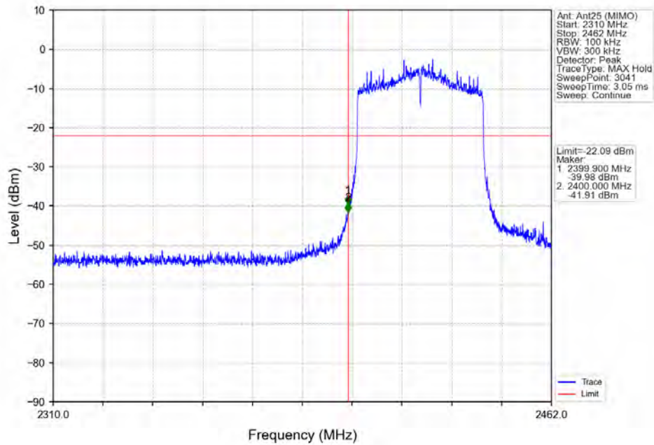
802.11ax(HEW40) LCH_2422MHz_RU484_Left_Ant25 (MIMO) NTN
