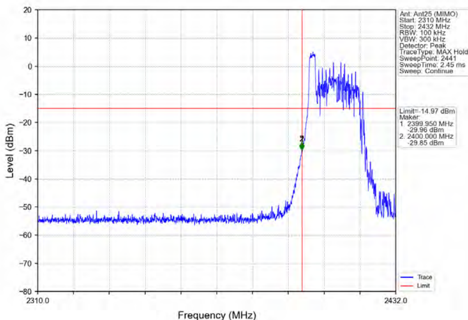
802.11ax(HEW20) LCH 2412MHz RU26 Left Ant25 (MIMO) NTN
