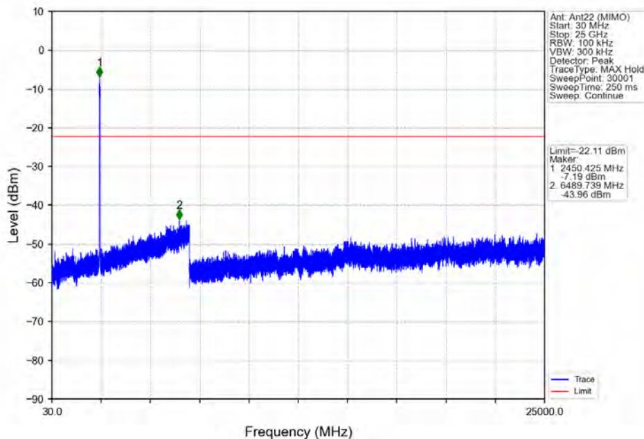
802.11ax(HEW40) HCH 2452MHz RU484 Left Ant22 (MIMO) NTN
