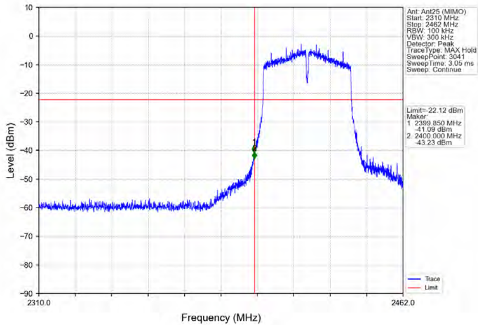
802.11ac(VHT40)_LCH_2422MHz_Ant25 (MIMO)_NTNV
