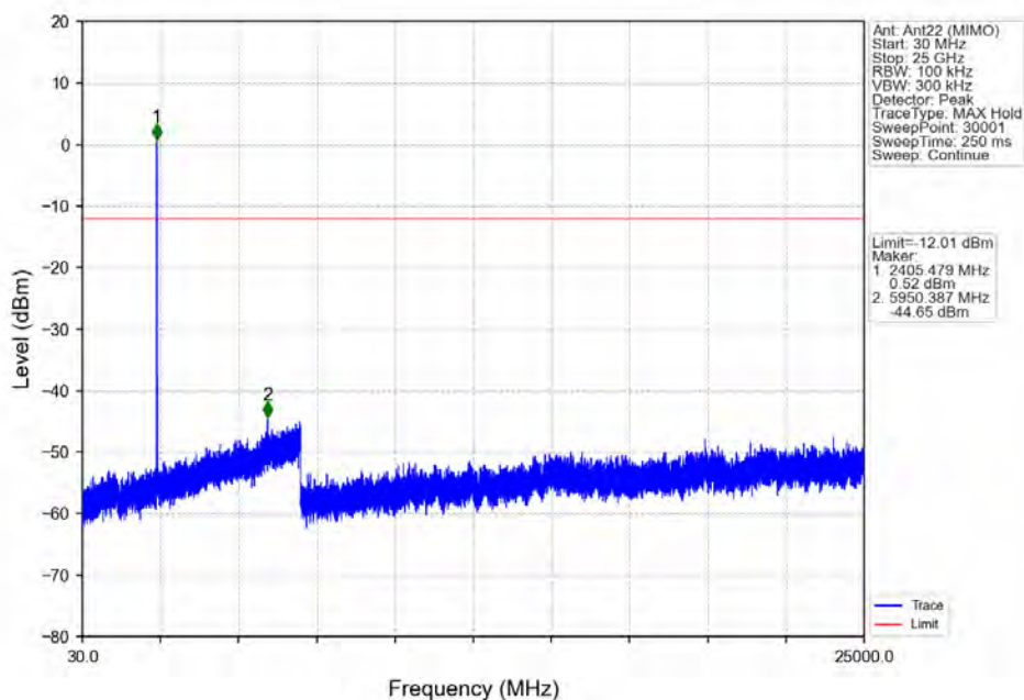
802.11ax(HEW20) LCH 2412MHz RU52 Left Ant22 (MIMO) NTN
