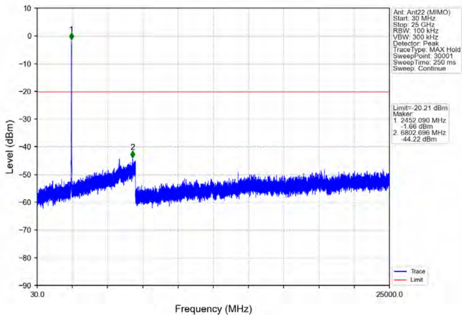
802.11ax(HEW40) HCH 2452MHz RU242 Right Ant22 (MIMO) NTNV
