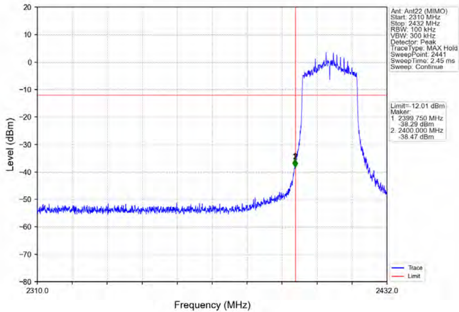
802.11ax(HEW20) LCH_2412MHz_RU242_Left_Ant22 (MIMO) NTN
