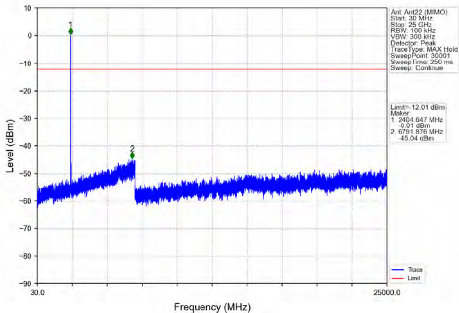
802.11ax(HEW20) LCH_2412MHz_RU106_Left_Ant22 (MIMO) NTN
