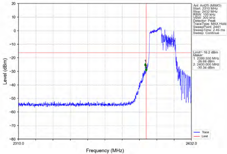
802.11ax(HEW20) LCH 2412MHz RU106 Left Ant25 (MIMO) NTN
