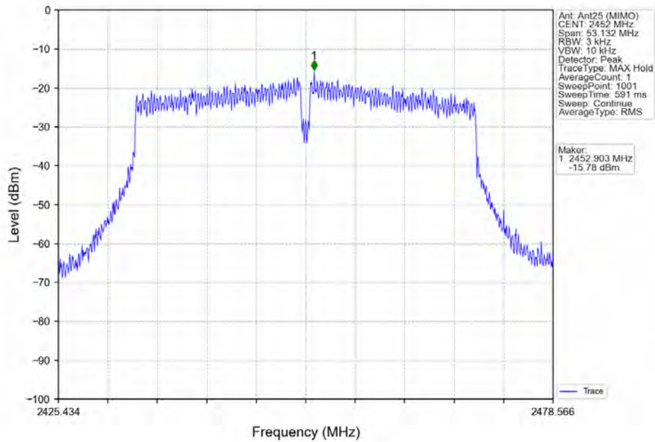
802.11ac(VHT40)_HCH_2452MHz_MIMO_NTNV
