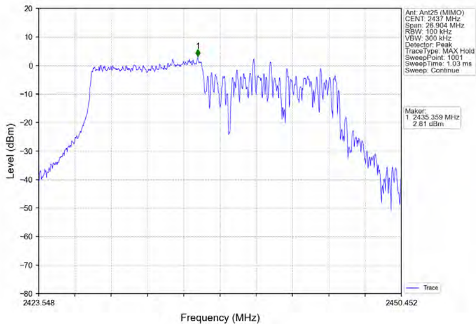
802.11ax(HEW20) MCH 2437MHz RU106 Left Ant25 (MIMO) NTV
