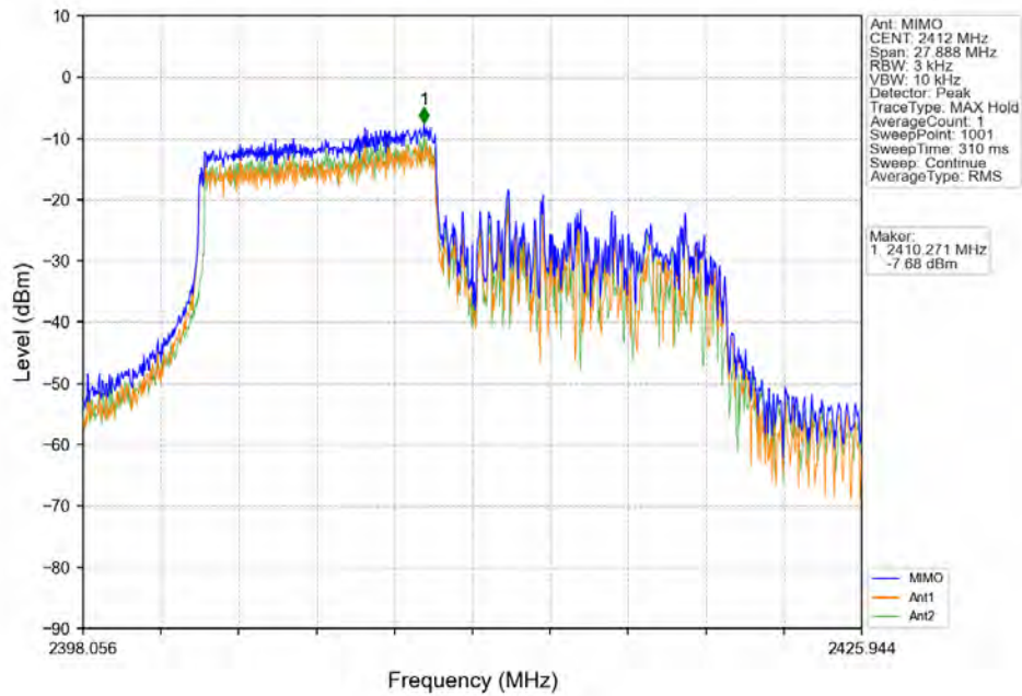
802.11ax(HEW20) LCH 2412MHz RU242 Left Ant22 (MIMO) NTN
