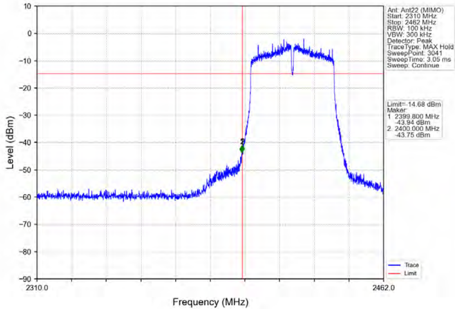
802.11n(HT40) LCH 2422MHz Ant22 (MIMO) NTNV
