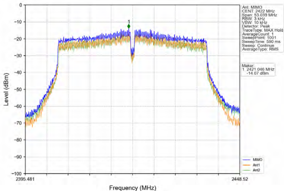
802.11ac(VHT40)_LCH_2422MHz_MIMO_NTNV
