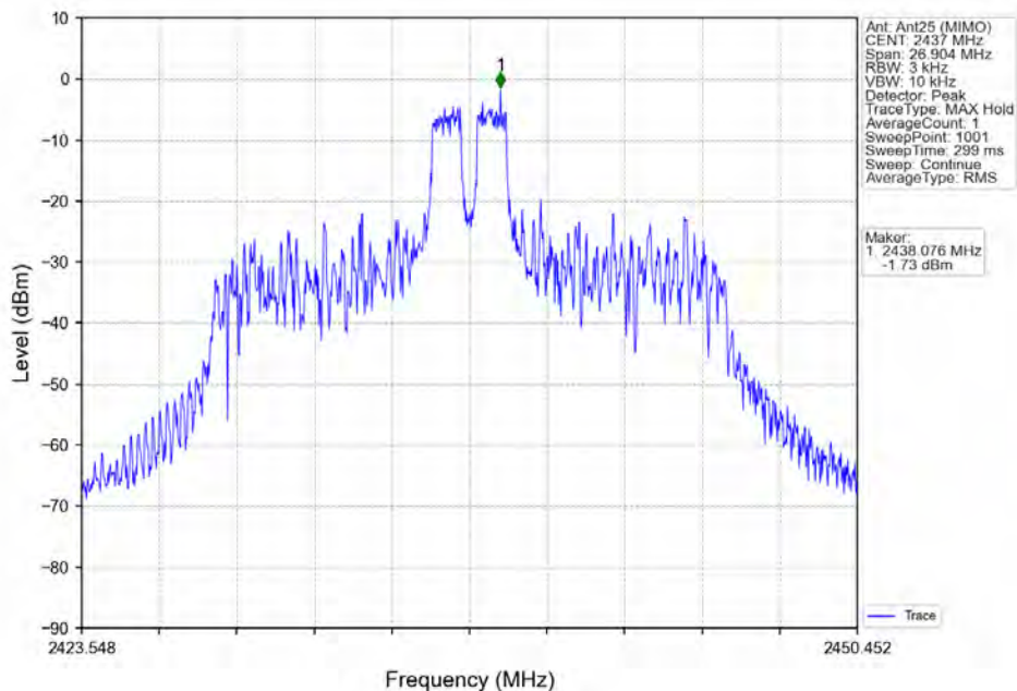
802.11ax(HEW20) MCH 2437MHz RU26 Mid_Ant25 (MIMO) NTNV
