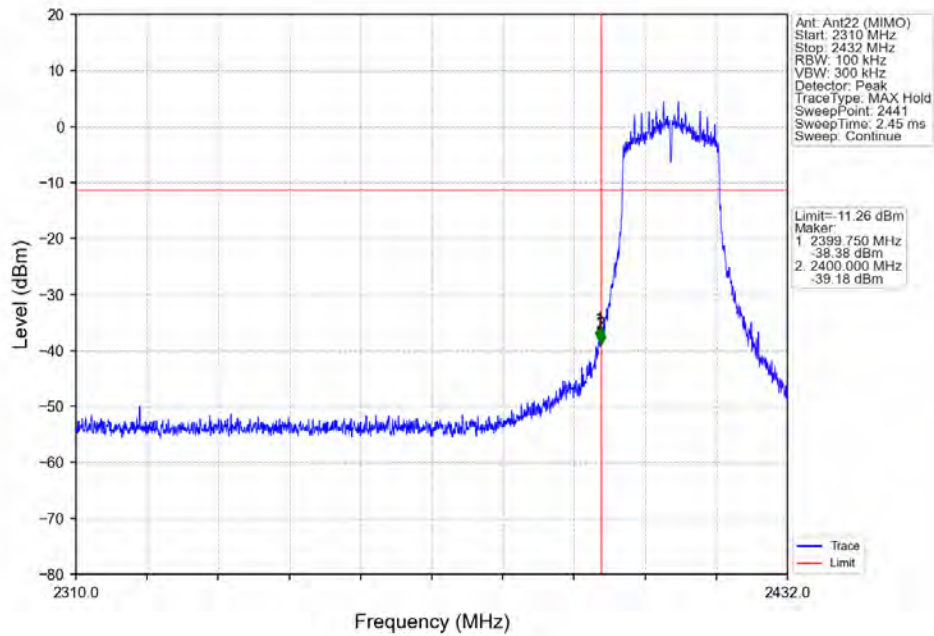
802.11g_LCH_2412MHz_Ant22 (MIMO) NTN
