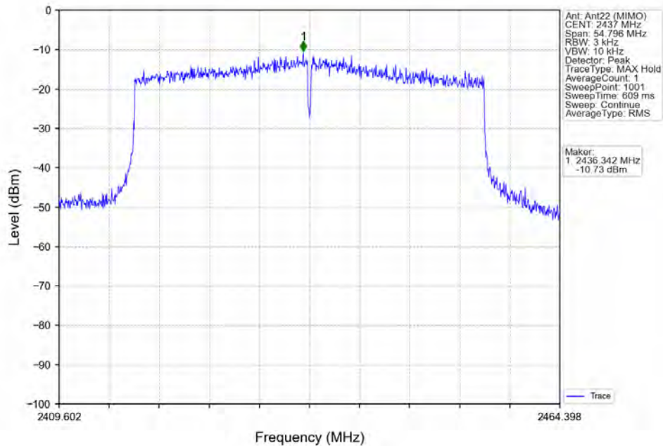
802.11ax(HEW40) MCH_2437MHz RU484 Left Ant22 (MIMO) NTN
