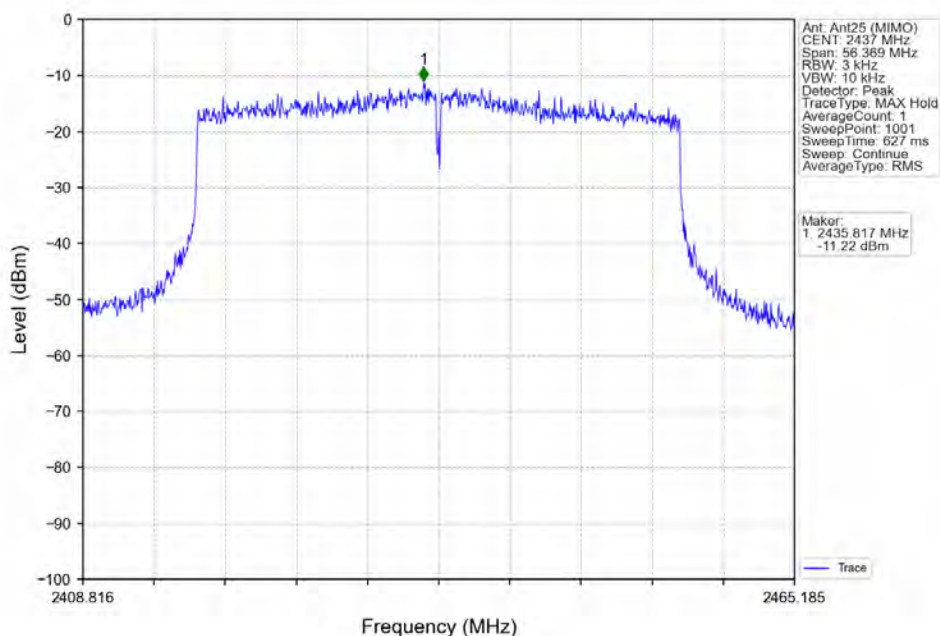
802.11ax(HEW40) MCH 2437MHz RU484 Left MIMO NTN
