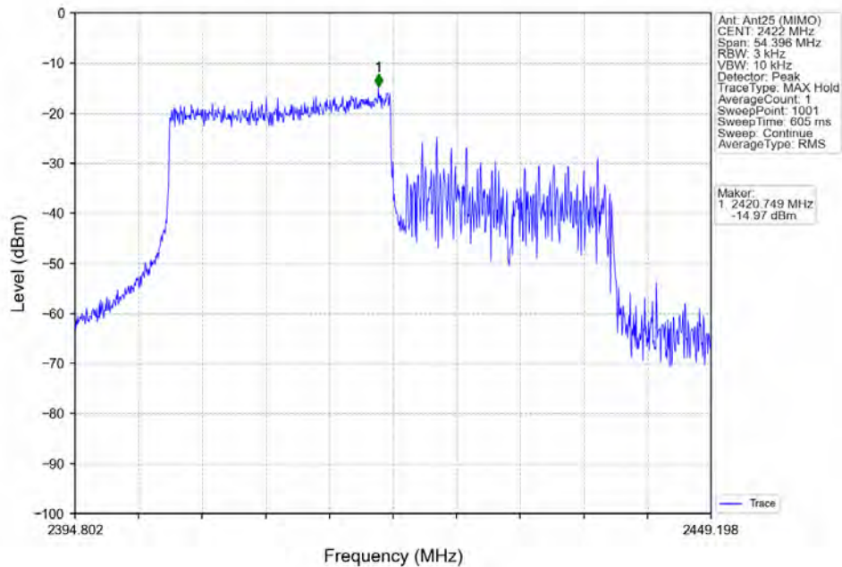
802.11ax(HEW40) LCH_2422MHz_RU242_Left_Ant25 (MIMO) NTN
