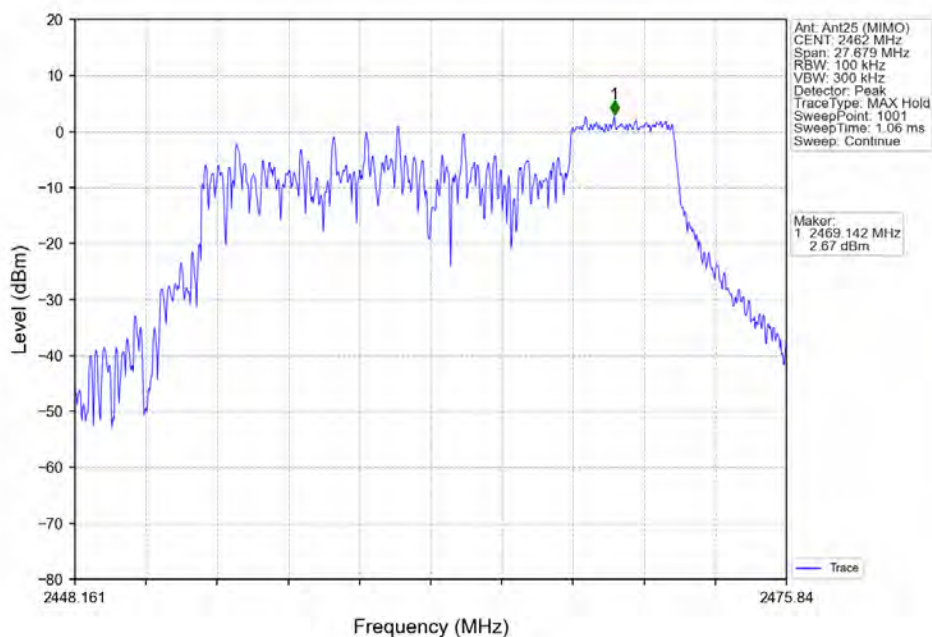
802.11ax(HEW20) HCH 2462MHz RU52 Right Ant25 (MIMO) NTV
