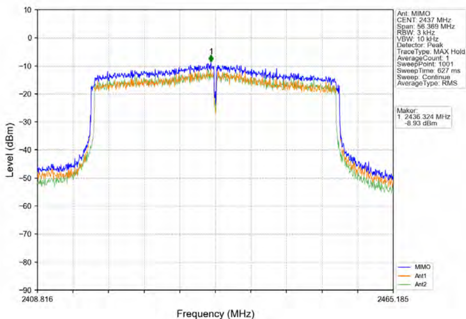
802.11ax(HEW40) MCH 2437MHz RU484 Left MIMO NTN
