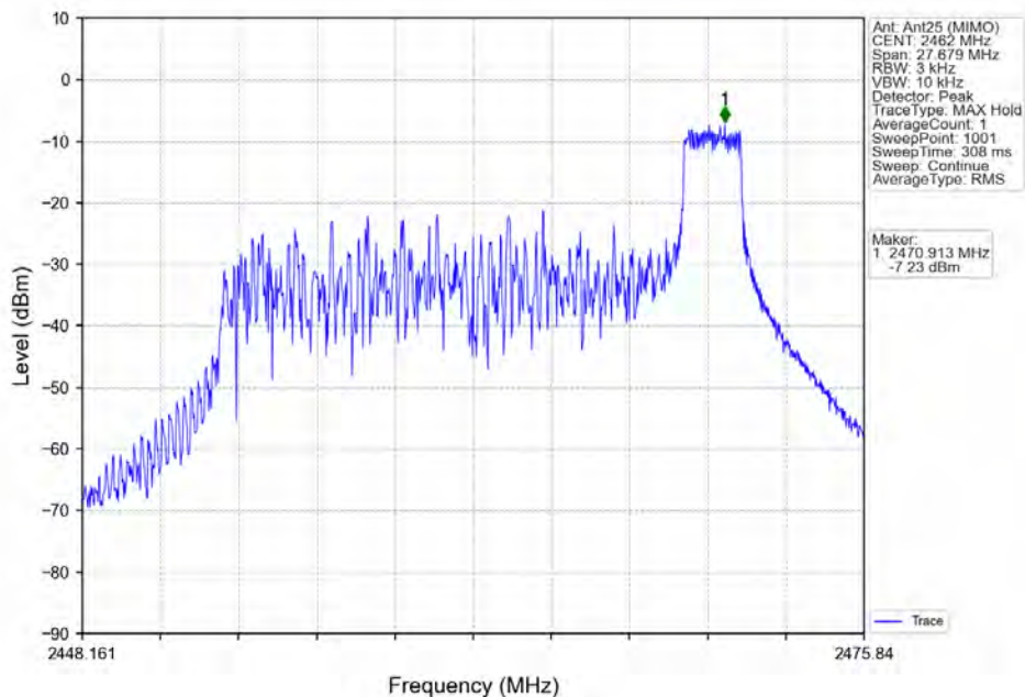
802.11ax(HEW20) HCH 2462MHz RU26 Right Ant25 (MIMO) NTV
