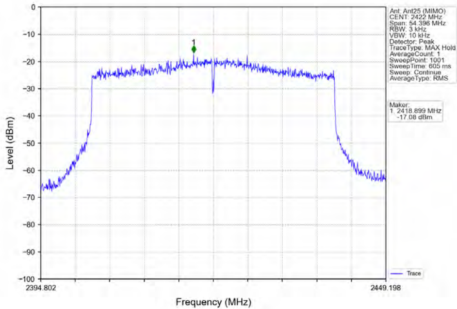
802.11ax(HEW40) LCH 2422MHz RU484 Left MIMO NTNV
