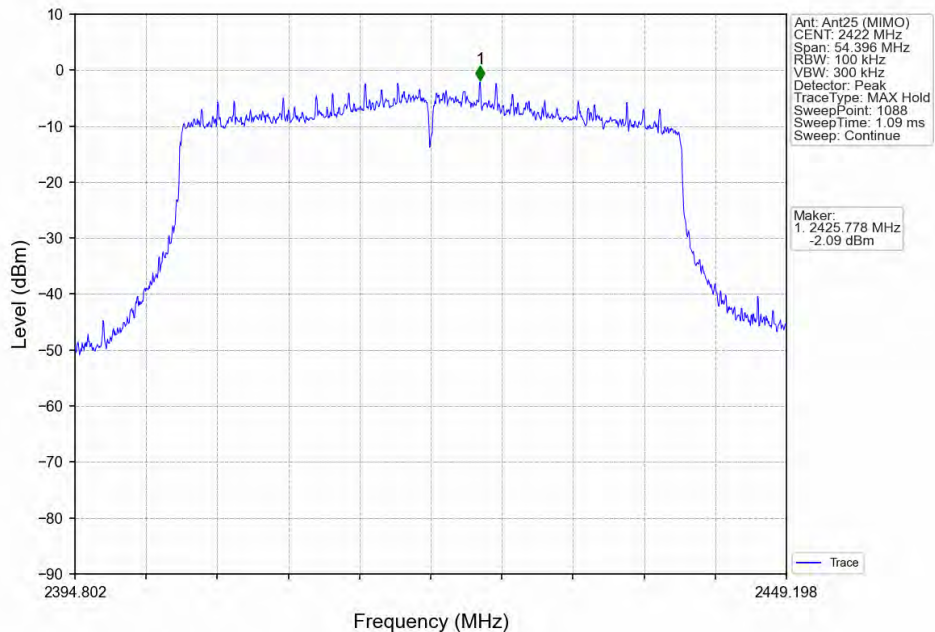
802.11ax(HEW40) LCH_2422MHz_RU484_Left_Ant25 (MIMO) NTNV
