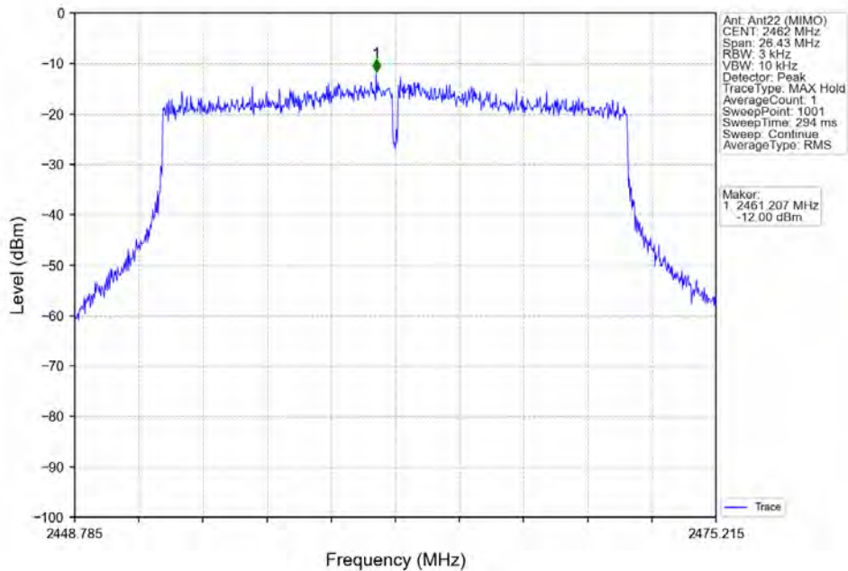
802.11ax(HEW20) HCH_2462MHz RU242 Left Ant22 (MIMO) NTN
