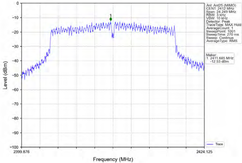
802.11g_LCH_2412MHz_MIMO NTN
