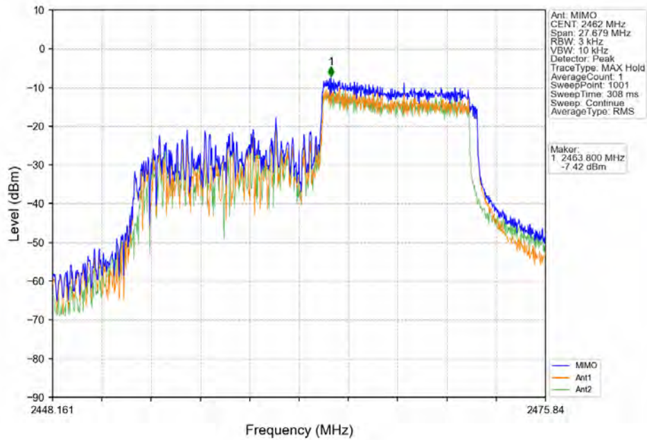
802.11ax(HEW20) HCH_2462MHz RU242 Left Ant22 (MIMO) NTN
