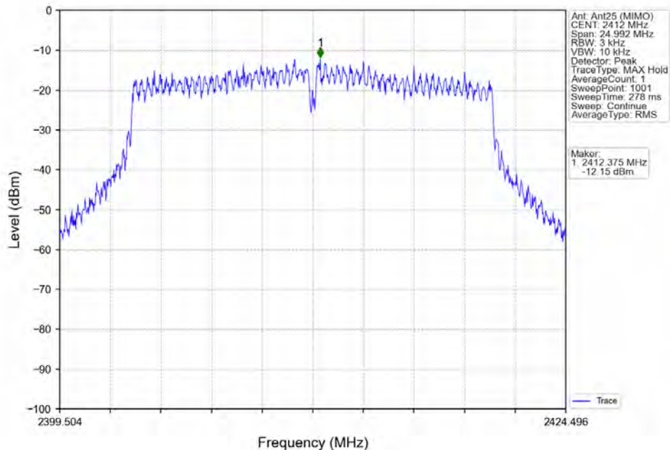
802.11ac(VHT20)_LCH_2412MHz_Ant25 (MIMO)_NTNV
