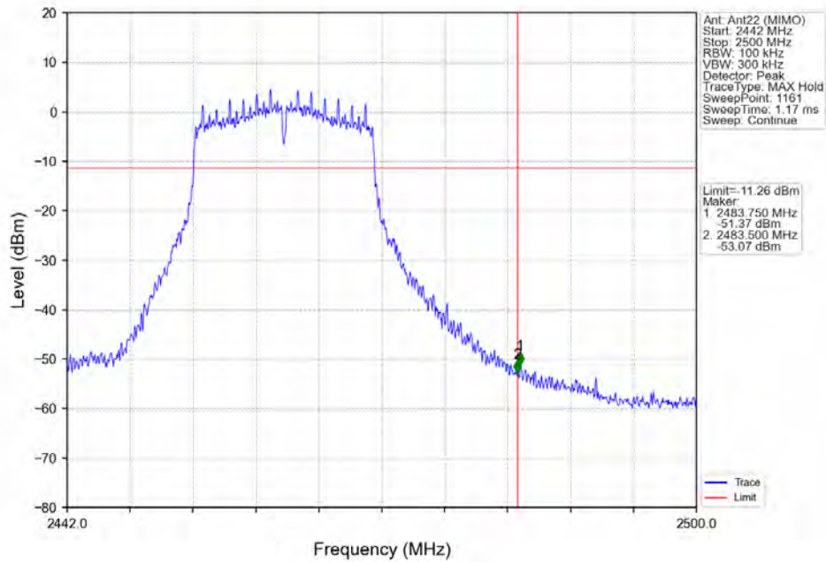
802.11g_HCH_2462MHz_Ant22 (MIMO)_NTNV
