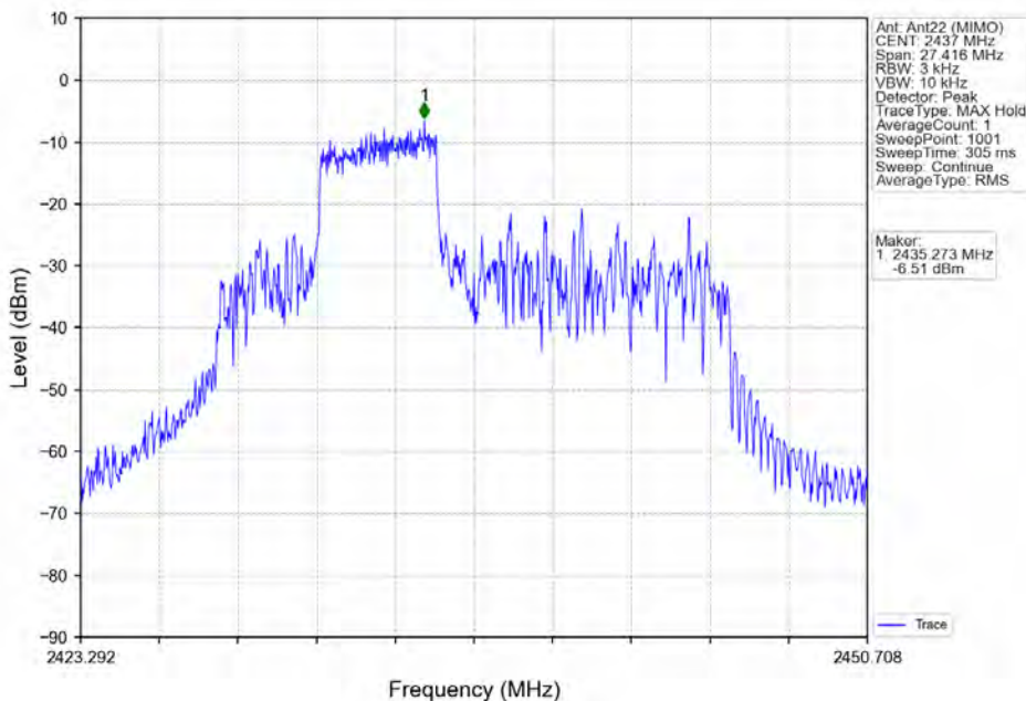
802.11ax(HEW20) MCH 2437MHz RU52 Mid Ant22 (MIMO) NTN
