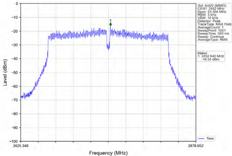
802.11ac(VHT40)_HCH_2452MHz_Ant22 (MIMO)_NTNV
