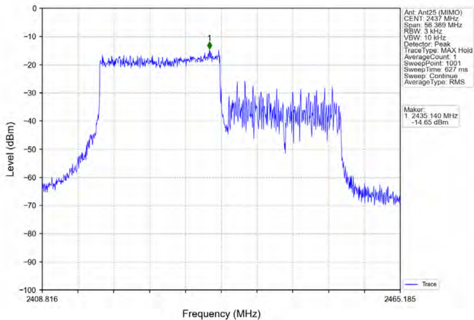
802.11ax(HEW40) MCH 2437MHz RU242 Left Ant25 (MIMO) NTVN
