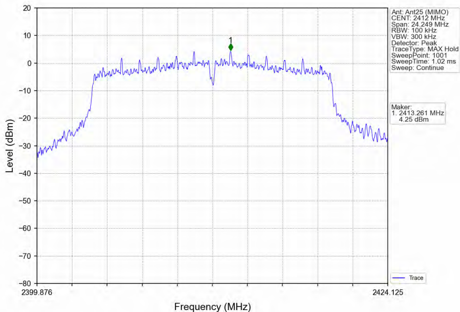
802.11g_LCH_2412MHz_Ant25 (MIMO) NTN
