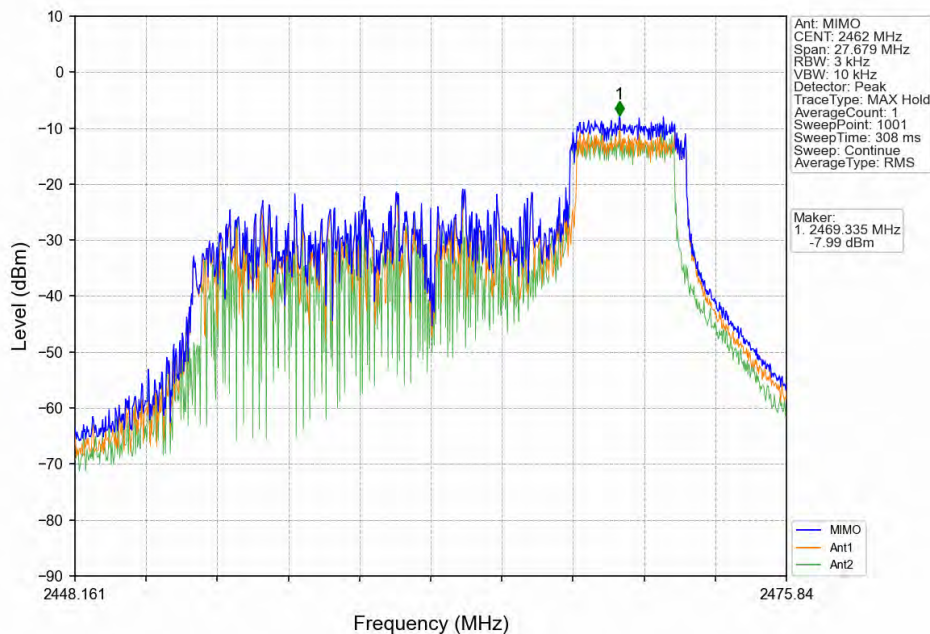
802.11ax(HEW20) HCH 2462MHz RU52 Right MIMO NTN
