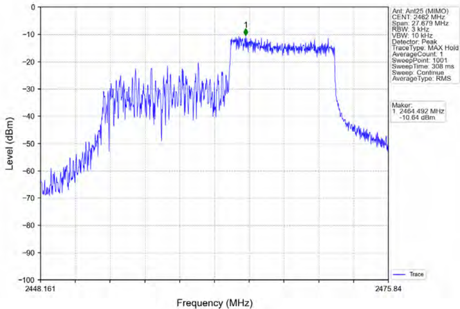
802.11ax(HEW20)_HCH_2462MHz_RU106_Right_Ant25 (MIMO) NTN
